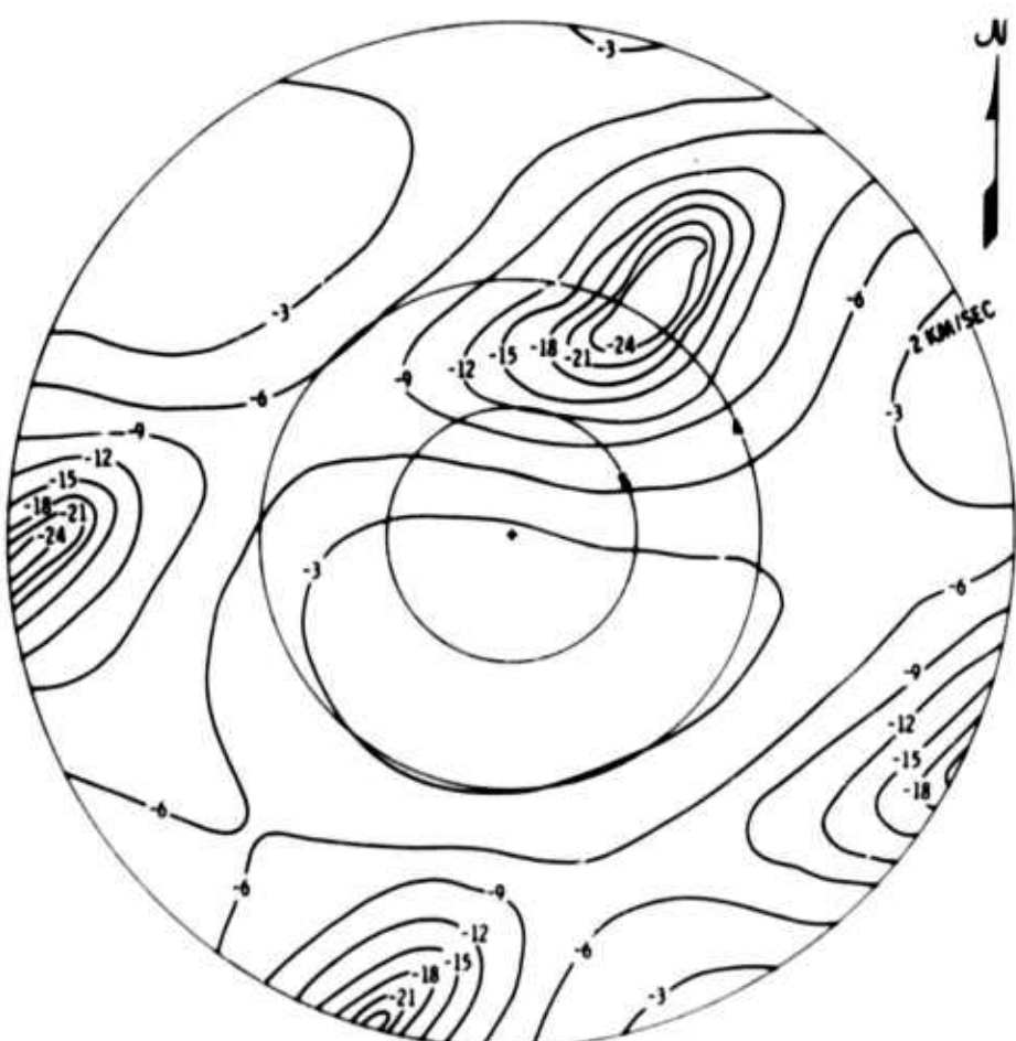
Figure IV-6. Wavenumber Response of 5-Channel MCF, Dispersive Signal Model, at 0.06 Hz
