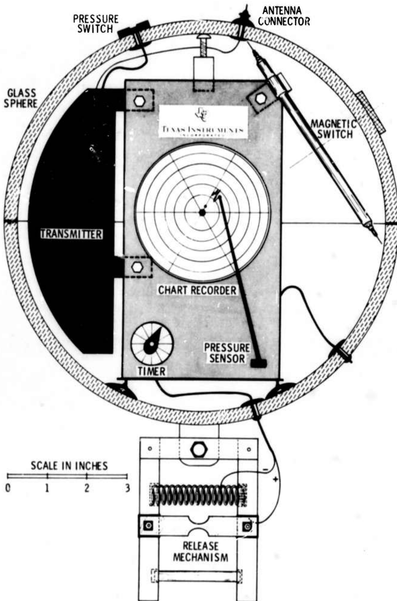
Figure II-2. Proposed Charge-Depth Recording Package
