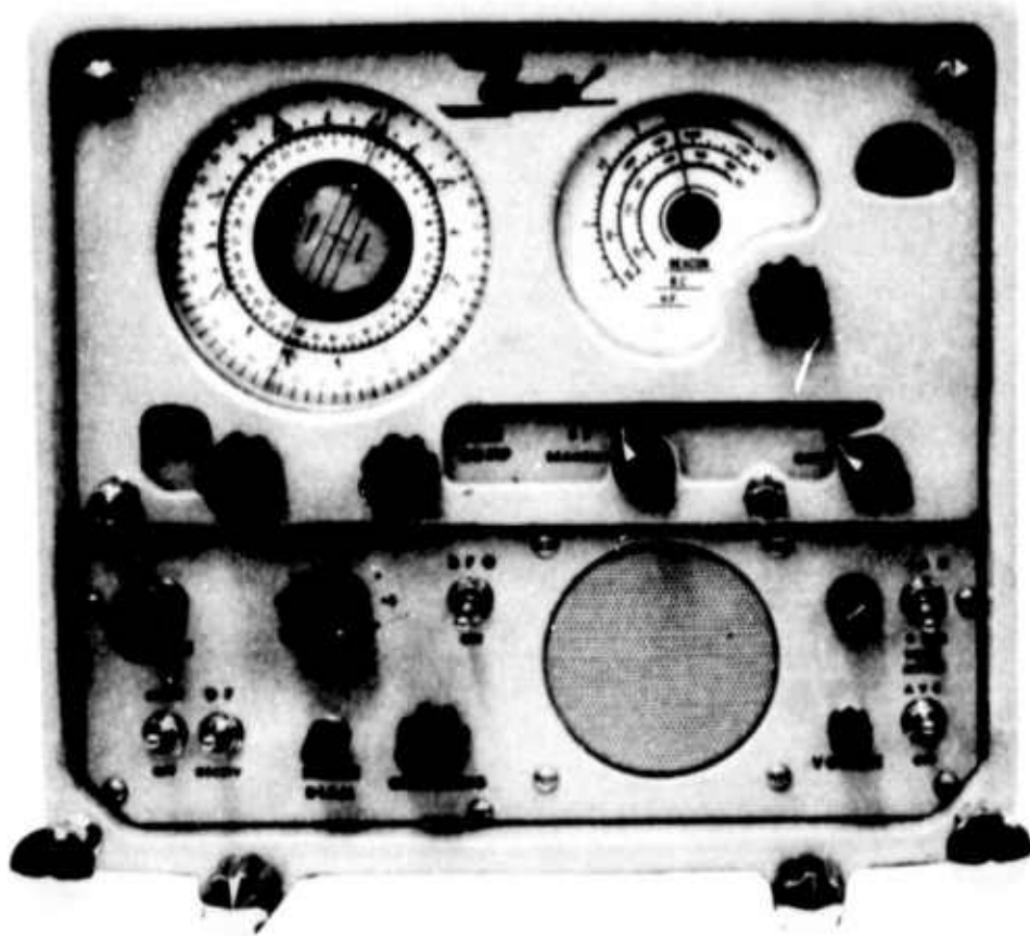
Figure III-4. Bendix Automatic Direction-Finder Model 100
