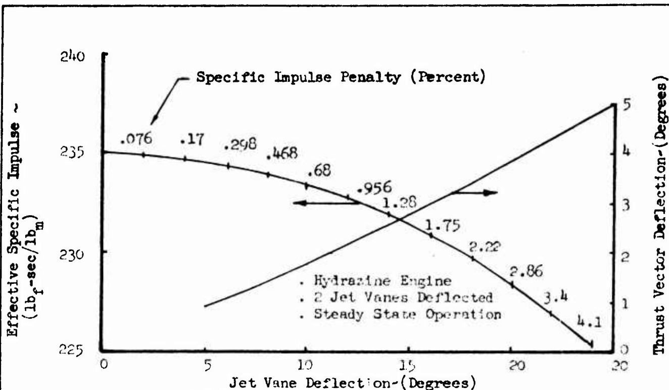
FIGURE 7.3-2 TYPICAL JET VANE TVC PERFORMANCE
