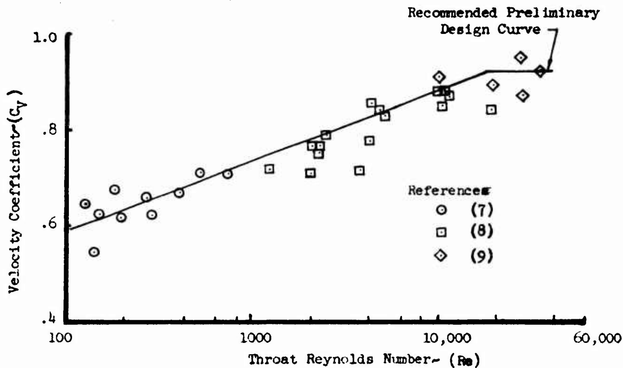
FIGURE 5.2-2 VELOCITY COEFFICIENT
