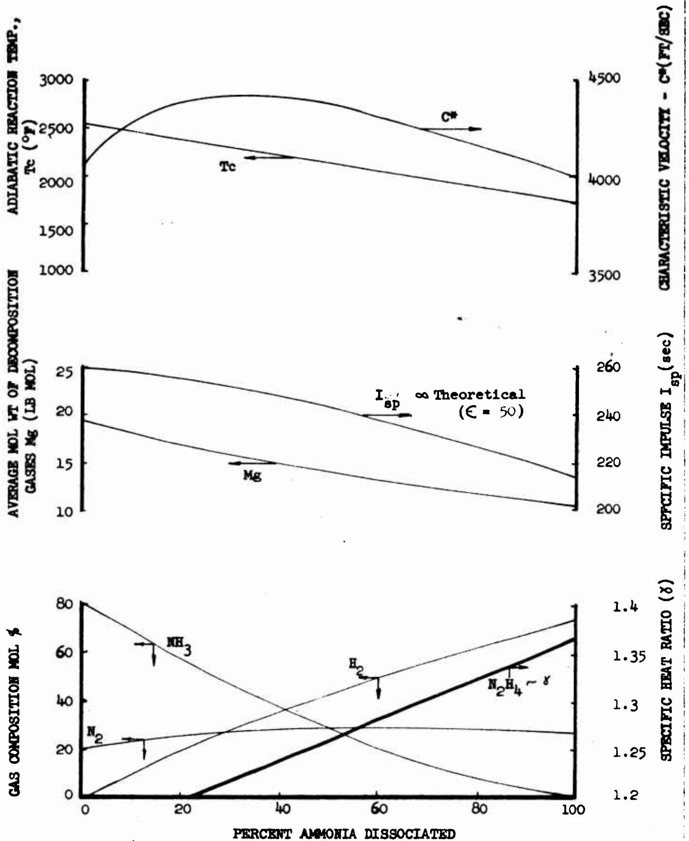
FIGURE 6.3-20 HYDRAZINE PERFORMANCE CURVES (100% N_2H_4 ) (Ref. 26)
