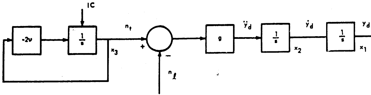
FIGURE 4. SIMPLIFIED HOMING SYSTEM
