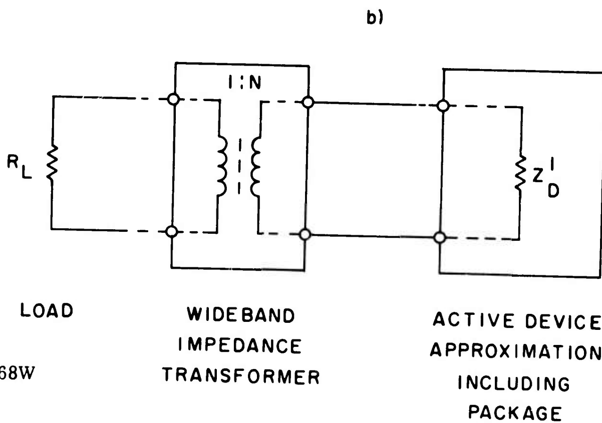
FIGURE 7 AVALANCHE OSCILLATOR DESIGN PRINCIPLES
