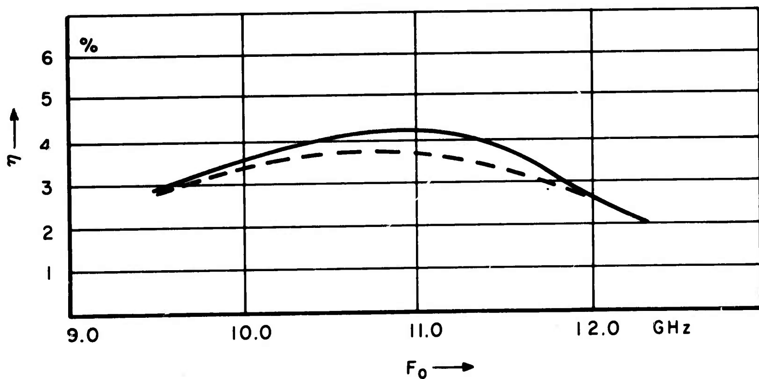
FIGURE 2 OUTPUT POWER OF AN AVALANCHE OSCILLATOR AS A FUNCTION OF FREQUENCY
