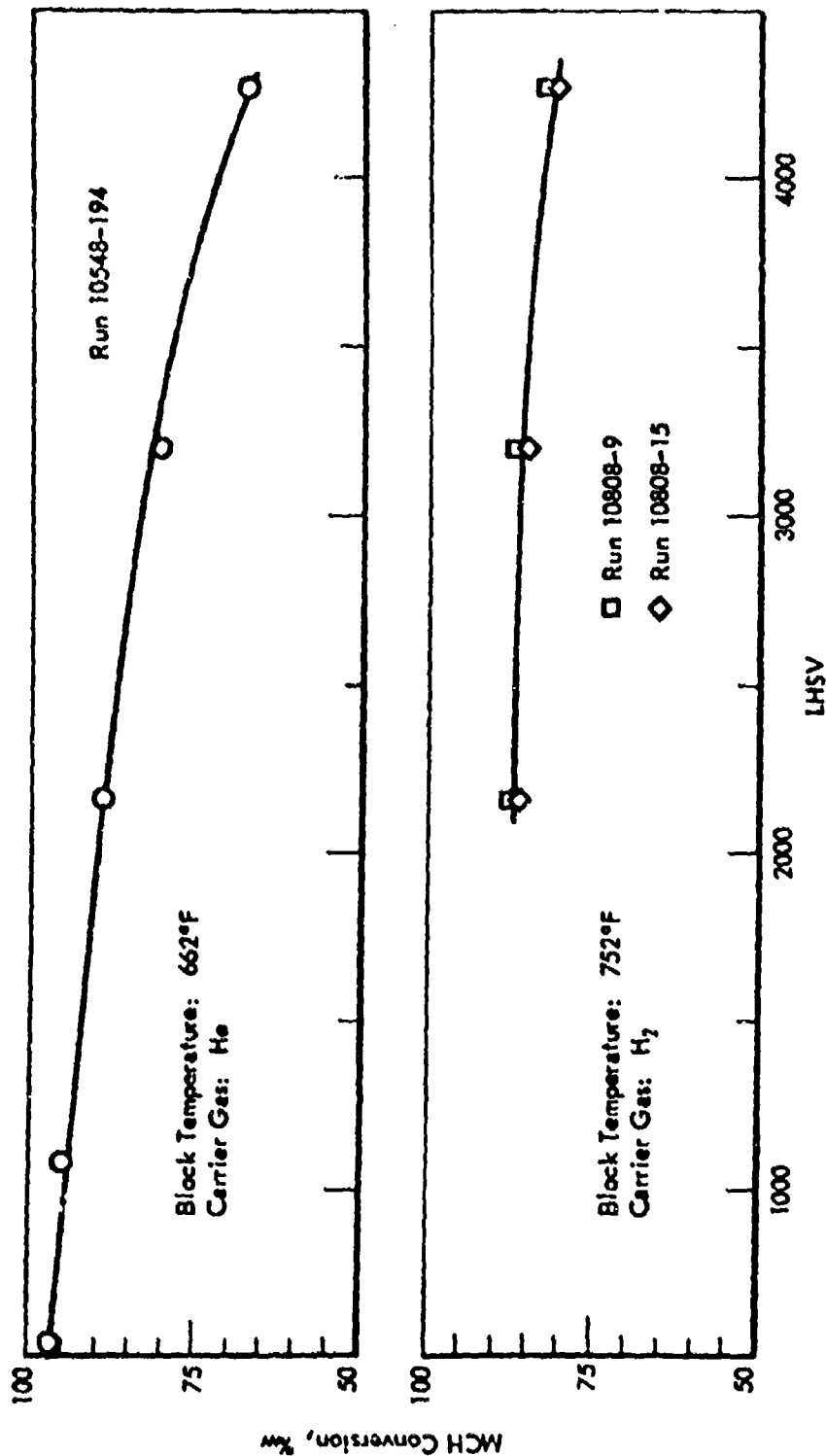
Figure 7. DEHYDROGENATION OF METHYLCYCLOHEXANE: PULSE REACTOR - EFFECT OF LHSV ON CONVERSION
