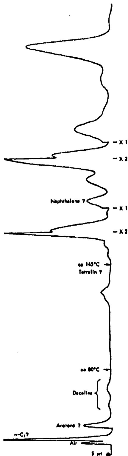
Figure 73. GLC ANALYSIS OF ADSORBATE FROM DECALIN PURIFICATION
