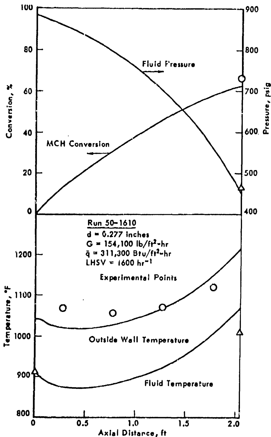
Figure 47. CALCULATED PROFILES FOR MCH DEHYDROGENATION IN THE FSSTR FROM FSSTR KINETIC DATA
