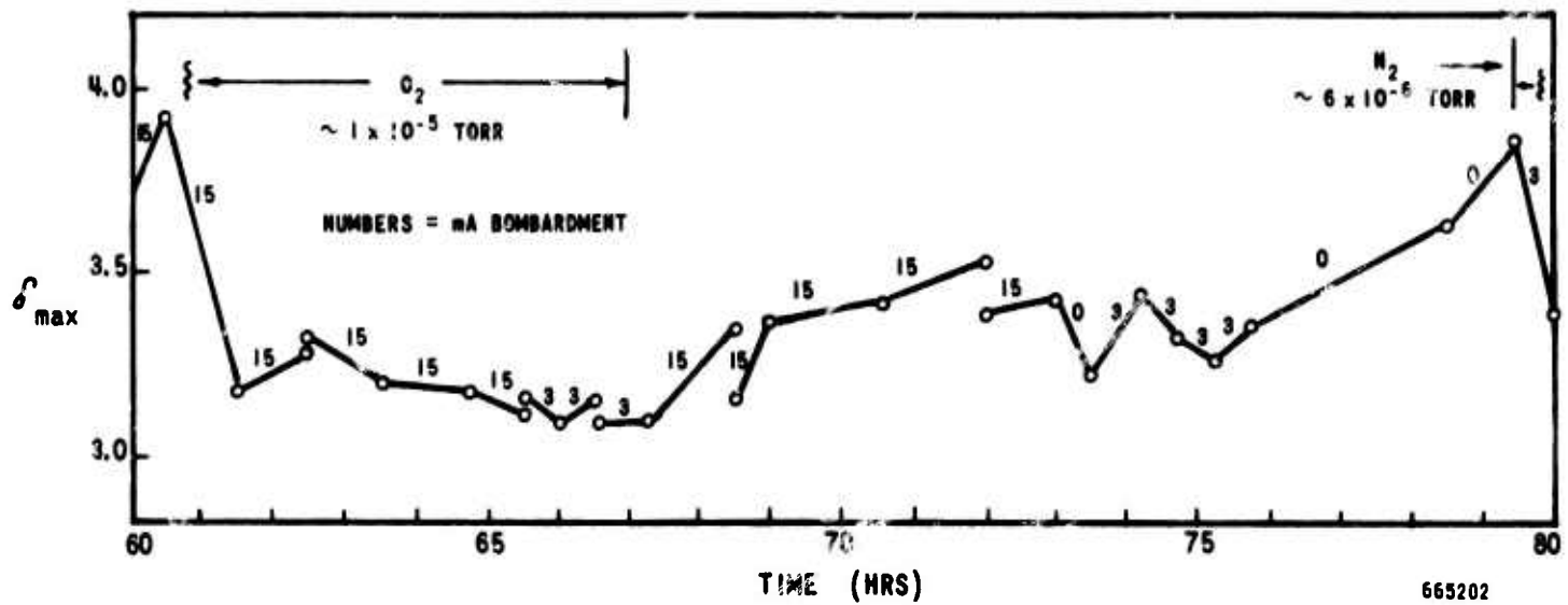
Figure 1, Sheet 2. \delta_{max} vs EBV Time for 300Å Anodized Beryllium
