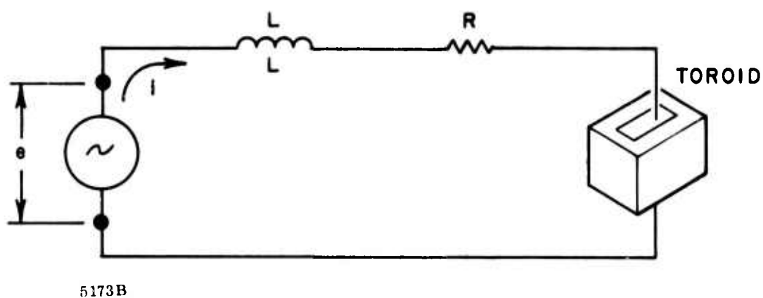
Figure 27. Equivalent Phase Shifter Driver-Load Circuit
