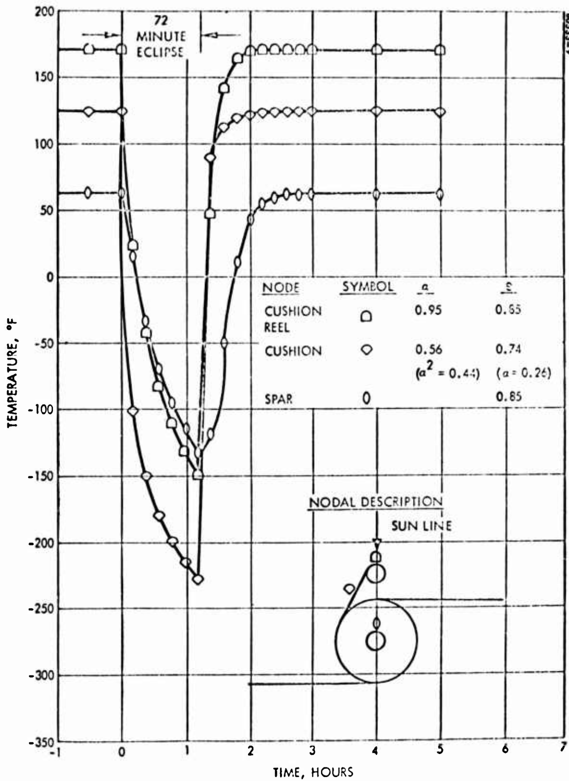
b) Cushion, Cushion Reel, and Spar
