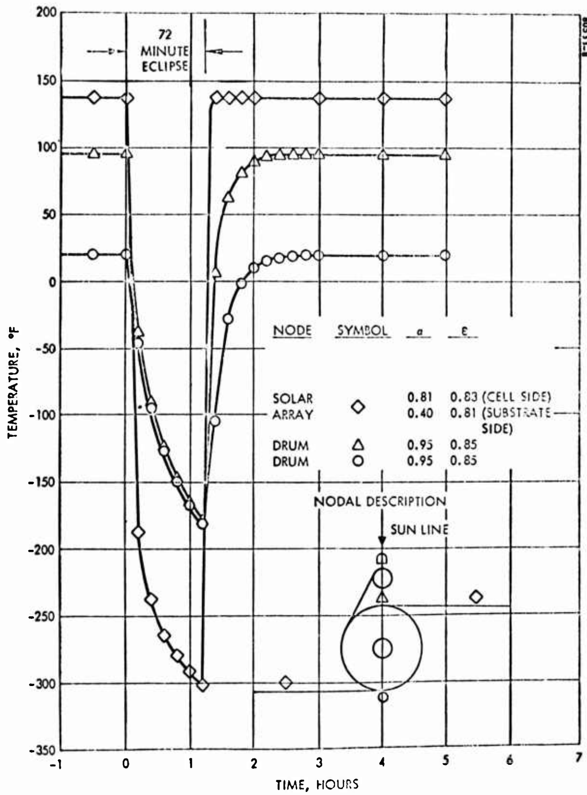
a) Solar Array and Storage Drum
