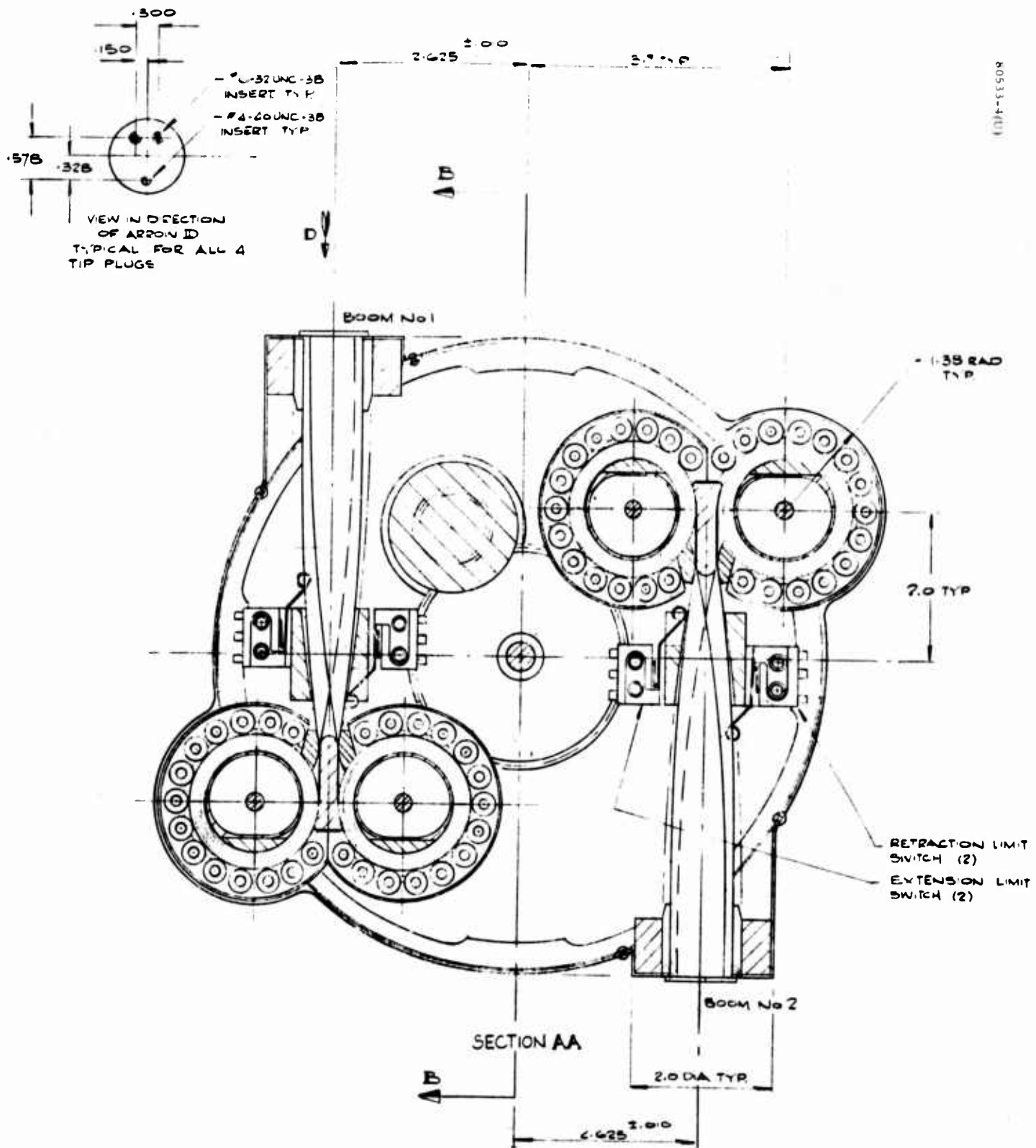
Figure 4. Details of Extensible Boom Actuator Unit
