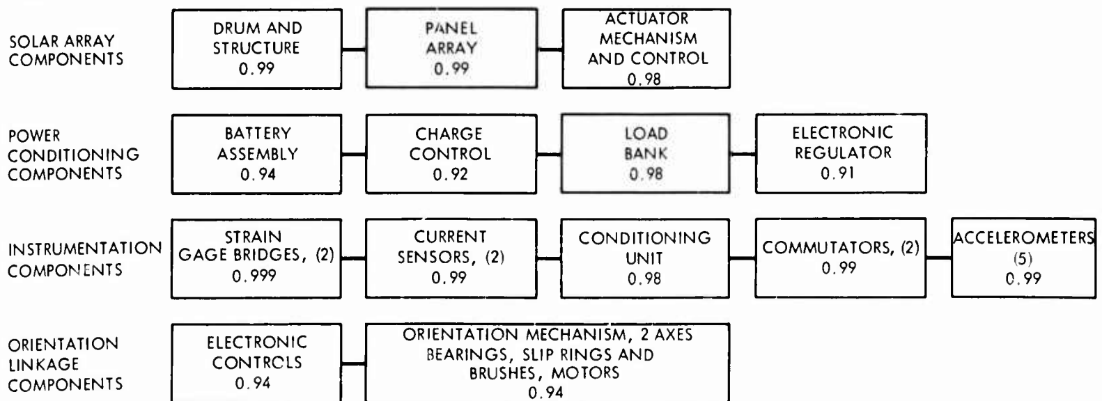
Figure 11. Reliability Apportionment for 1.5 kw Design System reliability goal 0.65 for 1 year
