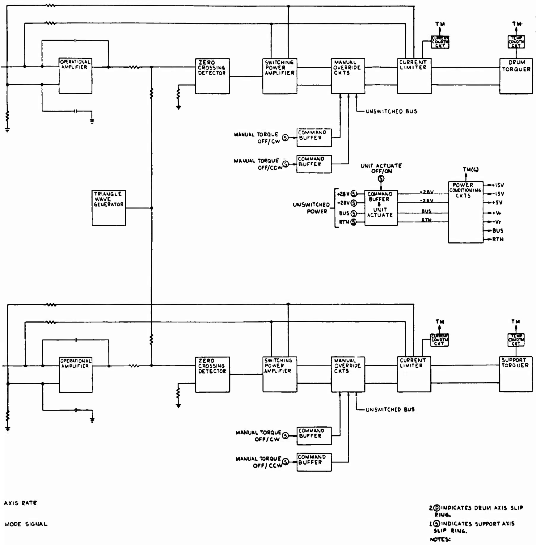
Figure 9. Control Electronics Unit Mechanization
