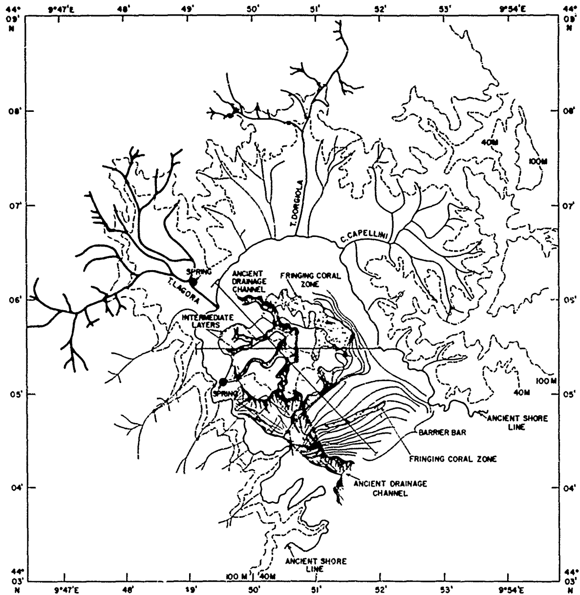
FIG. 25 SUB-BOTTOM GEOLOGY IN THE GULF OF LA SPEZIA
