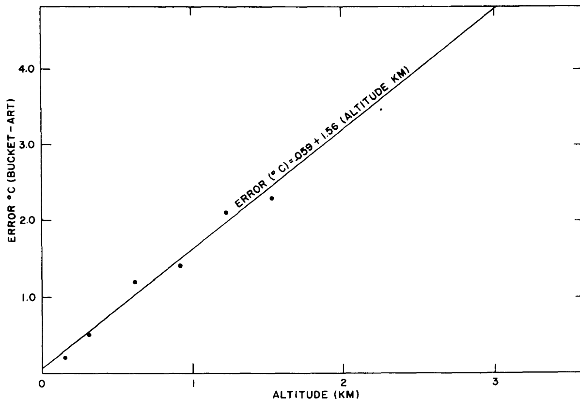
Figure 13 Radiation Thermometer Error as a Function of Altitude—Nighttime
