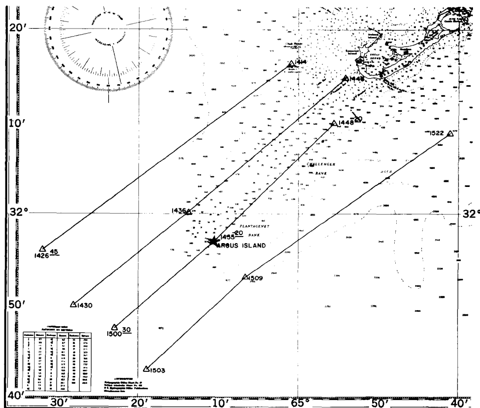
Figure 7 Sea Surface Temperature Flight Track—10 March 1966
