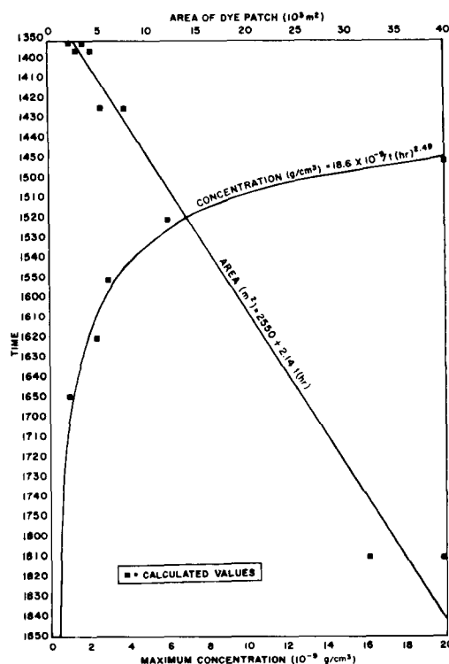
Figure 16 Characteristics of Dye Patch as a Function of Time
