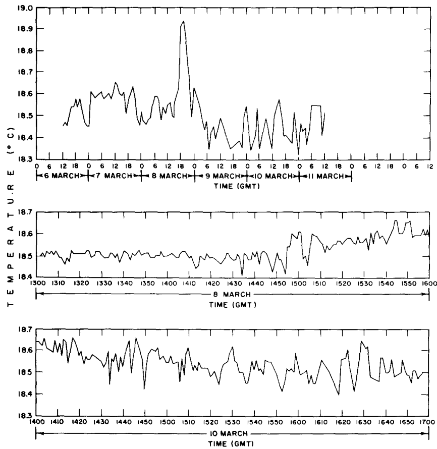
FIGURE A-1 Sea Surface Temperature, ARGUS ISLAND 6-11 March 1966
