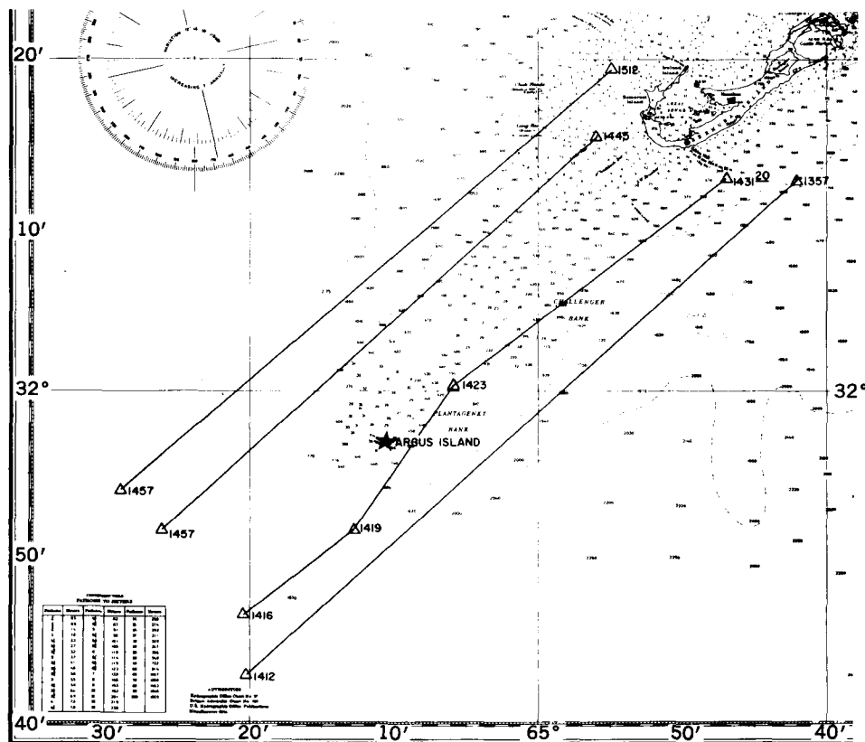
Figure 6 Sea Surface Temperature Flight Track—8 March 1966
