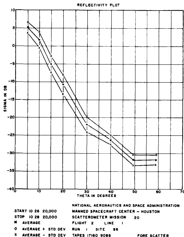
Figure 17 Example of a Scatterometer Reflectivity Plot
