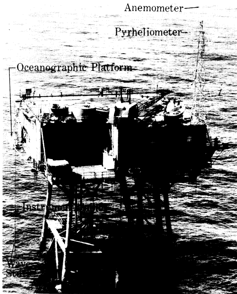
Figure 3 ARGUS ISLAND Tower
