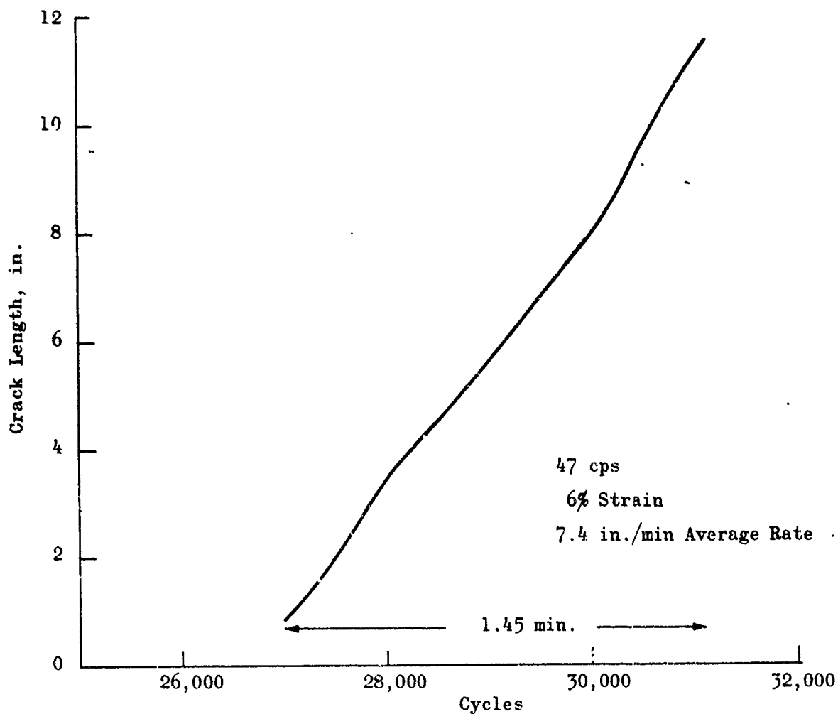
Figure 65. Biaxial Fatigue Test 92
