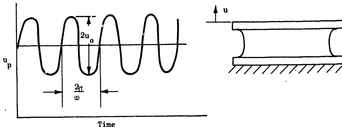
Figure 26. Vibratory Tensile Displacement Input for which a Viscoelastic Fracture Formula is Available
