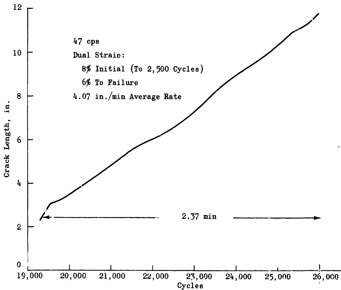
Figure 77. Biaxial Fatigue Test 105
