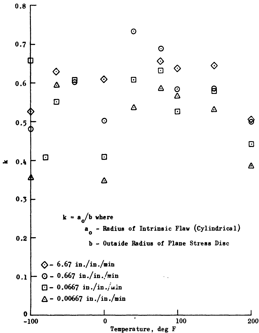
Figure 16. The Values Calculated for k Using Propellant Failure Data Furnished by Lockheed. (The biaxial strip tests were run with the cross-head set to move at a constant rate.)
