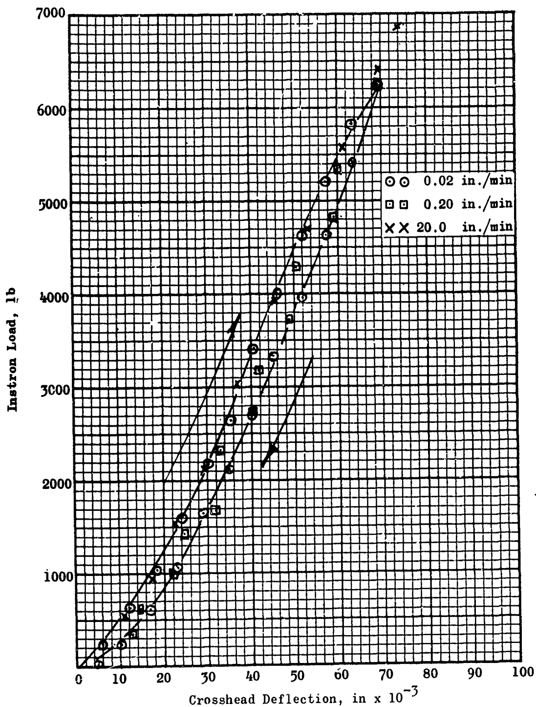
Figure 50. Compliance Curve (Load vs Deflection) for Poker Chip Apparatus with 10K Instron Load Cell
