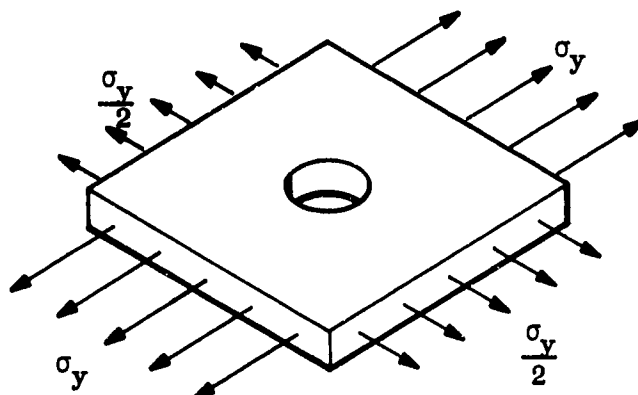
b. Model Appropriate for Biaxial Strip (2:1 Stress Ratio)
