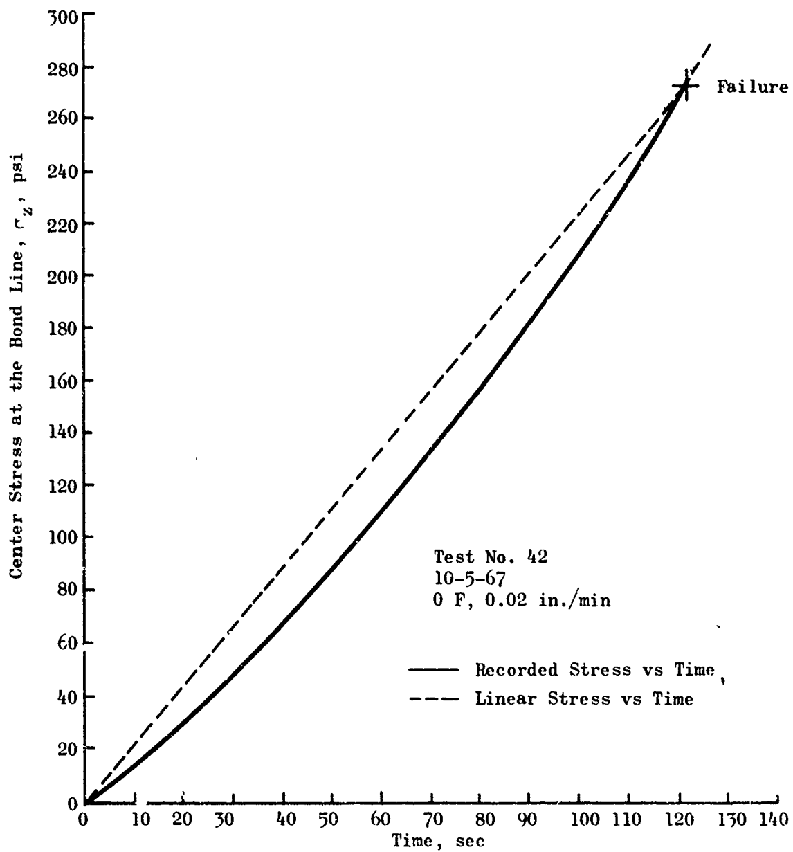
Figure 8. Typical Stress-vs-Time Relationship for Poker Chip Test
