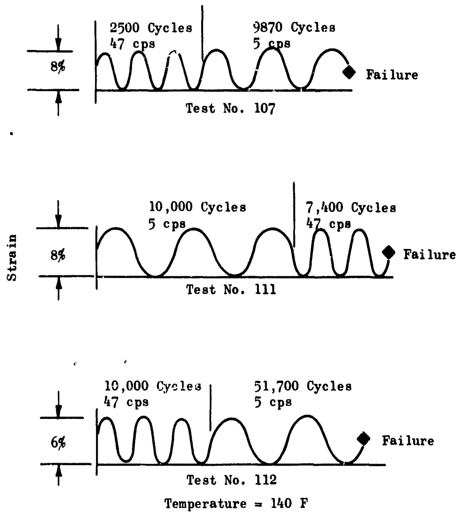
Figure 37. Summary of the Dual Frequency, Constant Amplitude Vibration Fatigue Tests (Biaxial Strip Specimens)
