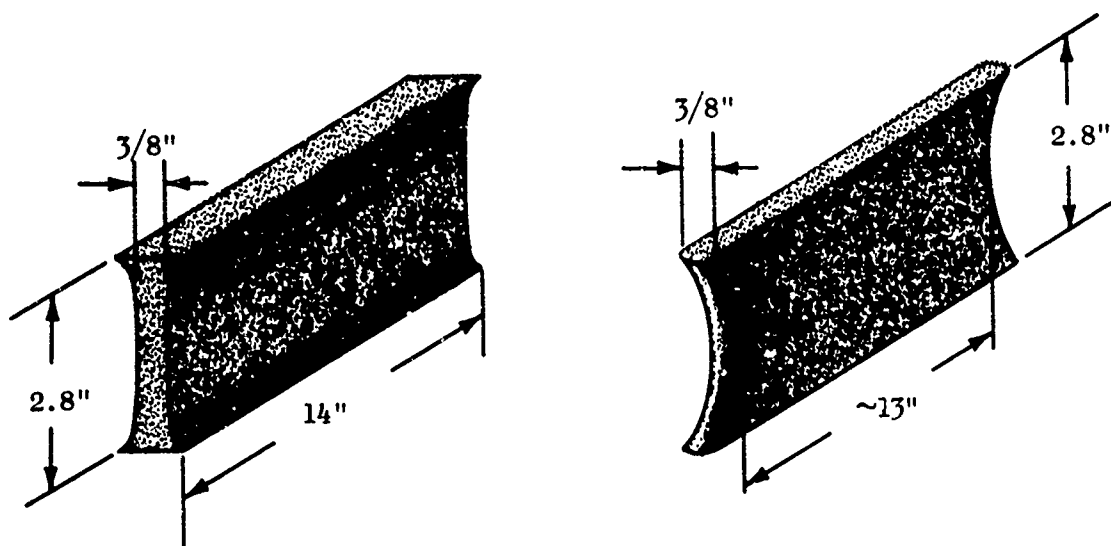
Figure 23. Original Biaxial Strip Specimen Design and the Revised Design Actually Used
