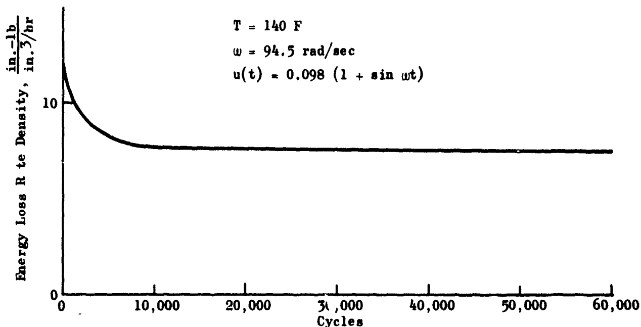
Figure 29. Deterioration in Energy Loss Measured During a Biaxial Strip Vibration Test
