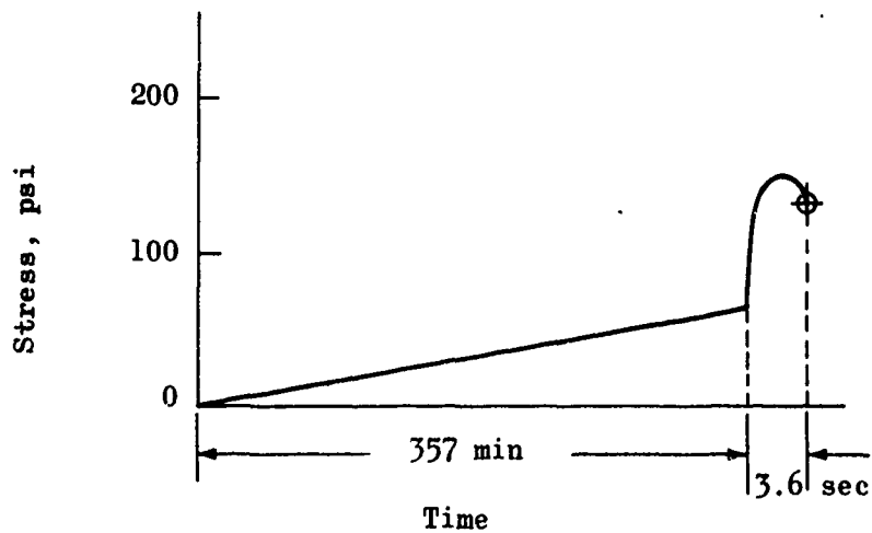
Figure 20. Stress and Strain Histories of the Two Bilinear Strain Rate Tests (biaxial strip specimen)
