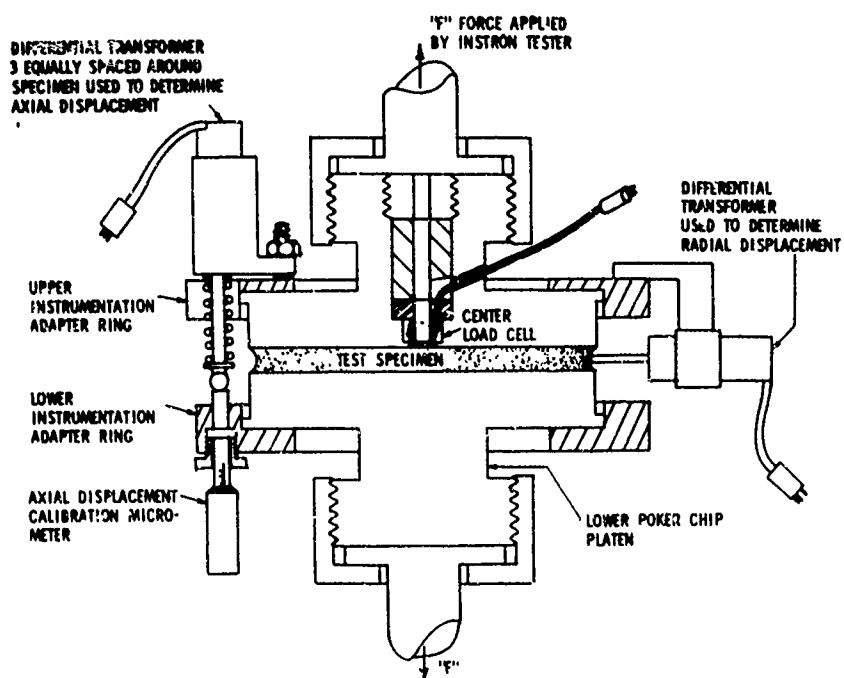
Figure 5. Poker Chip Assembly Installed In Instrumentation Rings Ready for Testing
