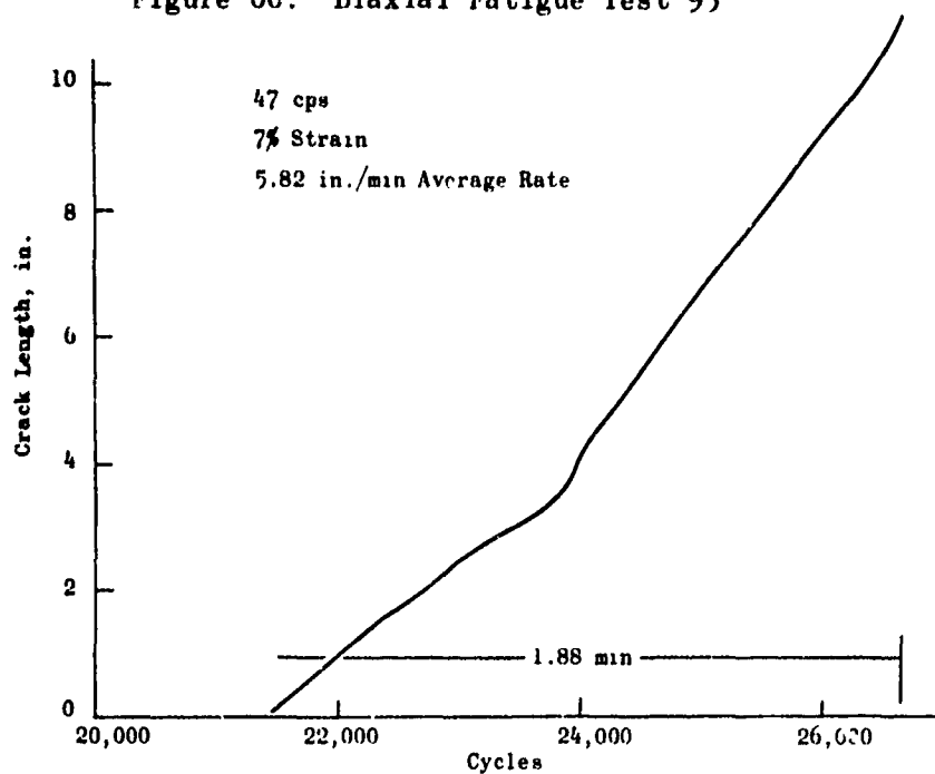
Figure 67. Biaxial Fatigue Test 94
