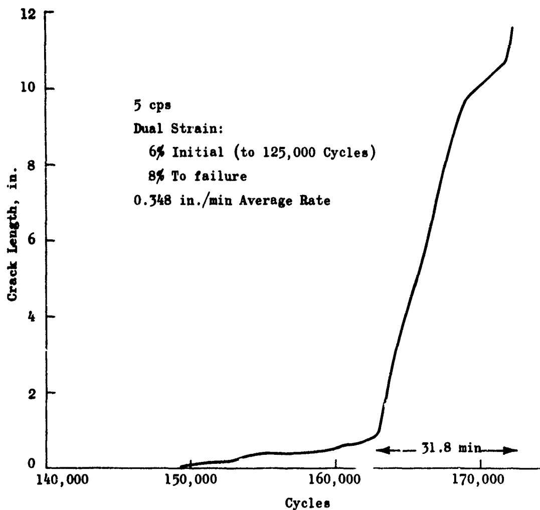
Figure 72. Biaxial Fatigue Test 100
