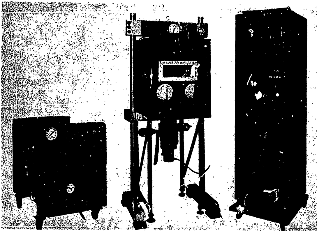
Figure 25. Cumulative Damage Tester
