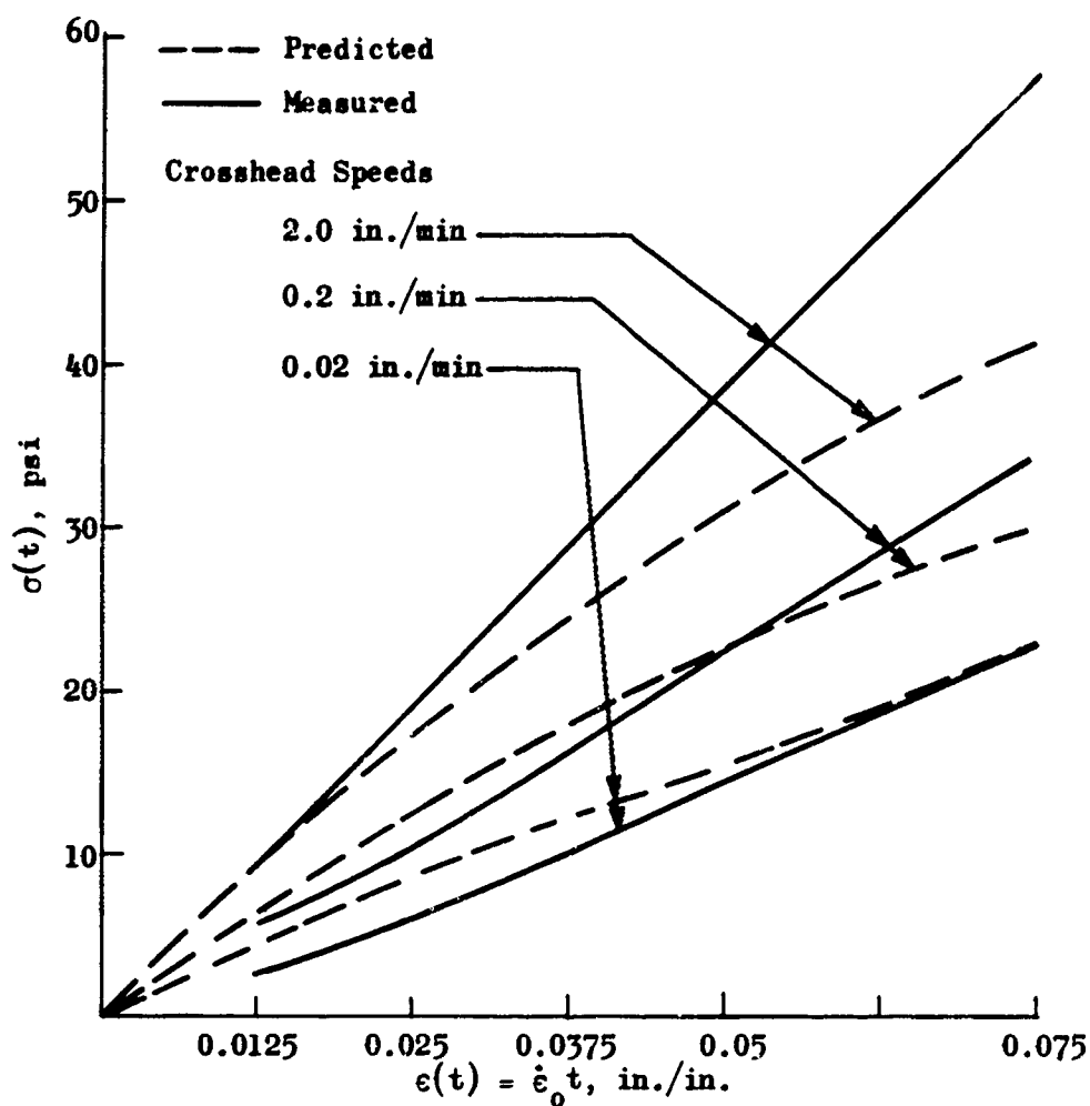
Figure 90. Comparisons of the Stresses, Predicted and Measured, Resulting from Uniaxial Constant Strain Rate Tests-- (Predictions Based on Uniaxial Relaxation Data)
