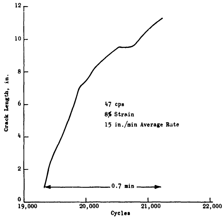
Figure 68. Biaxial Fatigue Test 95
