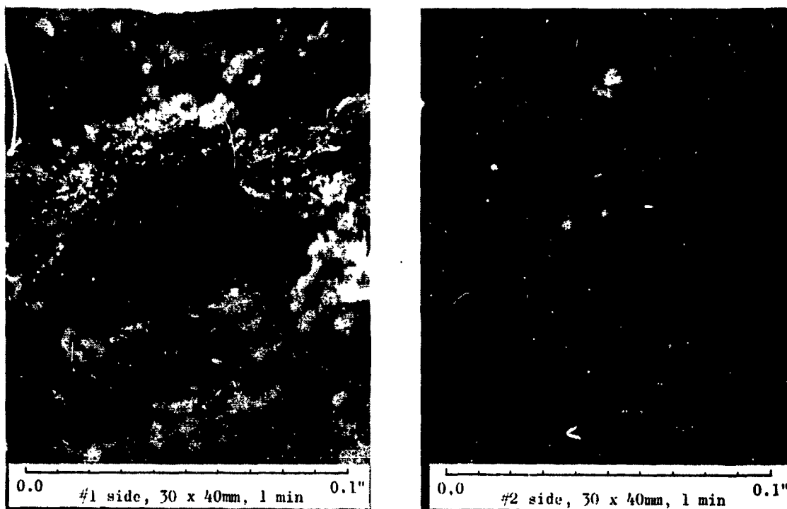
Figure 31. Photomicrographs of a Small Void From Which One Biaxial Test Specimen Failed
