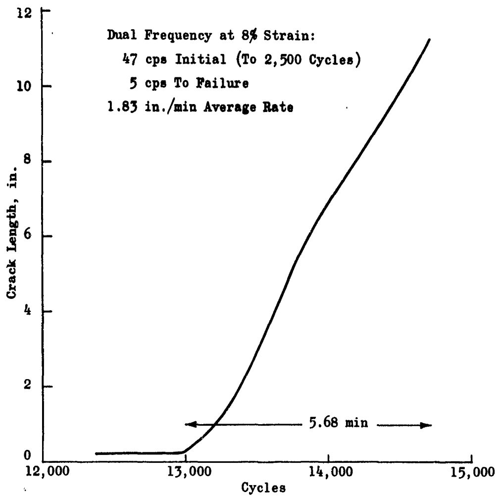
Figure 79. Biaxial Fatigue Test 107
