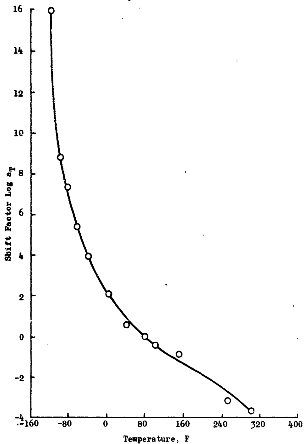
Figure 86. Time-Temperature Shift Factors Corresponding to the Uniaxial Relaxation Data of Fig. 85
