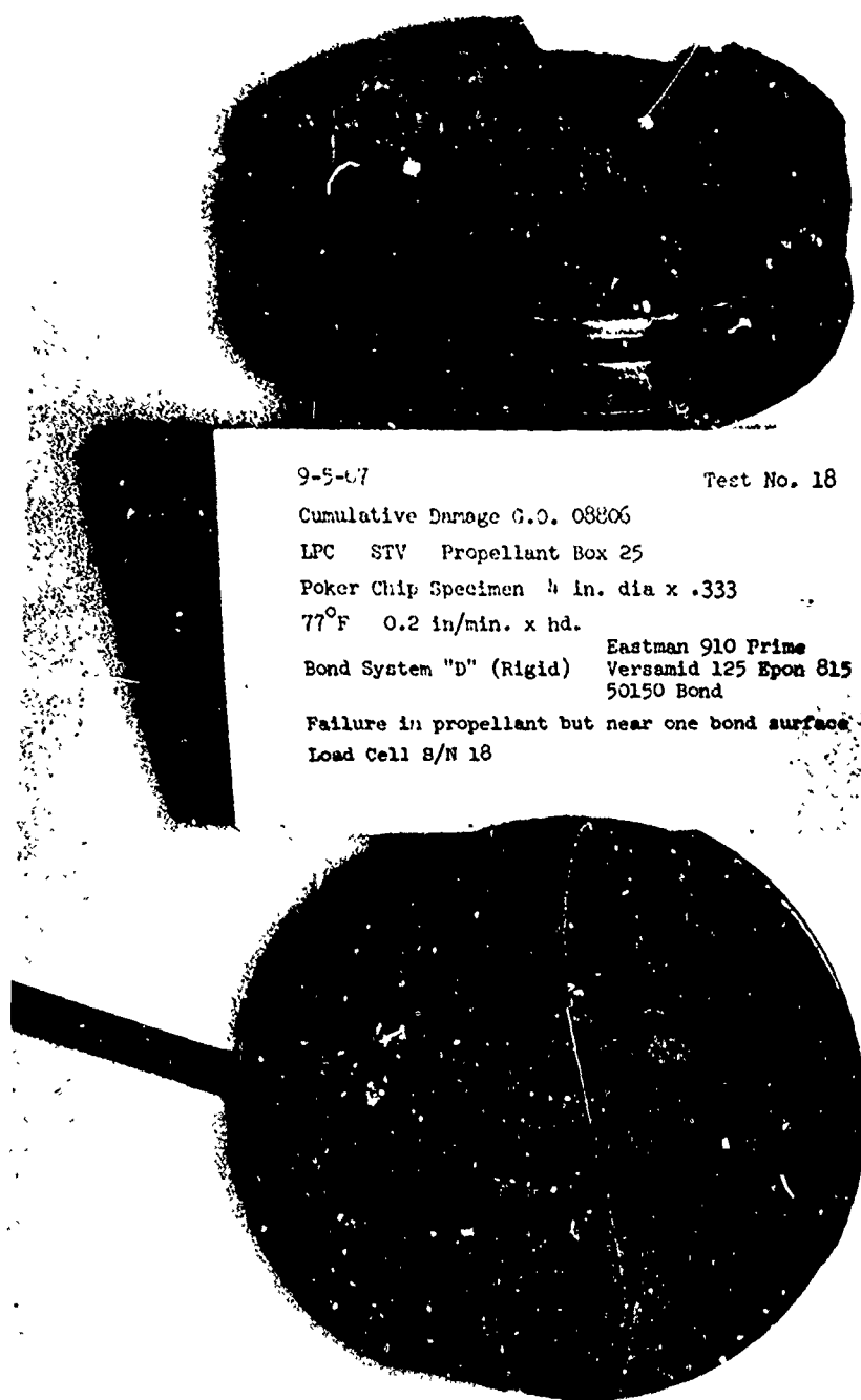
Figure 7. Typical Surface Following Complete Separation of Platens
