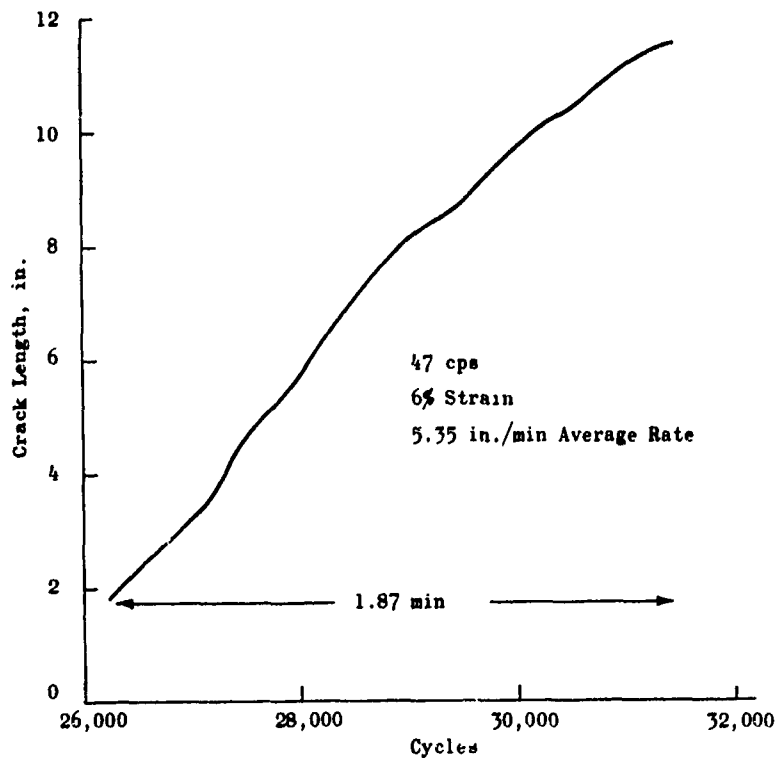
Figure 69. Biaxial Fatigue Test 96
