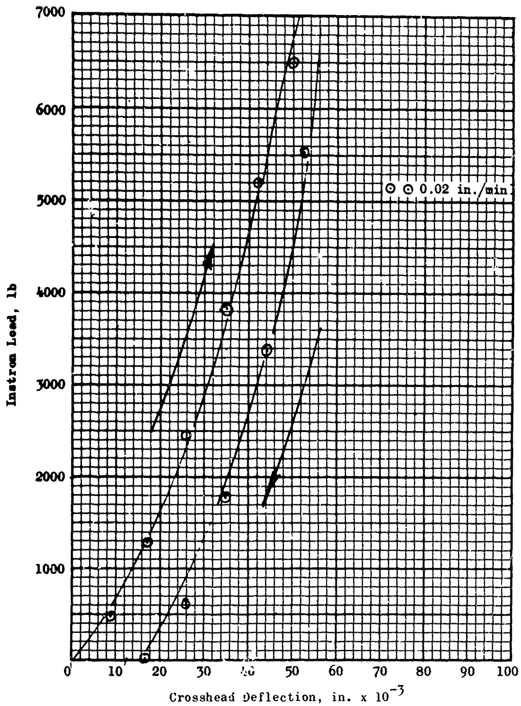
Figure 51. Compliance Curve (Load vs Deflection) for Instron Model TTD S/N 1572 with 10K Load Cell
