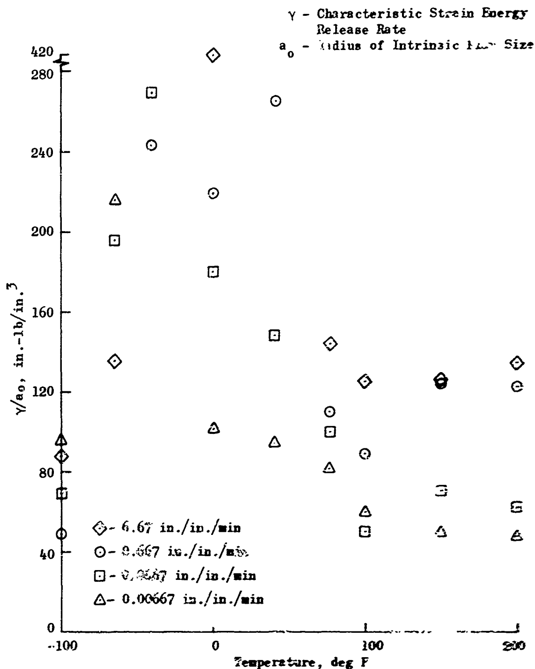
Figure 17. The Values Calculated for \gamma/a_0 Using Propellant Failure Data Furnished By Lockheed. (The biaxial strip tests were run with the crosshead set to move at a constant rate.)
