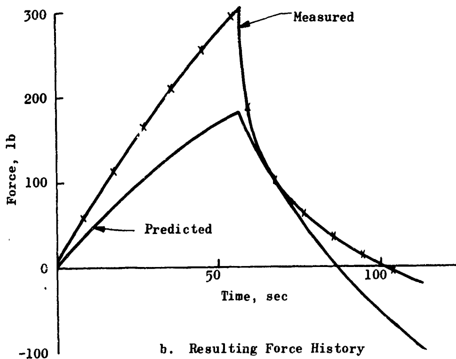
Figure 89. Comparisons of the Biaxial Force-Time Curves, Measured and Predicted, Resulting from the Sawtooth Displacement-Time History
