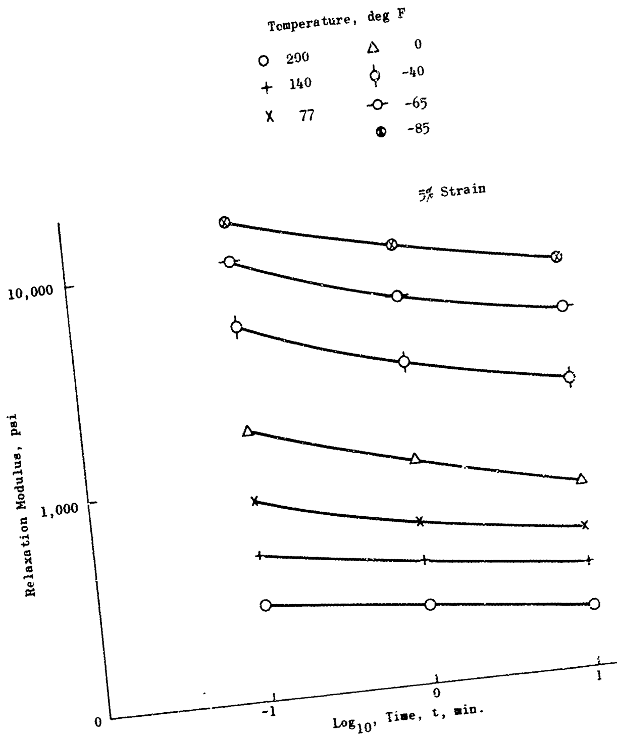
Figure 91. Raw Biaxial Relaxation Data as Furnished by LPC
