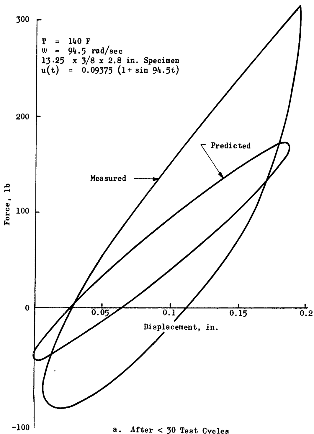
Figure 88. A Comparison of the Biaxial Force-Displacement Curves as Measured and Predicted
