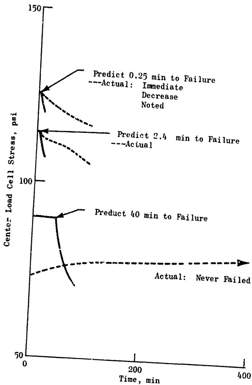
Figure 14. Theory-vs-Test Results for Constant Load Poker Chip Tests (Predictions based on \gamma/a_0 = 51.1 \text{ in.-lb/in.}^3 deduced from constant stress rate tests at 77 F)
