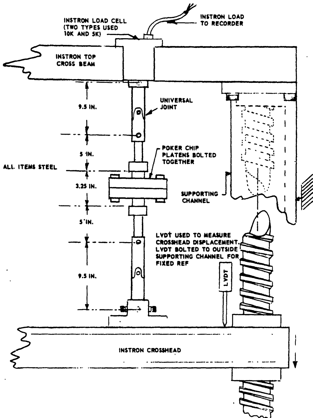
Figure 48. Arrangement of Poker Chip Apparatus on Instron Model TTD Tester in Determining Compliance for Hardware Alone
