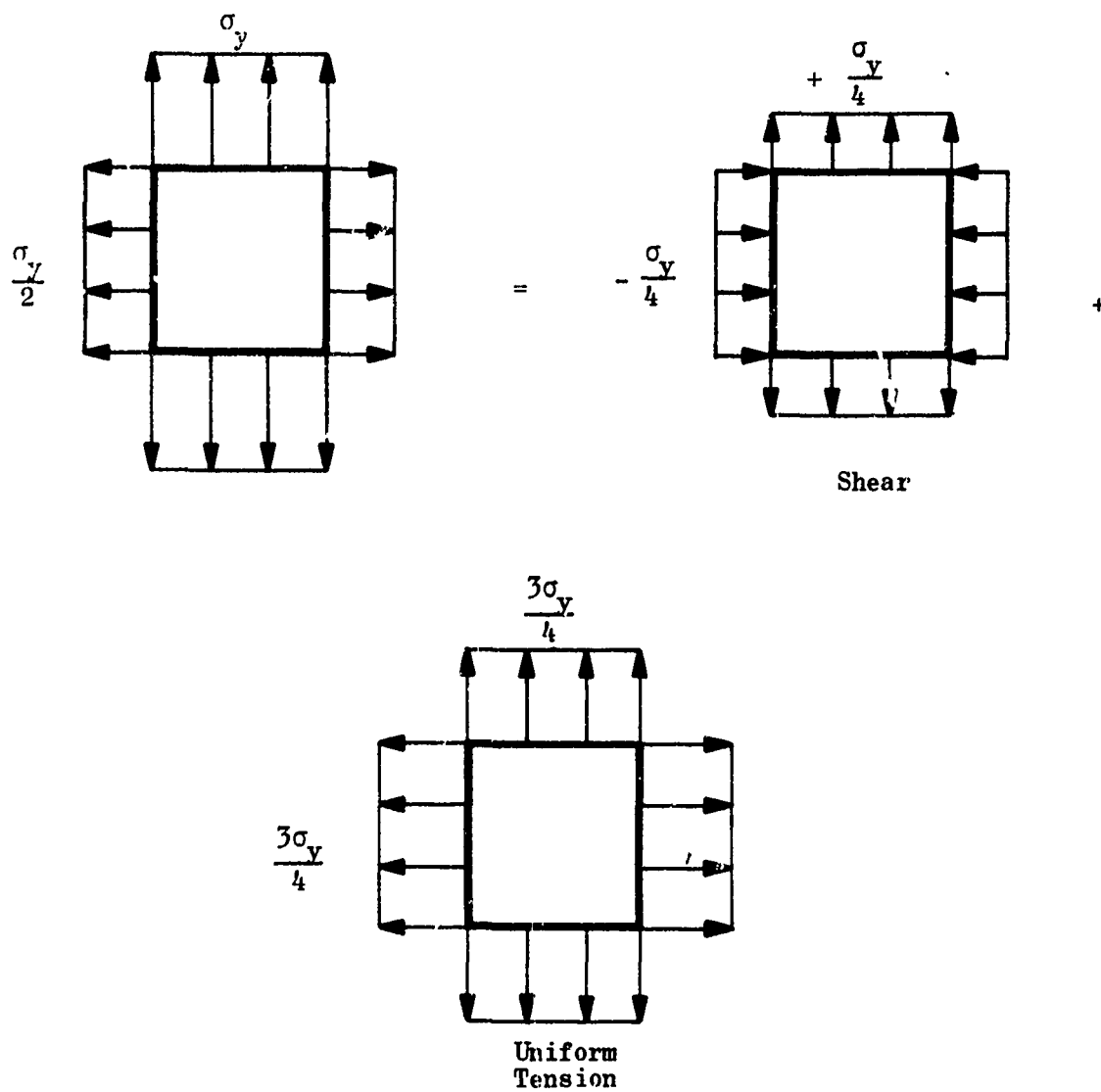
Figure 19. The Stresses of the Biaxial Strip Can Be Separated into a Uniform Tension Portion and a Pure Shear Portion. (Note the value of the uniform tensile stress is \frac{3\sigma_y}{4} ).
