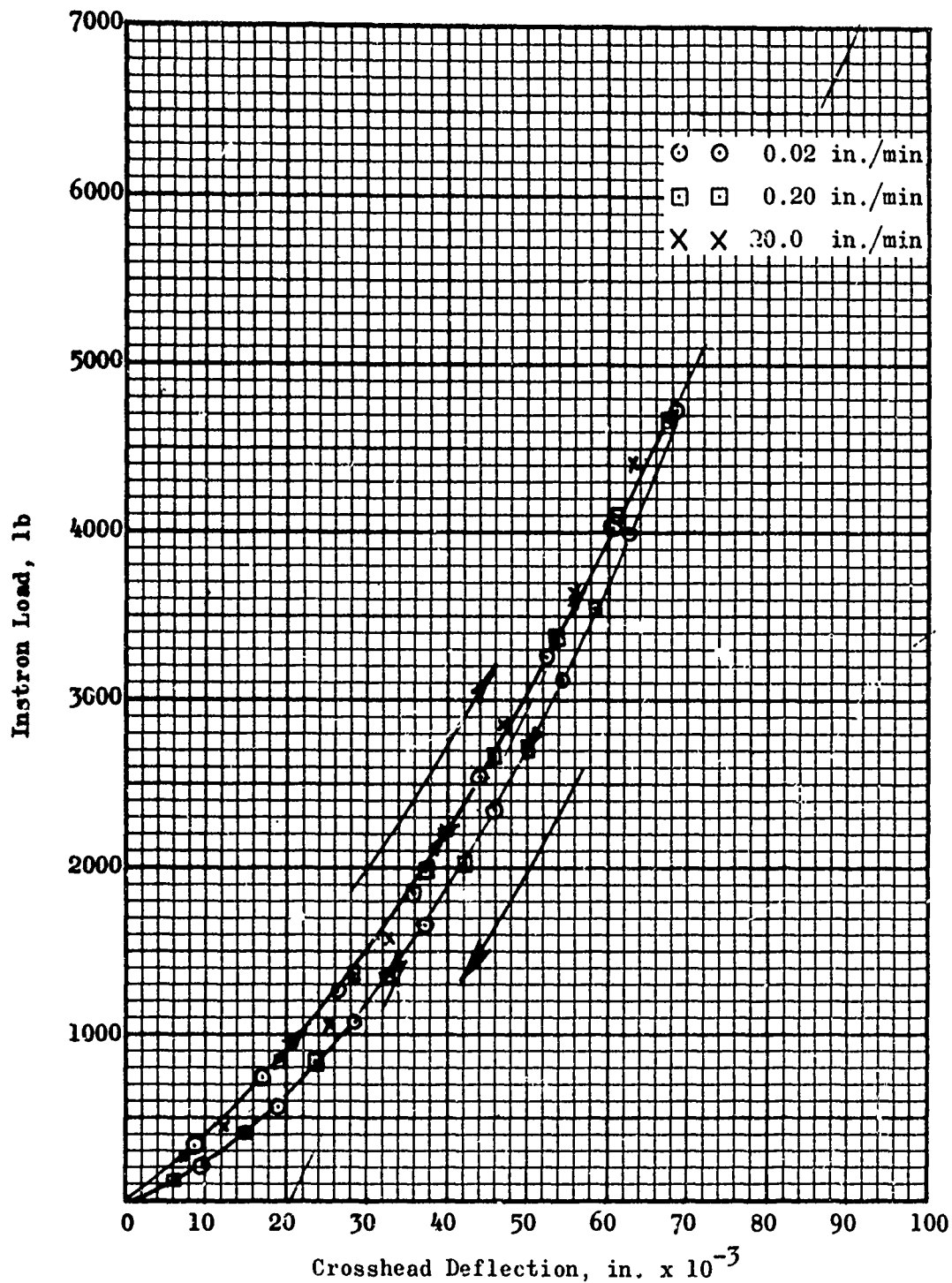
Figure 49. Compliance Curve (Load vs Deflection) for Poker Chip Apparatus with 5K Instron Load Cell
