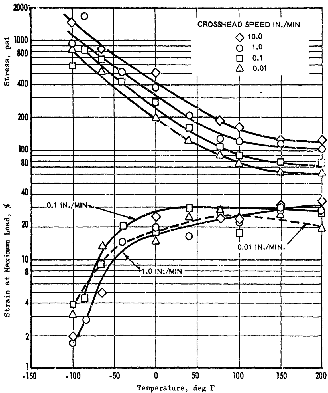
Figure 15. Strip Biaxial Failure Stress and Strain vs Temperature-0064-61E Control Propellant
