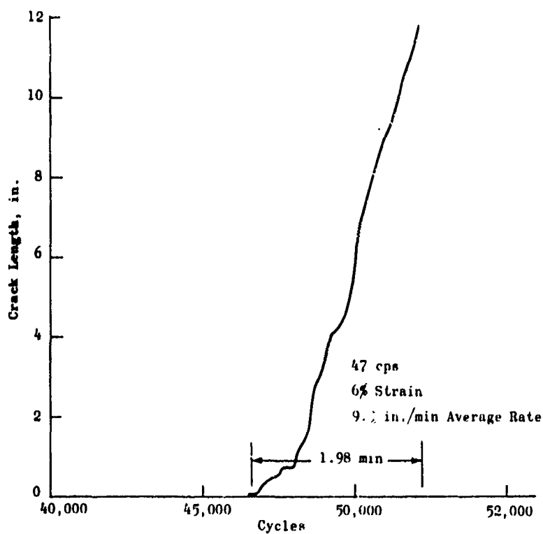
Figure 66. Biaxial Fatigue Test 93
