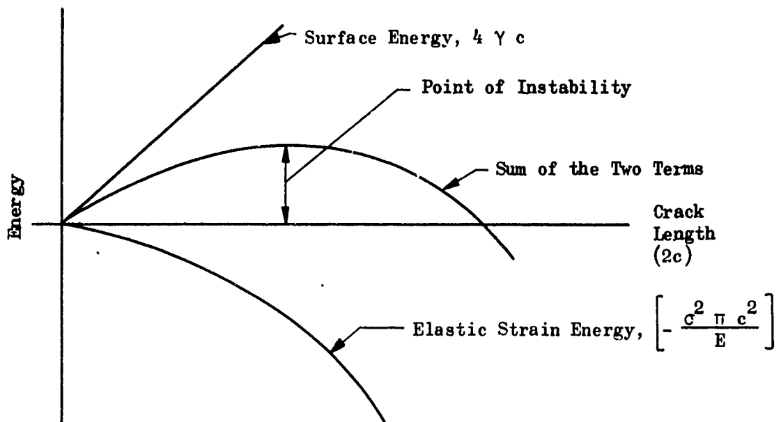
Figure 2. Energy Criterion For a Plate With a Crack of Length 2c
