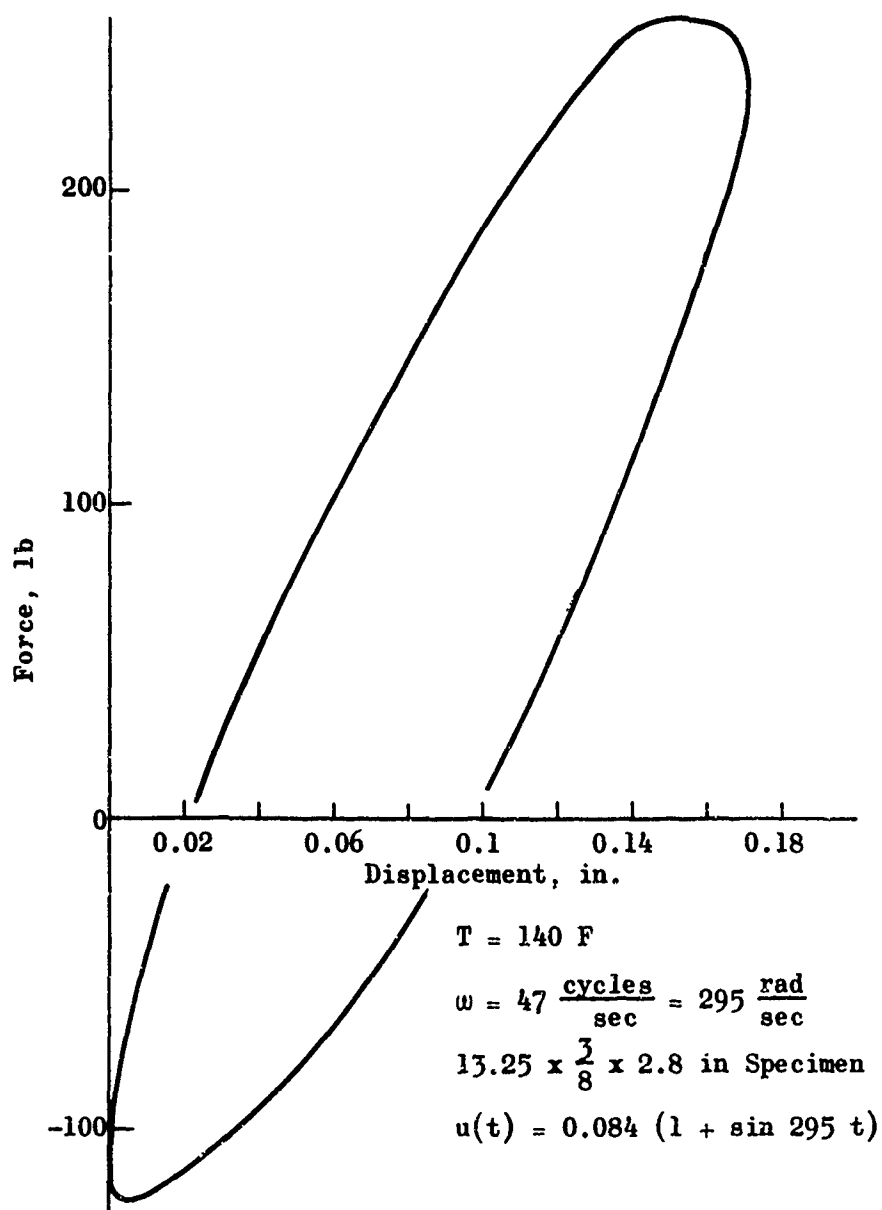
Figure 28. Force-Displacement Trace Taken During a Vibration Fatigue Test on a Biaxial Strip (The area within the ellipse represents total heat loss per cycle)
