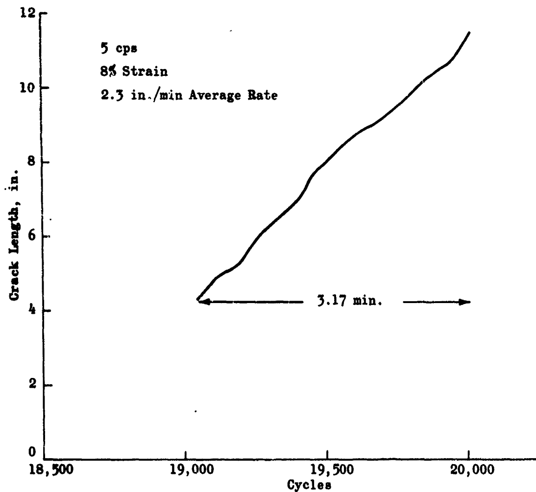
Figure 80. Biaxial Fatigue Test 103
