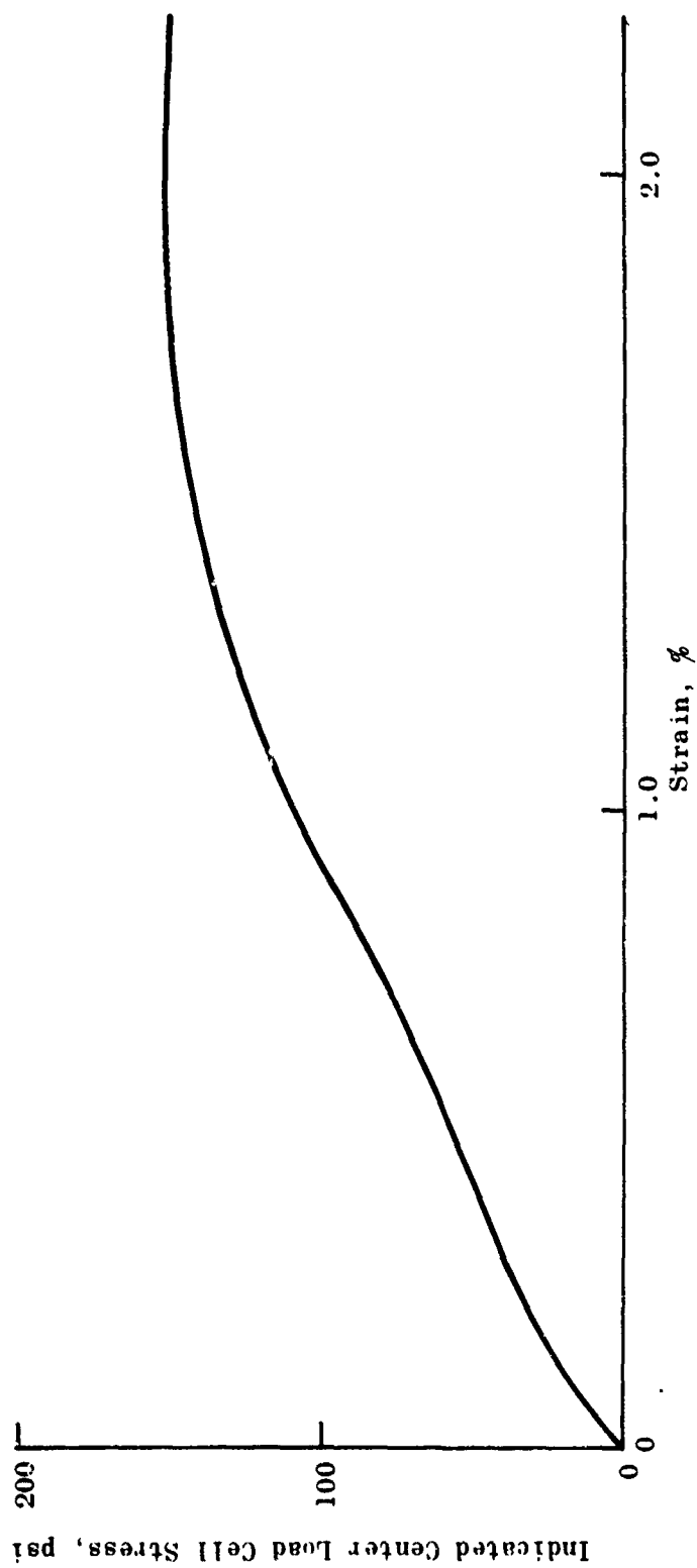
Figure 38. Stress-Strain Curve from Triaxial Test Following Constant Load Test (736 Pounds)
