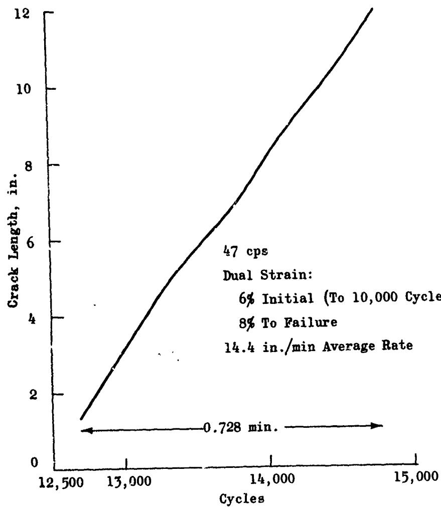
Figure 78. Biaxial Fatigue Test 106
