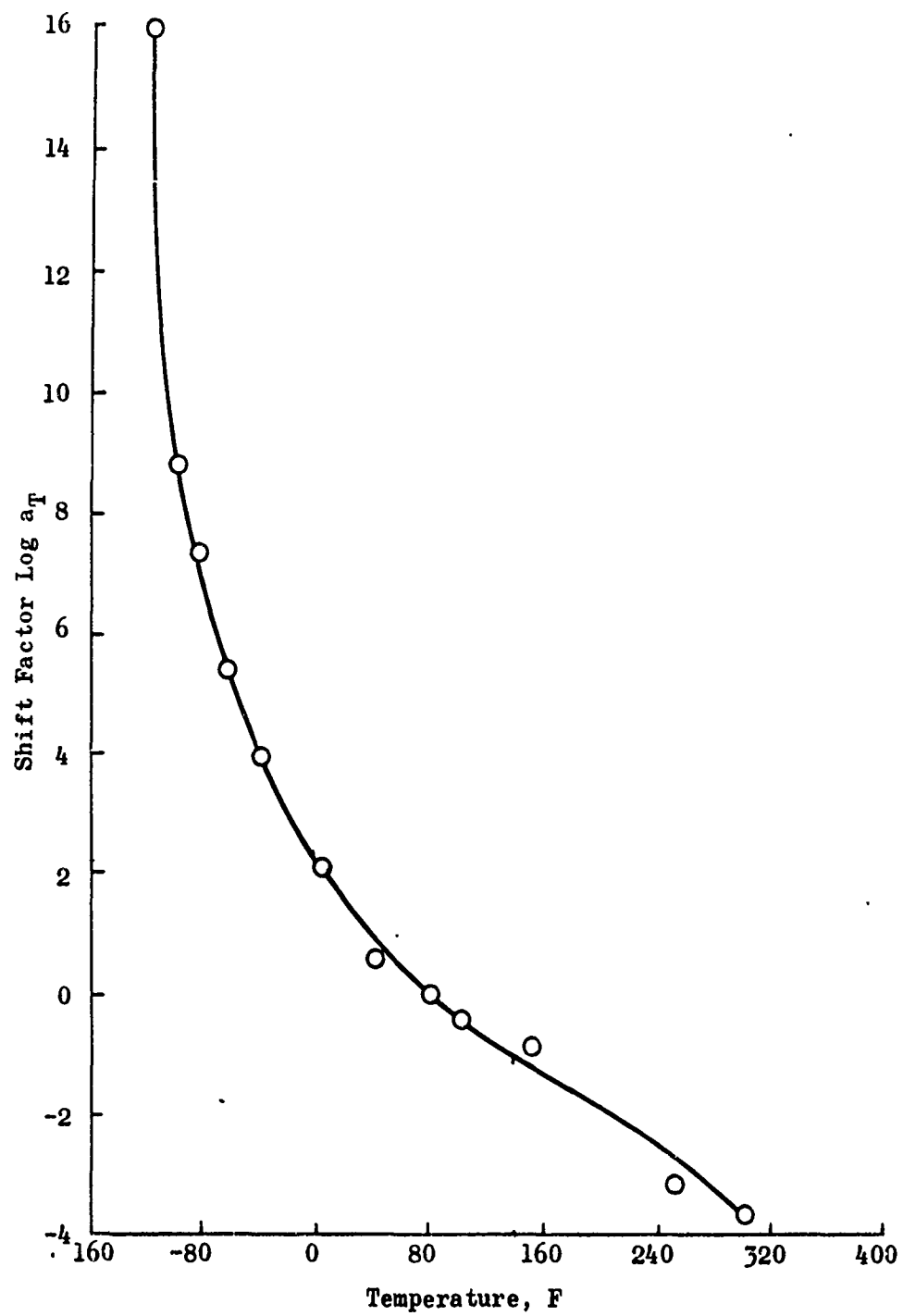
Figure 56. Uniaxial Shift Factors for Lockheed STV Propellant
