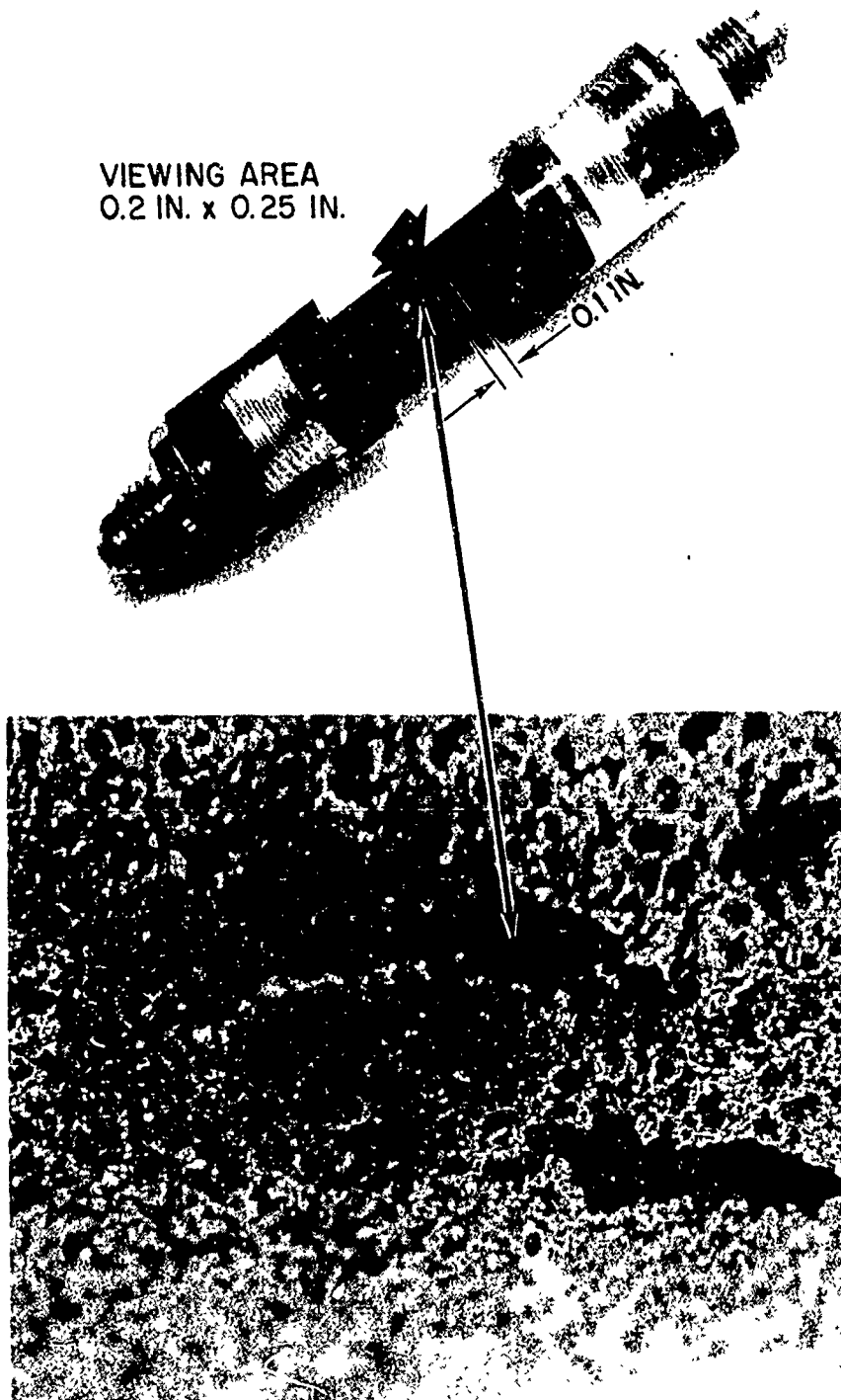
Figure 43. Machined Surface Crack Location, Low Stress Rate, Cylinder 005
