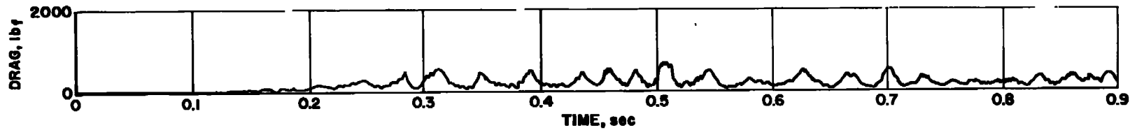
b. Supersonic X-3 Parachute, M_{\infty} = 4.0 Fig. 8 Parachute Deployment Characteristics
