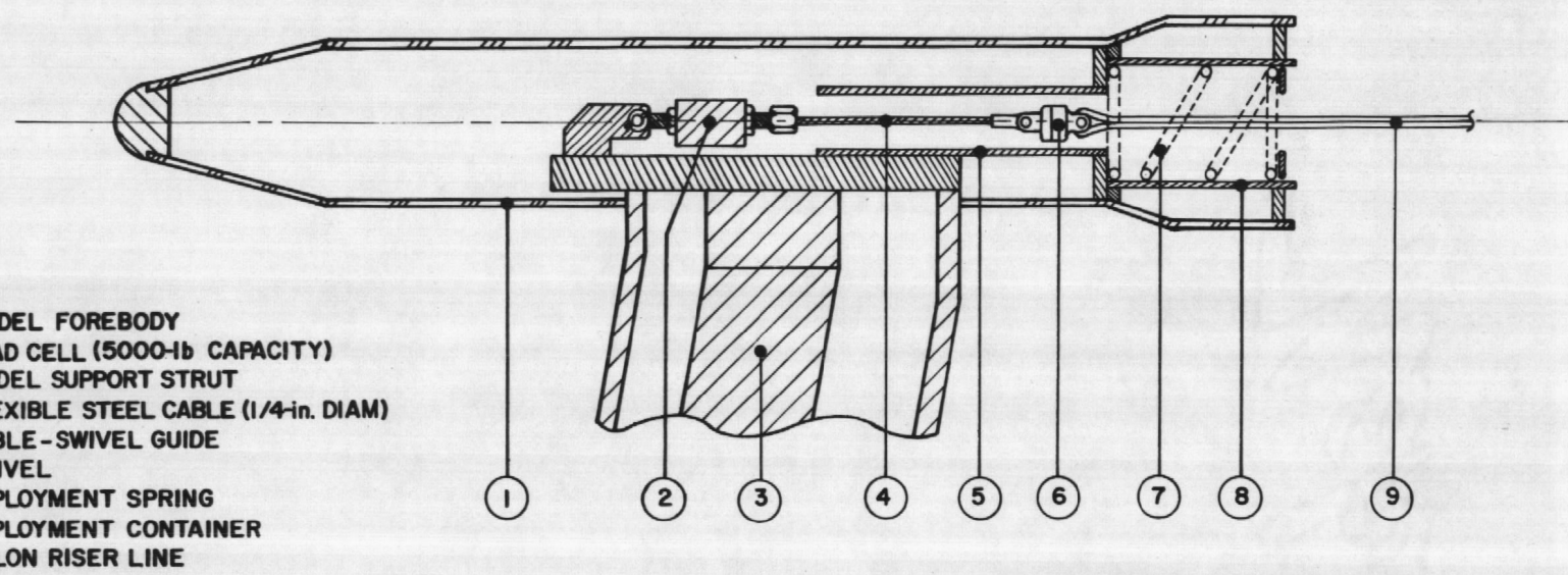
Fig. 4 Sketch of Model Forebody Showing Load Cell Installation
