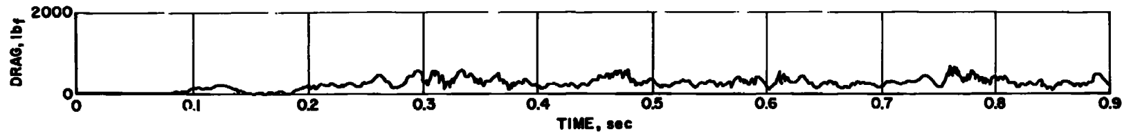
d. Backup Supersonic X-4 Parachute, M_{\infty} = 2.1
