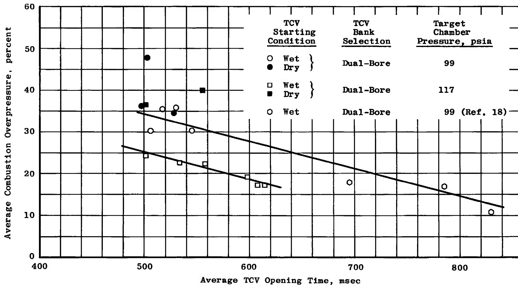
Fig. 16 Average Combustion Overpressure as a Function of Average TCV Opening Time
