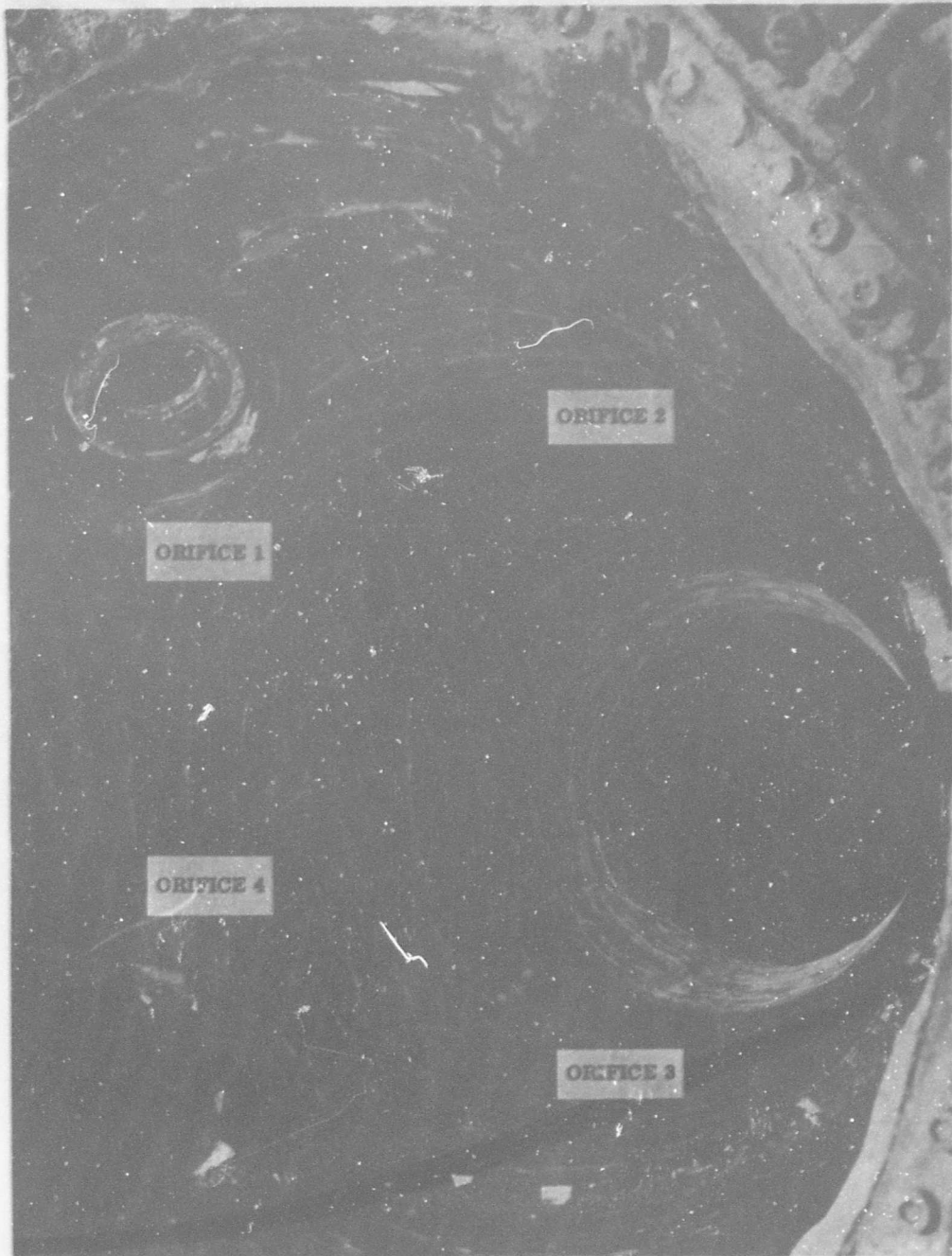
Figure 14. Nozzle-Orifice Ports Erosion at Exit Cone
