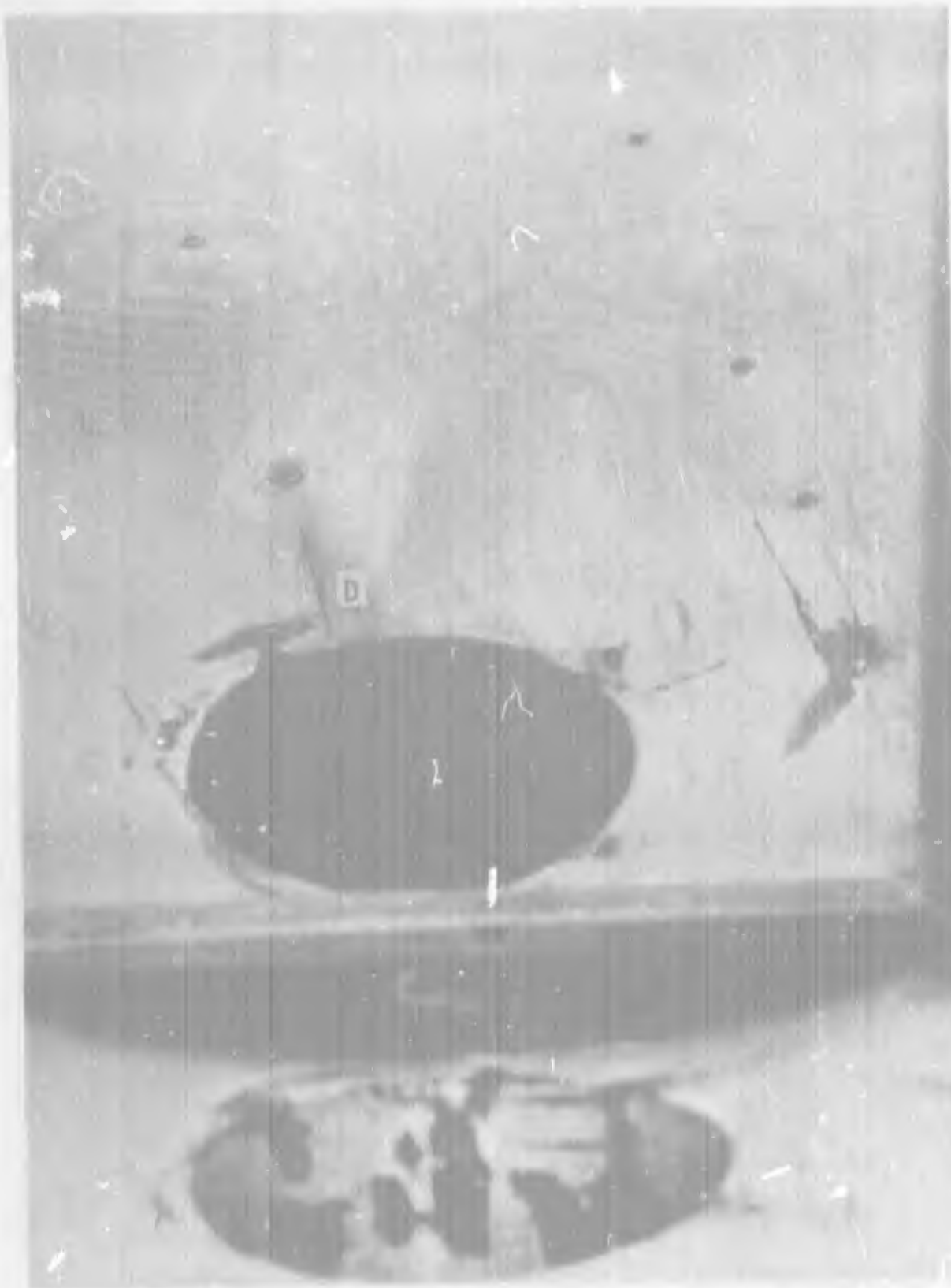
Figure 68. Orifice Smear Photo, Perpendicular to Centerline
