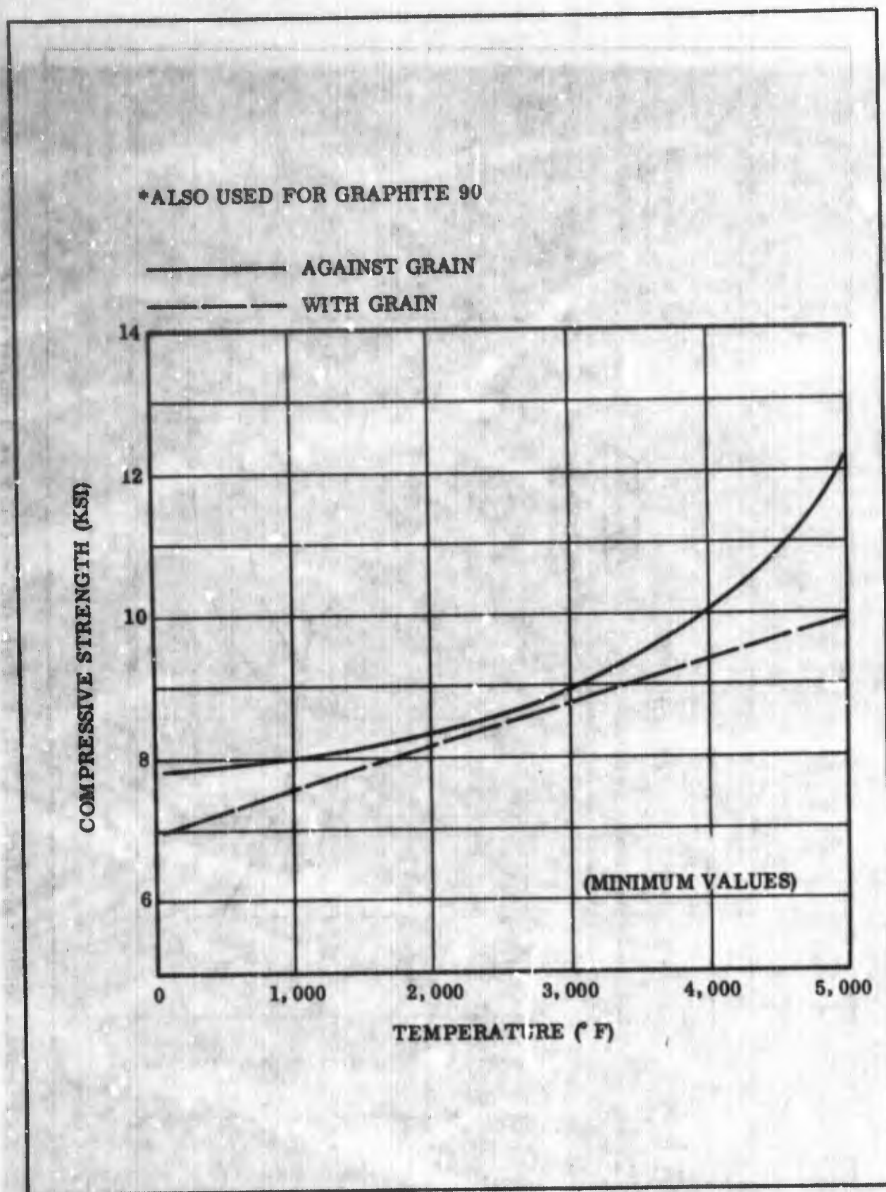
Figure 127. Graphite 30 Ultimate Compressive Strength vs Temperature
