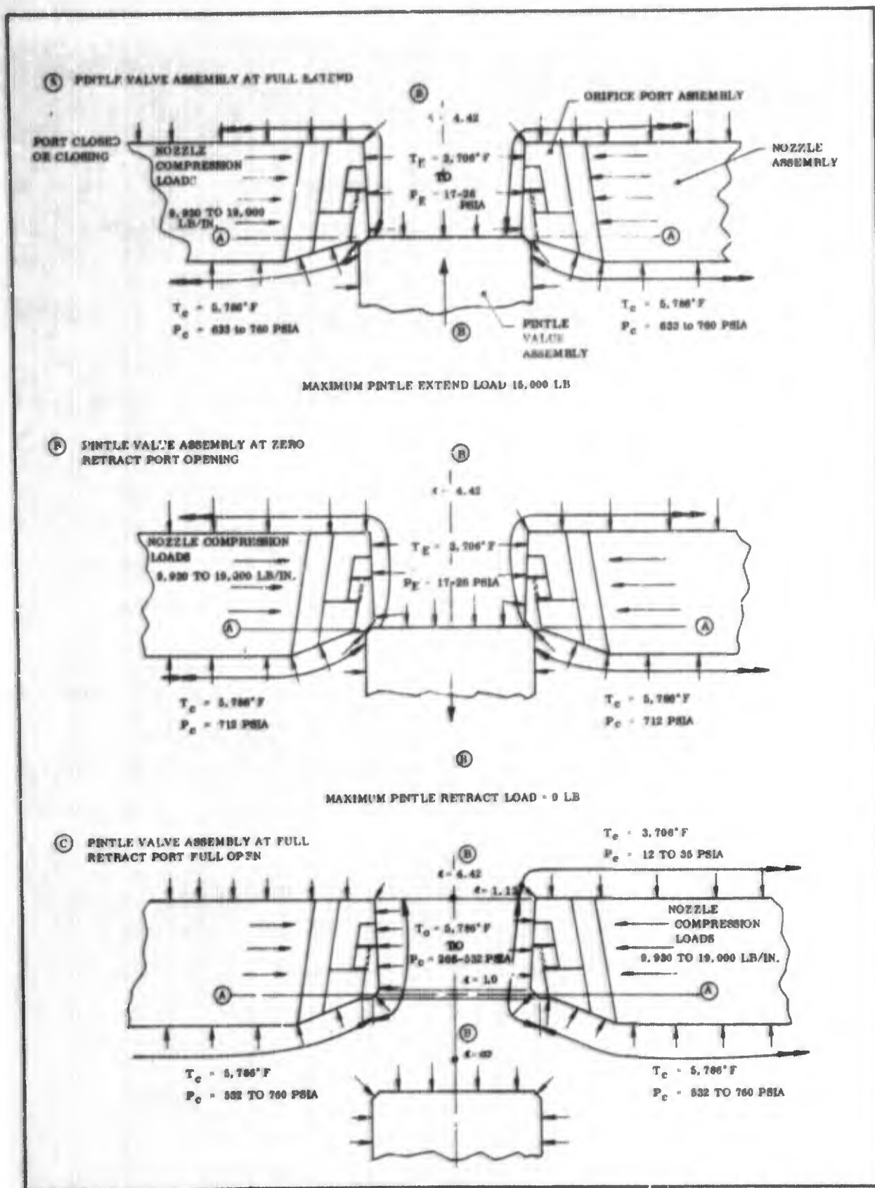
Figure 3. Orifice Port 3 Load Conditions
