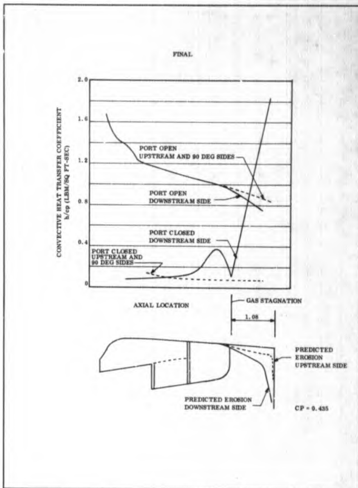
Figure 95. Orifice Wall h/c_p vs Axial Location at 25 Sec - Final
