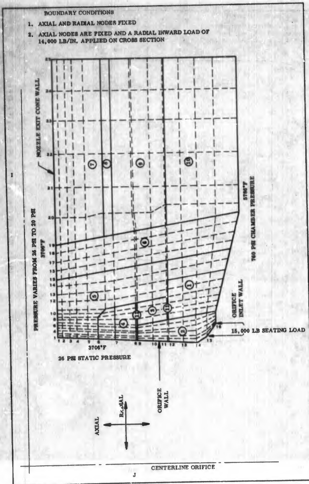
Figure 125. Orifice Port Boundary Conditions at 25.1 Sec. Valve Closed
