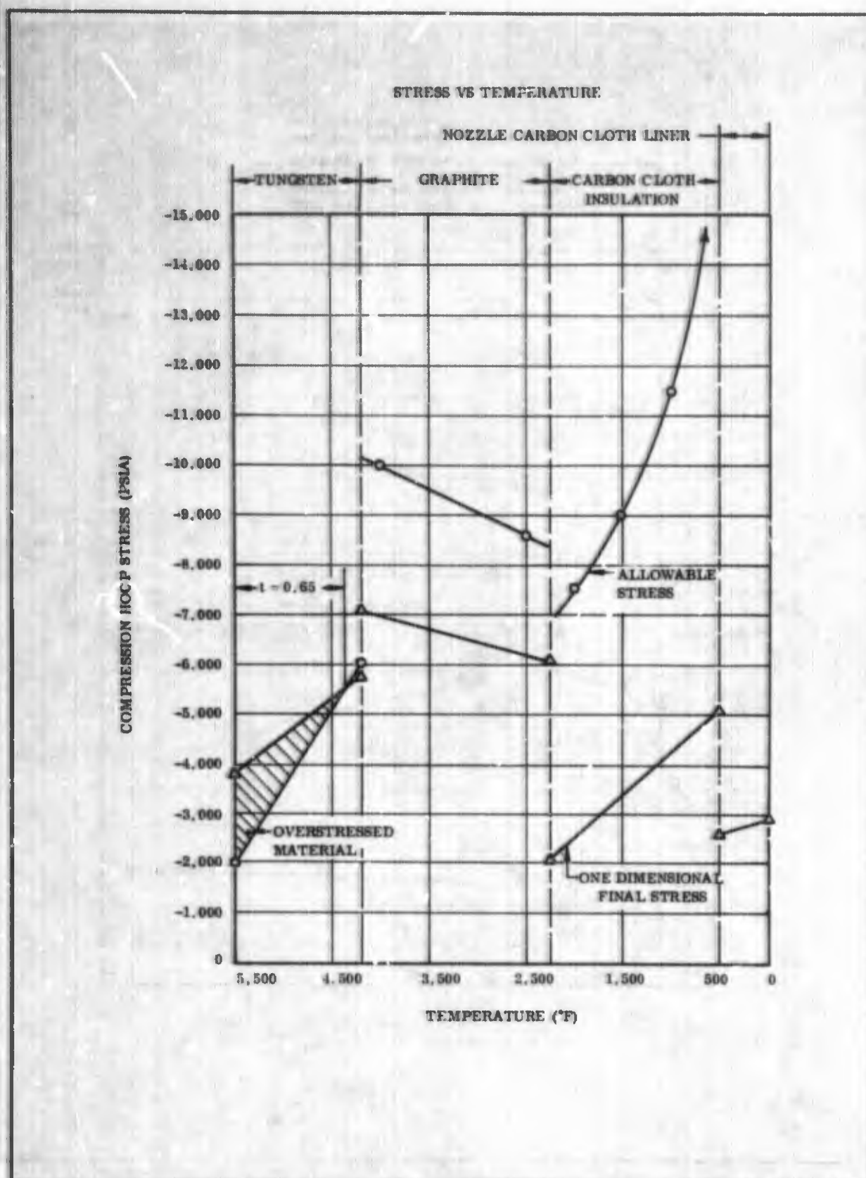
Figure 213. Present Design, Overstressed Material, Section B-B at 25.1 Sec
