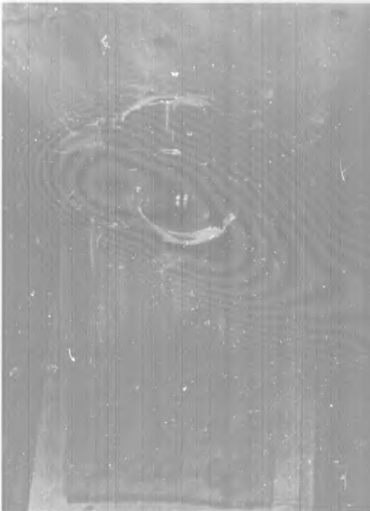
Figure 87. Orifice Smear Pattern, Perpendicular to Centerline, for PTB Missing
