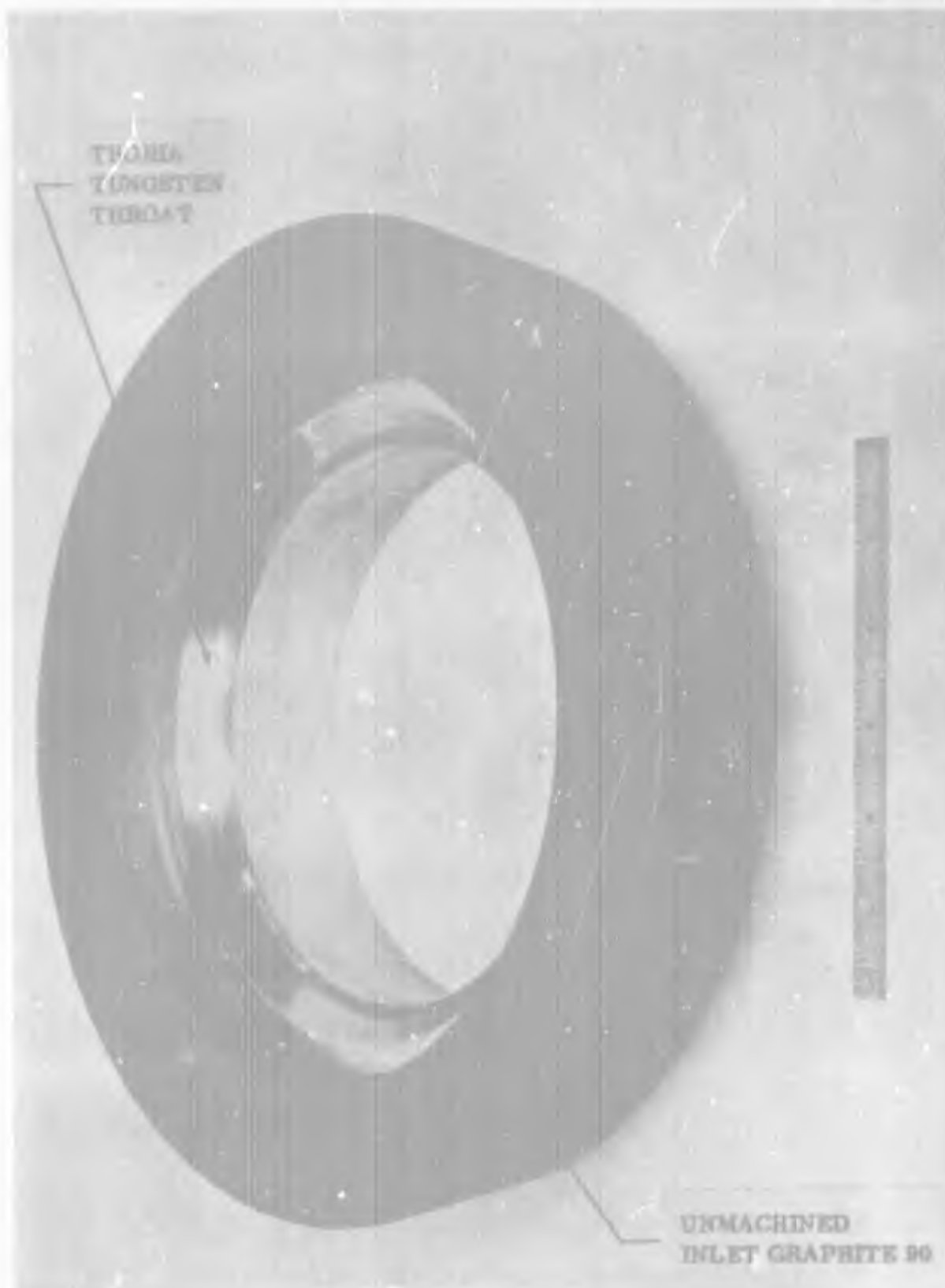
Figure 46. Orifice 3 Throat Subassembly - Aft View
