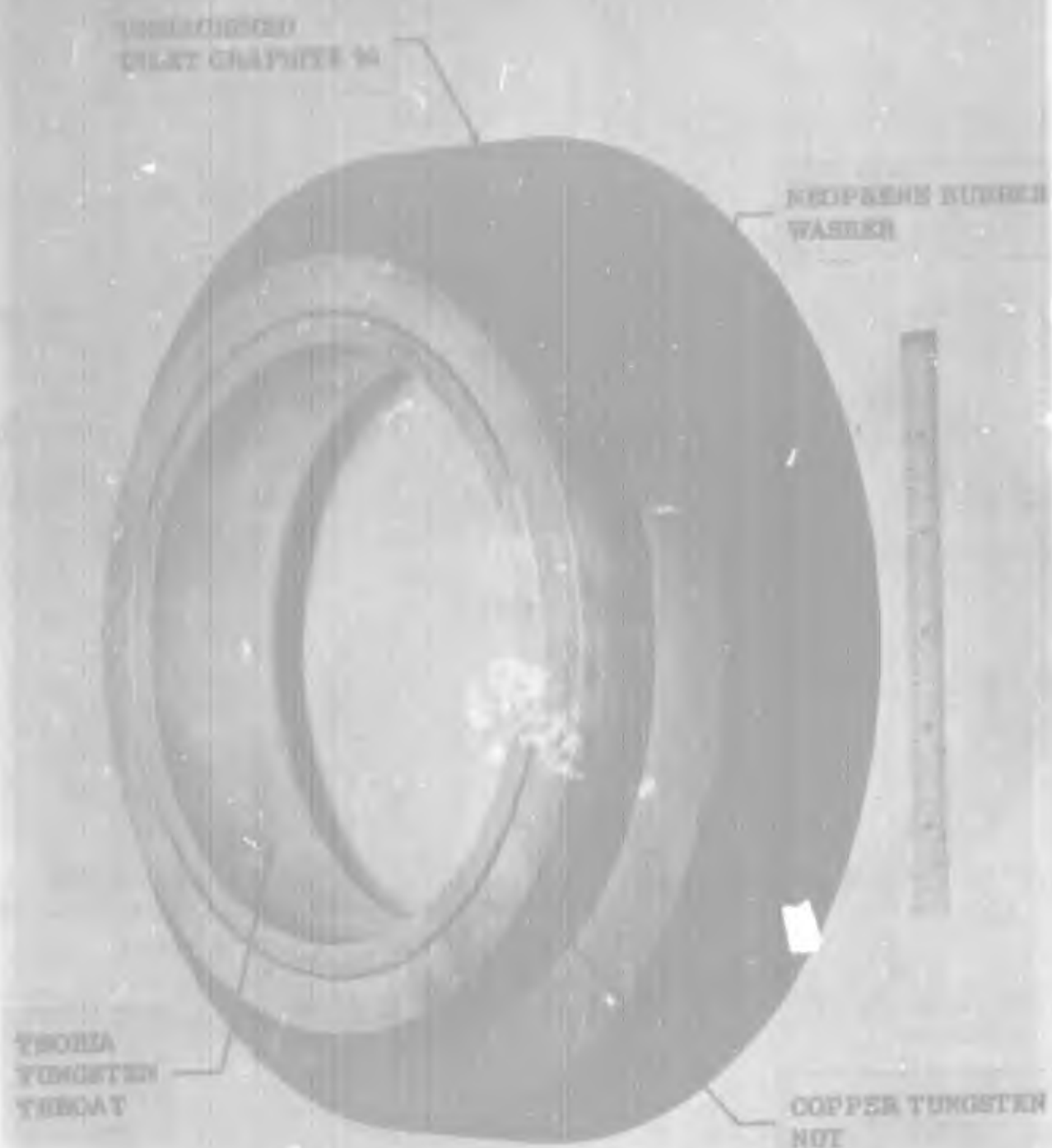
Figure 45. Orifice 3 Throat Subassembly - Forward View
