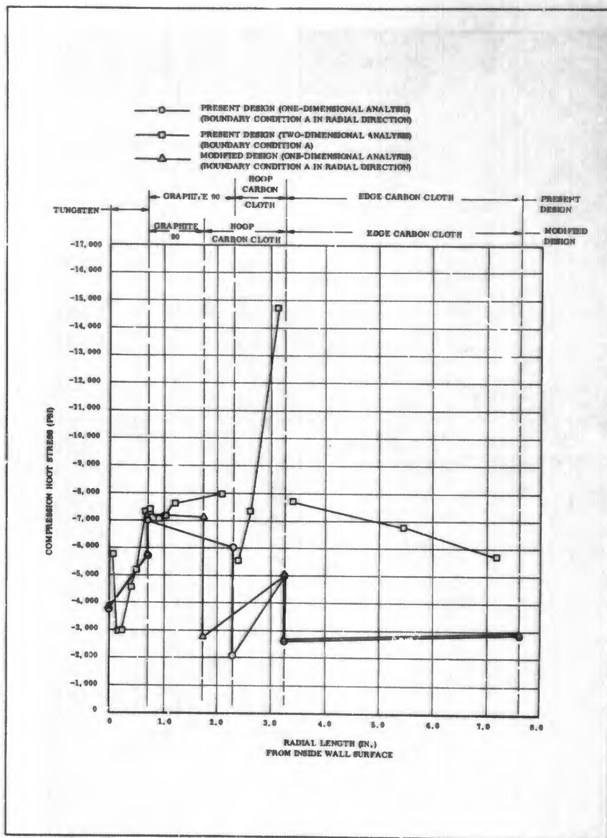
Figure 212. Present and Modified Orifice Design, Hoop Stress Profile, Section B-B at 25.1 Sec
