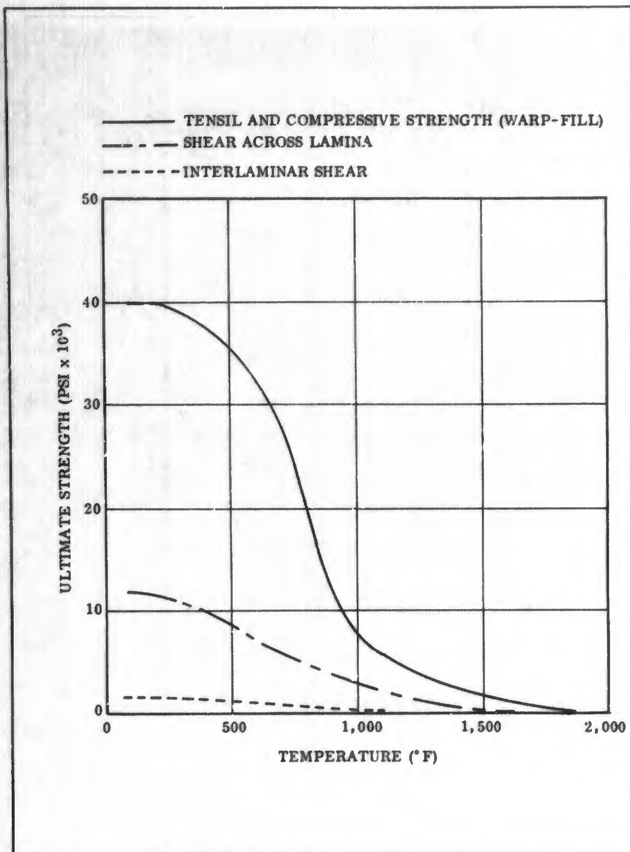
Figure 147. Glass Cloth Phenolic, Ultimate Tensile, Compressive, Shear Strength vs Temperature
