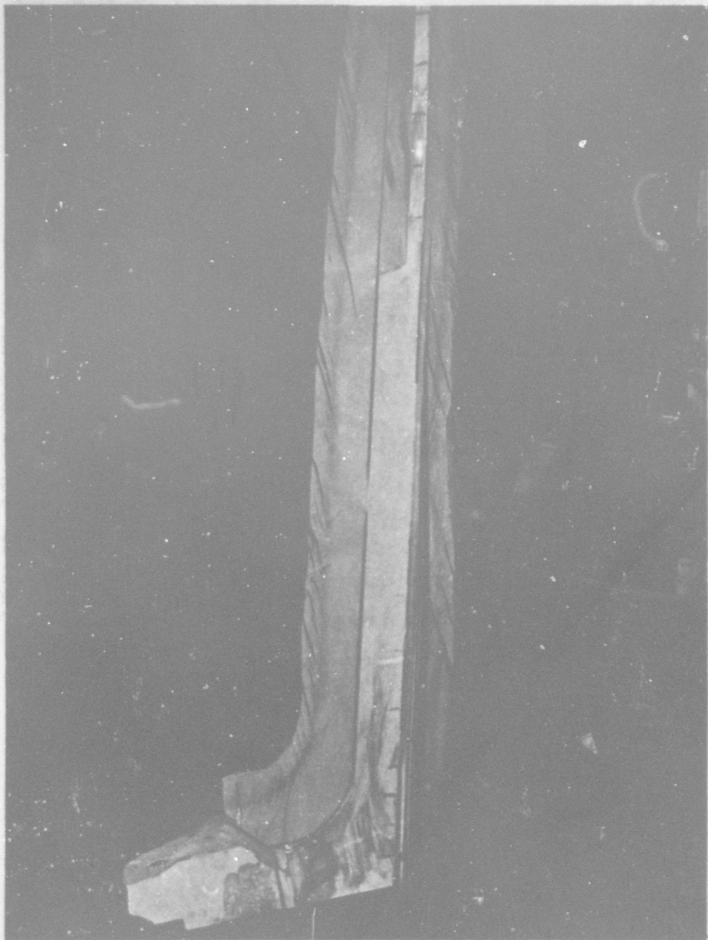
Figure 23. Submerged Nozzle Cross Section 45 Deg Away From Port 1
