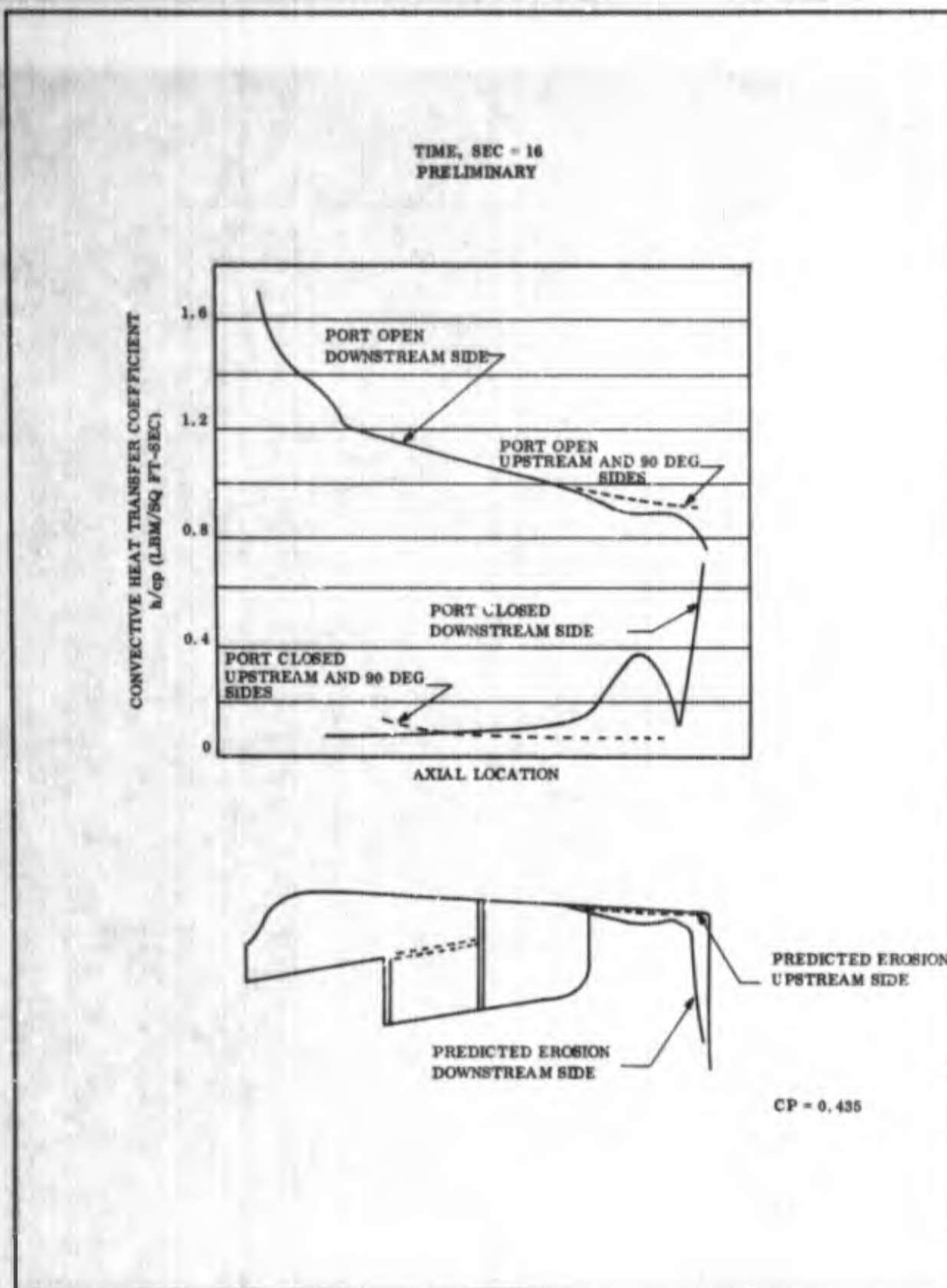
Figure 94. Orifice Wall h/c_p vs Axial Location at 16 Sec - Preliminary
