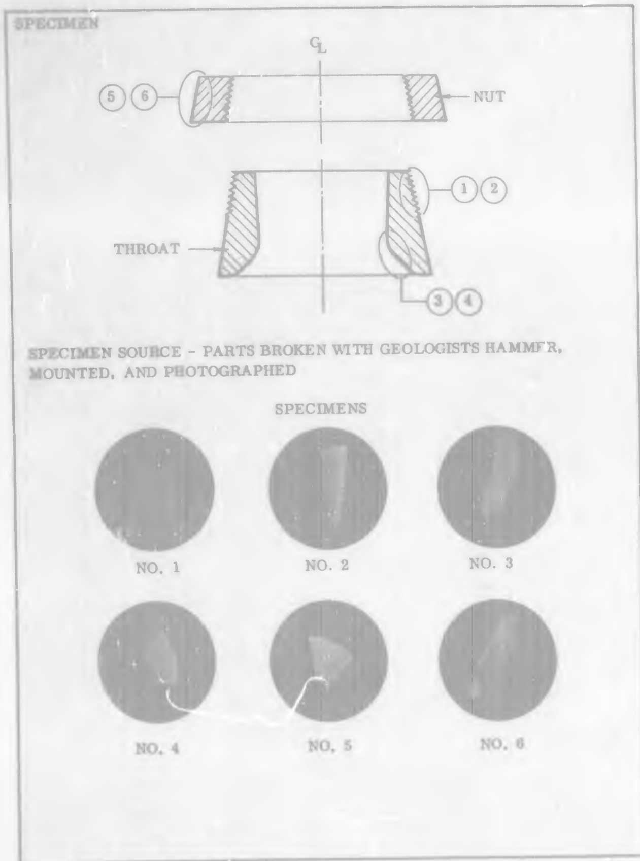
Figure 47. Orifice Tungsten Photomicrographs - Specimen Location
