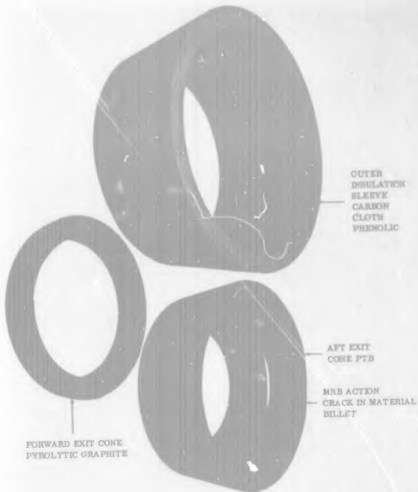
Figure 44. Orifice 3 Components
