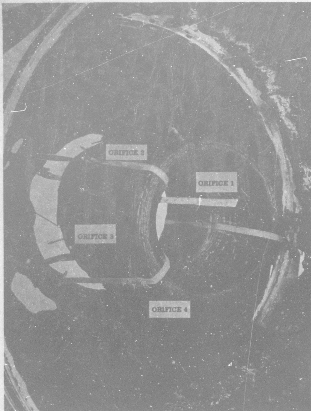
Figure 19. Nozzle-Case Closure Burnthrough
