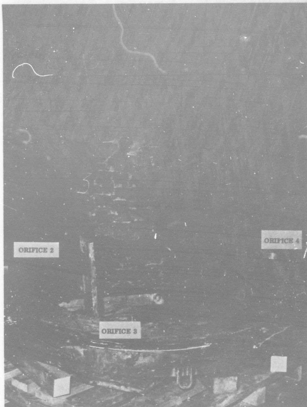
Figure 20. Nozzle Burnthrough, Ports 2, 3, and 4
