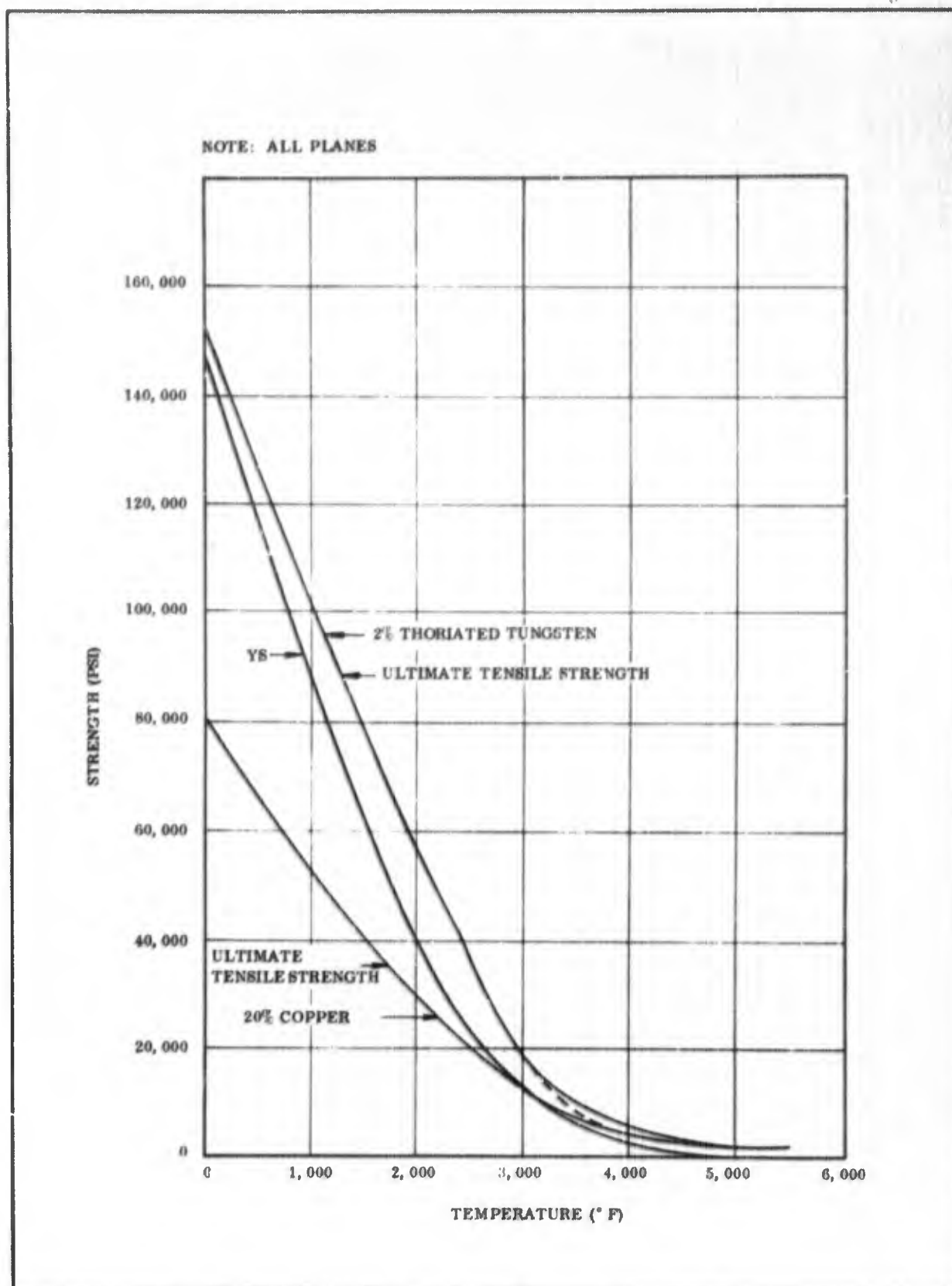
Figure 134. Tungsten, Ultimate and Yield Strength vs Temperature
