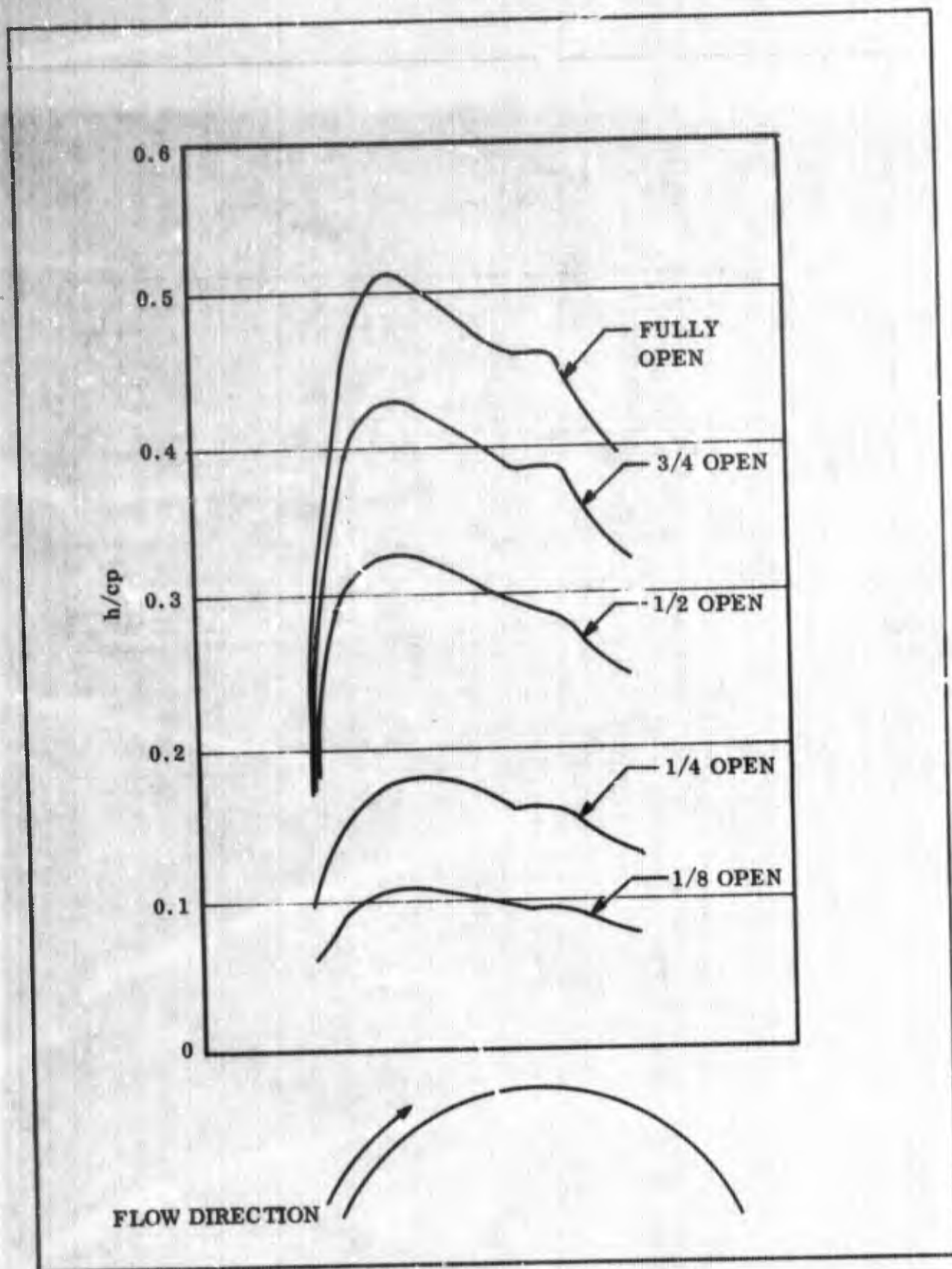
Figure 115. h/c_p Around Support Leg
