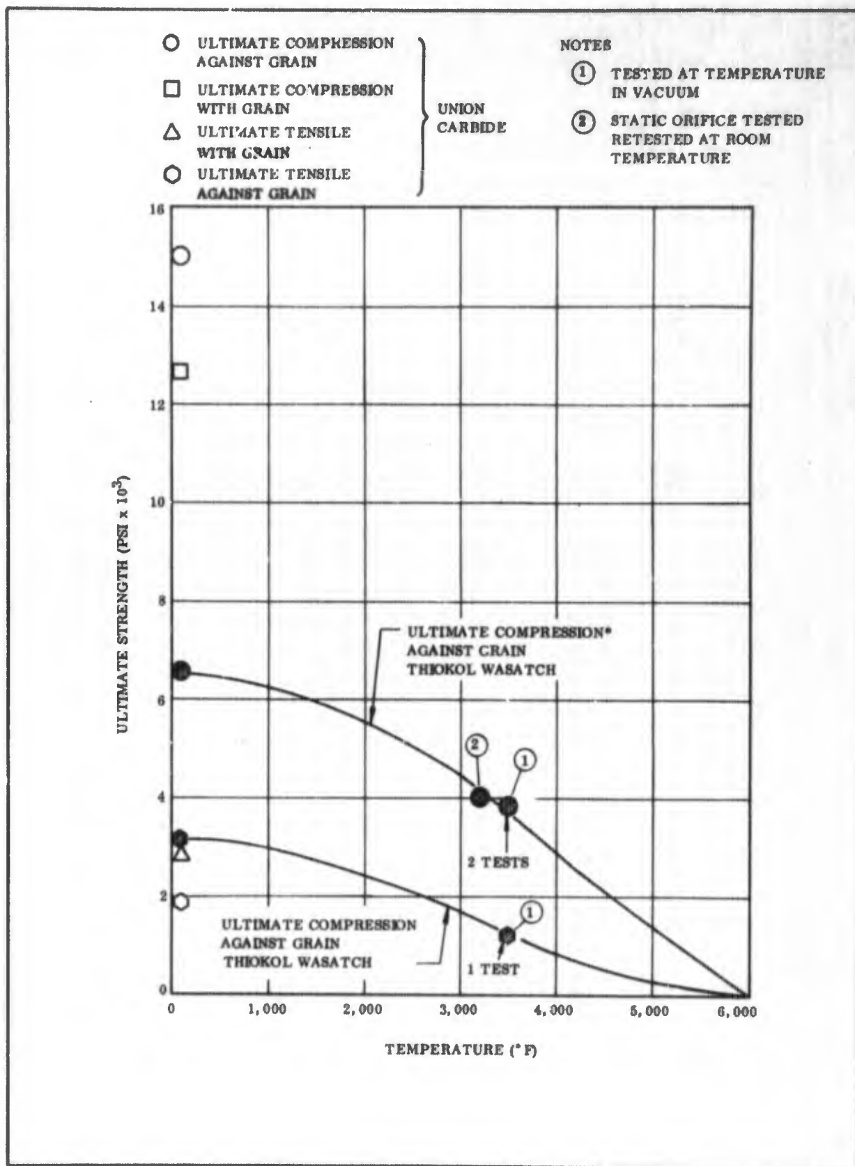
Figure 142. PTB Revised, Ultimate Tensile, Compressive and Shear Strength vs Temperature
