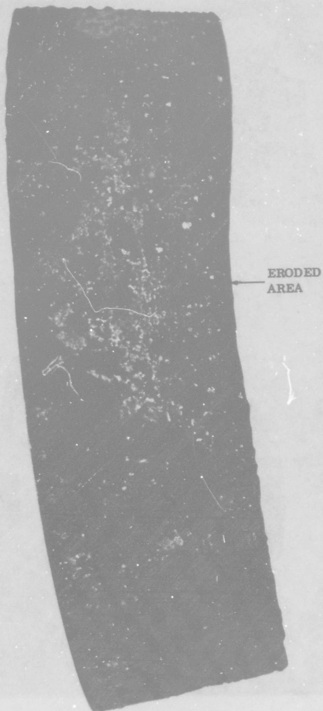
Figure 31. Port 2 Tungsten Throat
