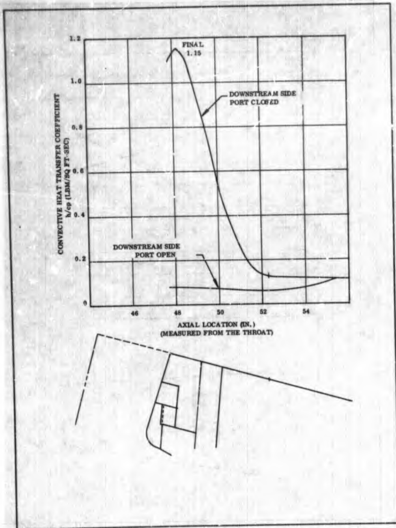
Figure 98. Downstream Nozzle Wall h/c_p vs Axial Location - Port Open and Closed
