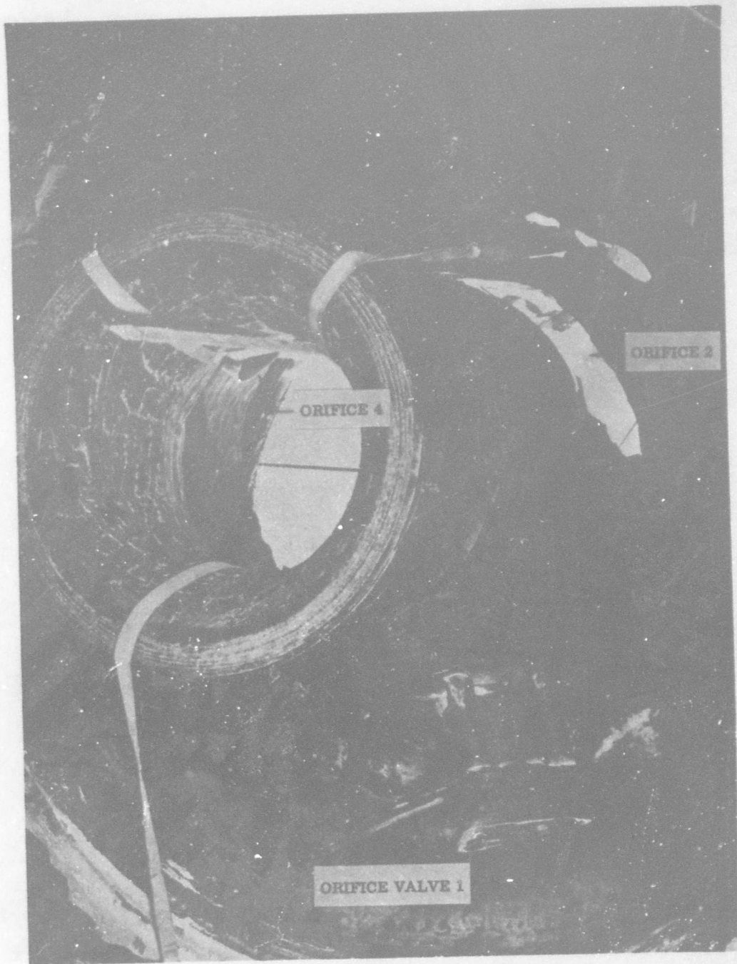
Figure 18. Port 1 Nozzle Burnthrough
