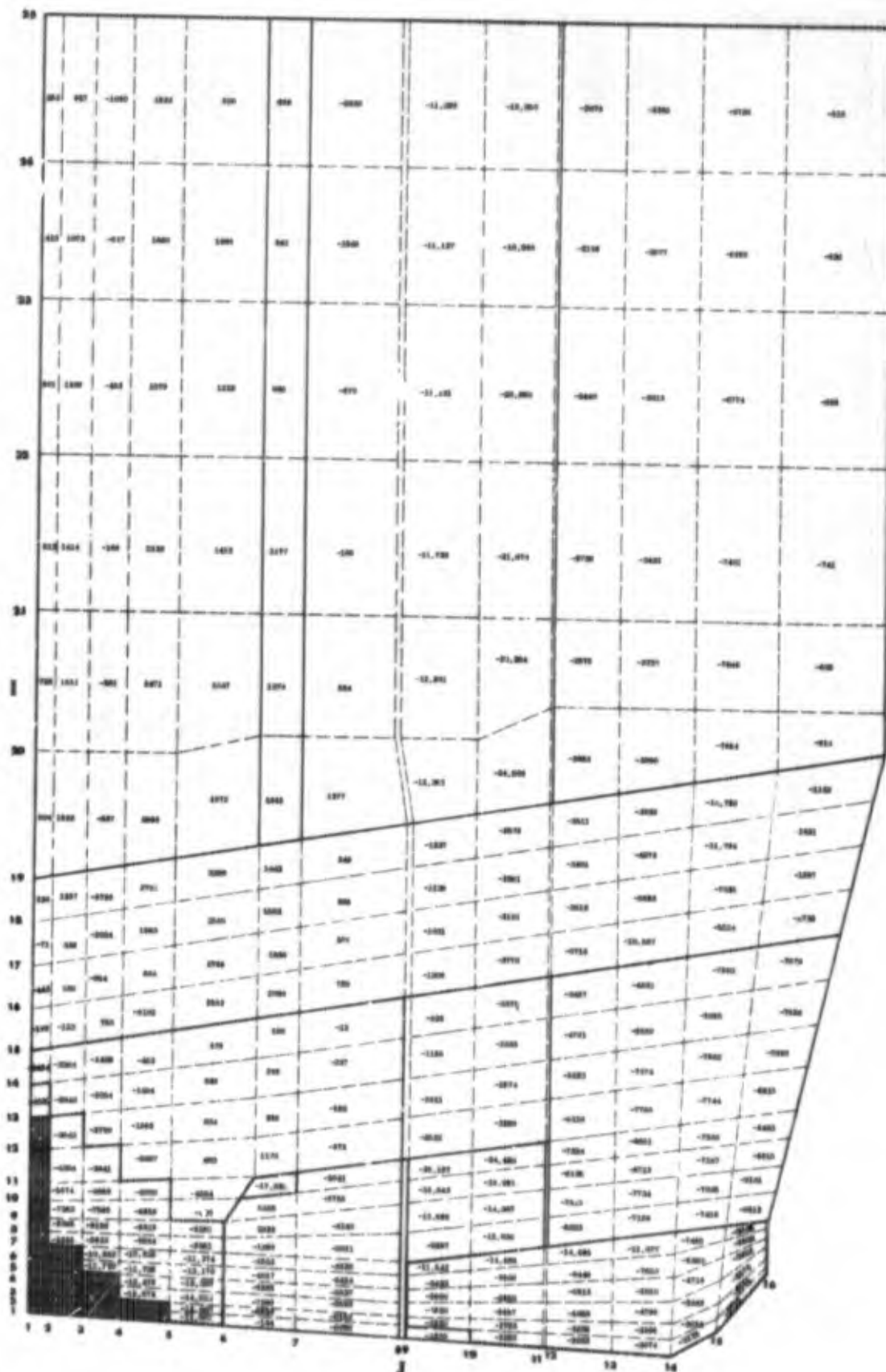
Figure 160. Boundary Condition A, Hoop Stress at 25.0 Sec, Valve Open
