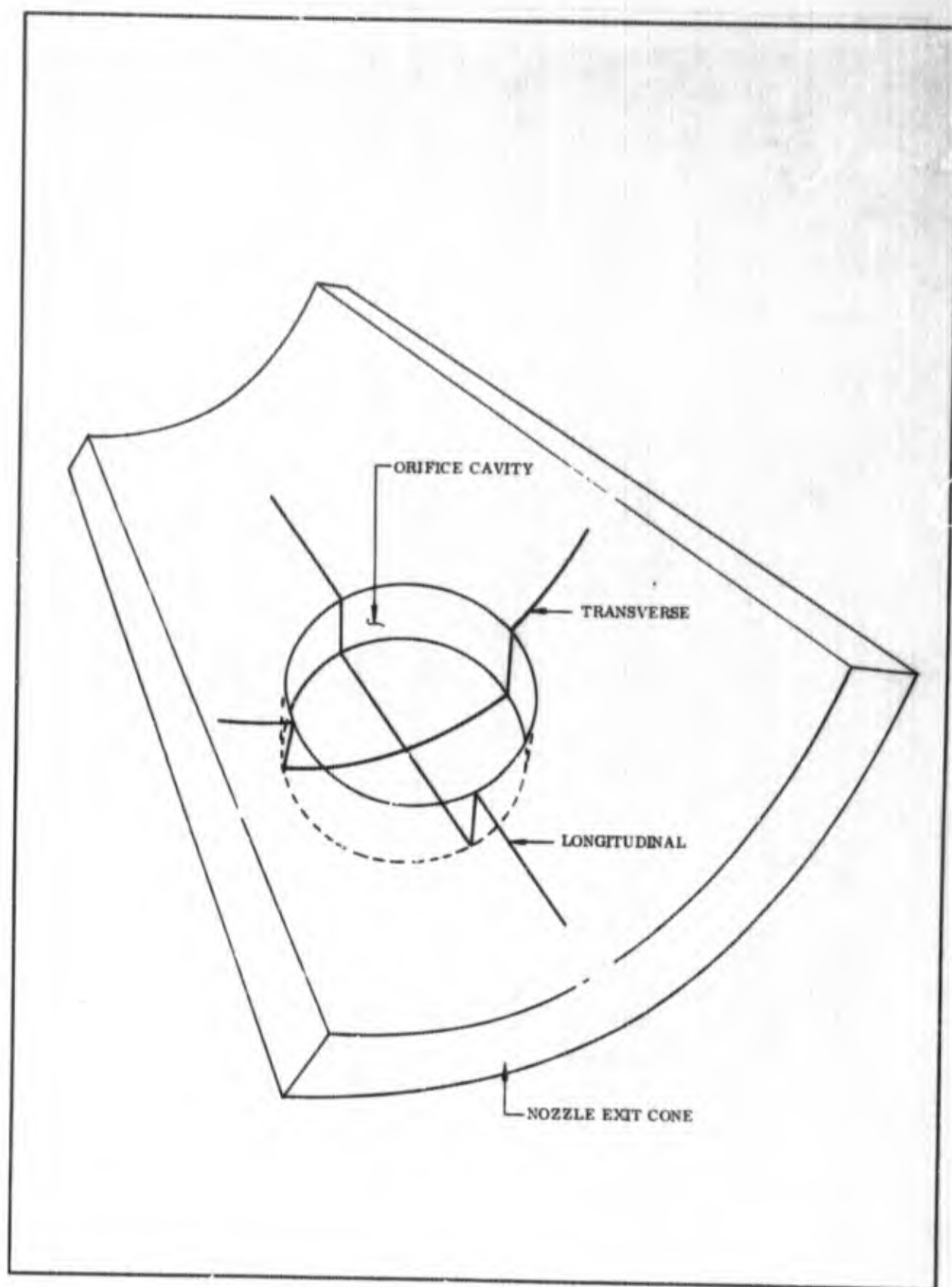
Figure 55. Plane of Gas Flow Conditions for Thermal Analysis
