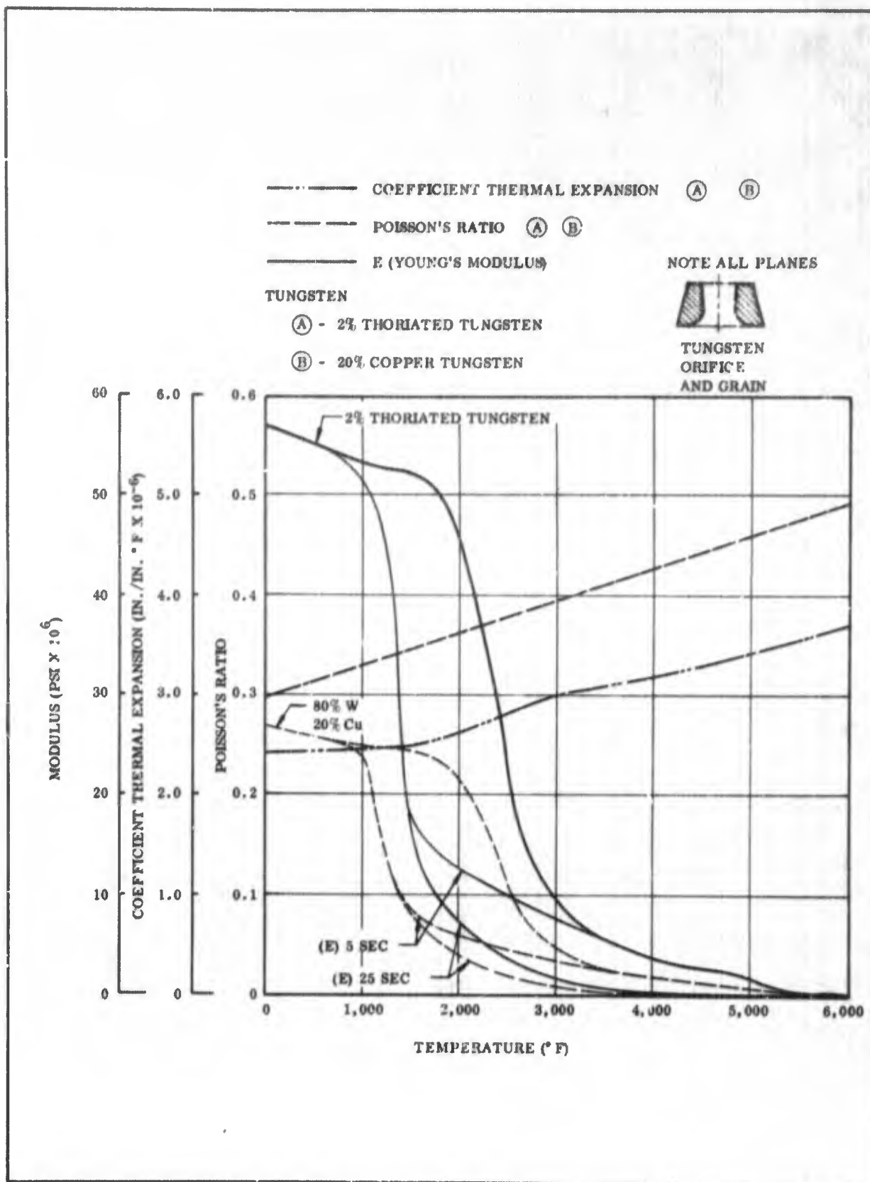
Figure 130. Tungsten CTE, E, Poisson's Ratio vs Temperature
