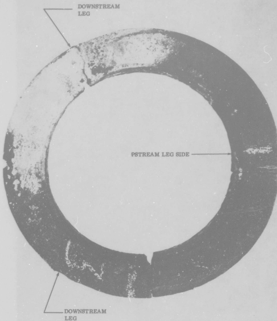
Figure 24. Port 1 Graphite - Inlet Face
