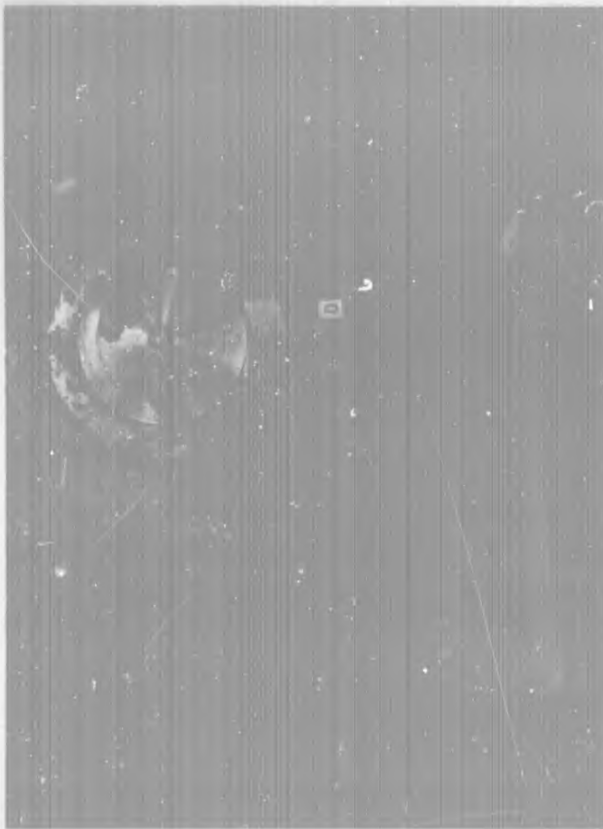
Figure 88. Orifice Smear Pattern, Perpendicular to Centerline, for PTB Missing
