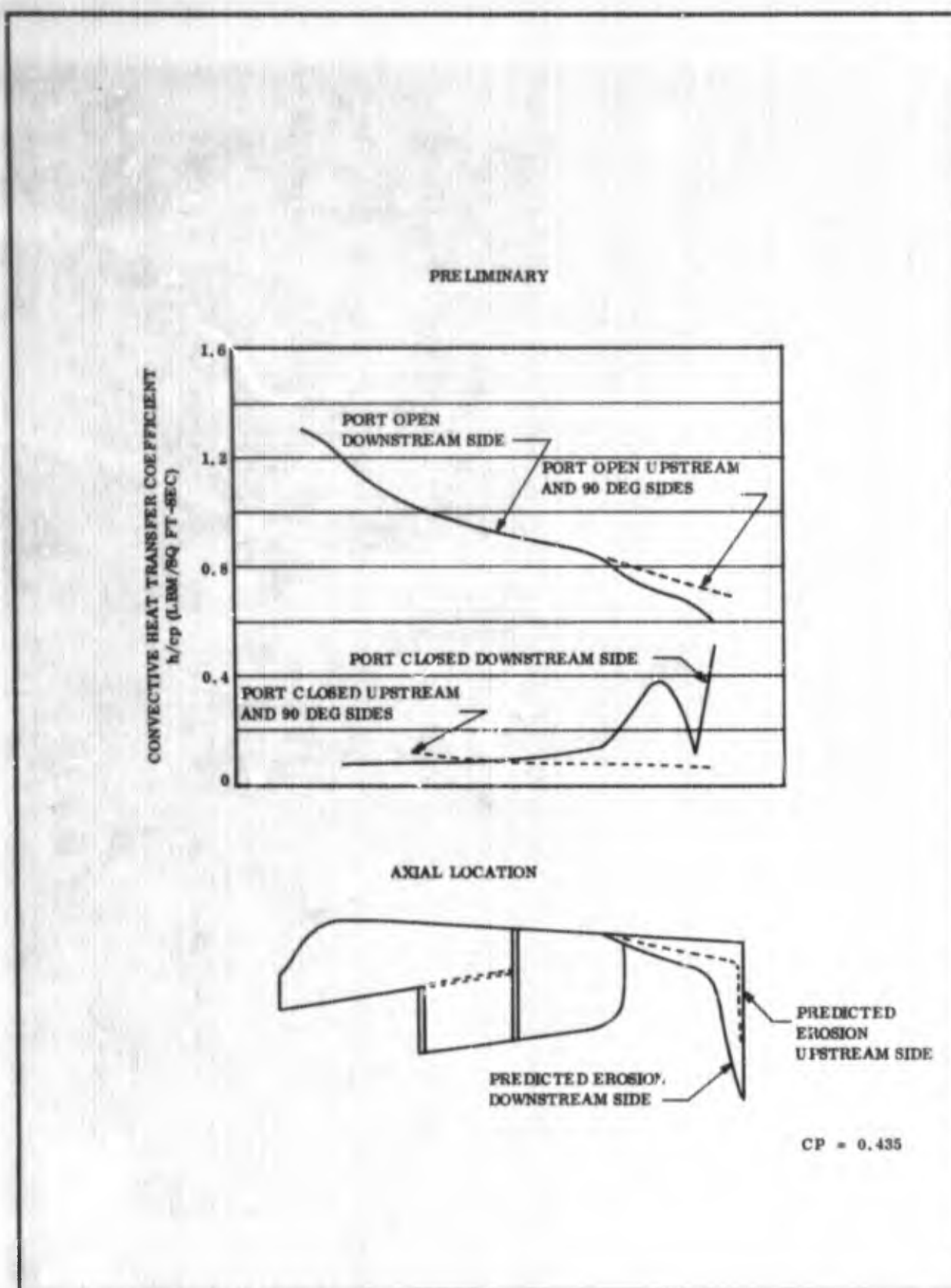
Figure 96. Orifice Wall h/c_p vs Axial Location at 25 Sec - Preliminary
