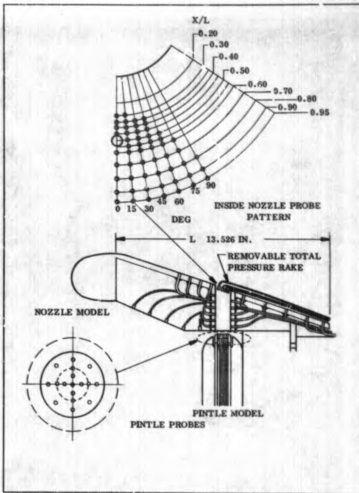
Figure 63. Cold Flow Test Model and Pressure Probe Locations
