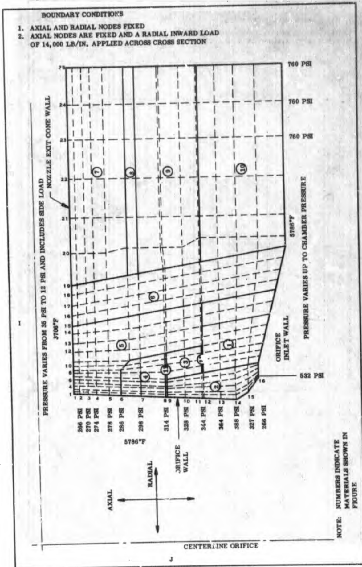
Figure 124. Orifice Port Boundary Conditions at 25.0 Sec, Valve Open
