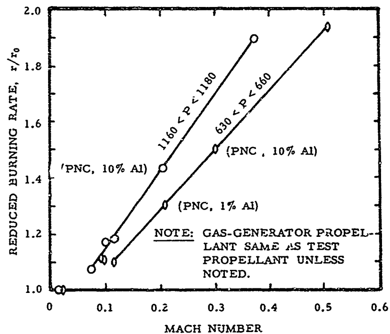
FIGURE 4. EFFECT OF VELOCITY ON AVERAGE BURNING RATES IN MOTORS FIRED UNDER EROSIVE BURNING CONDITIONS
