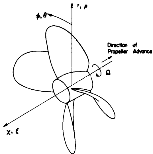
Figure 10 – Forces and Moments Acting on Propeller
