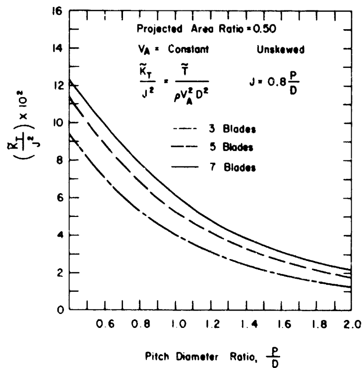
Figure 36 - Effect of Pitch on Blade-Frequency Thrust
