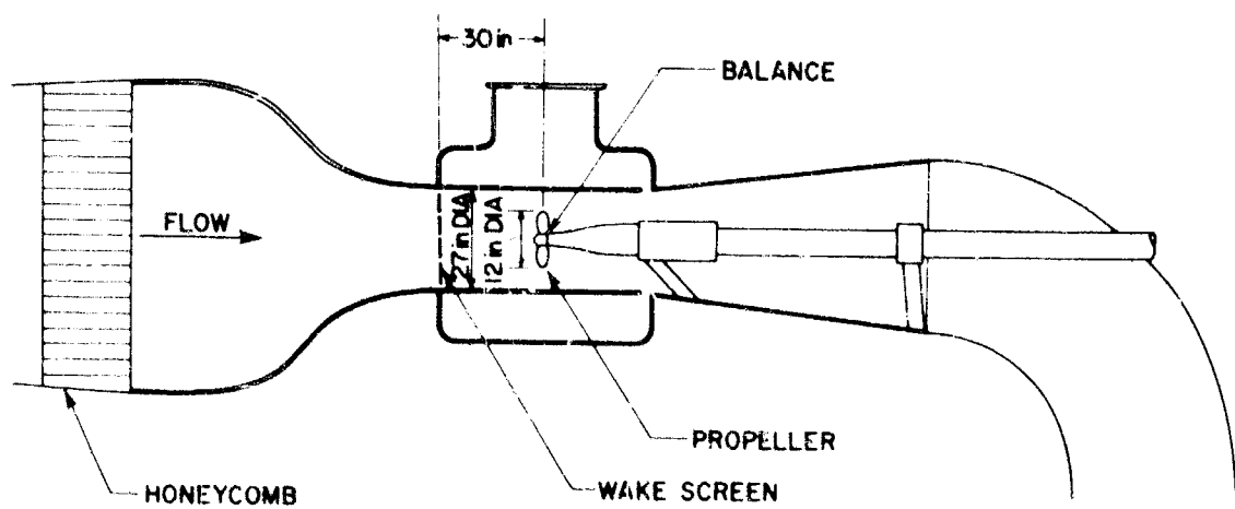
Figure 4 - Test Setup
