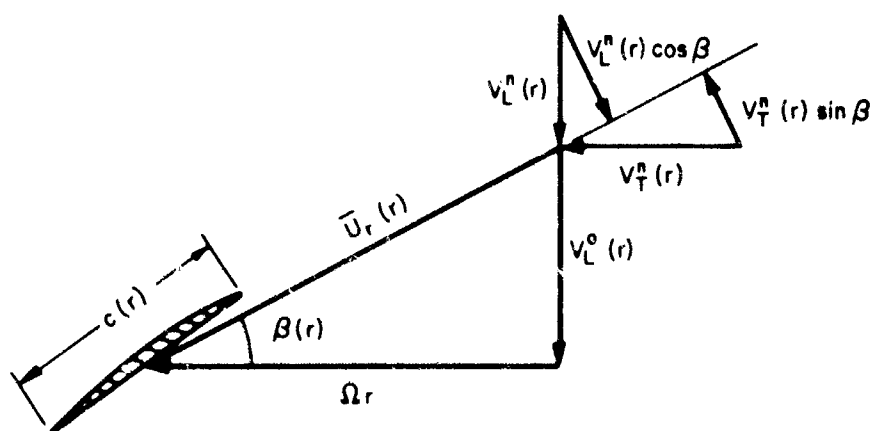
Figure 2 - Velocity Diagram
