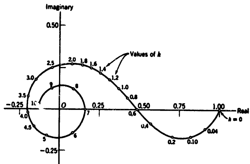
Figure 3 - Sears Function for Airfoil in Sinusoidal Gust
