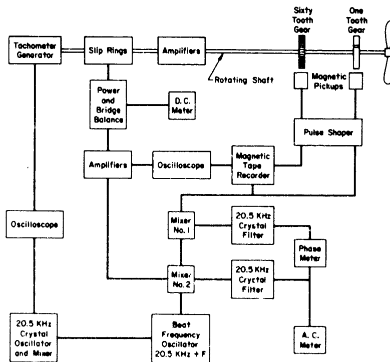
SCHEMATIC DIAGRAM OF INSTRUMENTATION
