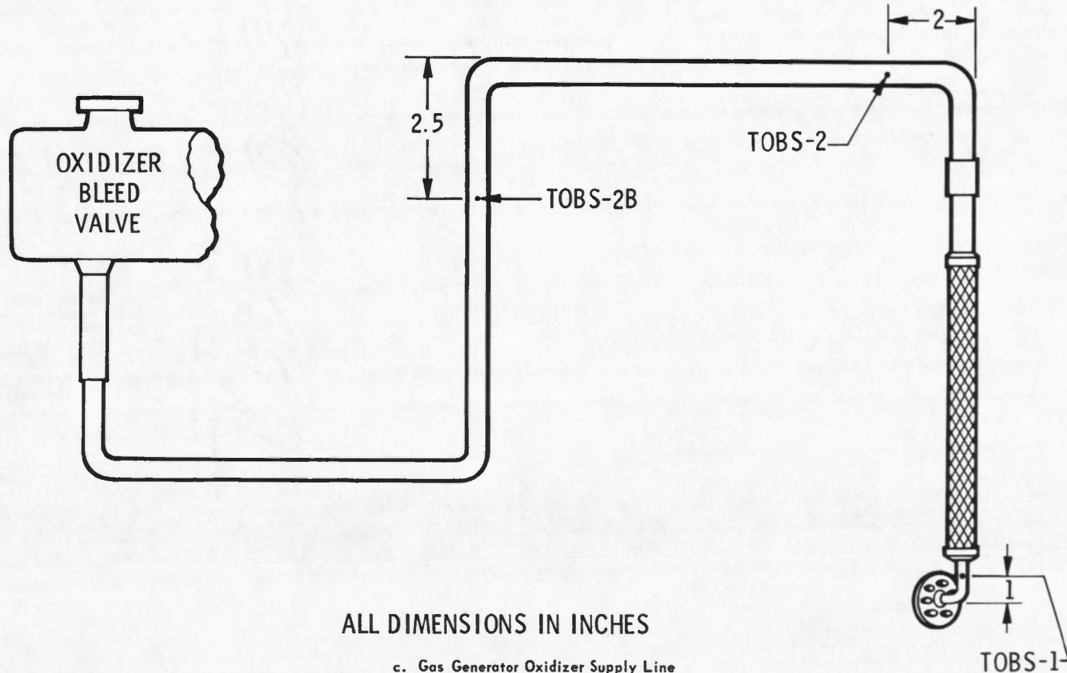
c. Gas Generator Oxidizer Supply Line Fig. III-1 Continued
