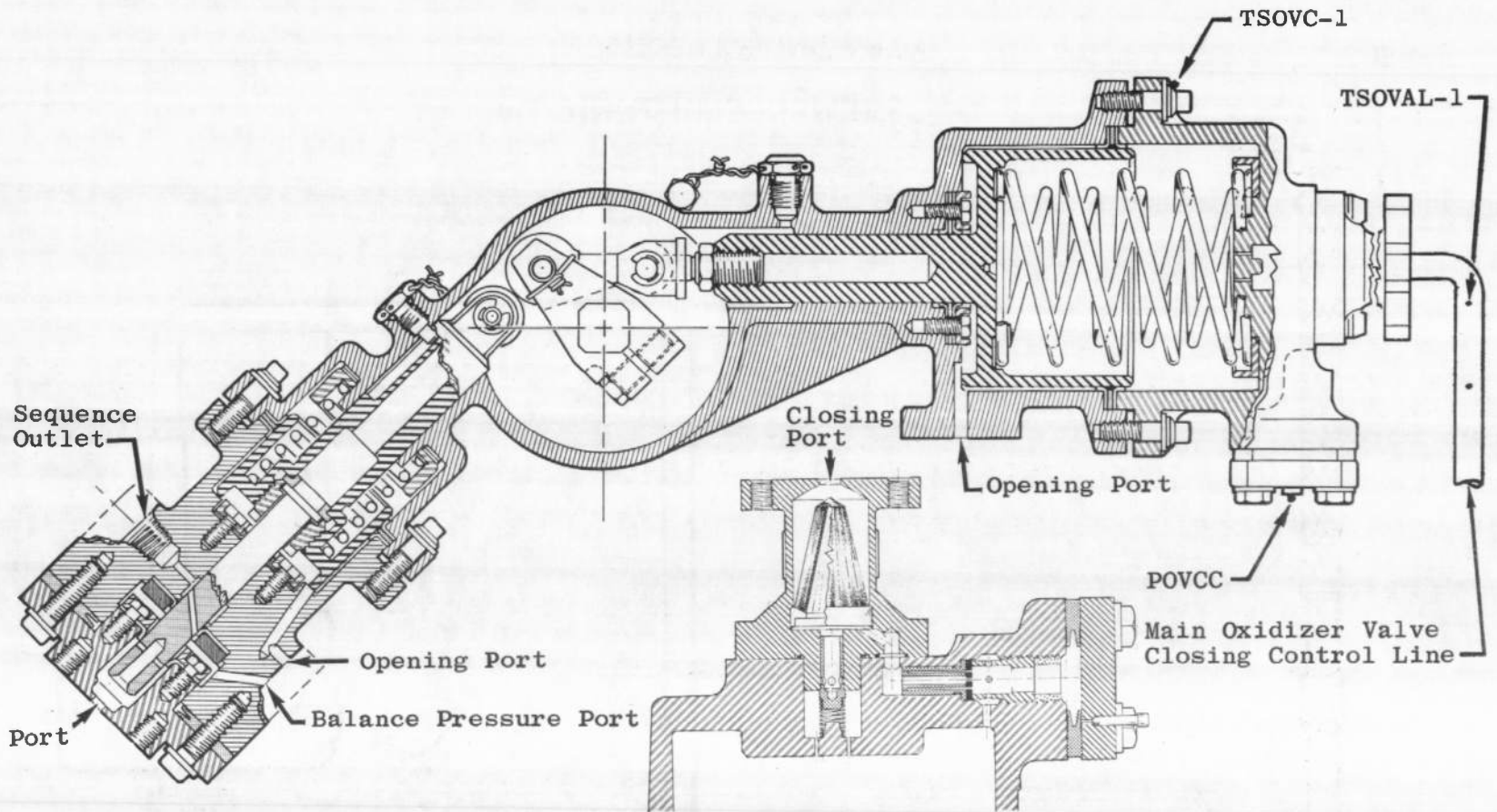
d. Main Oxidizer Valve Fig. III-1 Continued
