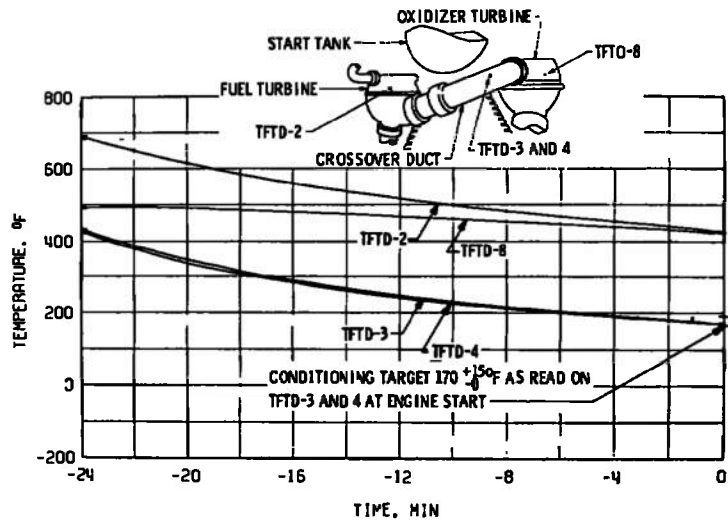
b. Crossover Duct, TFTD
