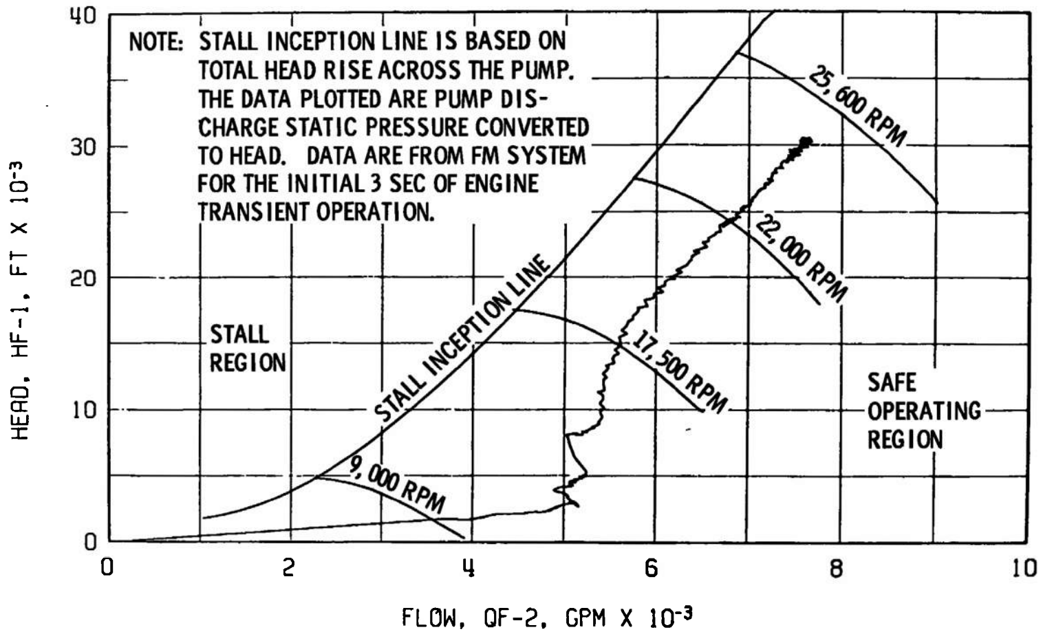
Fig. 15 Fuel Pump Start Transient Performance, Firing 09B
