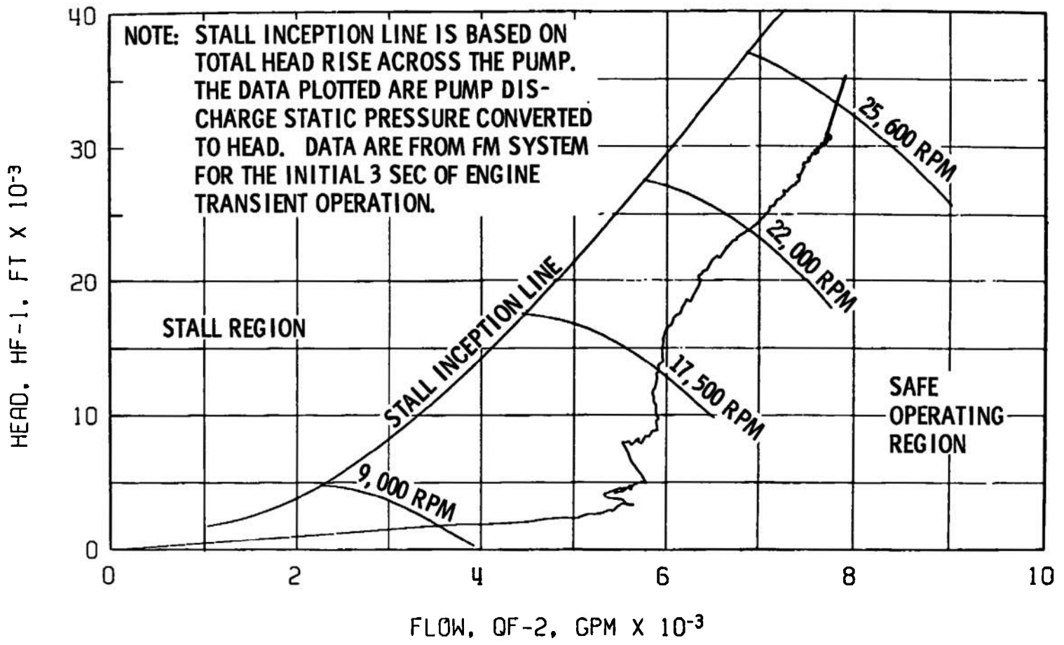
Fig. 27 Fuel Pump Start Transient Performance, Firing 09E
