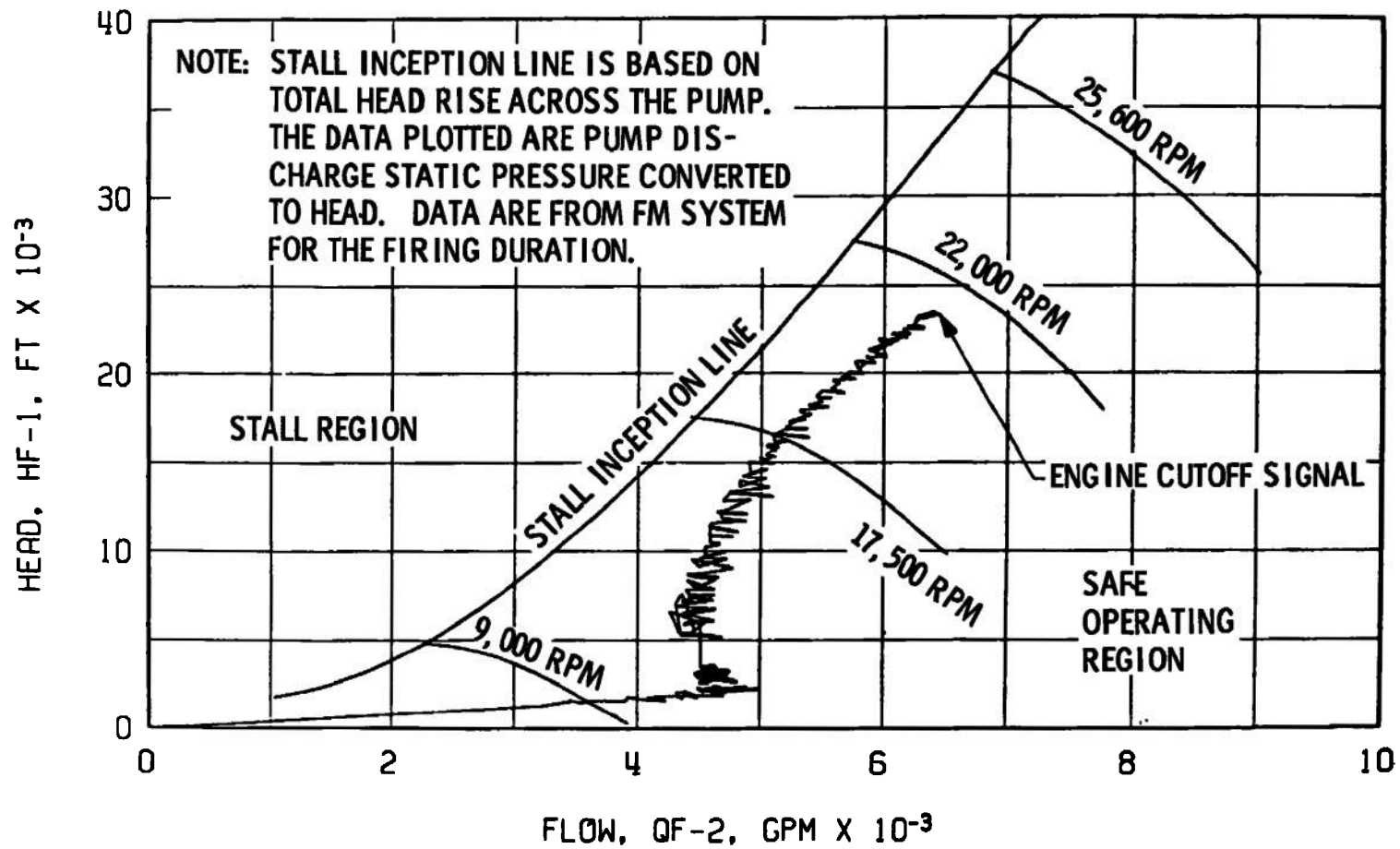
Fig. 59 Fuel Pump Start Transient Performance, Firing 11E
