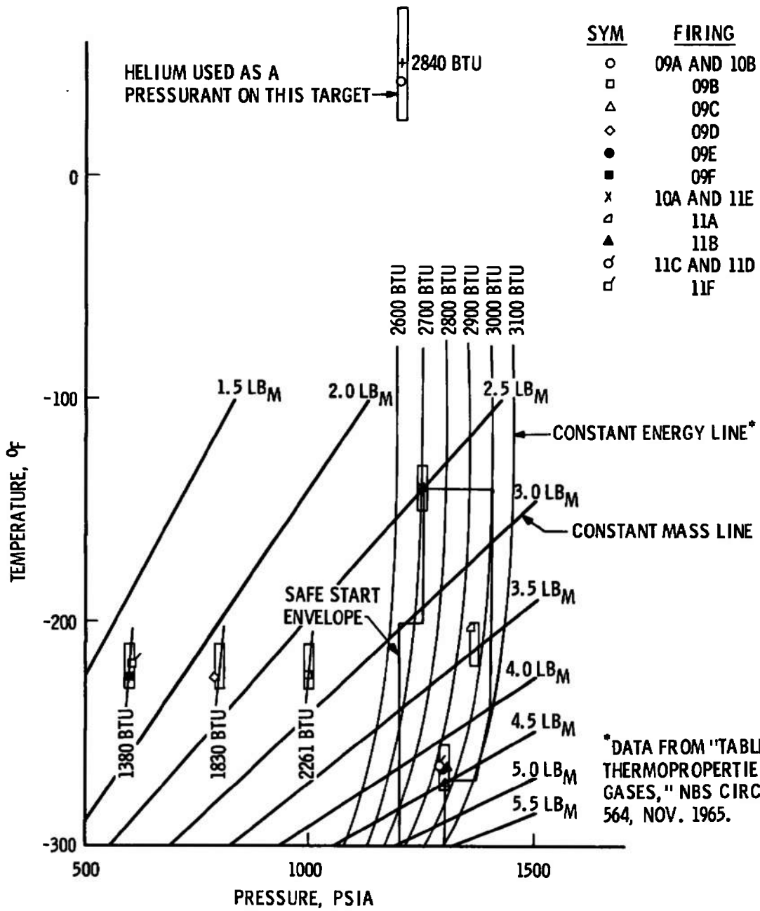
c. Start Tank Fig. 8 Continued
