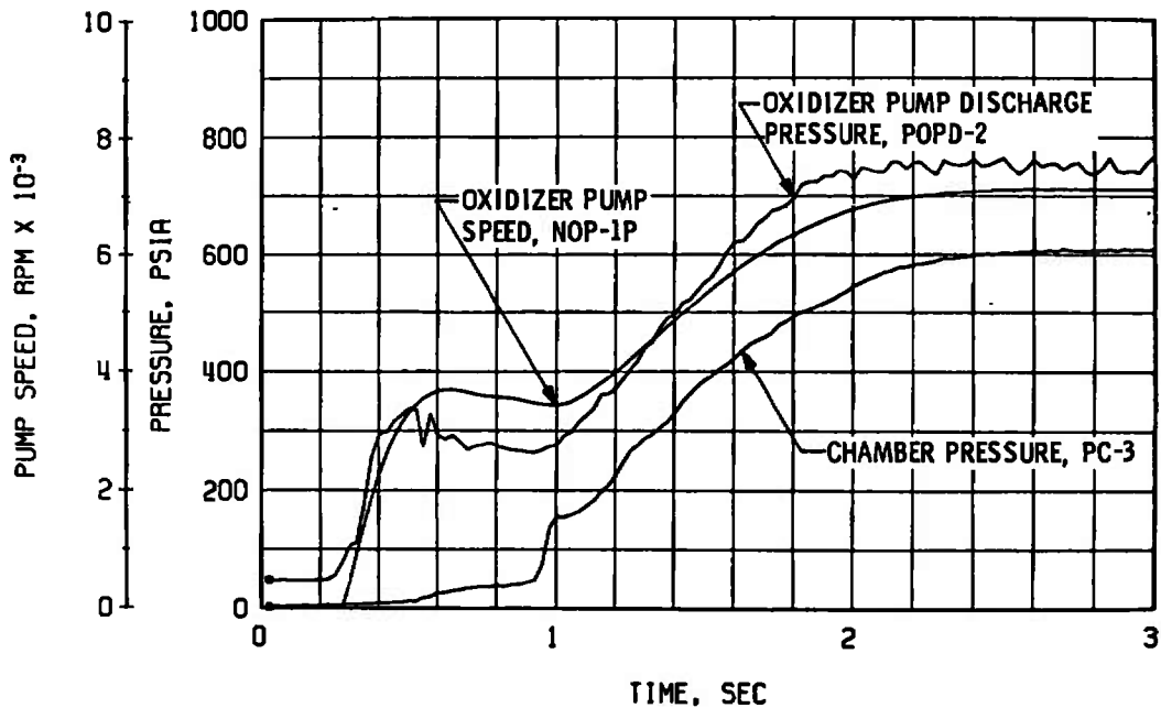
b. Thrust Chamber Oxidizer System, Start Fig.-46 Engine Transient Operation, Firing 11B
