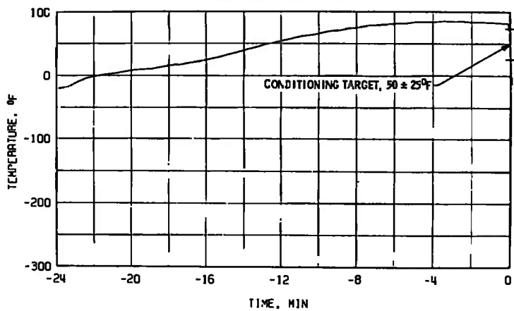
c. Thrust Chamber Throat, TTC-1P
