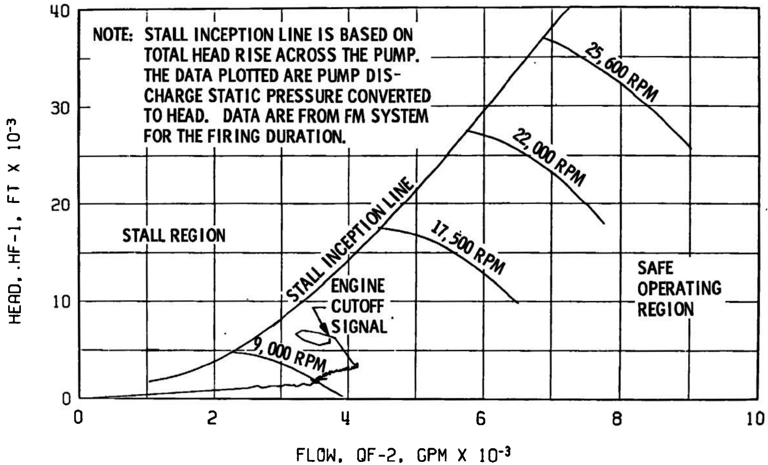
Fig. 63 Fuel Pump Start Transient Performance, Firing 11F
