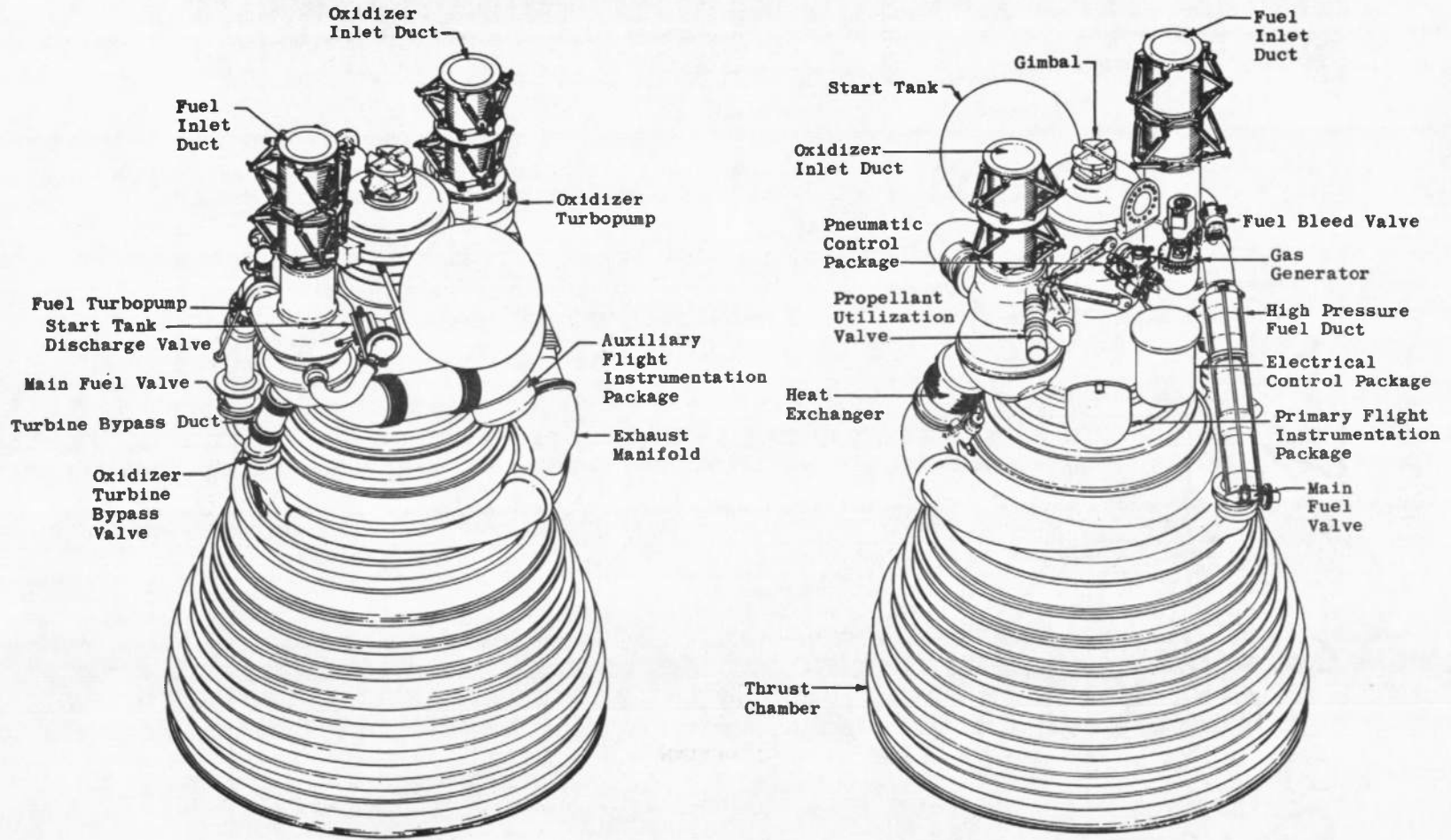
a. Major Engine Components Fig. 3 Engine Details
