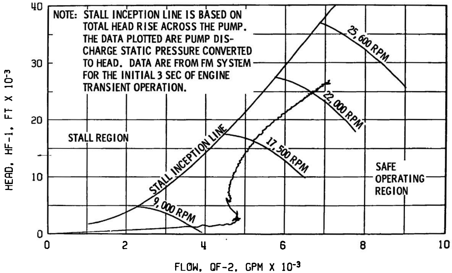
Fig. 39 Fuel Pump Start Transient Performance, Firing 10B
