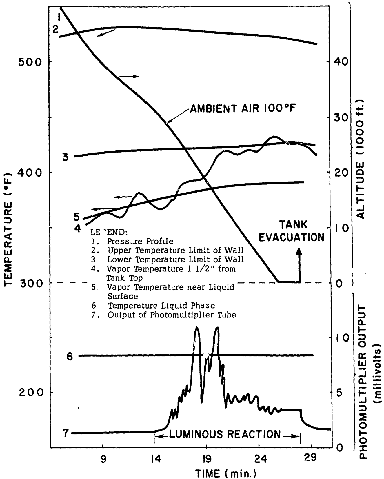
Figure 53. Representative Data Showing Temperature, Pressure and Photomultiplier Output During Descent of Test 5C
