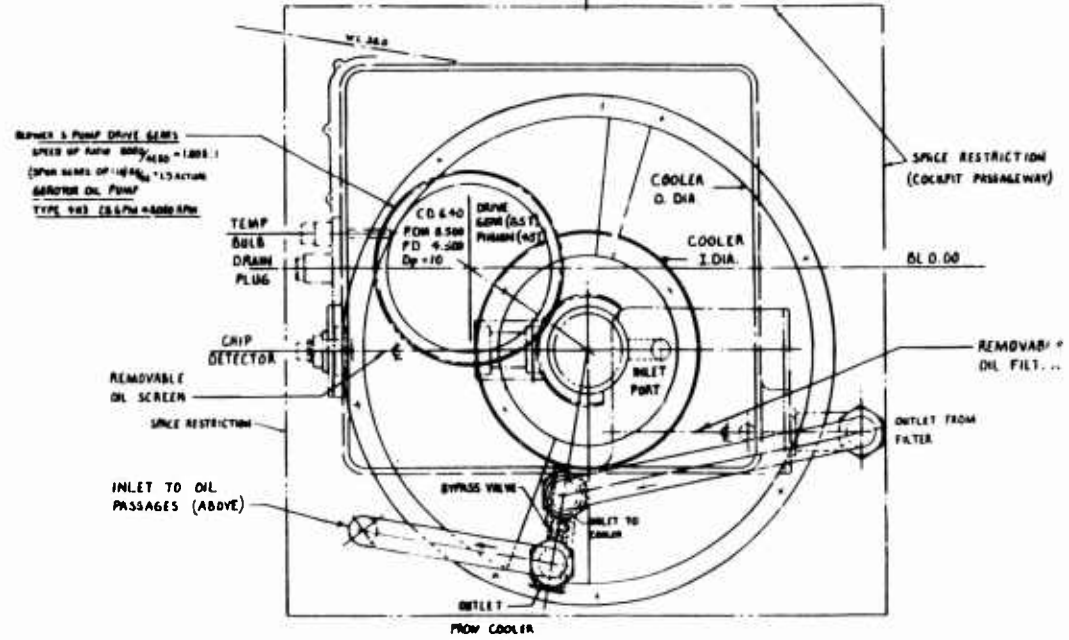
Centerline Section of Integrally Cooled Transmission.
