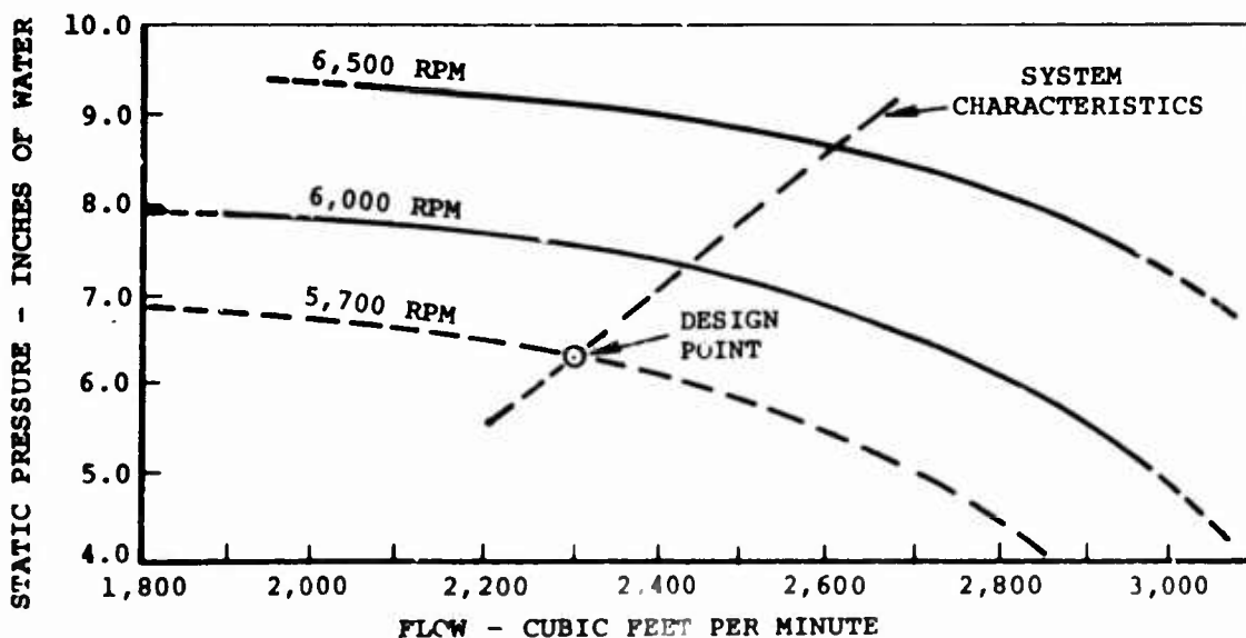
Figure 29. Blower Performance.
