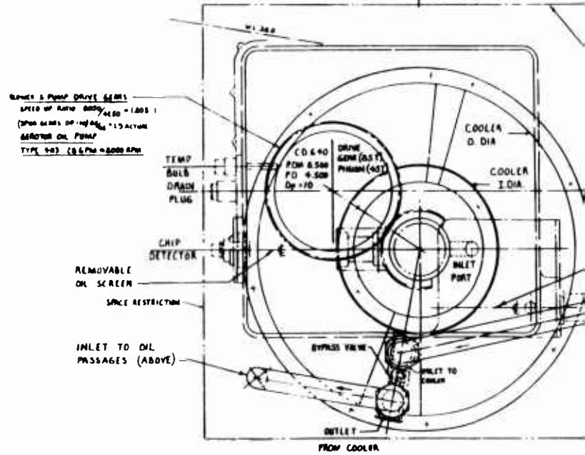
Figure 18. Centerline Section of Integrally Cooled Transmission.
