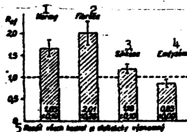
Fig. 5. Relation of effective ventilation of lungs to effective ventilation of model, if V_{eff}(l) = \frac{V_{eff}(l)}{V_{eff}(m)} - Rat. 1) Standards; 2) fibrosis; 3) silicosis; 4) emphysema; 5) the distributions of all values are statistically significant.
