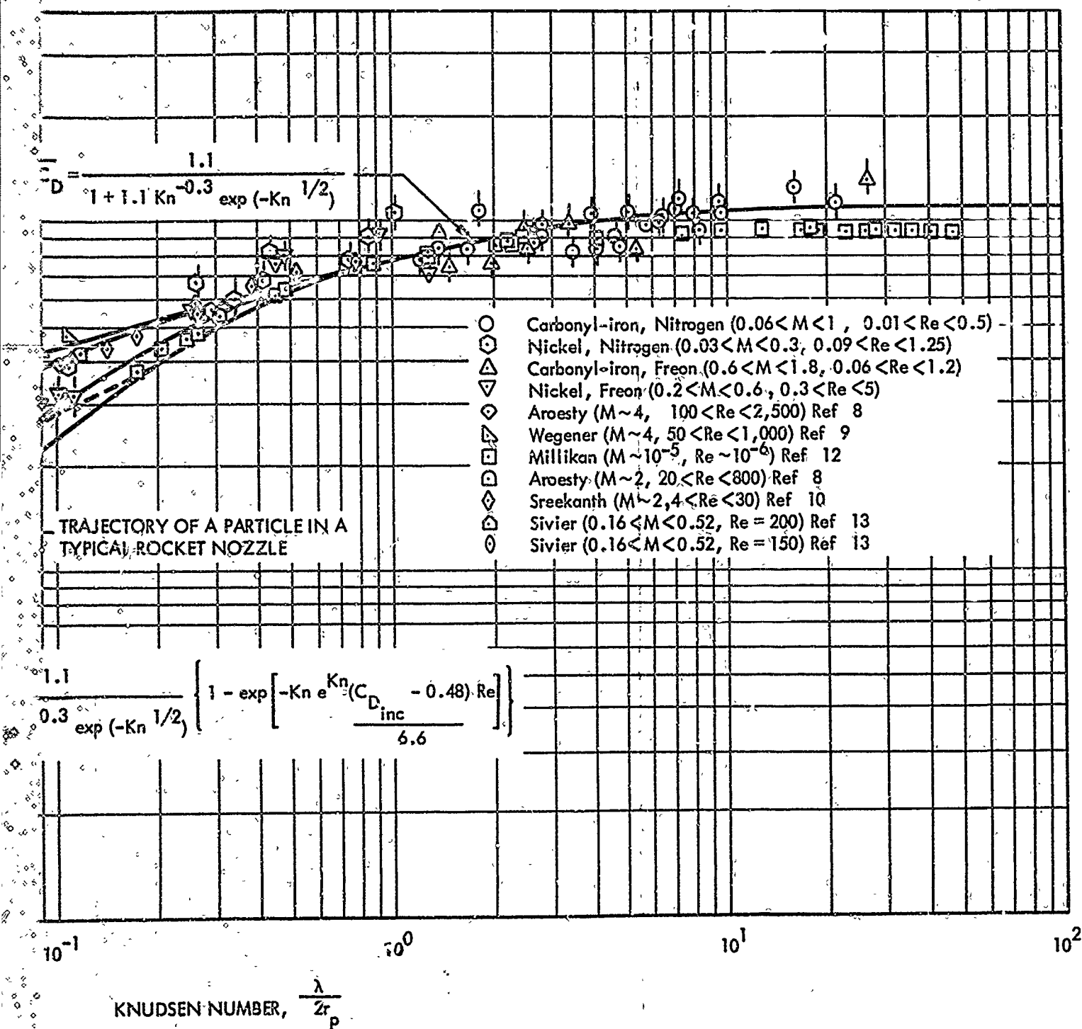
Figure 17. Nondimensional Drag Coefficient for a Sphere vs Knudsen Number
