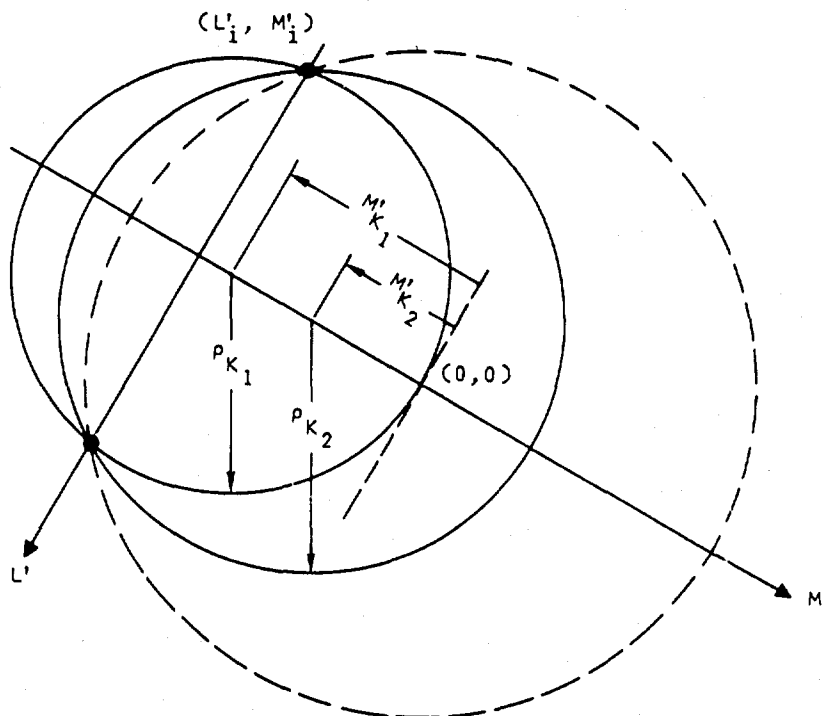
FIG. 10. Gain Circle Intersections.
