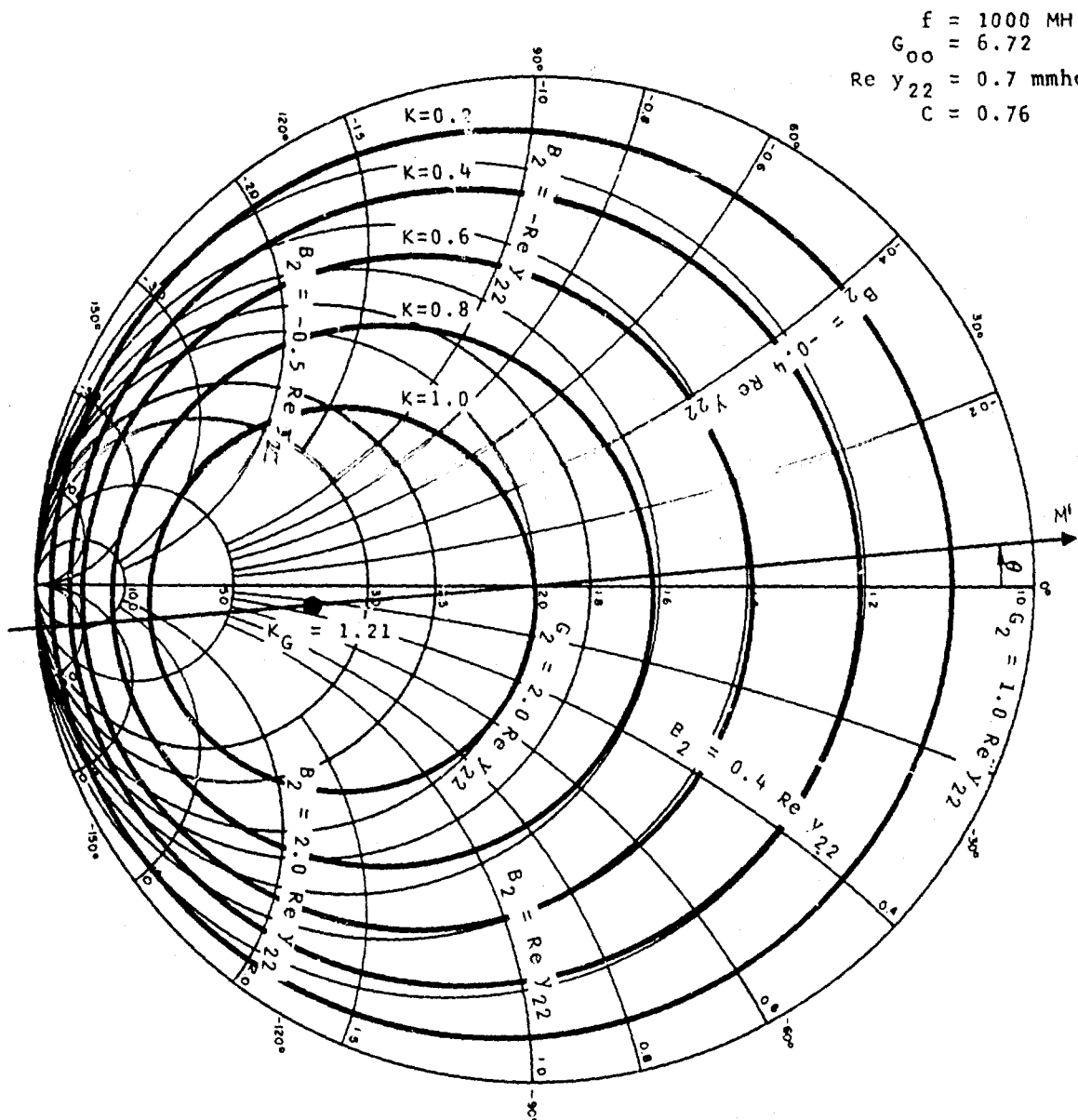
FIG. 8. Linville Chart for C = 0.76 .
