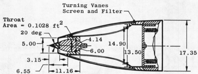
All Dimensions in Inches
