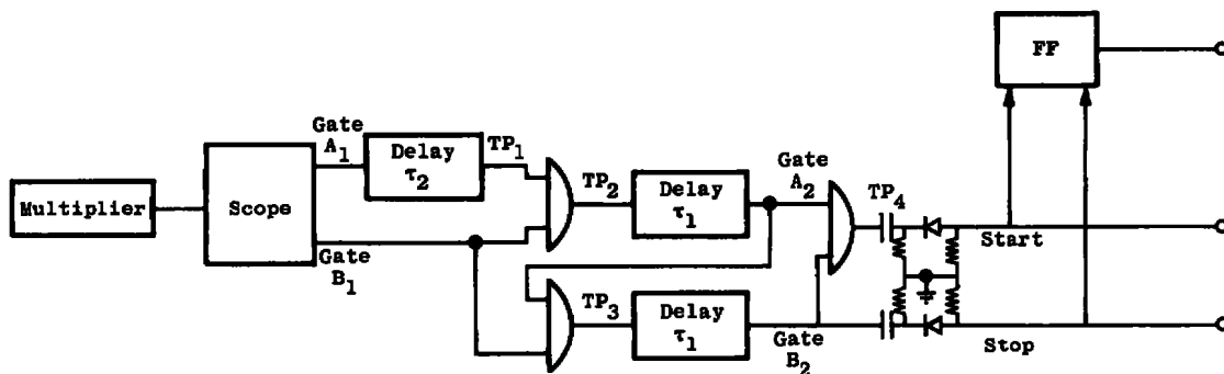
Fig. 22 Particle Velocity Instrumentation Schematic
