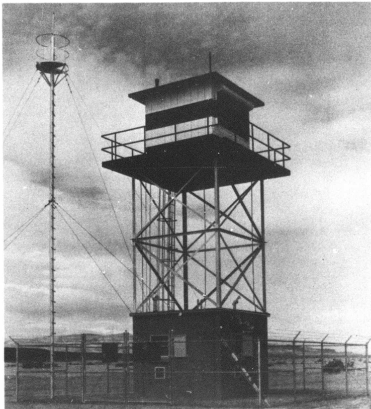
FIG. 7. Spotting Tower.
