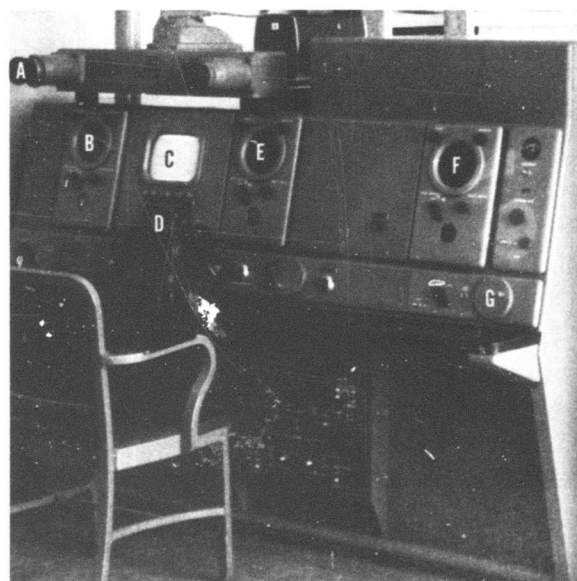
FIG. 8. M-33 Radar Tracker. (A) Optics system, (B) elevation scope, (C) TV monitor, (D) azimuth elevation monitor, (E) azimuth scope, (F) range scope, and (G) range control.
