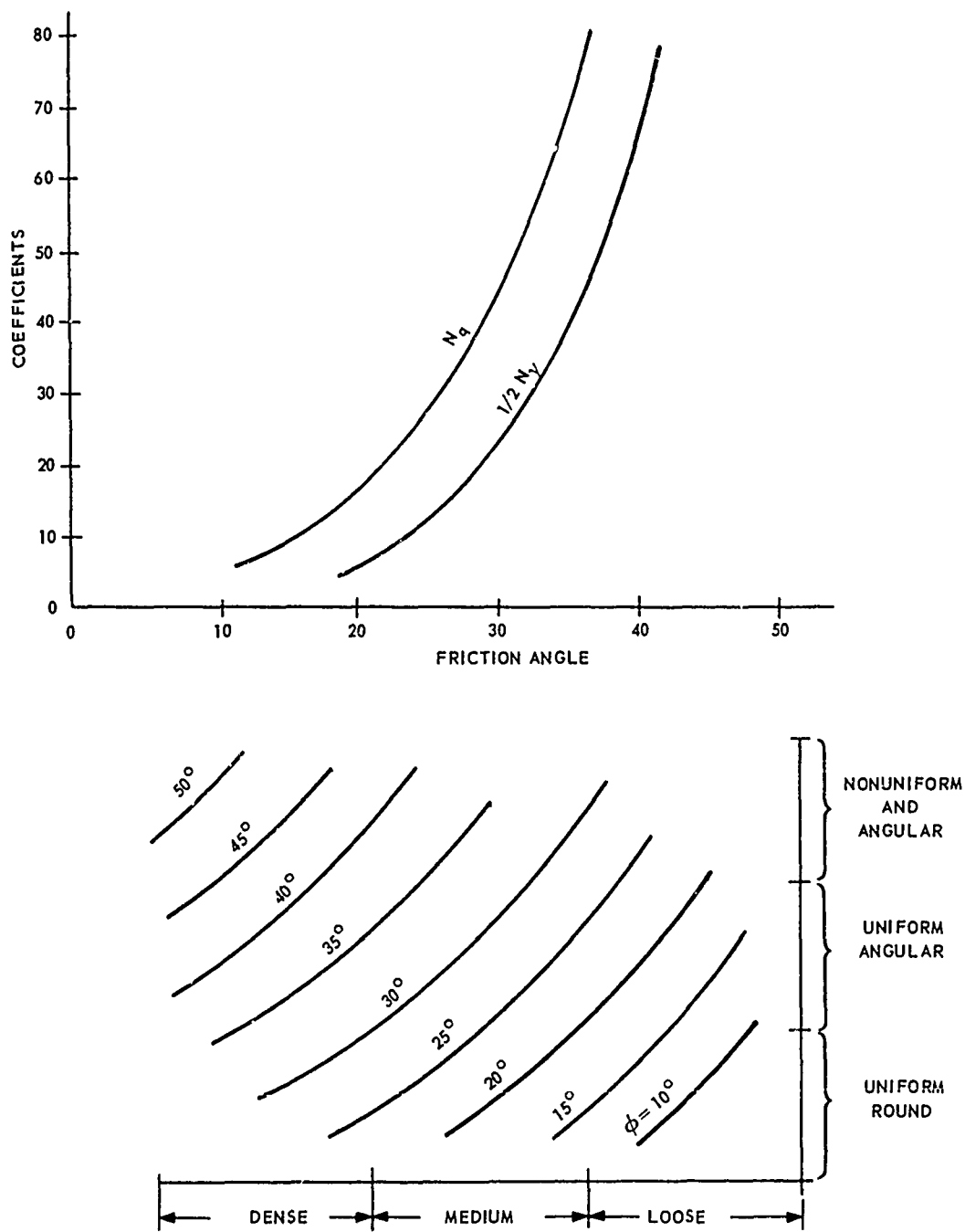
Figure 2-3. Bearing Capacity Coefficients and Friction Angle for Cohesionless Sand.
