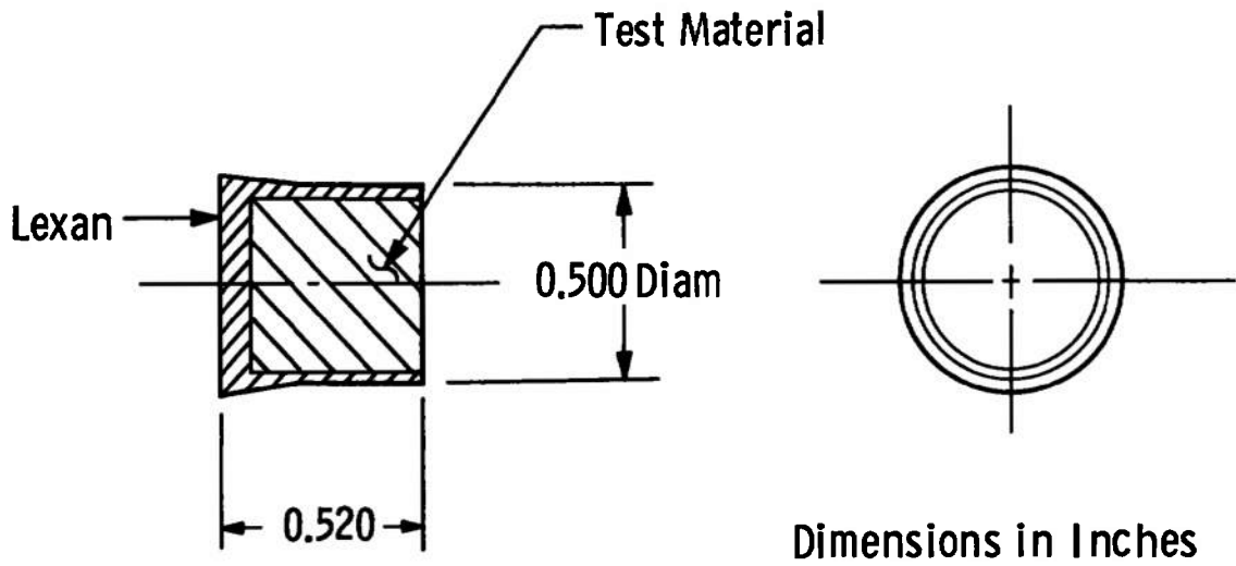
Fig. 3 Projectile with Test Material Insert
