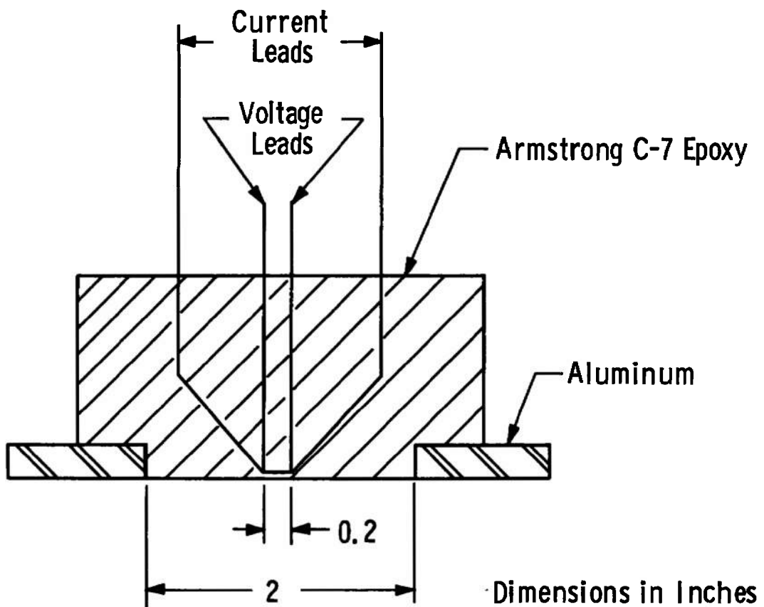
Fig. 4 Manganin-Epoxy Transducer
