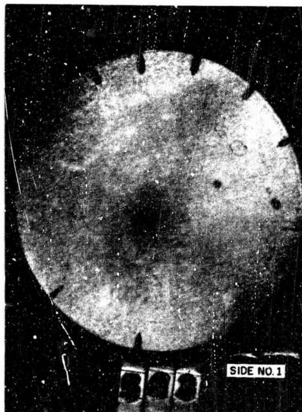
Figure 2 CRACKS AND POROSITY DETECTED BY DYE PENETRANT TECHNIQUE
