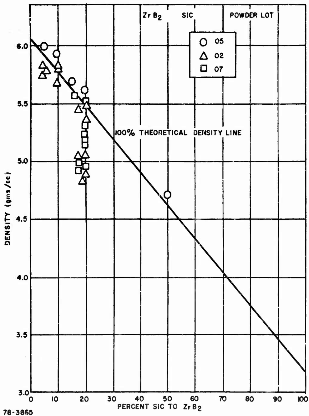
Figure 19 EFFECT OF SIC ADDITIONS TO ZrB 2 ON DENSITY OF BILLETS
