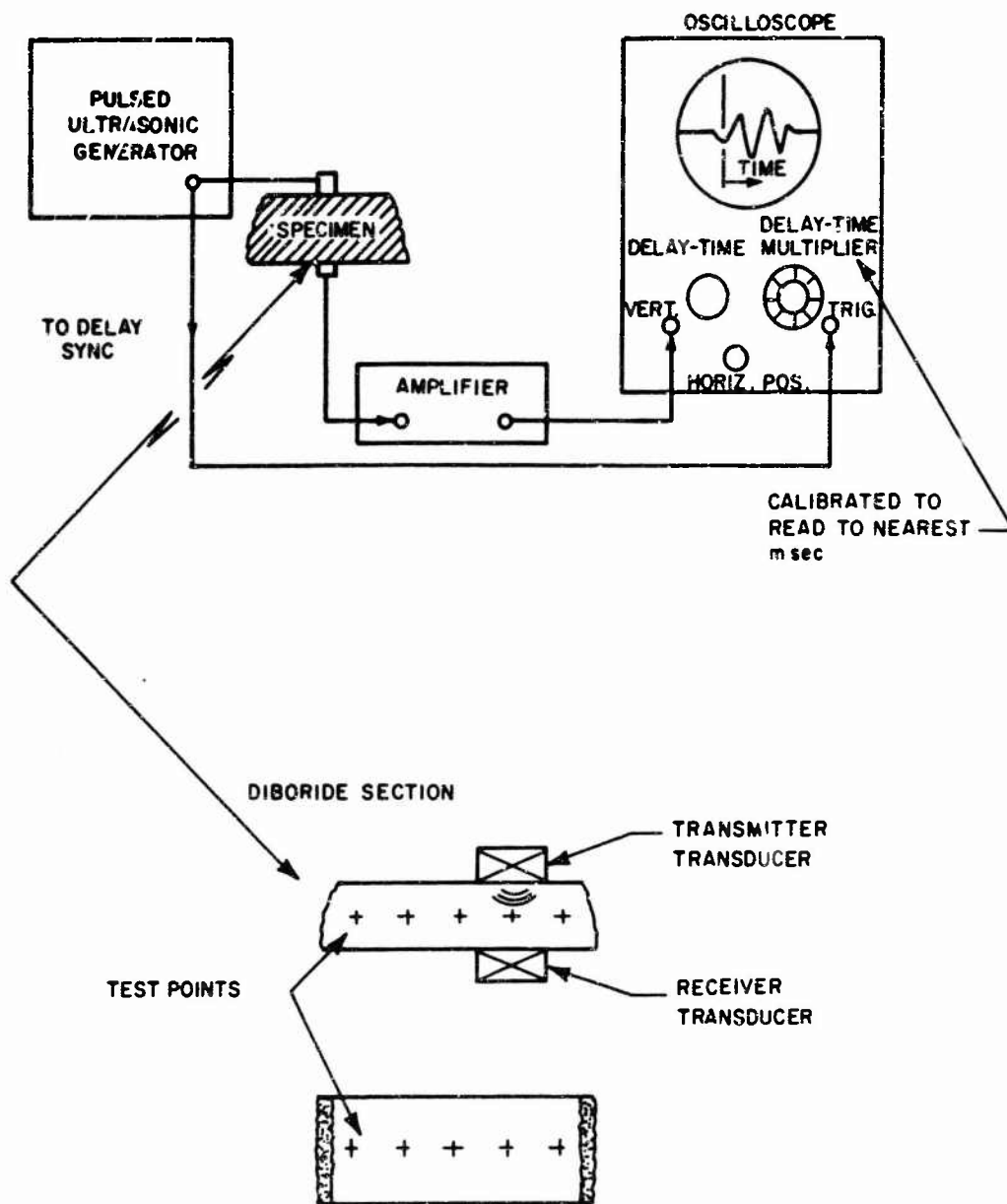
Figure 16 DIAGRAM OF ULTRASONIC VELOCITY MEASURING APPARATUS
