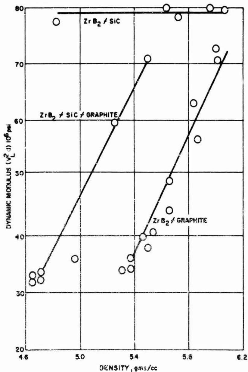
Figure 26 EFFECTS OF ADDITIONS OF SiC AND/OR GRAPHITE TO ZrB₂ ON DYNAMIC MODULUS
