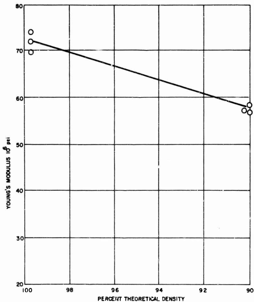
Figure 20 YOUNG'S MODULUS VERSUS DECREASING DENSITY (POROSITY) IN \text{ZrB}_2 + 20 PERCENT SiC
