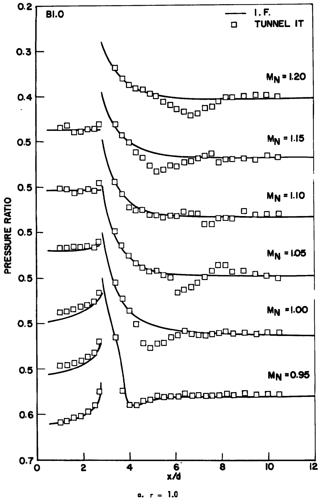
Fig. 12 Model Pressure Distributions with Wall B, \theta_w = 0
