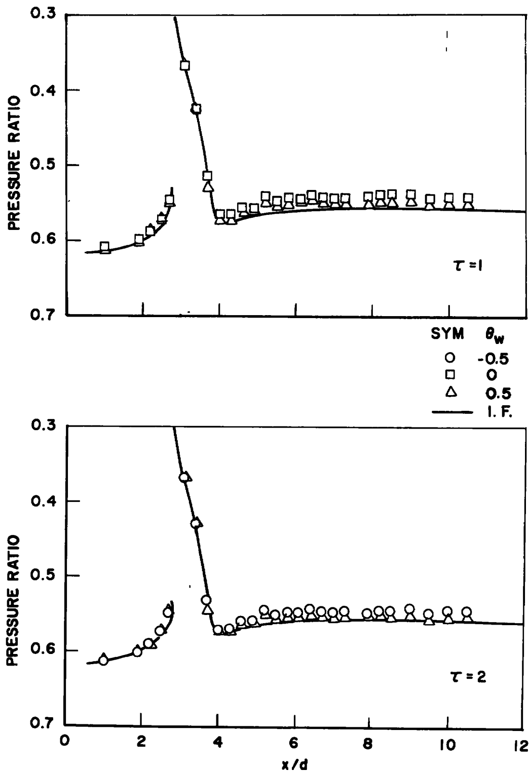
Fig. 17 Influence of Wall Angle upon the Model Pressure Distributions with Wall C
