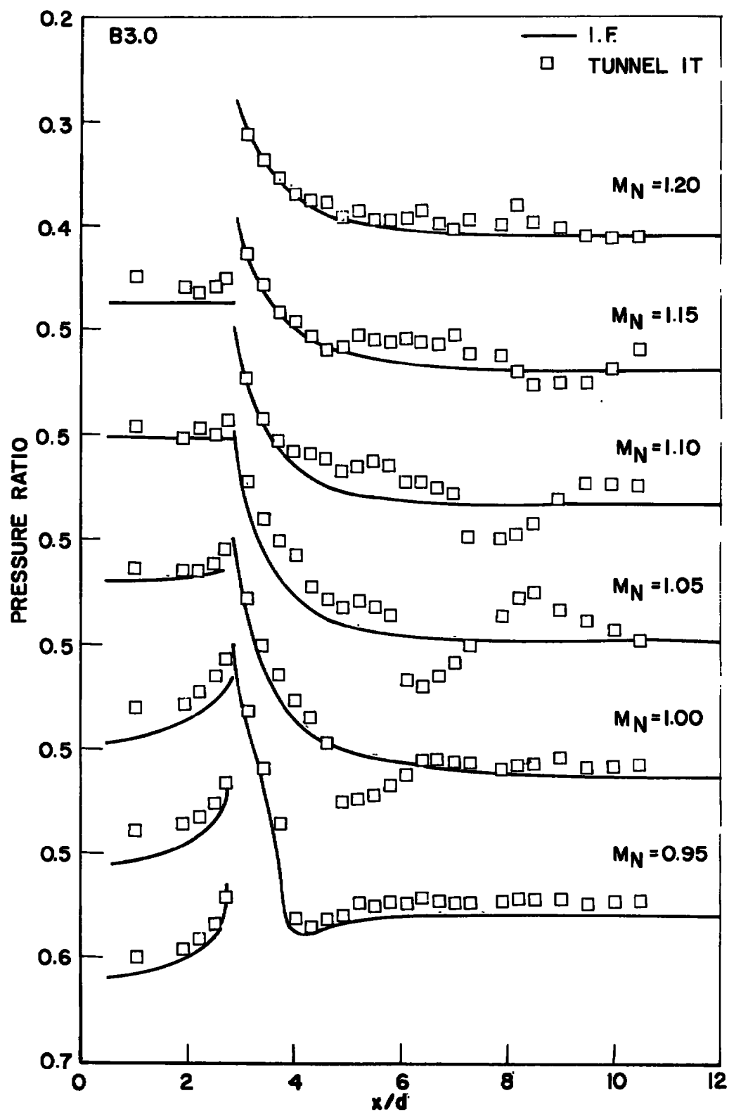
c. r = 3.0 Fig. 12 Continued
