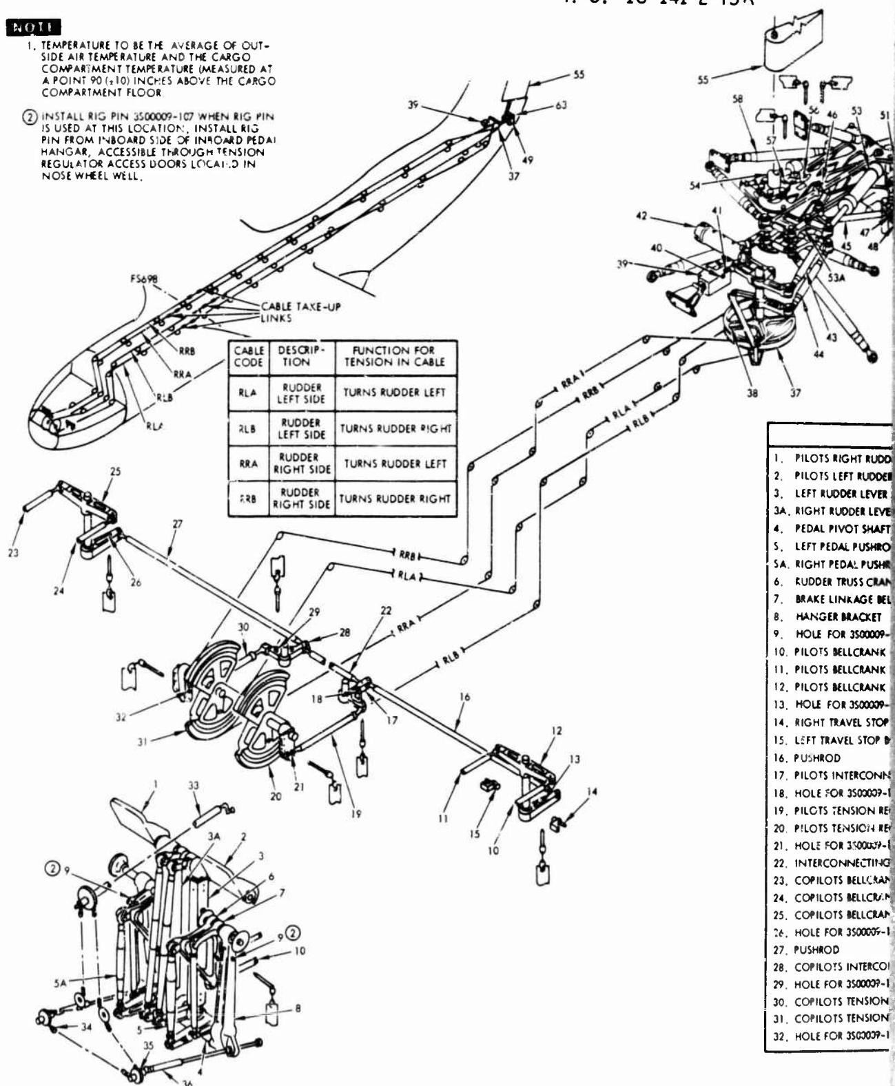
Figure 6. Rudder Control &amp; Trim System Parts Location
