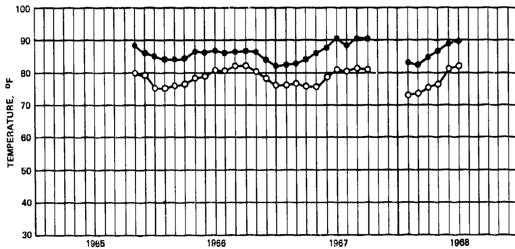
FIG. 4. The Average Maximum and Average Minimum Temperatures of Non-Earth-Covered Magazines at NS, Puerto Rico.
