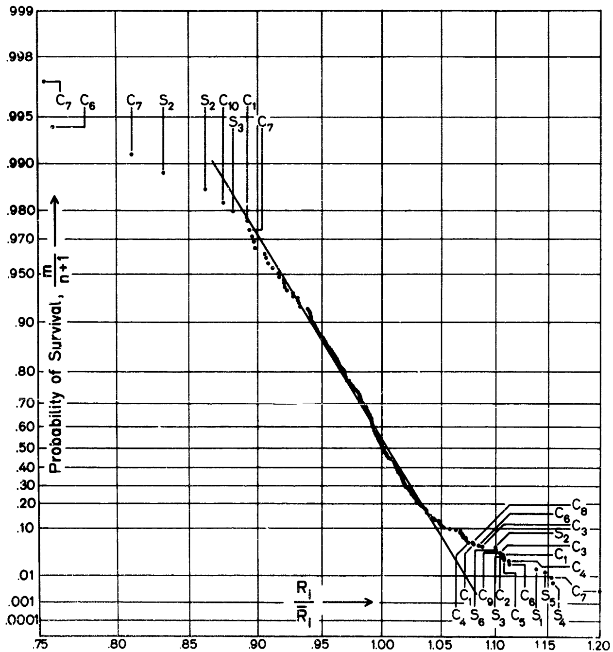
Fig. 2 Probability distribution of structural resistance (341 test data).
