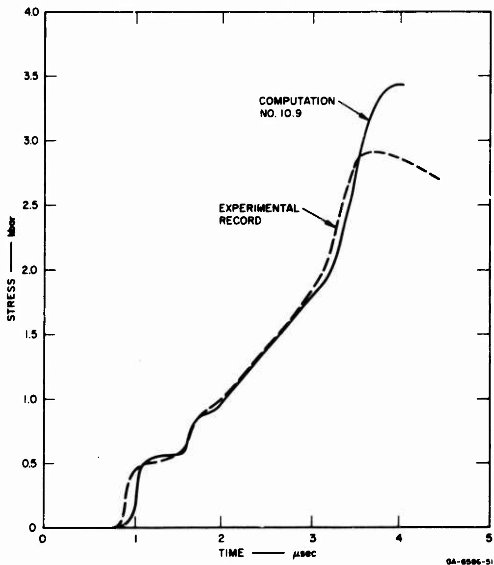
FIG. 23 IRON/POROUS IRON IMPACT, SHOT 13347
