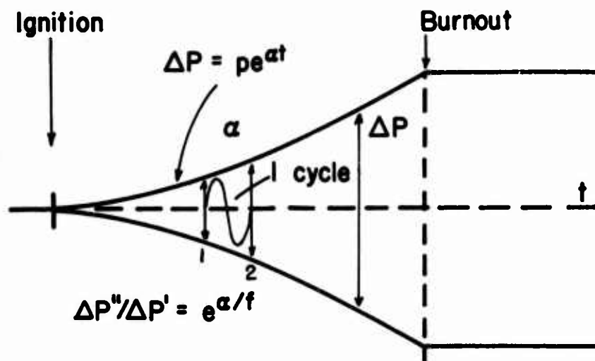
(a) System with no acoustic losses ( \alpha_2 = 0 )
