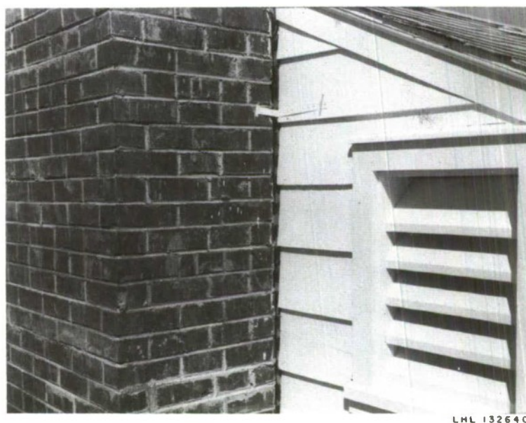
FIG. 17. Views of Chimney Damage, Test No. 2.
