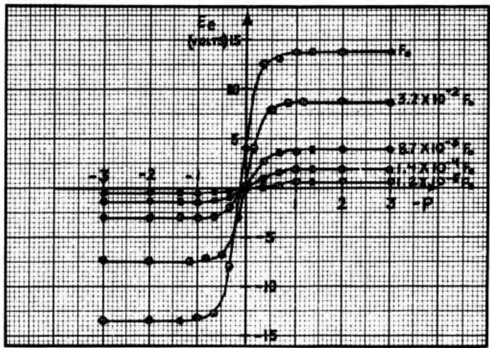
Fig.14. Measured Error Signal Vs. Position Error.80 v. bias.
