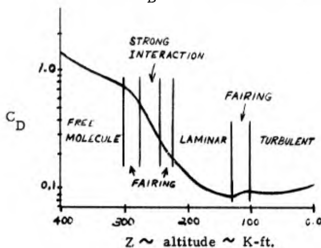
Typical C_D Curve with Flow Regions
