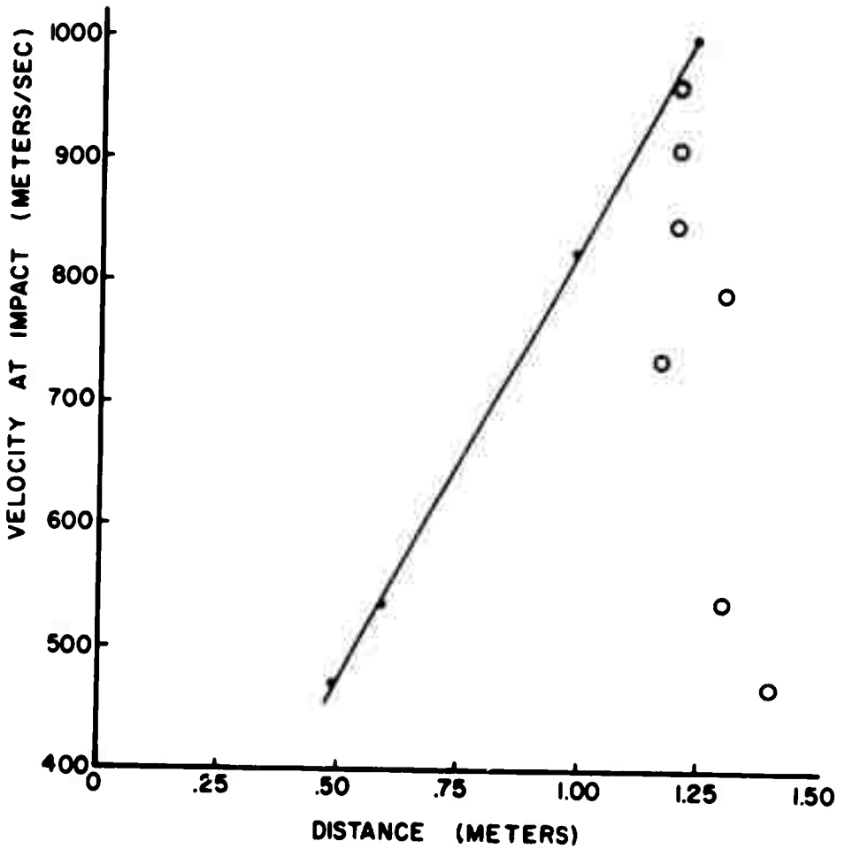
FIGURE A-1. 14.5 MM API, LENGTH OF FLIGHT MAXIMUM YAW AFTER IMPACT vs. IMPACT VELOCITY.
