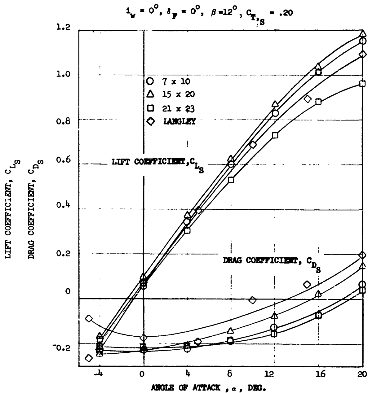
FIGURE 25 COMPARISON OF CRUISE DATA FROM VAD AND LANGLEY
