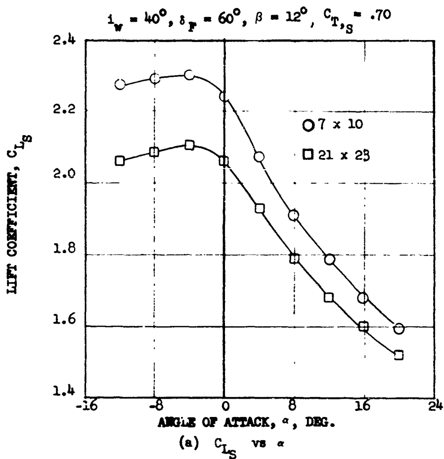
FIGURE 27 COMPARISON OF STOL ( i_w = 40^\circ ) CONFIGURATION DATA FROM VAD TEST SECTIONS
