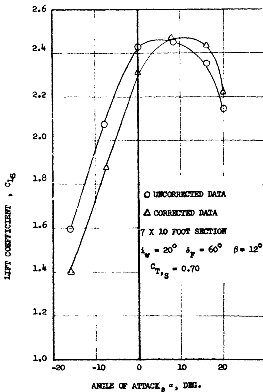
FIGURE 23 EFFECT OF TUNNEL WALL CORRECTIONS FOR ANGLE-OF-ATTACK RUNS
