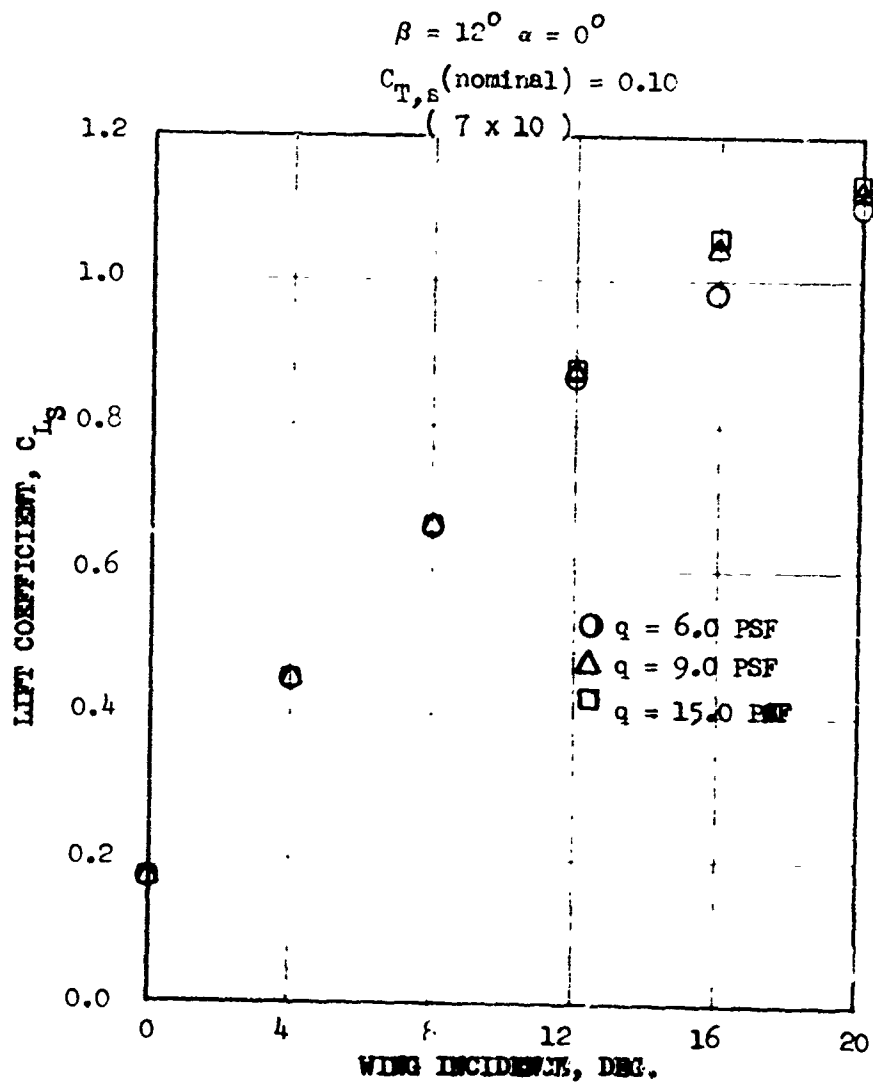
FIGURE 36 EFFECT OF REYNOLDS NUMBER, CRUISE CONFIGURATION
