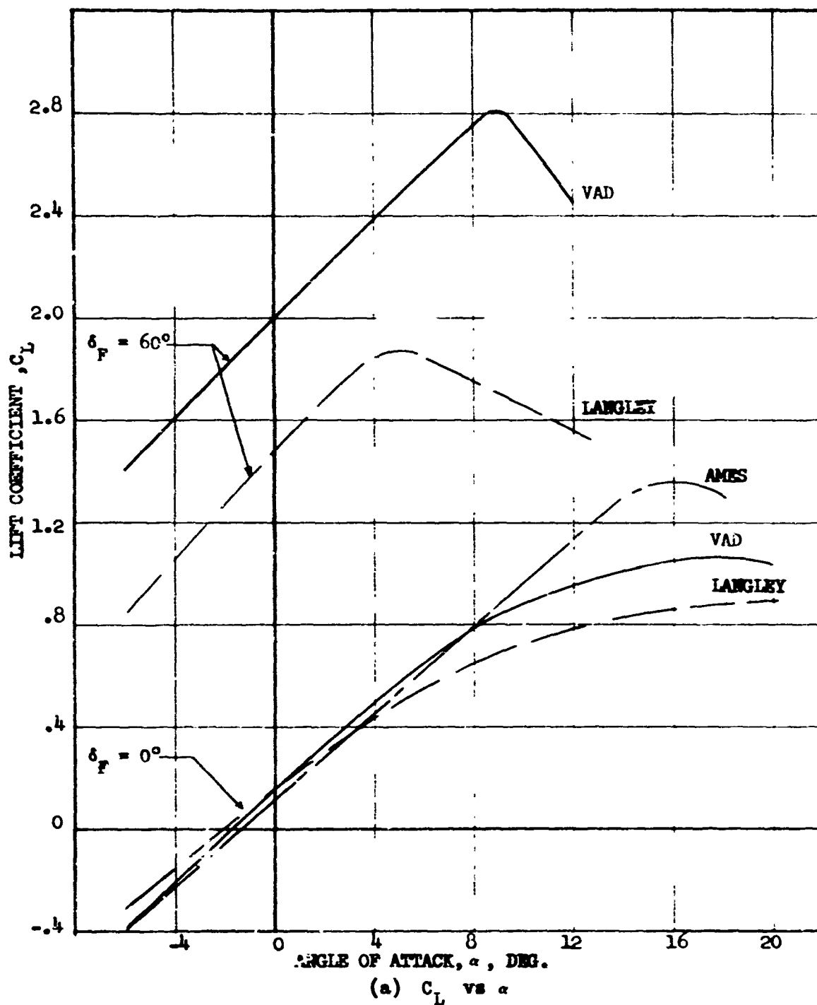
FIGURE 7 COMPARISON OF AMES, LANGLEY, AND VAD DATA (PROPELLERS OFF)
