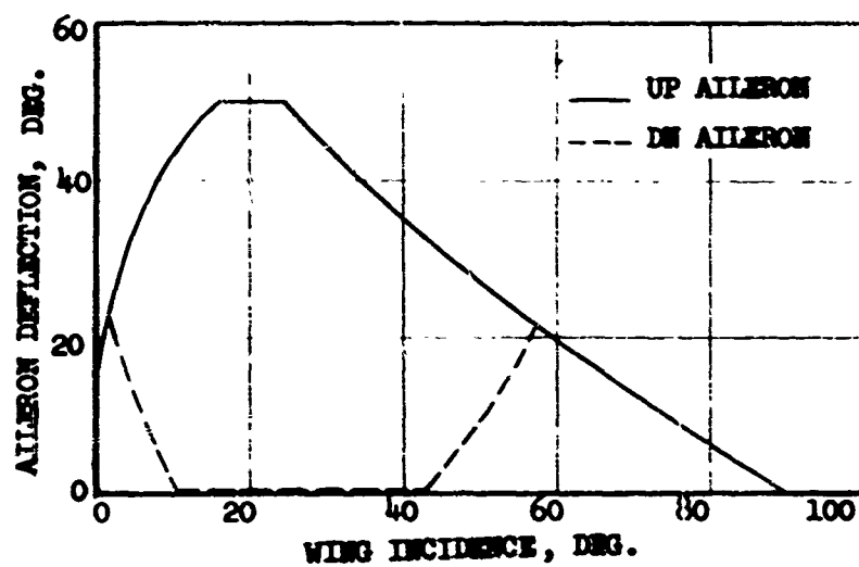
FIGURE 41 LATERAL CONTROL PROGRAMMING
