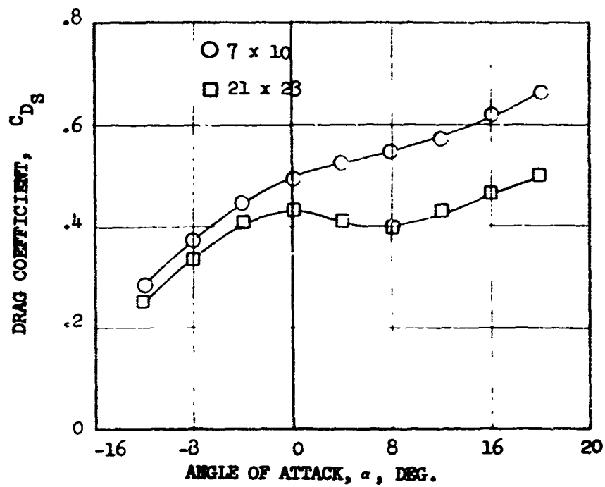
(b) C_{D_S} vs \alpha
