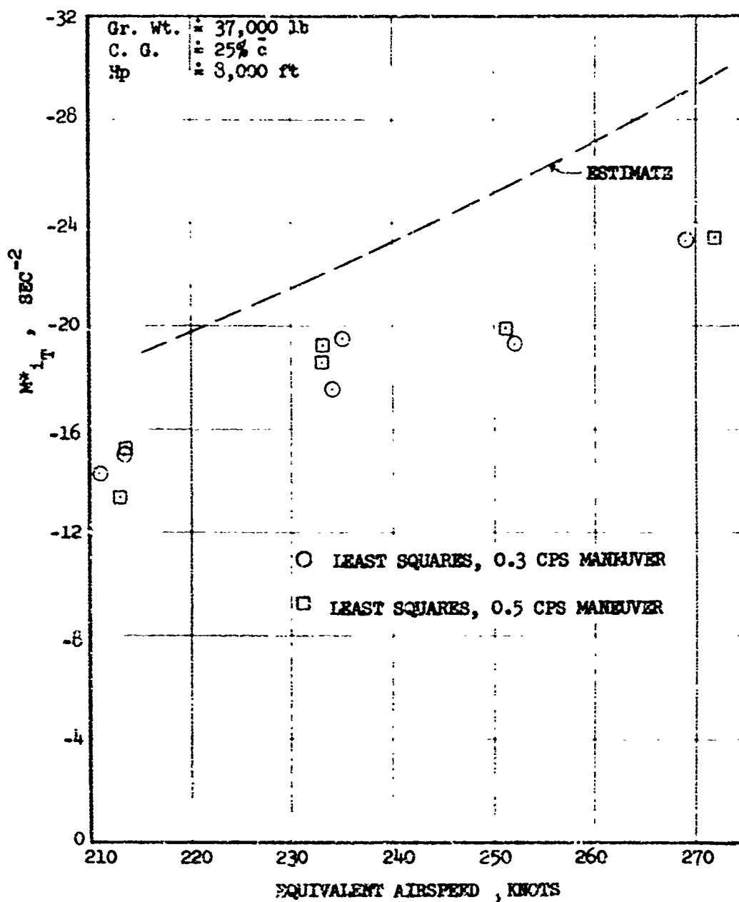
FIGURE 57 LONGITUDINAL CONTROL EFFECTIVENESS, M^*_{i_T} (25% C.G.)
