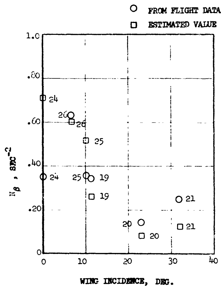
(b) N_\beta VS. WING INCIDENCE
