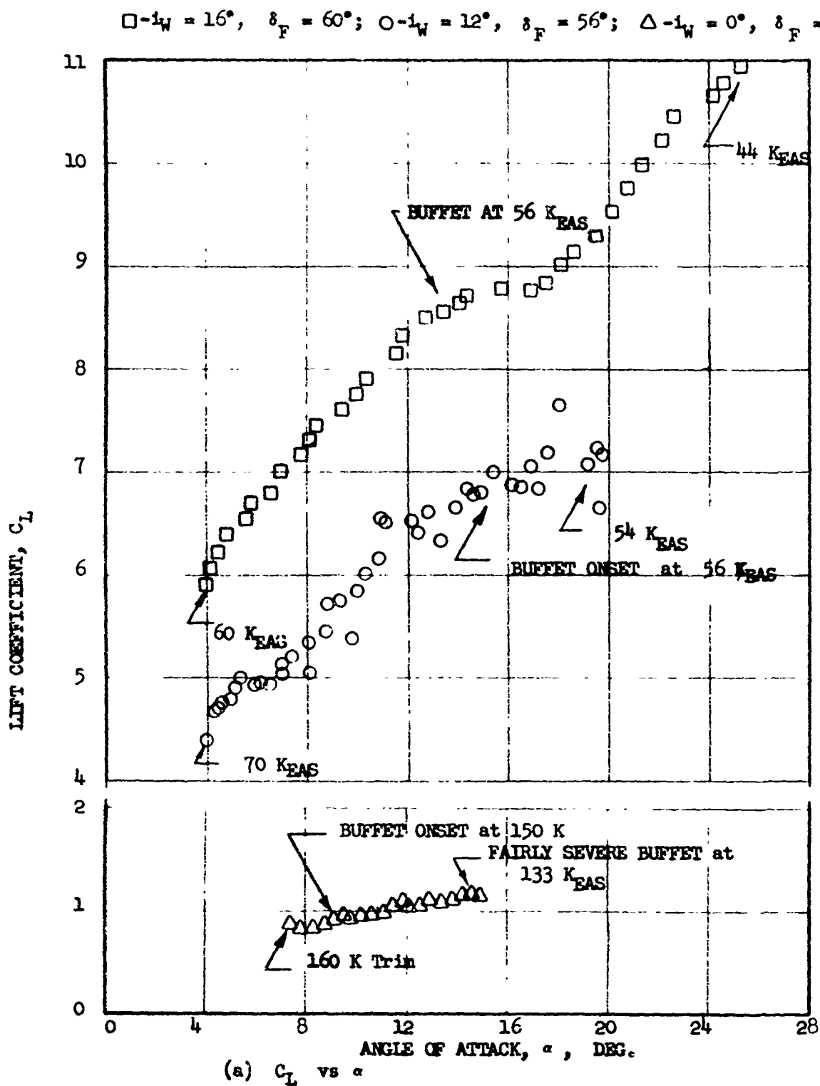
FIGURE 53 VARIATION OF AIRPLANE LIFT COEFFICIENT WITH ANGLE-OF-ATTACK
