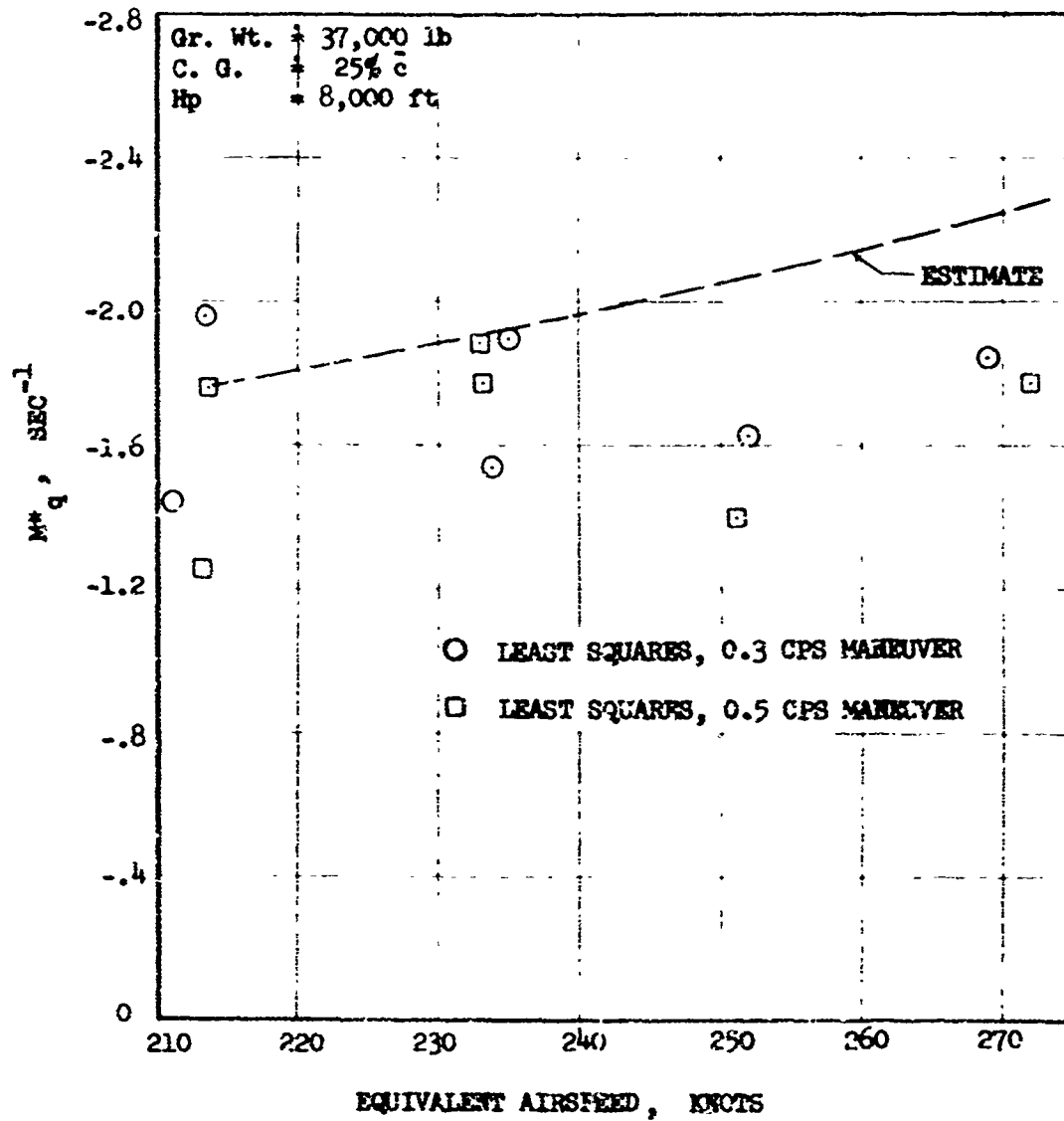
FIGURE 59 LONGITUDINAL DAMPING PARAMETER, M^*_q (25% C.G.)
