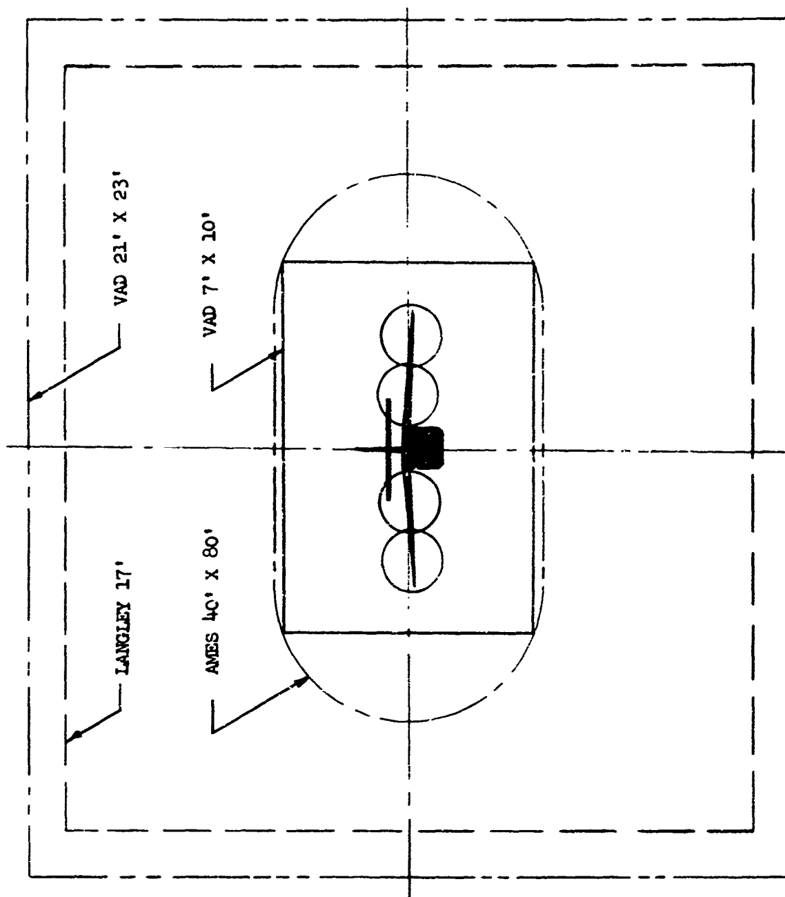
FIGURE 19 MODEL SIZE RELATIVE TO TEST SECTION SIZE
