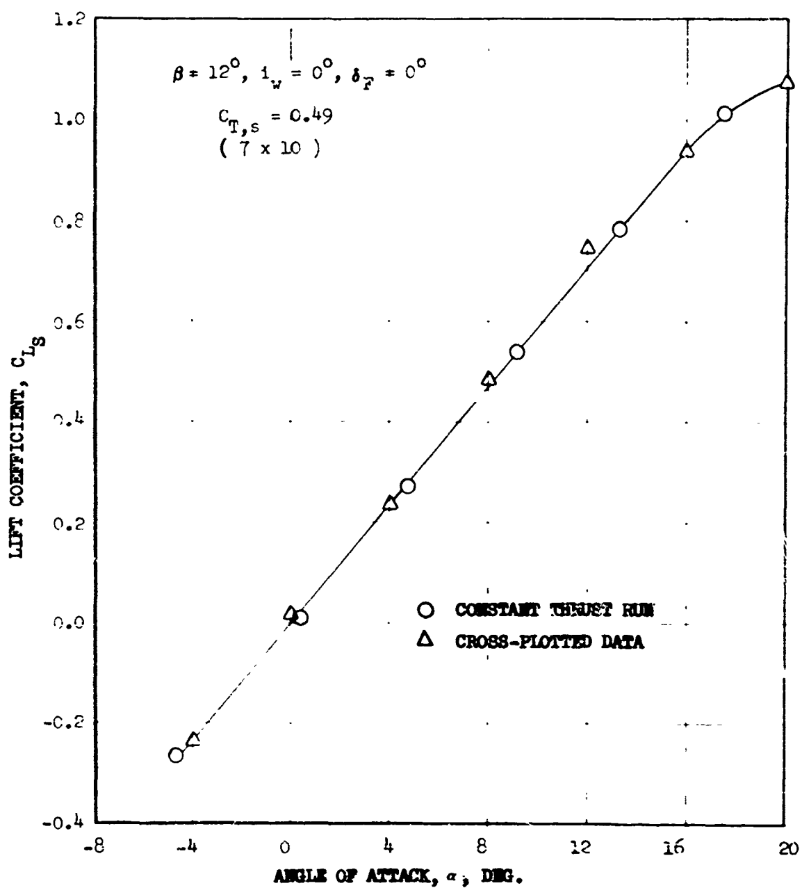
FIGURE 32 COMPARISON OF CONSTANT THRUST DATA OBTAINED BY DIFFERENT METHODS
