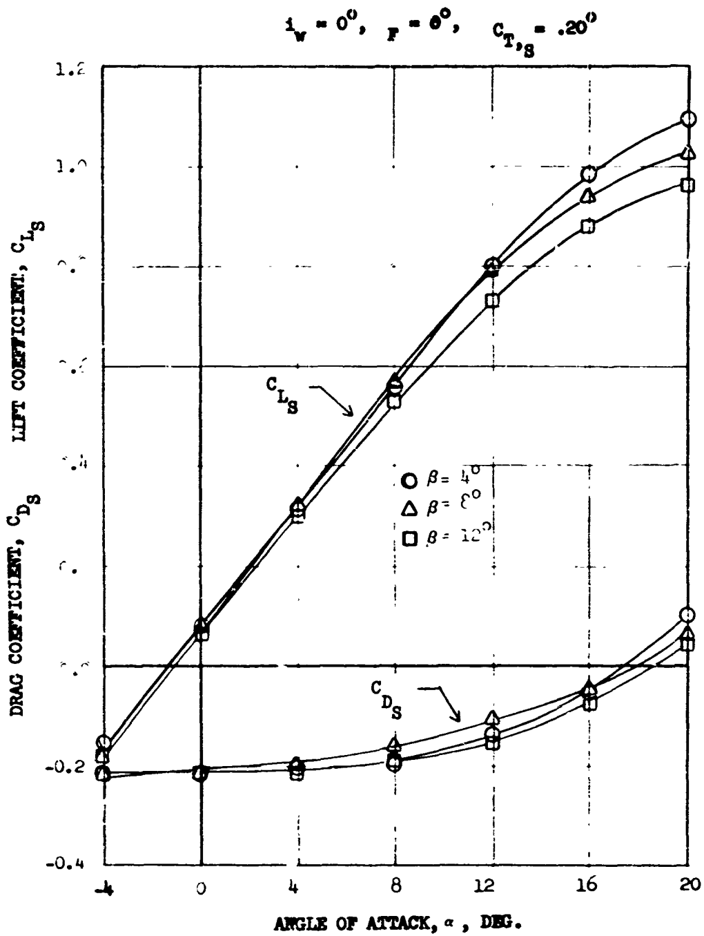
FIGURE 31 EFFECT OF PROPELLER BLADE PITCH ANGLE
