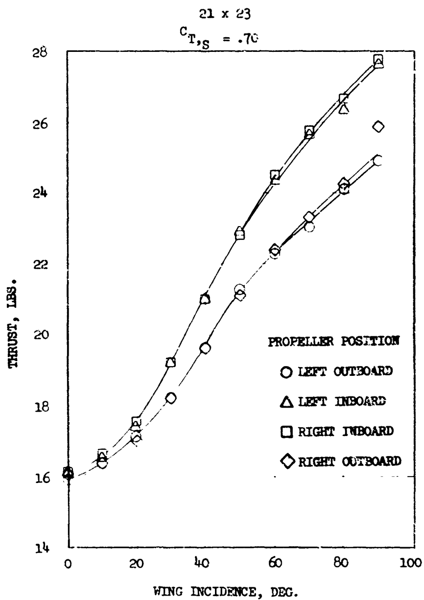
FIGURE 29 COMPARISON OF INBOARD AND OUTBOARD PROPELLER THRUST VARIATION
