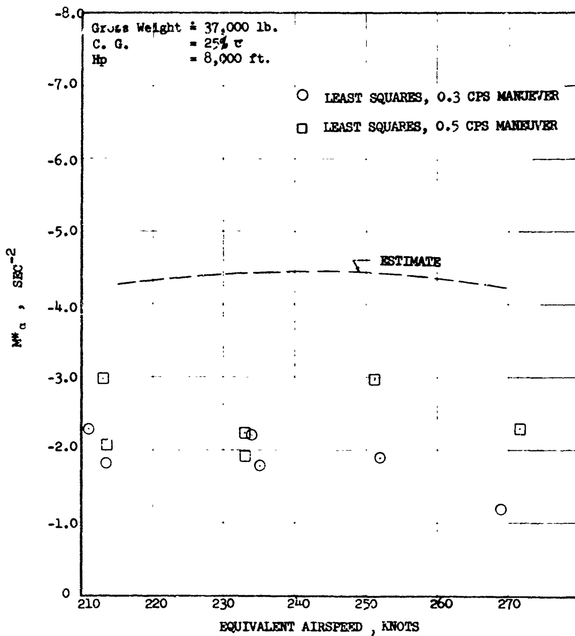
FIGURE 55 LONGITUDINAL STABILITY PARAMETER, M^*_\alpha (25% C.G.)
