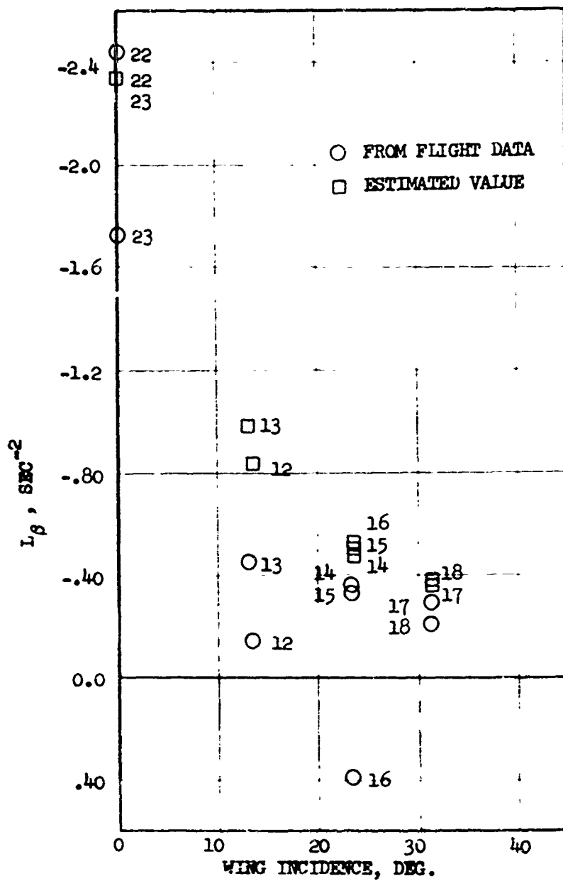
(b) L_{\beta} VS. WING INCIDENCE FIGURE 50 (CONCLUDED)
