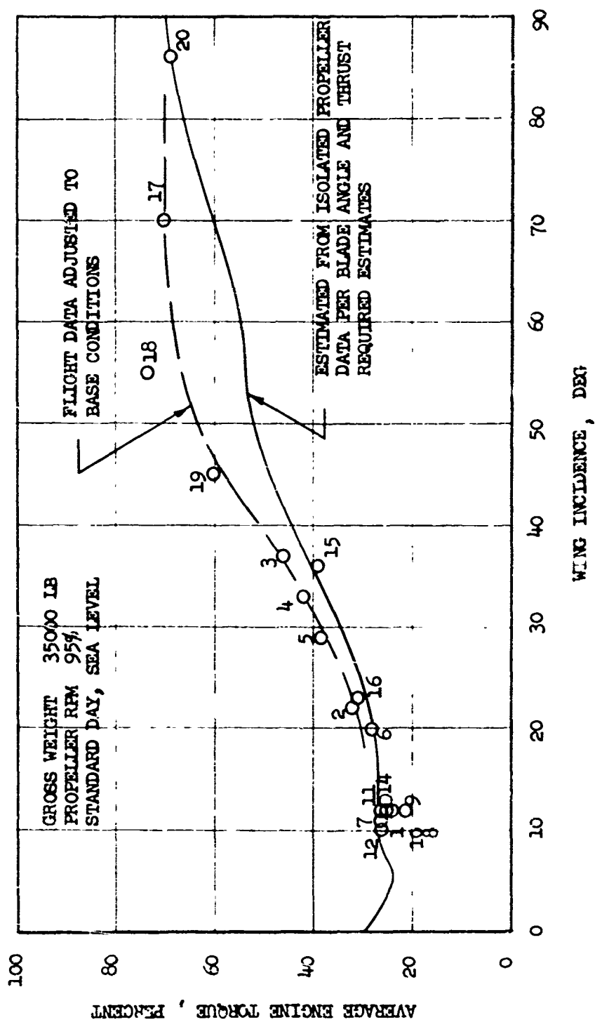
FIGURE 65 COMPARISON OF ESTIMATED AND MEASURED TORQUE REQUIRED IN TRANSITION
