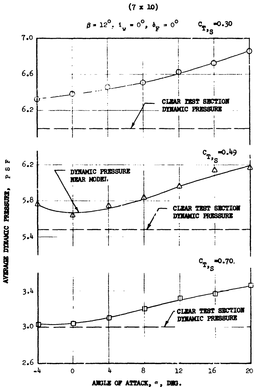
FIGURE 35 COMPARISON OF DYNAMIC PRESSURE DETERMINED BY TWO METHODS
