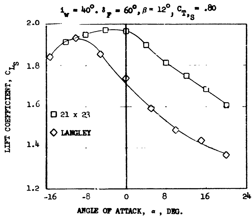
FIGURE 28 COMPARISON OF STOL ( i_w = 40^\circ ) CONFIGURATION DATA FROM VAD AND LANGLEY
