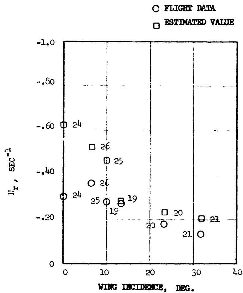
(b) N_r VS. WING INCIDENCE
