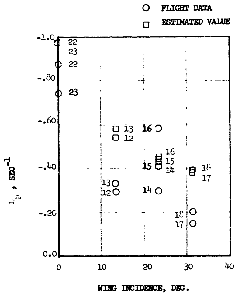
(b) L_p VS. WING INCIDENCE
