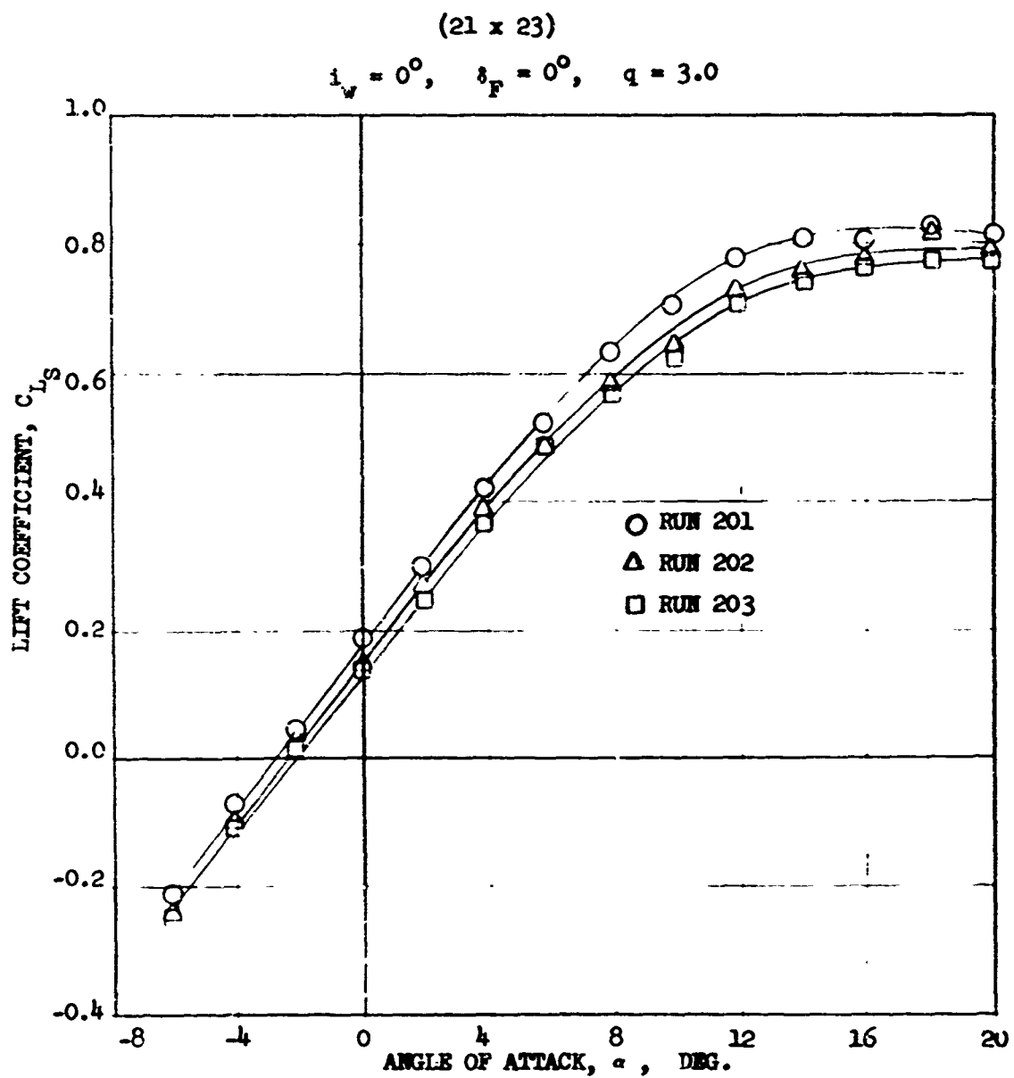
FIGURE 39 EFFECT OF TUFTS, CRUISE CONFIGURATION
