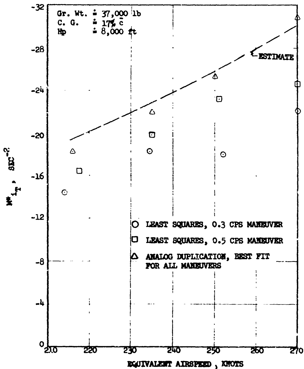
FIGURE 56 LONGITUDINAL CONTROL EFFECTIVENESS, M^* i_T (17% C.G.)
