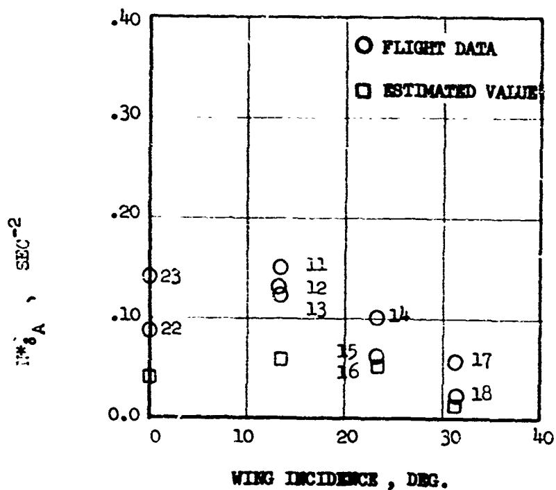
FIGURE 45 YAW DUE TO ROLL CONTROL, N^*_{\delta A}
