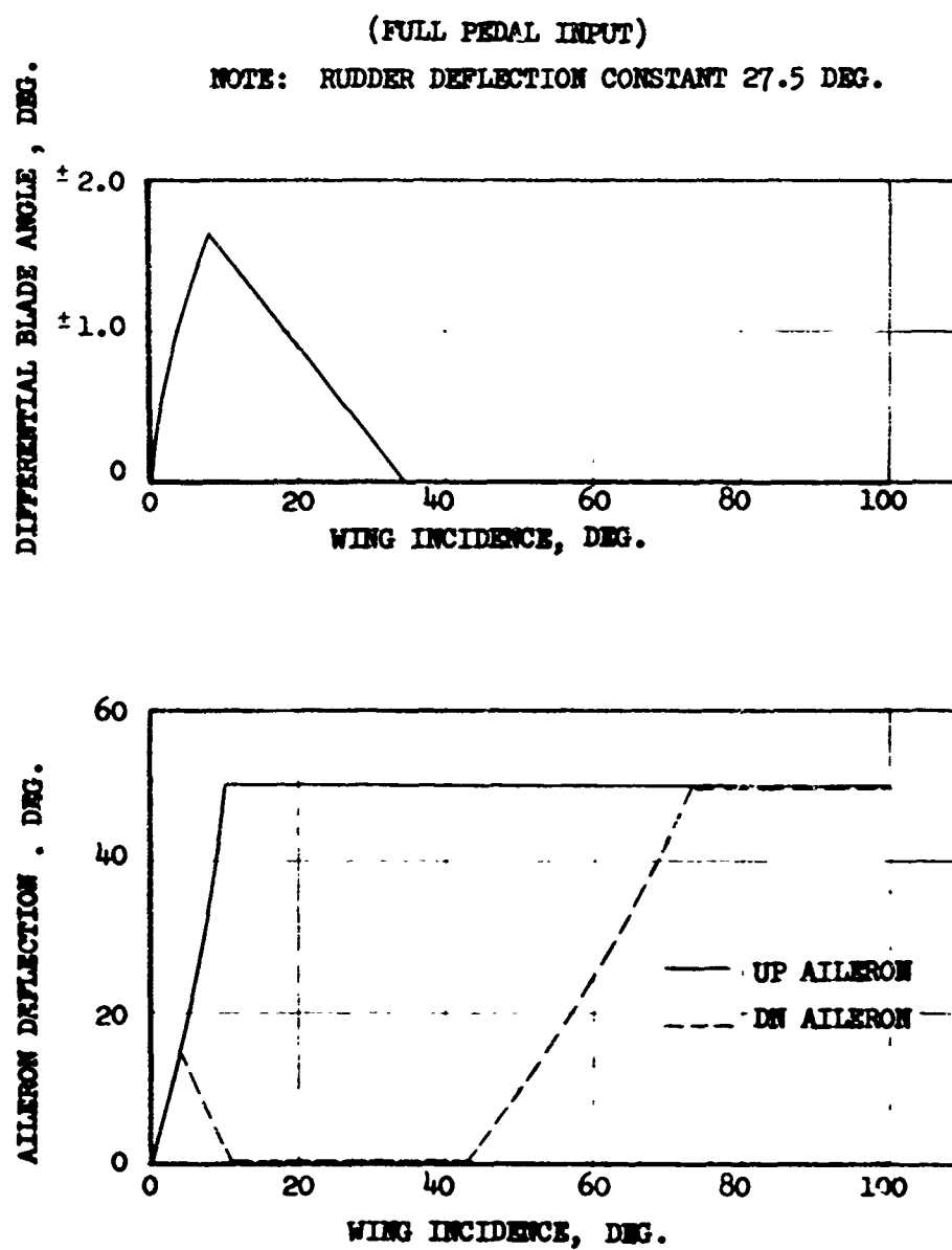
FIGURE 46 DIRECTIONAL CONTROL PROGRAMMING
