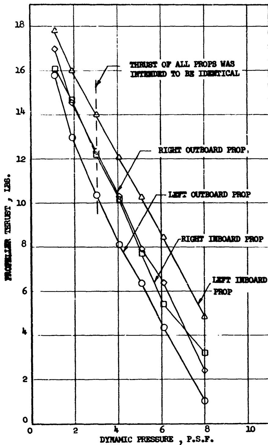
FIGURE 16 LANGLEY PROPELLER THRUST VARIATION
