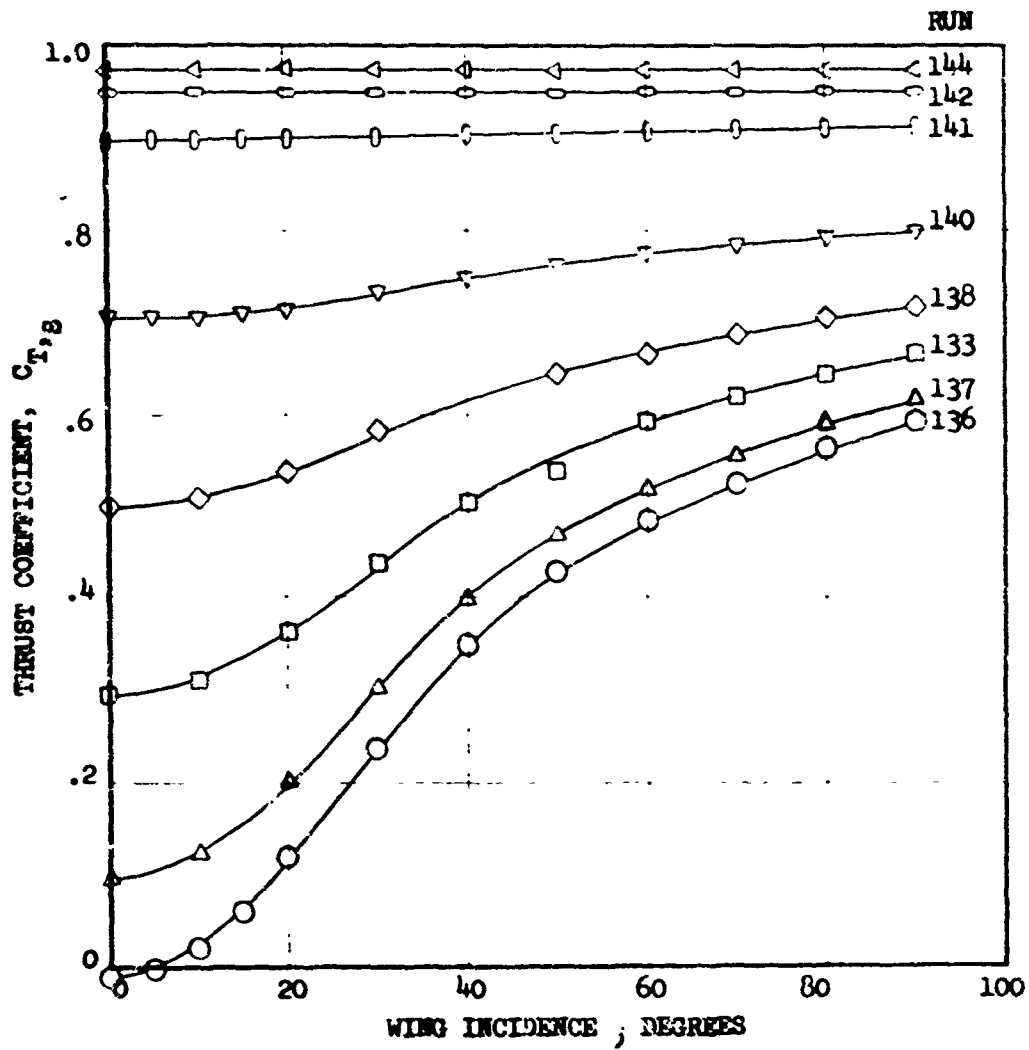
FIGURE 30 EFFECT OF WING INCIDENCE ON THRUST COEFFICIENT
