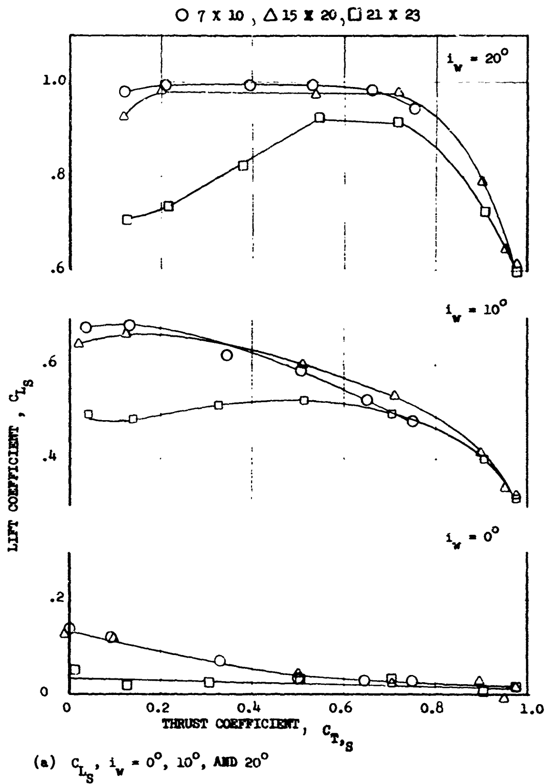
FIGURE 21 COMPARISON OF DATA FROM THREE DIFFERENT SIZE TEST SECTIONS, CORRECTED FOR WALL EFFECTS
