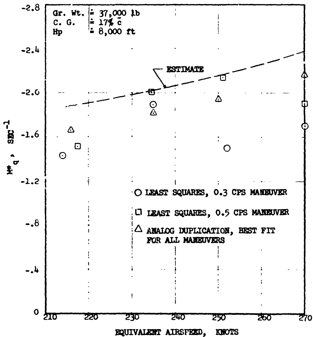
FIGURE 58 LONGITUDINAL DAMPING PARAMETER, M^*_q (17% C.G.)
