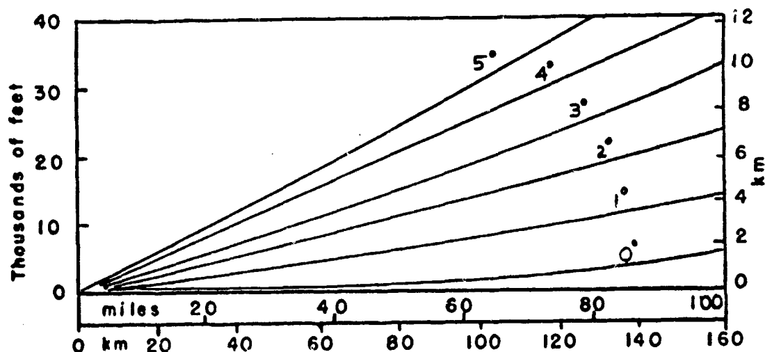
Fig. 23. Height of beam center above earth as a function of slant range and elevation angle.
