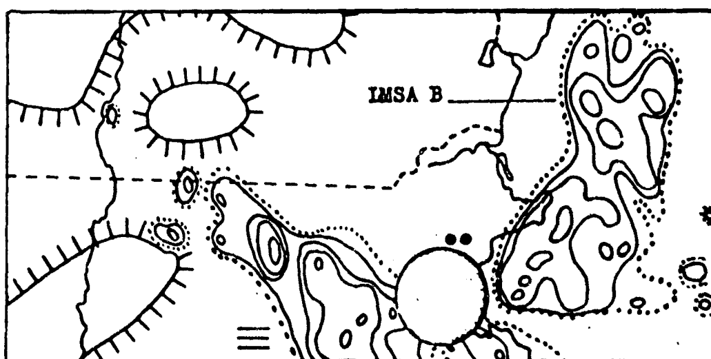
Fig. 45. Precipitation pattern for 0635 EST, 8 July 1963, with blob-shaped large mesoscale area. Contours: 0( \equiv ), 1( \cdots ), 2, 4, 8 and 16 mm hr -1 .
