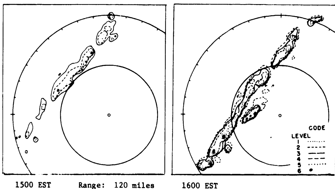
Fig. 49. Maps of range-normalized signal intensity on the SCR-615-B radar showing storm development in the squall line of 19 August 1965.
