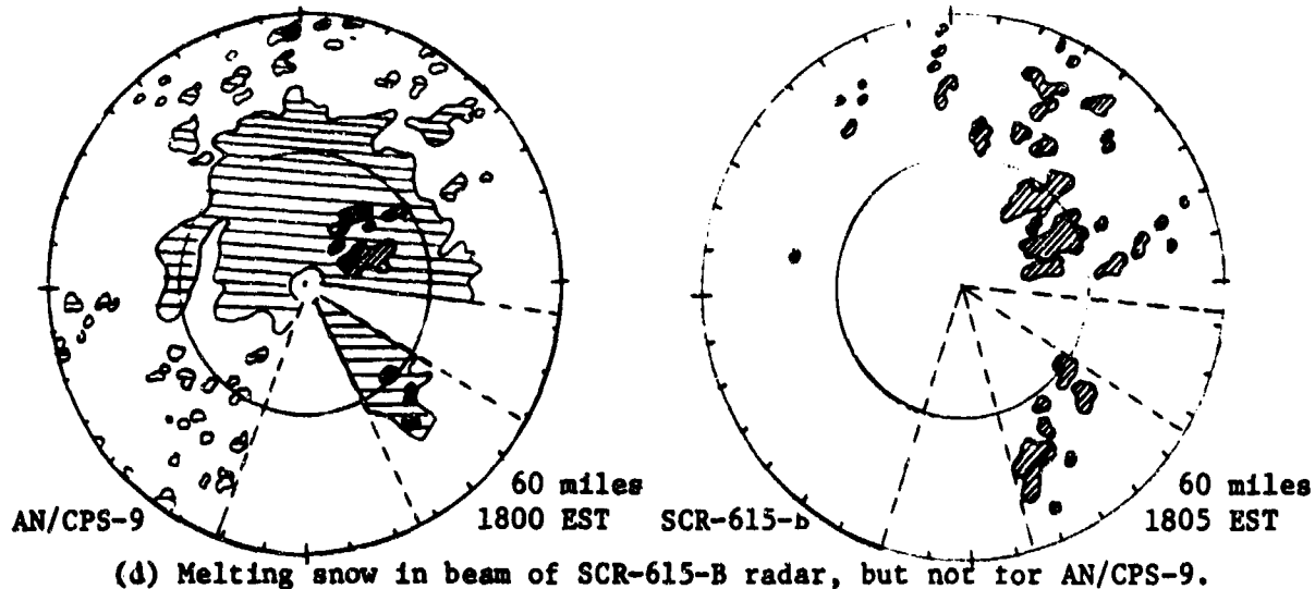
Fig. 24. Examples illustrating effects of changes in hydrometeors in low levels of the atmosphere.
