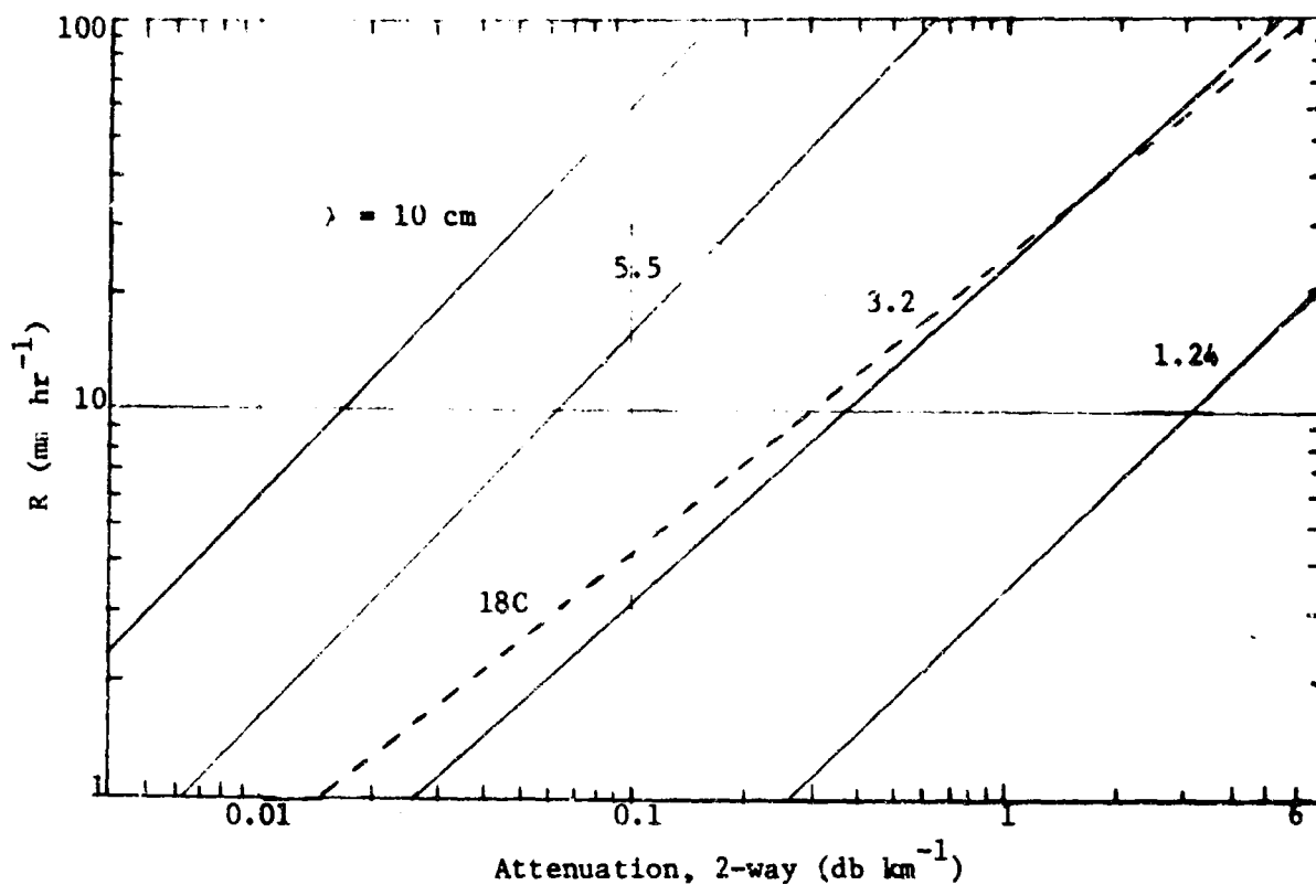
Fig. 25. Empirical values of two-way attenuation as a function of rainfall rate for radiation of various wave lengths. All except the dashed curve are for a temperature of 0C. (From summary in Atlas, 1964).
