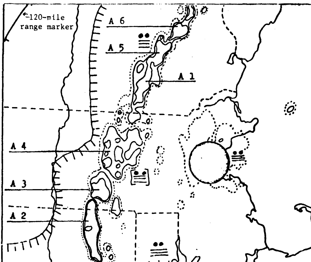
Fig. 44. Precipitation pattern for 0440 EST, 29 August 1962, containing band-shaped large mesoscale area. Contours: 0( \equiv ), 2( \cdots ), 6, 12 and 24 mm hr -1 . Circle represents radar site and ground clutter.
