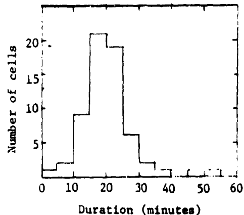
Fig. 56. Distribution of durations of cells in thunderstorm complexes.
