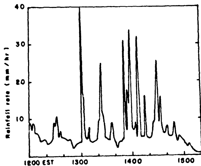
Fig. 42. Detailed rain-gauge record, 7 November 1963.
