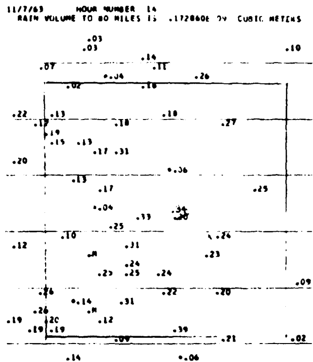
Fig. 41. Computer-plotted hourly rainfall amounts in inches. Added square is 4 \times 10^4 km 2 . x marks radar site.
