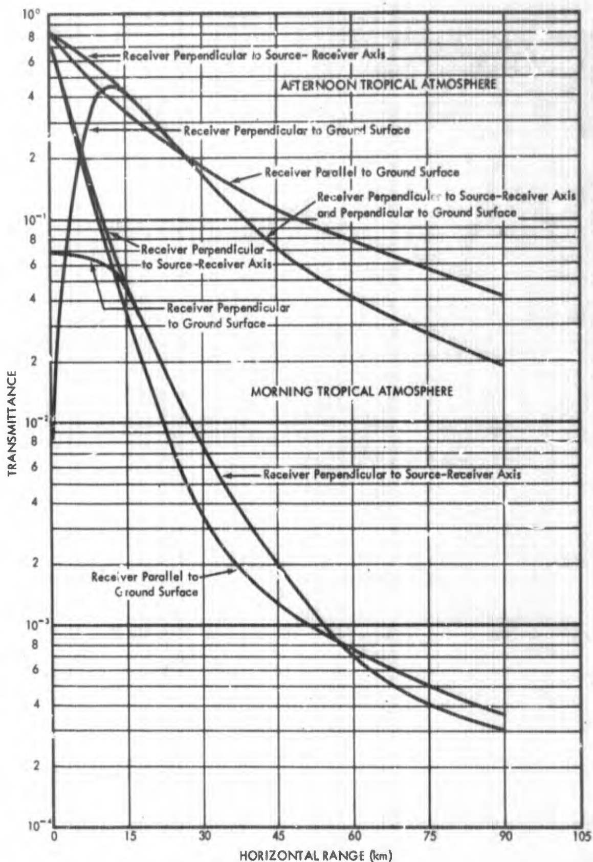
Fig. 10. Comparison of the Transmittances for Receivers Oriented Perpendicular to the Source-Receiver Axis, Parallel to the Ground Surface, and Perpendicular to the Ground Surface for a Nuclear Weapon Burst at 1 km Altitude in the Morning and Afternoon Tropical Atmospheres: Ground Albedo = 0.0
