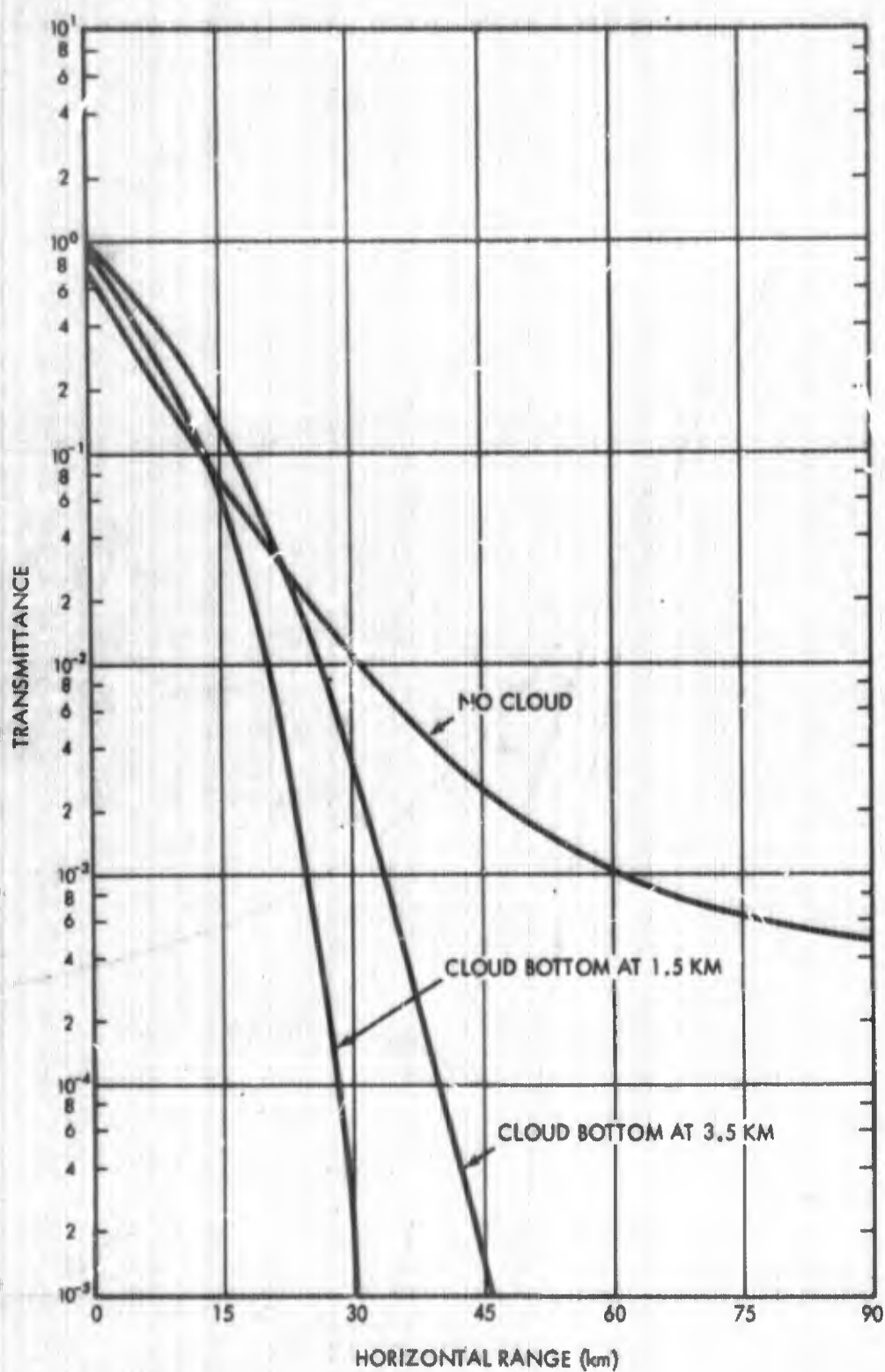
Fig. 17. Variation of the Transmittance for a Nuclear Weapon Burst at 1 km Altitude in the Morning Tropical Atmosphere with Horizontal Range for Cloud Bottom Altitudes of 1.5 and 3.5 km: Receiver Normal to Source-Receiver Axis, Ground Albedo = 0.9
