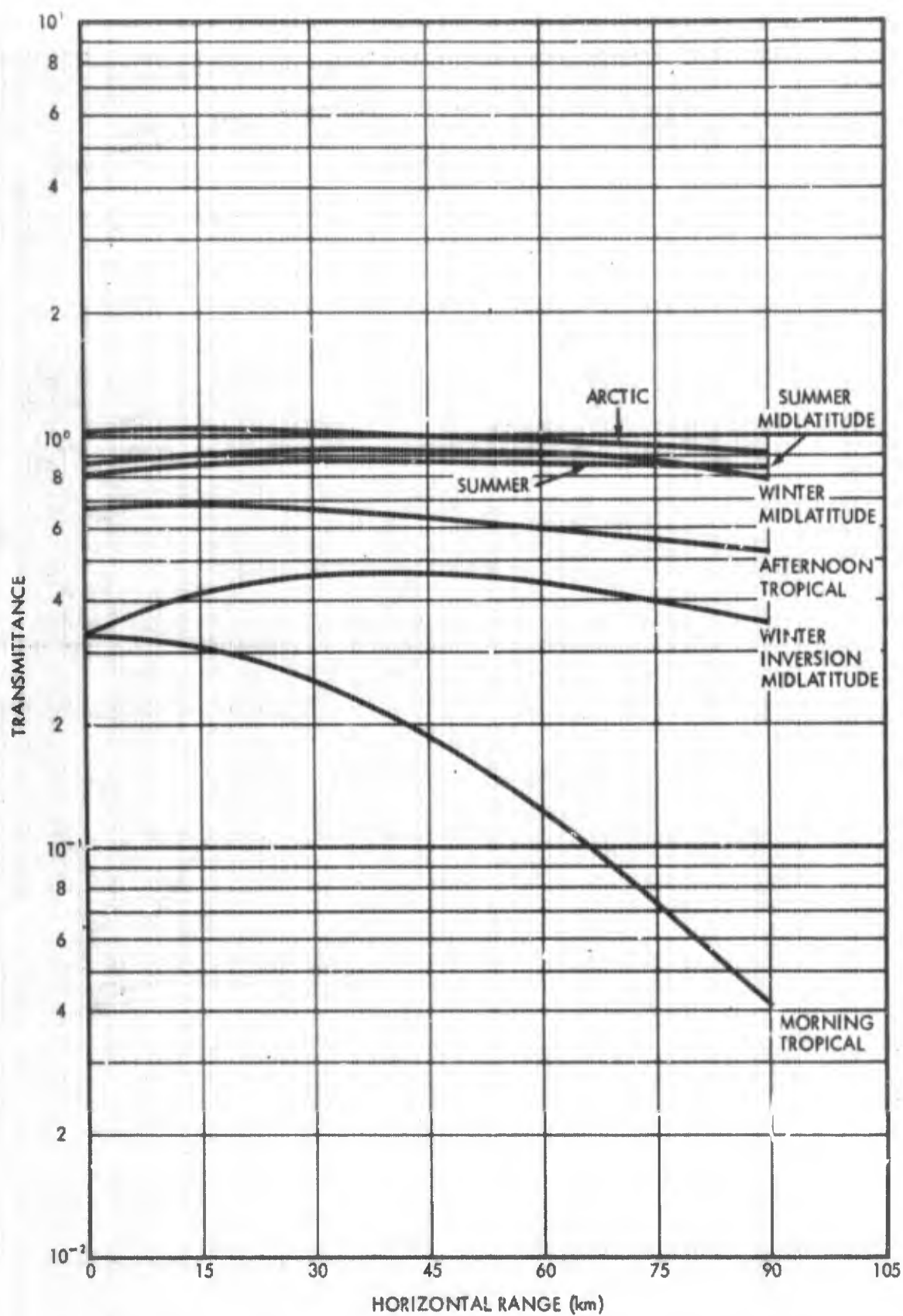
Fig. 9. Transmittance for Representative Air Burst in Model Atmospheres: Burst Altitude = 50 km, Albedo = 0.9, Receiver Normal to Source-Receiver Axis
