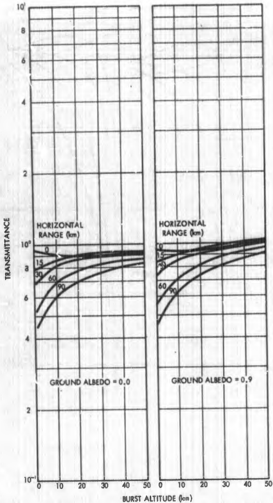
Fig. 25. Variation of the Transmittance for a Nuclear Weapon Burst in the Arctic Atmosphere with Burst Altitude: Receiver Parallel to Source-Receiver Axis
