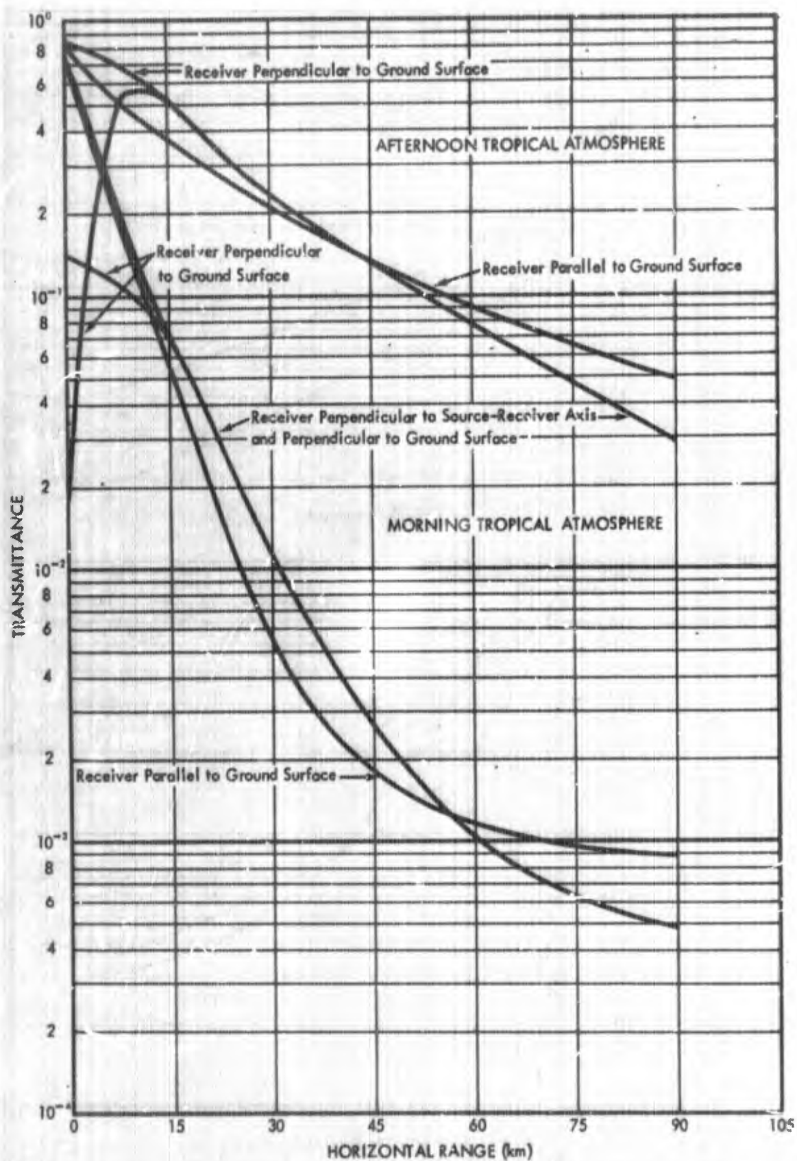
Fig. 11. Comparison of the Transmittances for Receivers Oriented Perpendicular to the Source-Receiver Axis, Parallel to the Ground Surface, and Perpendicular to the Ground Surface for a Nuclear Weapon Burst at 1 km Altitude in the Morning and Afternoon Tropical Atmospheres: Ground Albedo = 0.9
