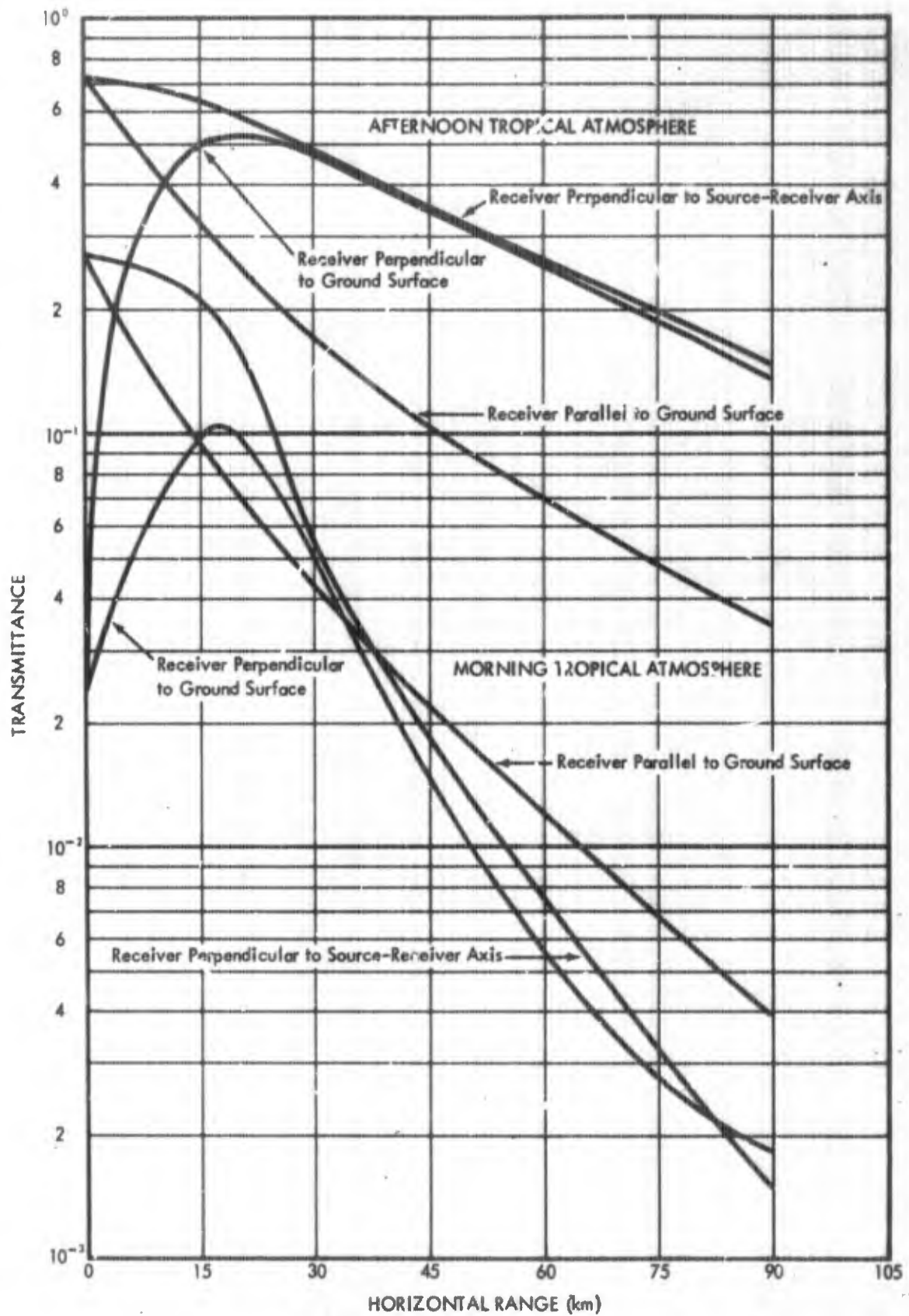
Fig. 12. Comparison of the Transmittances for Receivers Oriented Perpendicular to the Source-Receiver Axis, Parallel to the Ground Surface, and Perpendicular to the Ground Surface for a Nuclear Weapon Burst at 9 km Altitude in the Morning and Afternoon Tropical Atmospheres: Ground Albedo = 0.0
