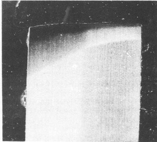
Heat-Affected Zone on Mill Cut Edge 7.5X
