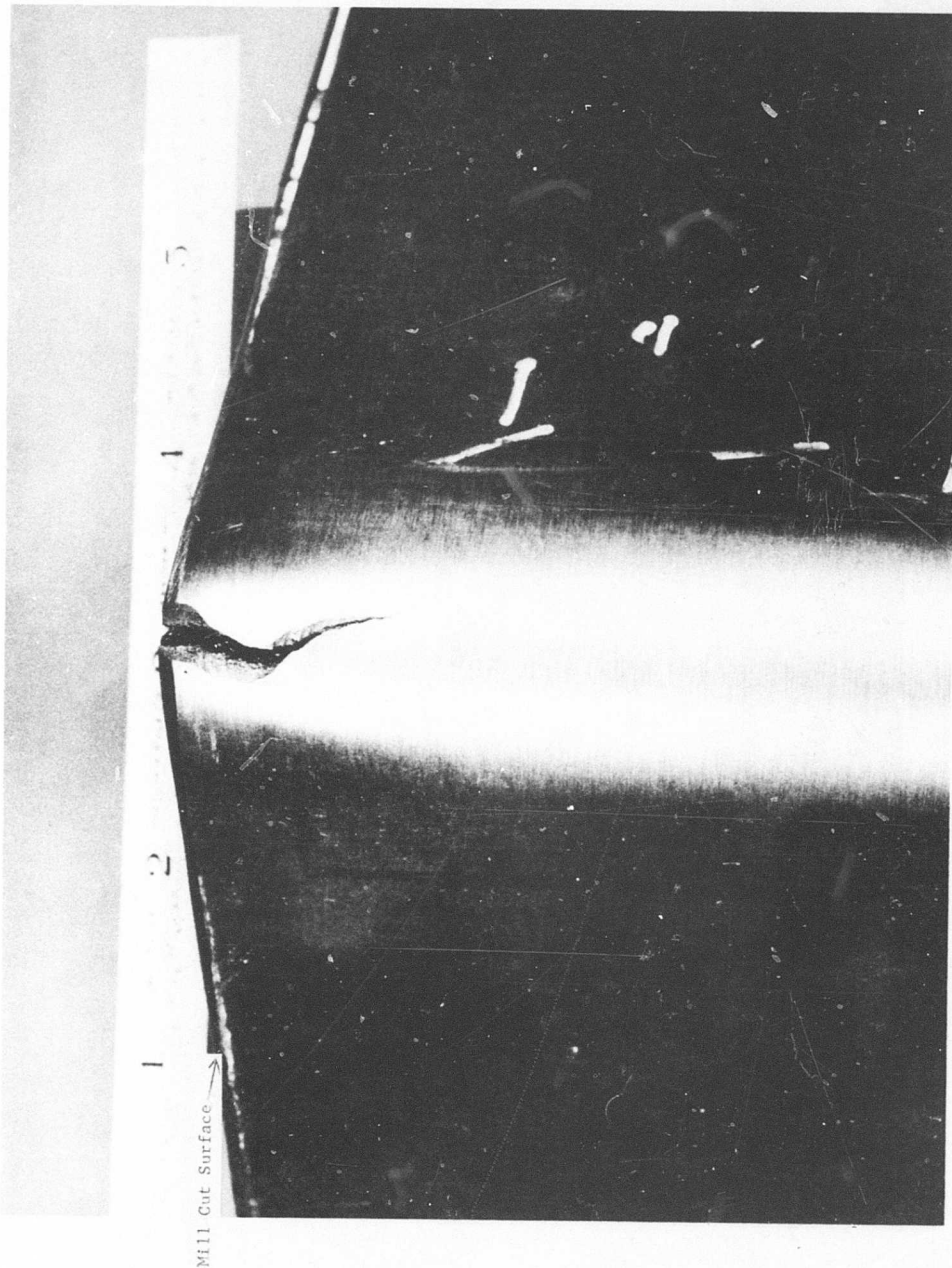
Figure 2. Crack Starting at Mill Cut Edge (Specimen I-1).
