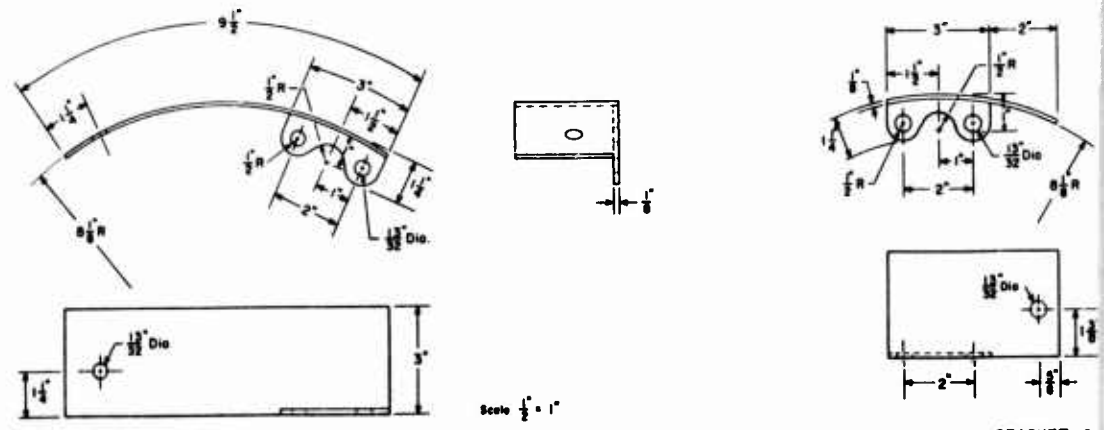
BRACKET 4
