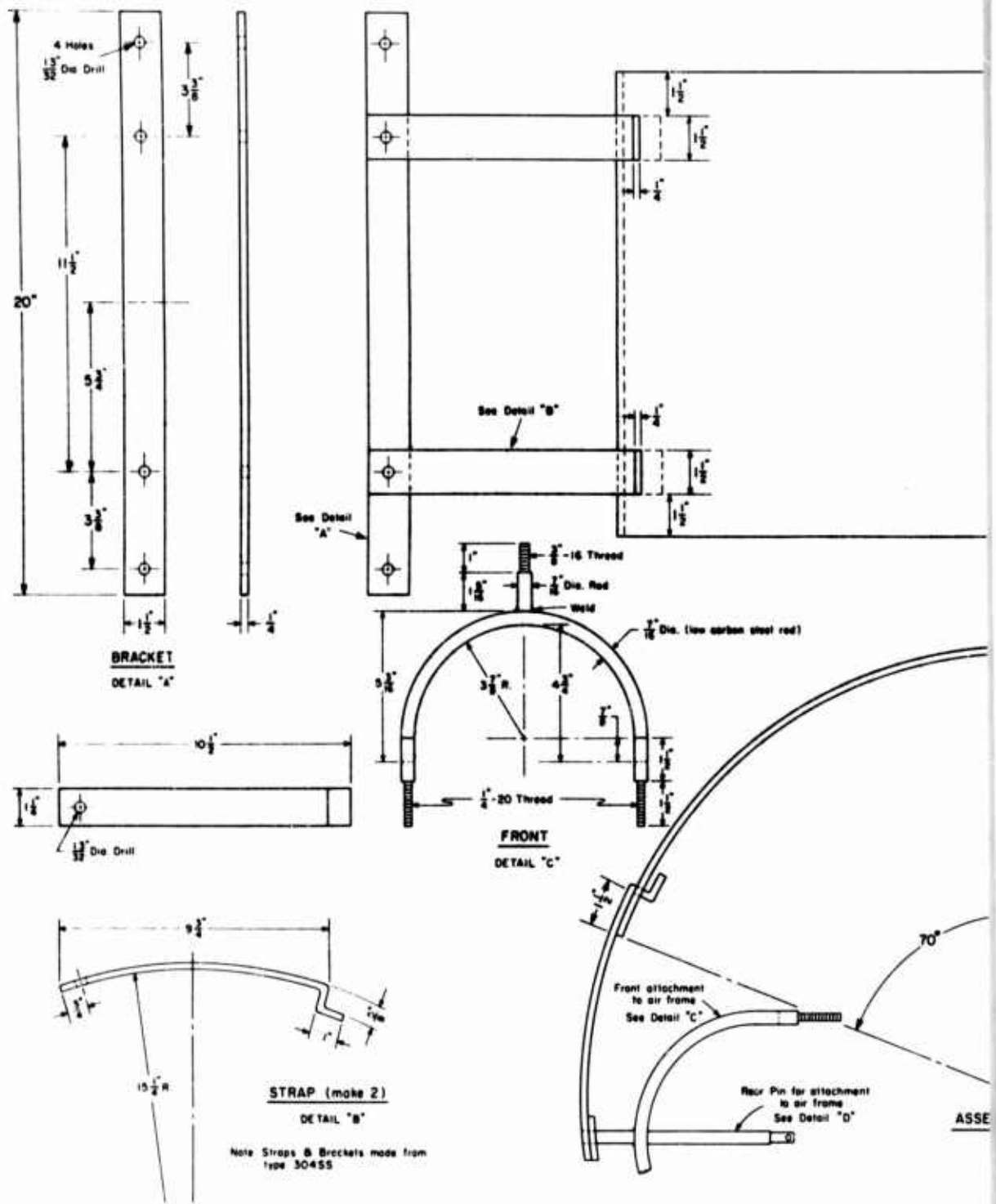
Figure 23. Dual-Hardness Armor - Compressor Cover, Left Side.
