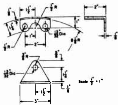
BRACKETS 2 & 3
