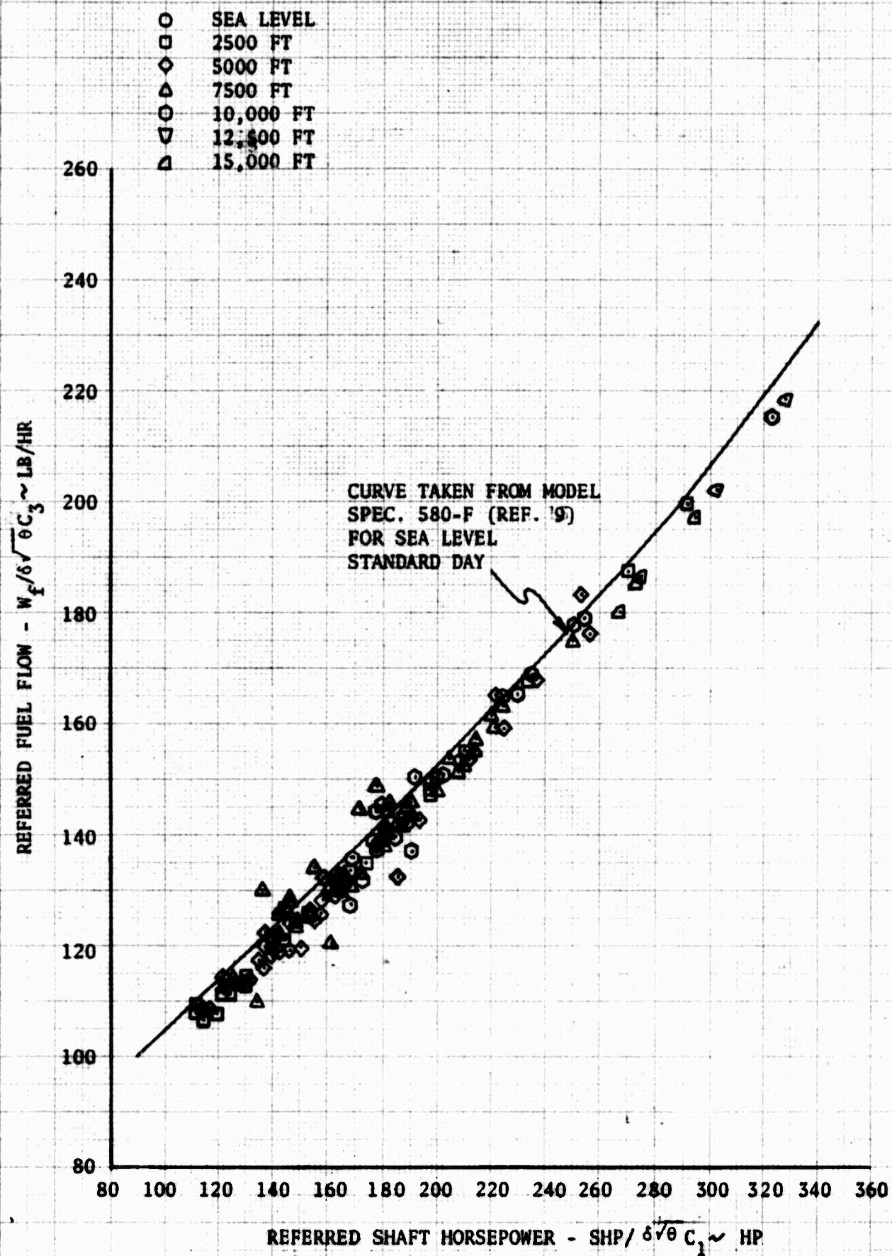
FIGURE NO. 64 ENGINE CHARACTERISTICS T63-A-5A
