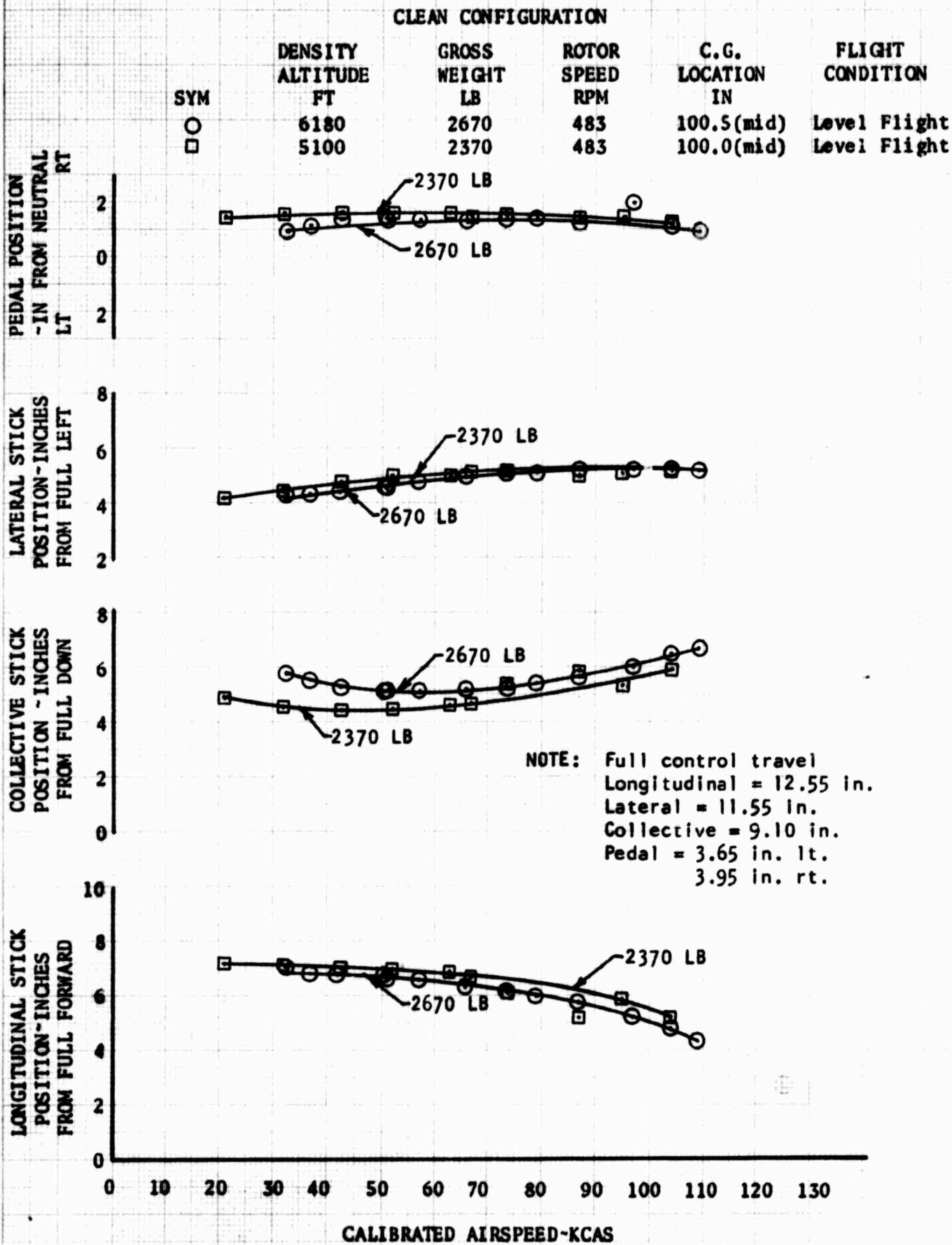
FIGURE NO. 69 CONTROL POSITION TRIM CURVES OH-6A S/N 65-12919
