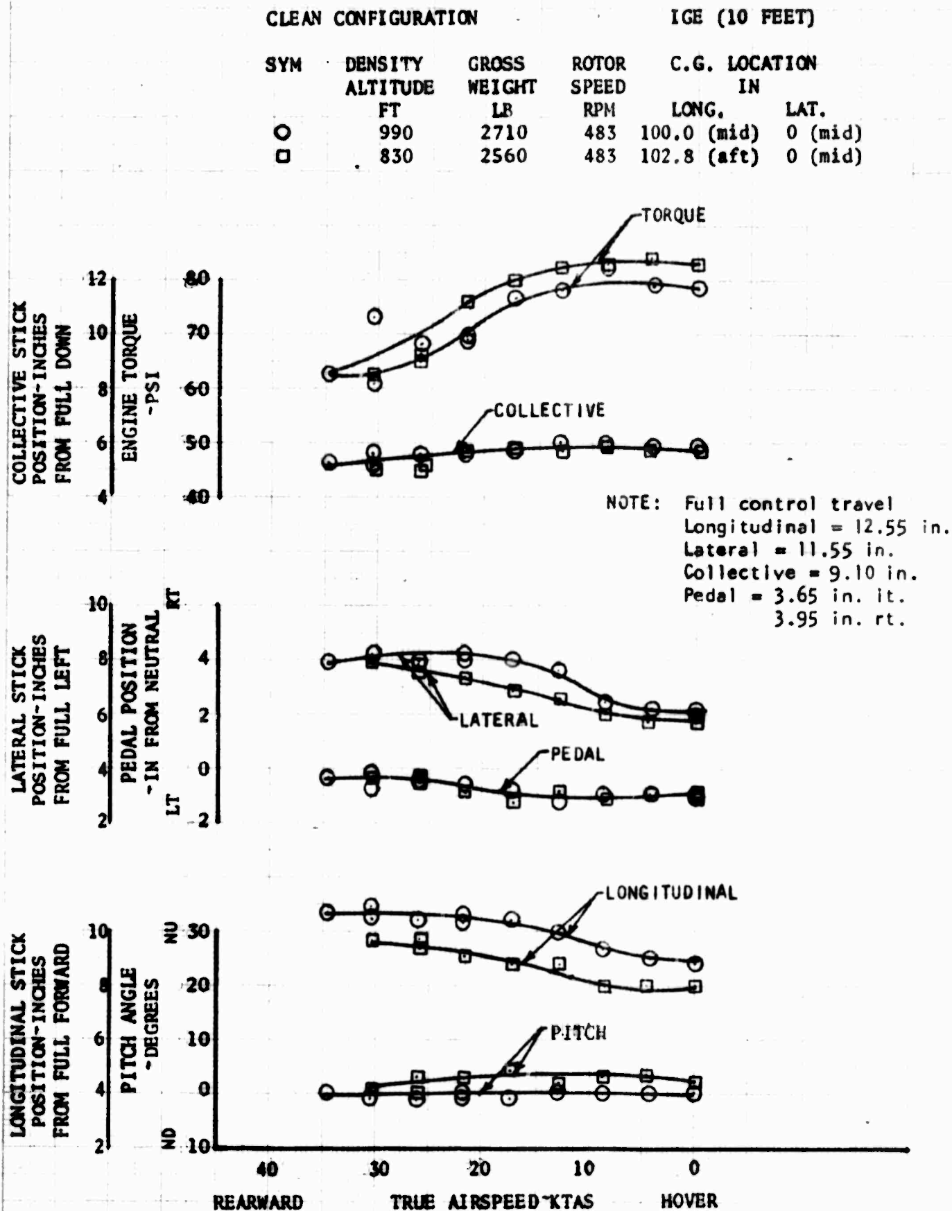
FIGURE NO. 156 CONTROL POSITIONS DURING REARWARD FLIGHT OH-6A S/N 65-12919
