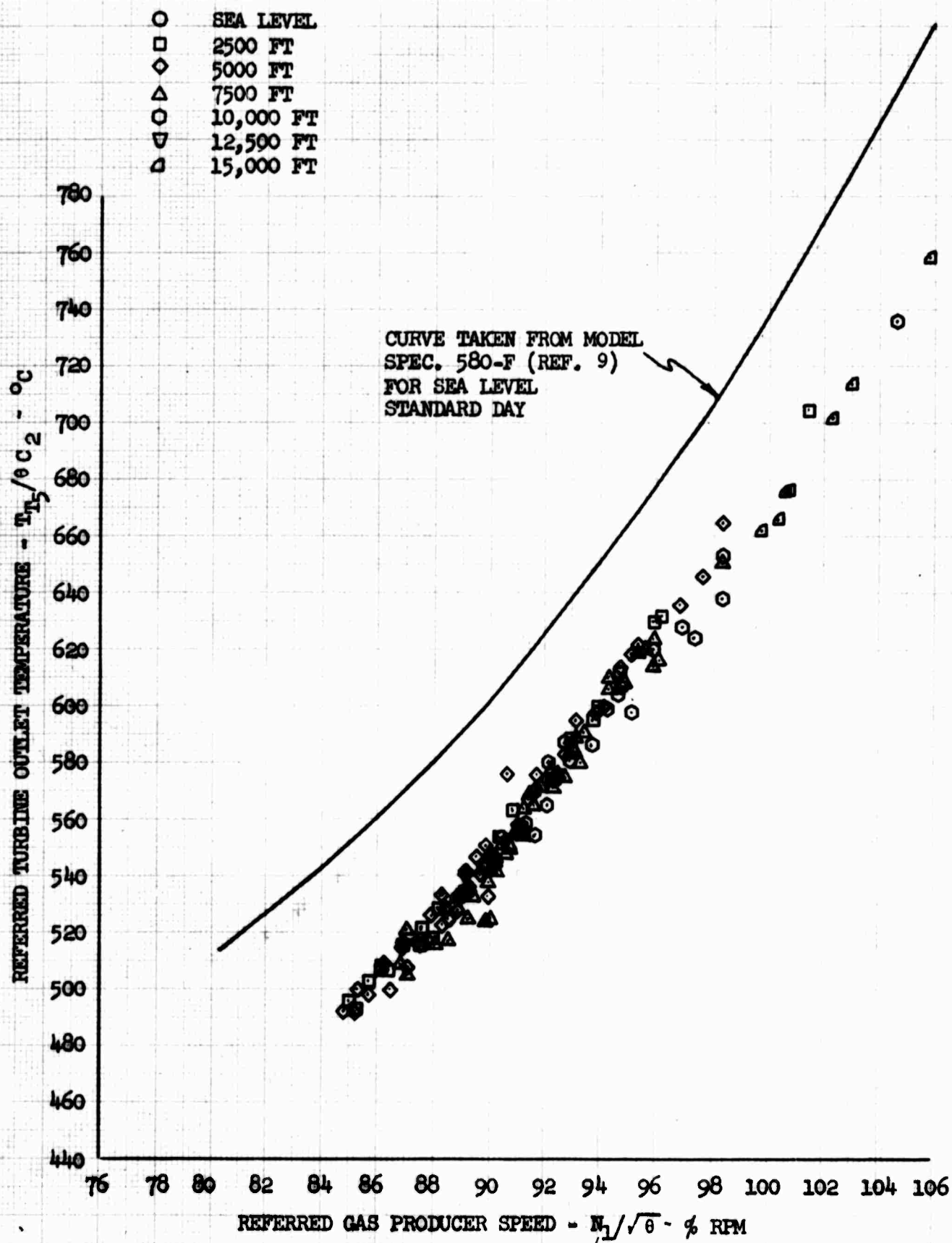
FIGURE NO. 67 ENGINE CHARACTERISTICS T63-A-5A
