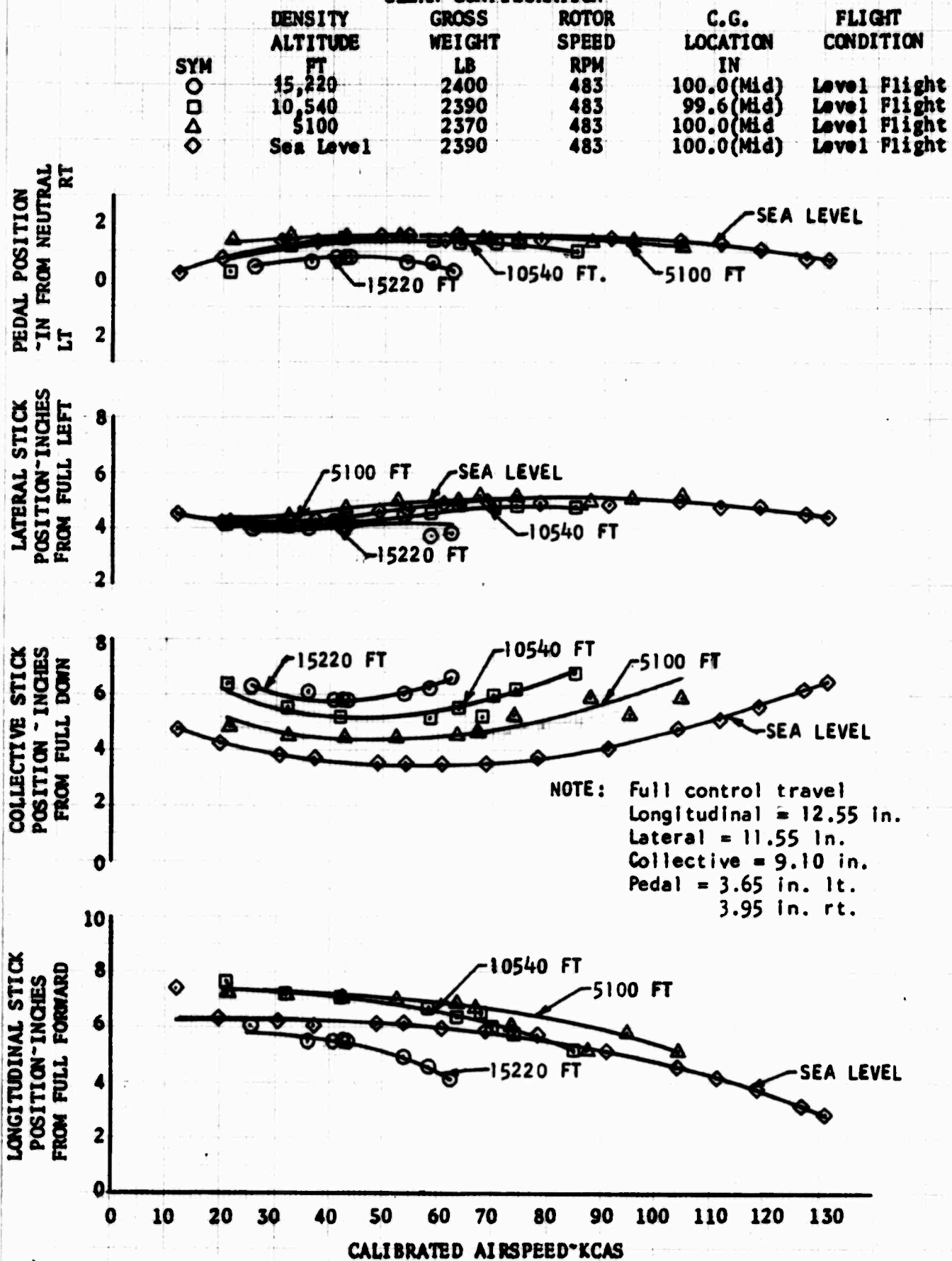
FIGURE NO. 68 CONTROL POSITION TRIM CURVES OH-6A S/N 62-12919 CLEAN CONFIGURATION
