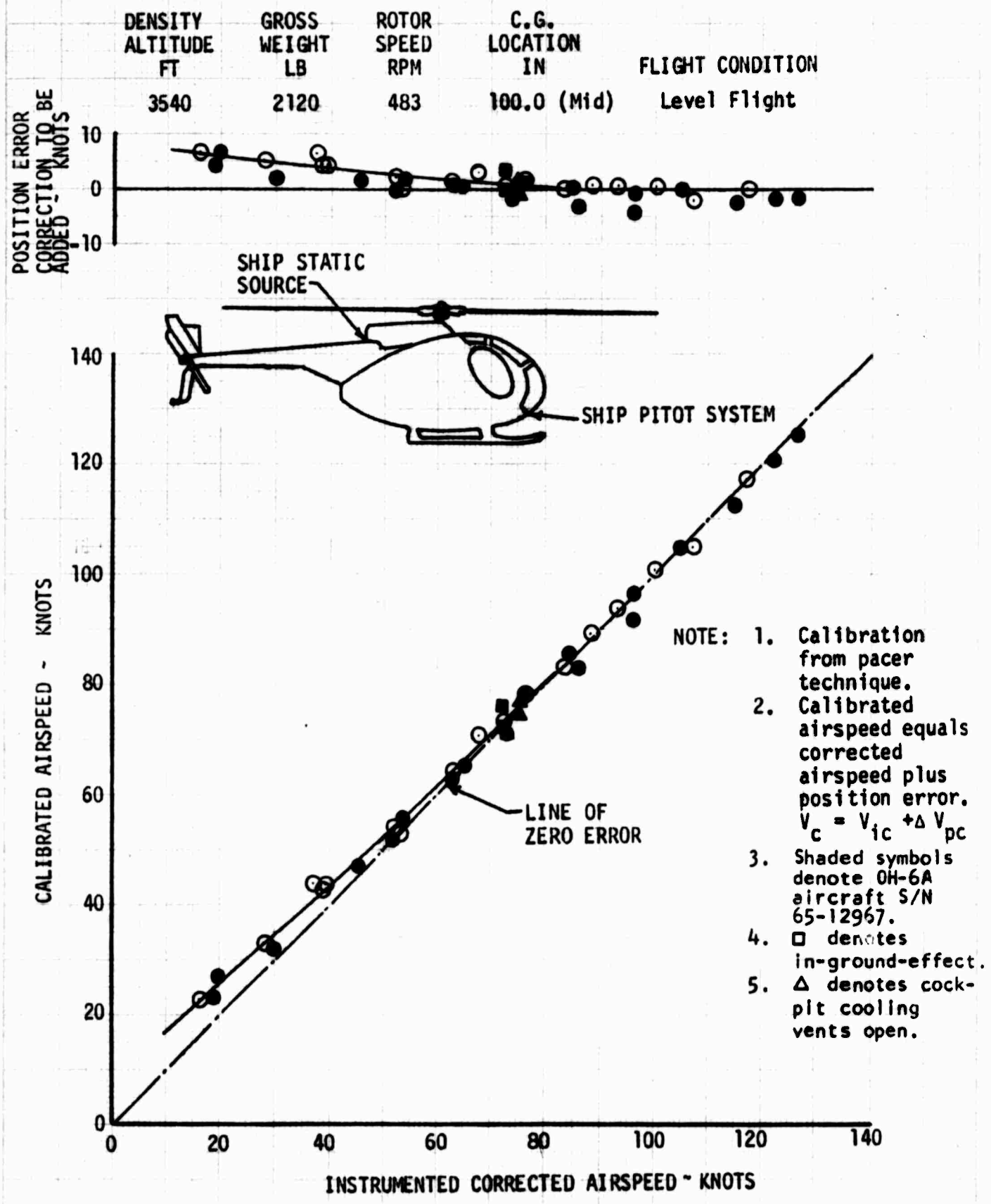
FIGURE NO. 57 AIRSPEED CALIBRATION OH-6A S/N 65-12919 STANDARD SYSTEM CLEAN CONFIGURATION
