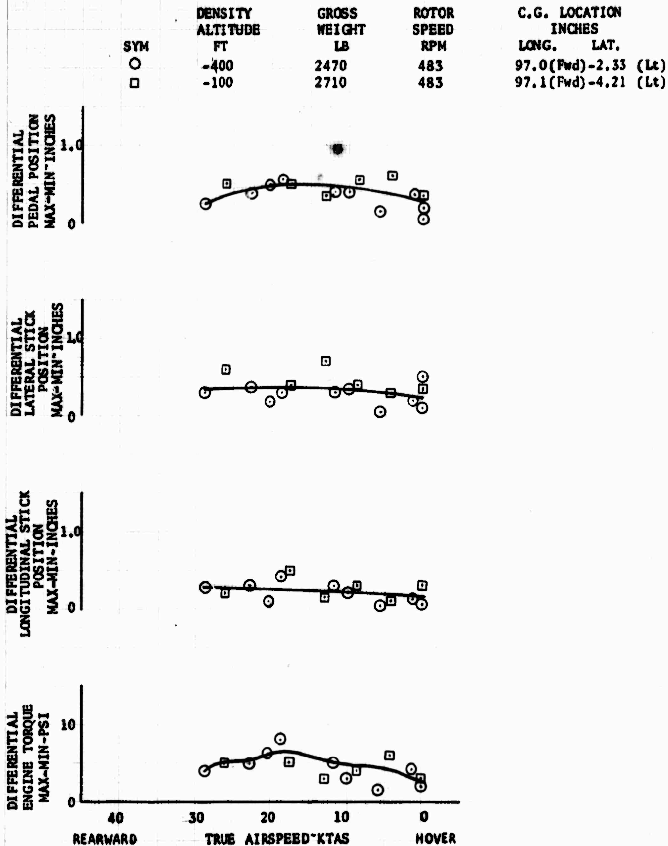
FIGURE NO. 161 CONTROL POSITION VARIATIONS DURING REARWARD FLIGHT OH-6A S/N 65-12919 CLEAN CONFIGURATION IGE (10 FEET)
