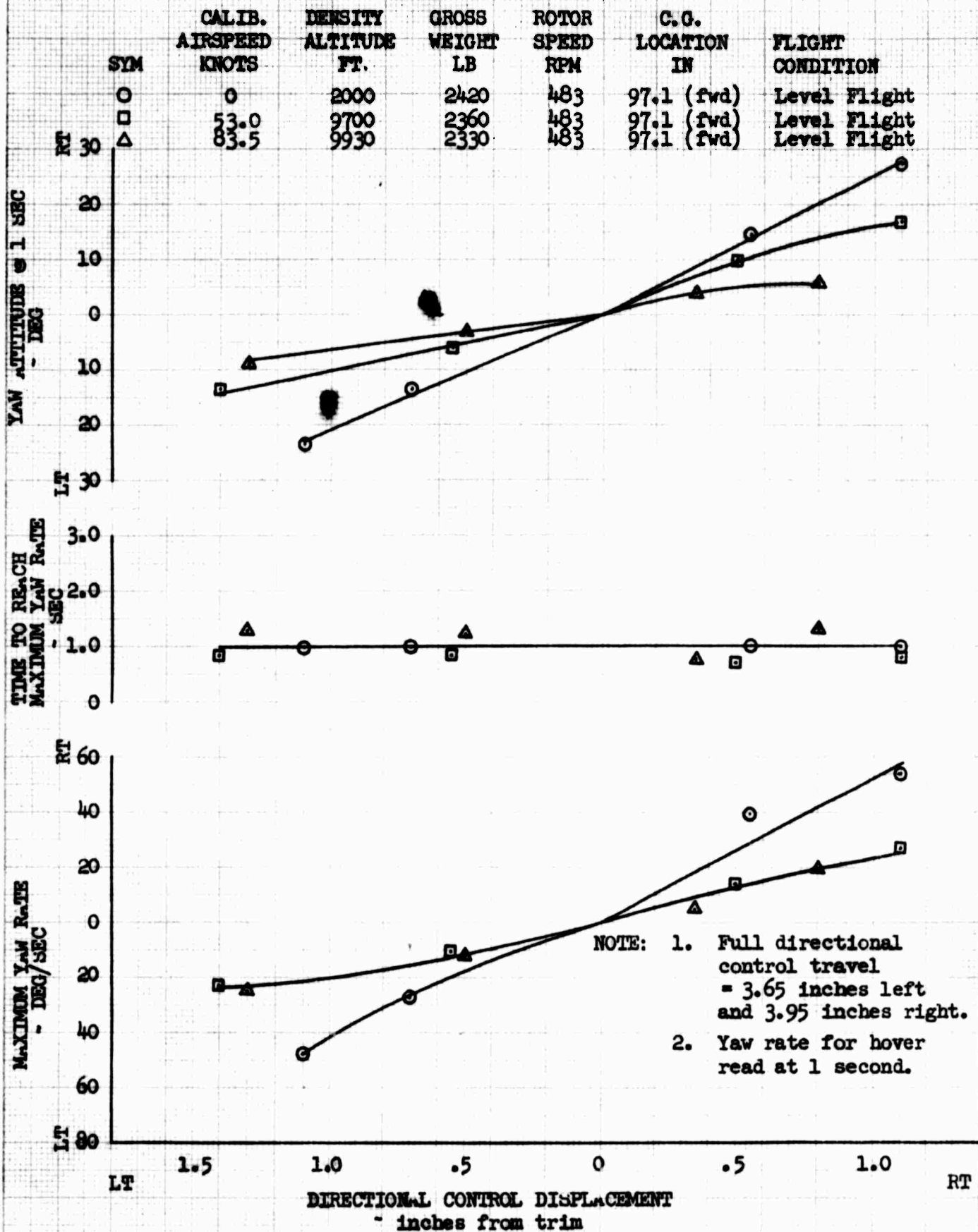
FIGURE NO. 124 DIRECTIONAL CONTROL RESPONSE OH-6A S/N 65-12919 CLEAN CONFIGURATION
