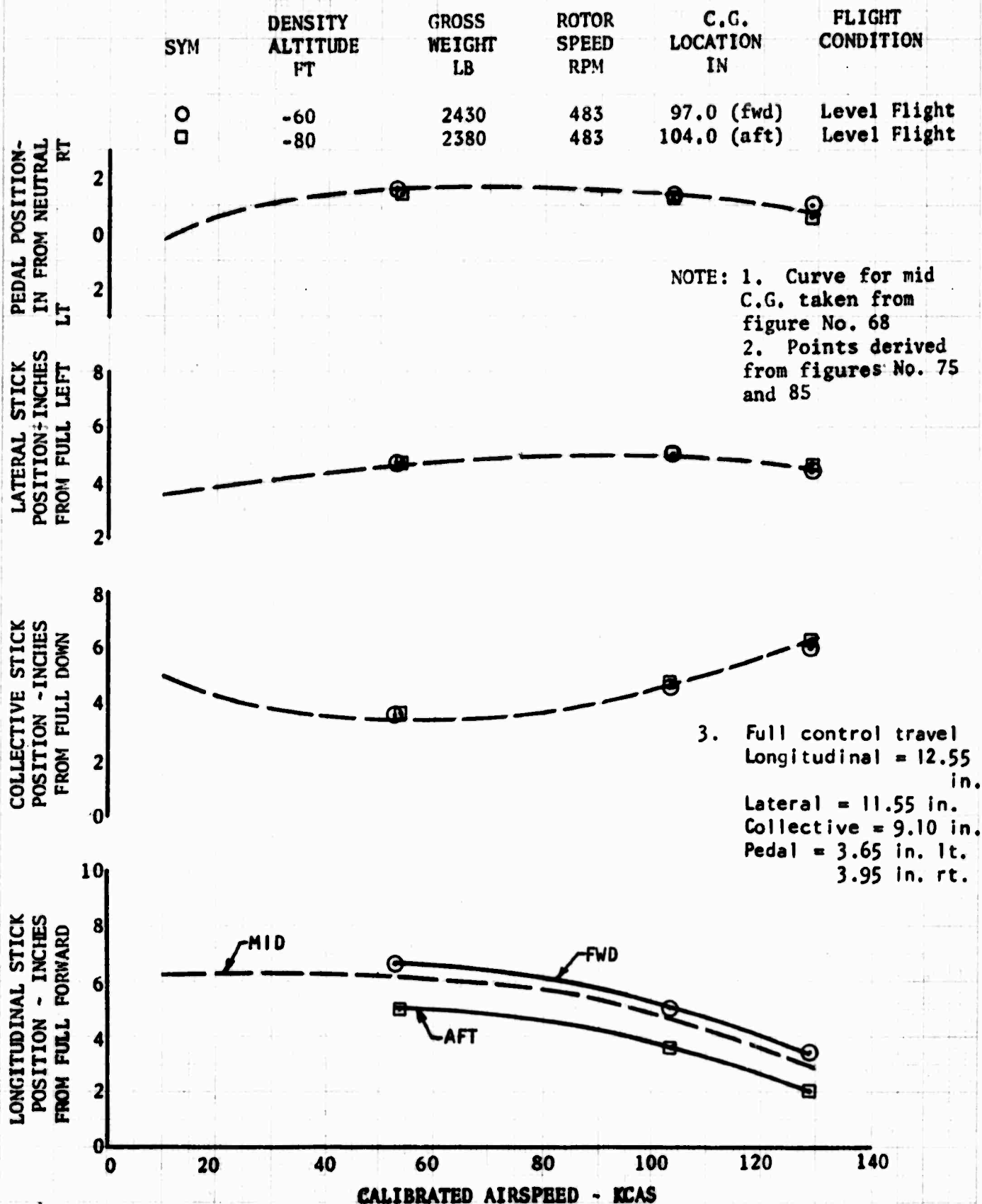
FIGURE NO. 71 CONTROL POSITION TRIM CURVES OH-6A S/N 65-12919 CLEAN CONFIGURATION
