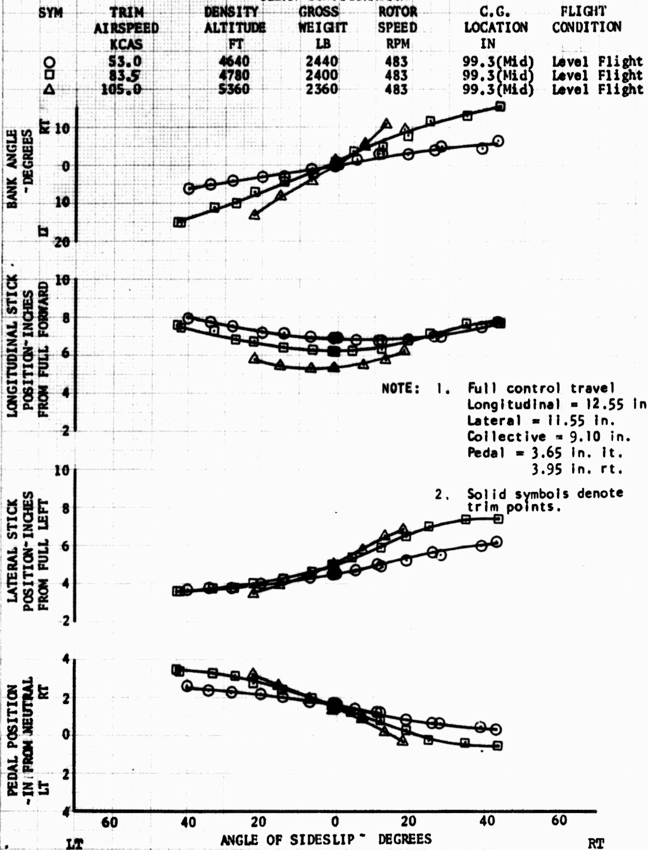
FIGURE NO. 96 STATIC LATERAL-DIRECTIONAL STABILITY OH-6A S/N 65-12919 CLEAN CONFIGURATION
