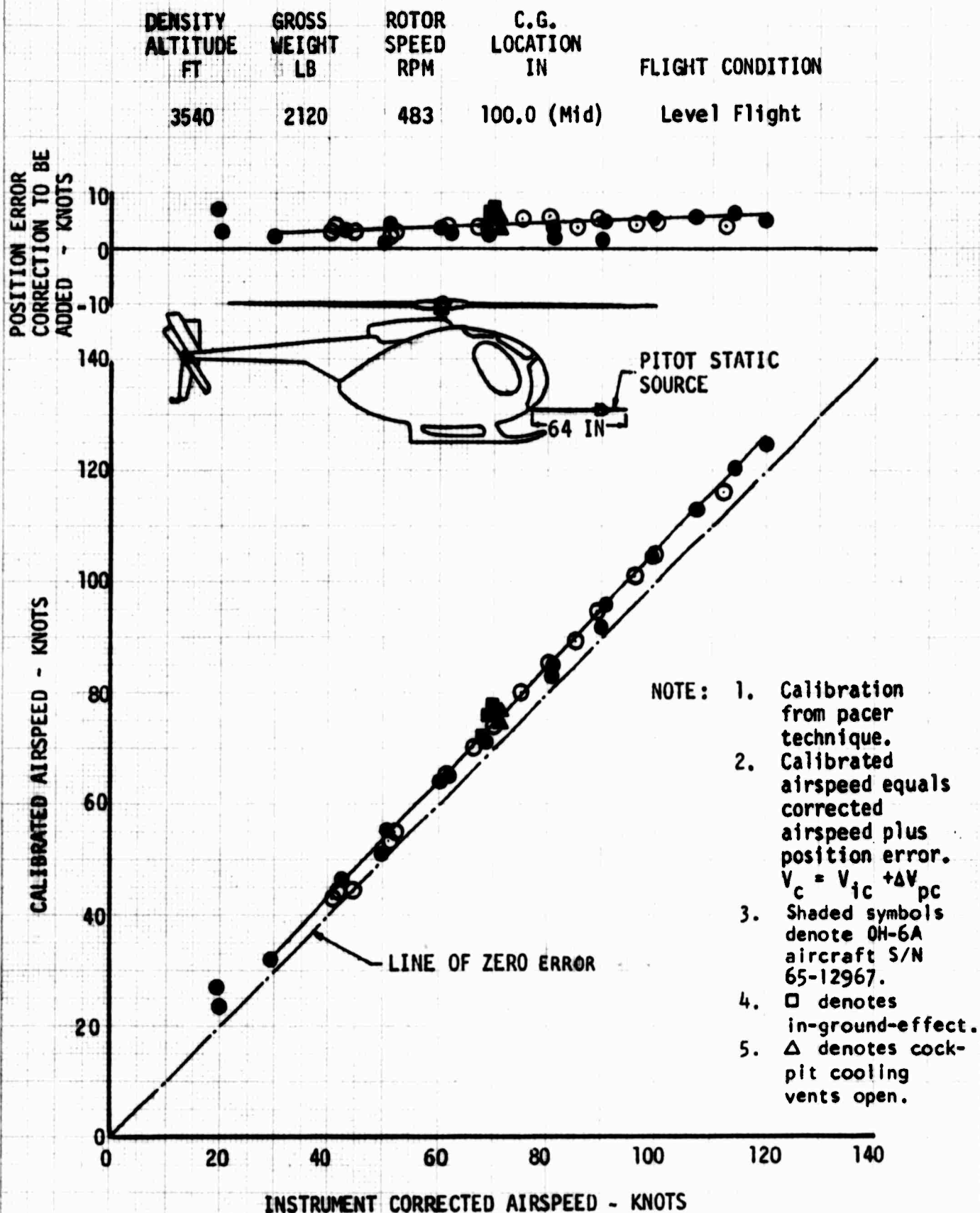
FIGURE NO. 56 AIRSPEED CALIBRATION OH-6A S/N 65-12919 CLEAN CONFIGURATION BOOM SYSTEM
