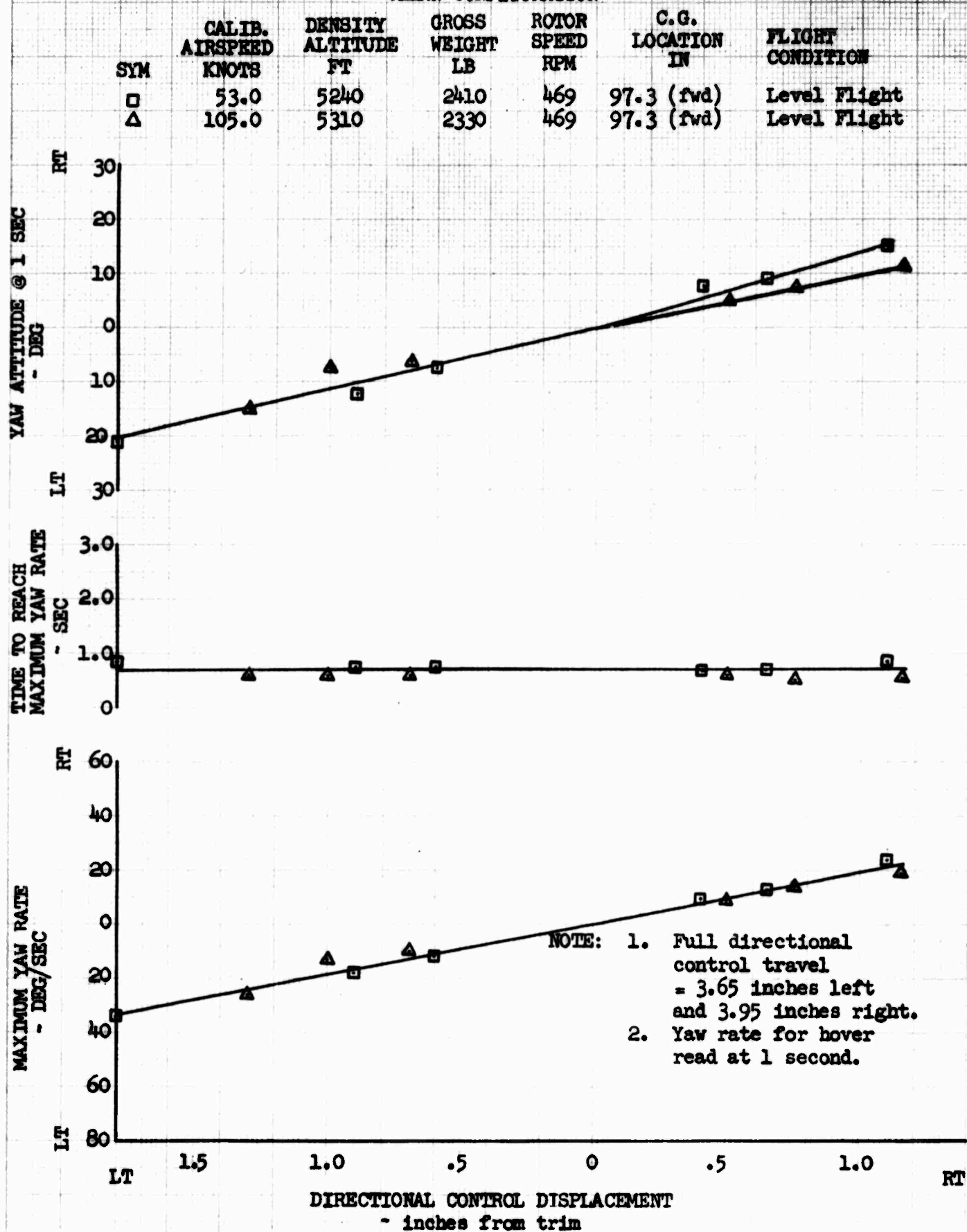
FIGURE NO. 125 DIRECTIONAL CONTROL RESPONSE OH-6A S/N 65-12919 CLEAN CONFIGURATION
