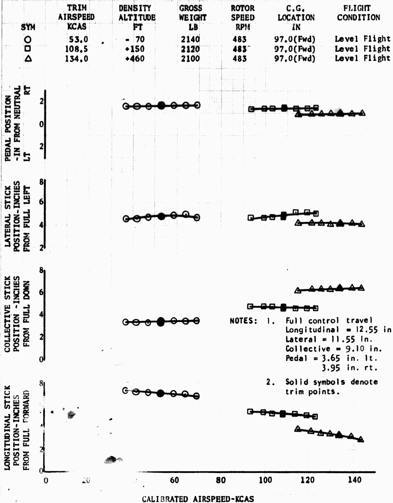
FIGURE NO. 85 STATIC LONGITUDINAL COLLECTIVE FIXED STABILITY OH-6A S/N 65-12919 CLEAN CONFIGURATION
