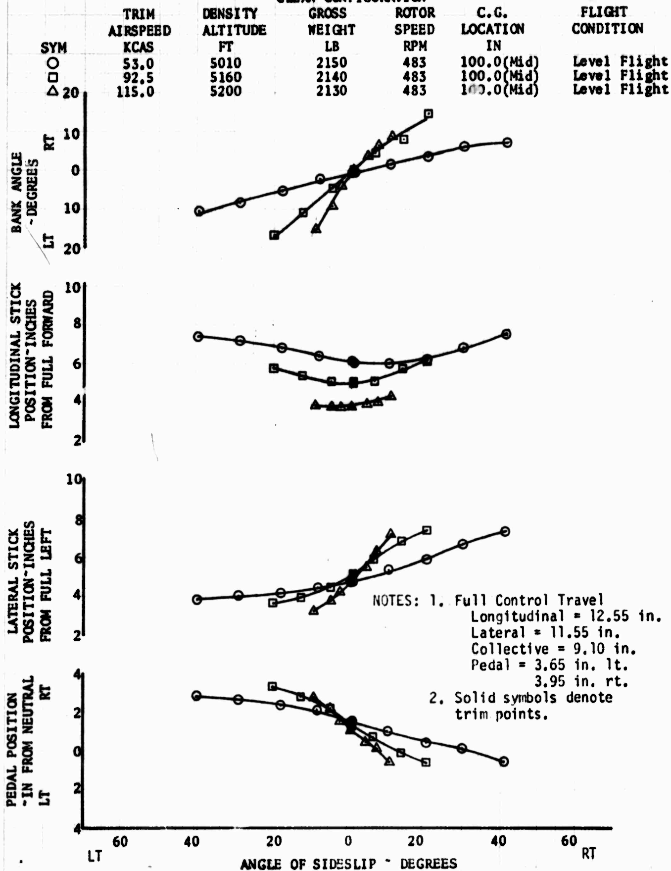
FIGURE NO. 95 STATIC LATERAL-DIRECTIONAL STABILITY OH-6A S/N 65-12919 CLEAN CONFIGURATION
