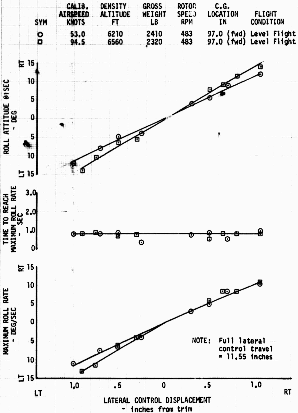
FIGURE NO. 118 LATERAL CONTROL RESPONSE OH-6A S/N 65-12919 CLEAN CONFIGURATION
