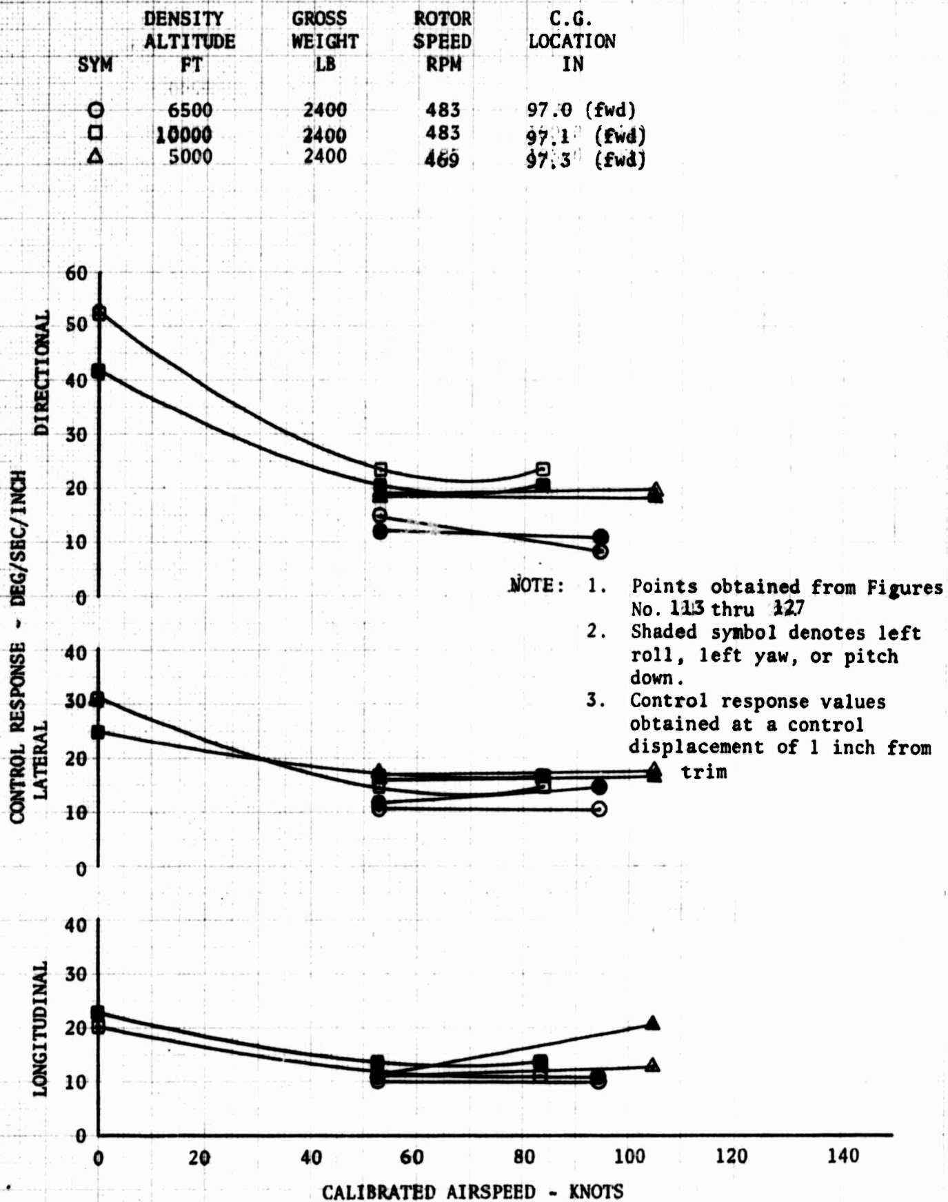
FIGURE NO. 109 SUMMARY OF CONTROL RESPONSE OH-6A S/N 65-12919 CLEAN CONFIGURATION
