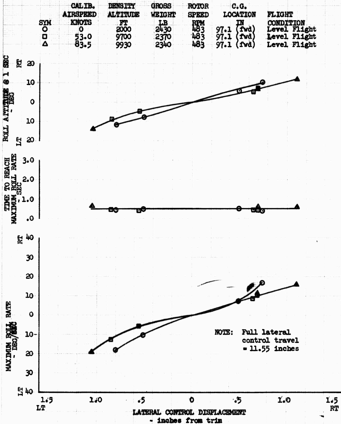
FIGURE NO. 119 LATERAL CONTROL RESPONSE OH-6A S/N 65-12919 CLEAN CONFIGURATION
