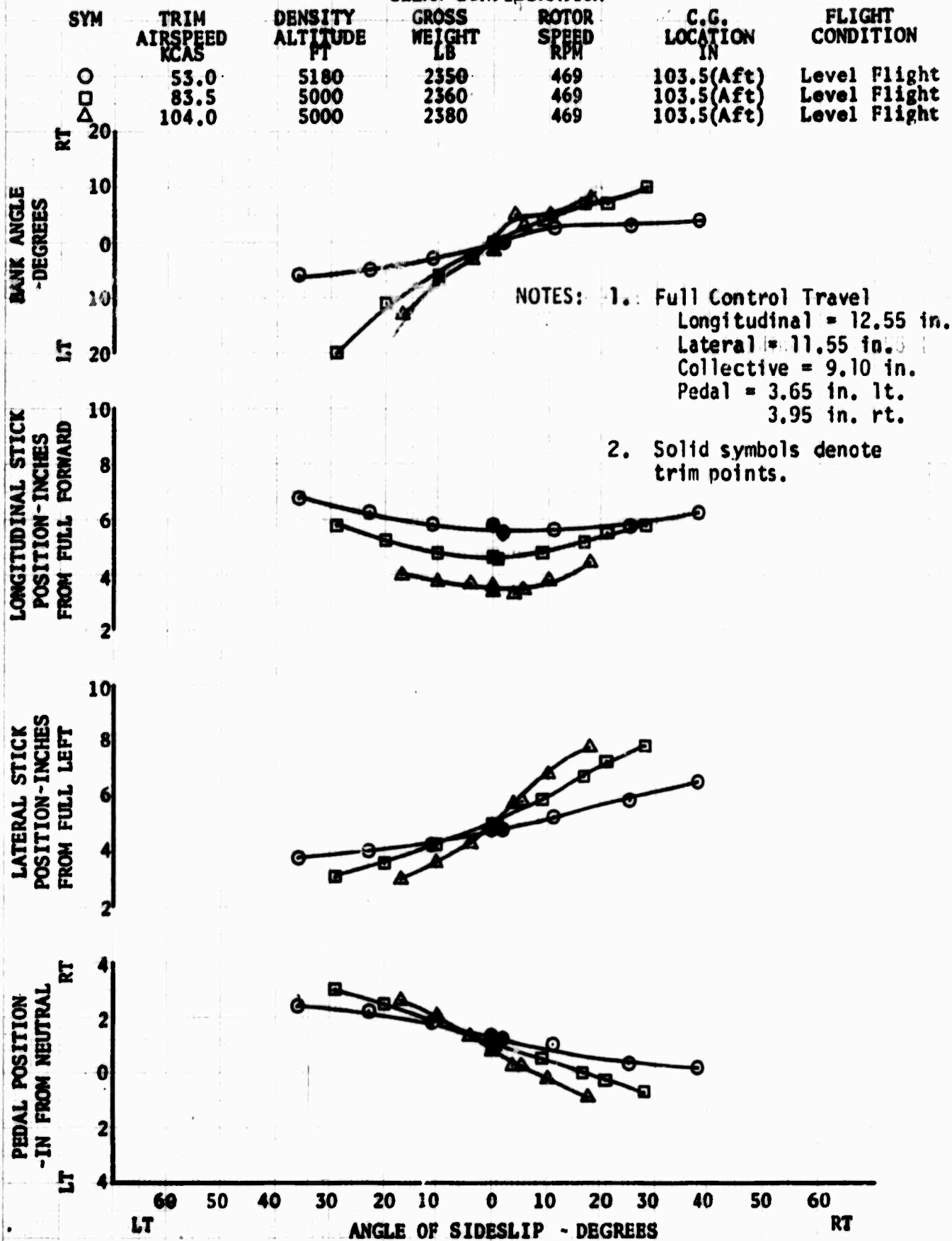
FIGURE NO. 94 STATIC LATERAL-DIRECTIONAL STABILITY OH-6A S/N 65-12919 CLEAN CONFIGURATION
