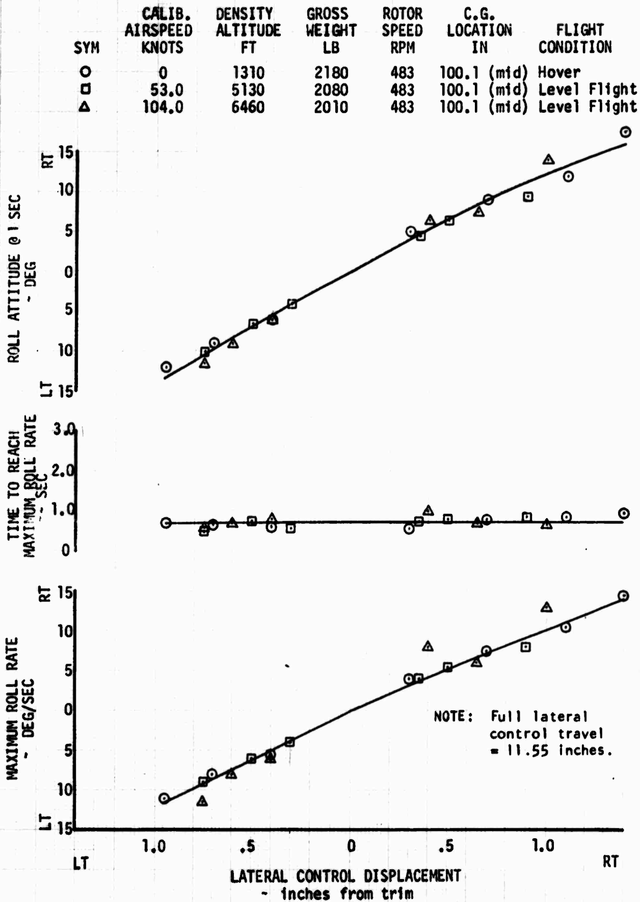
FIGURE NO. 121 LATERAL CONTROL RESPONSE OH-6A S/N 65-12919 CLEAN CONFIGURATION
