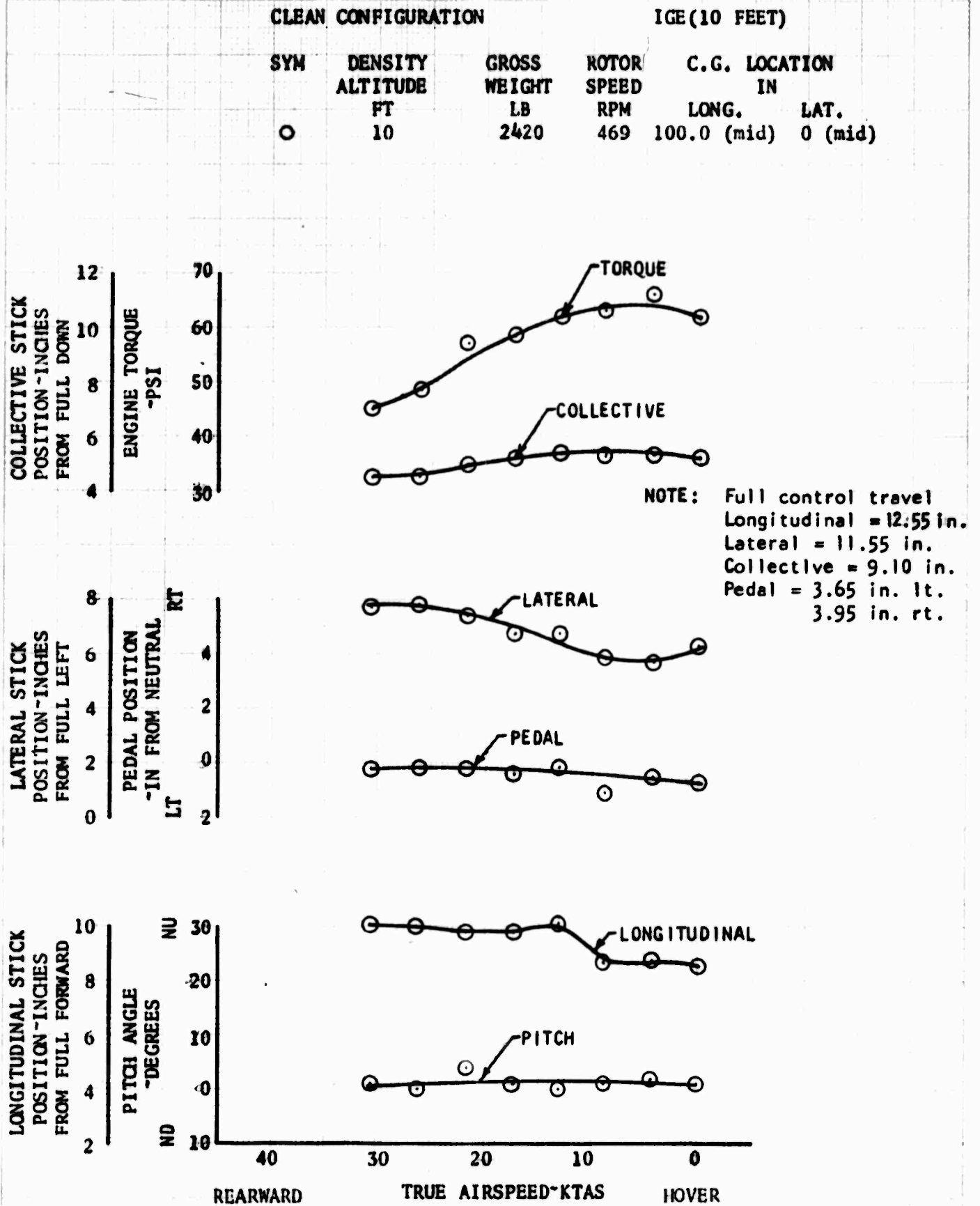
FIGURE NO. 158 CONTROL POSITIONS DURING REARWARD FLIGHT OH-6A S/N 65-12919
