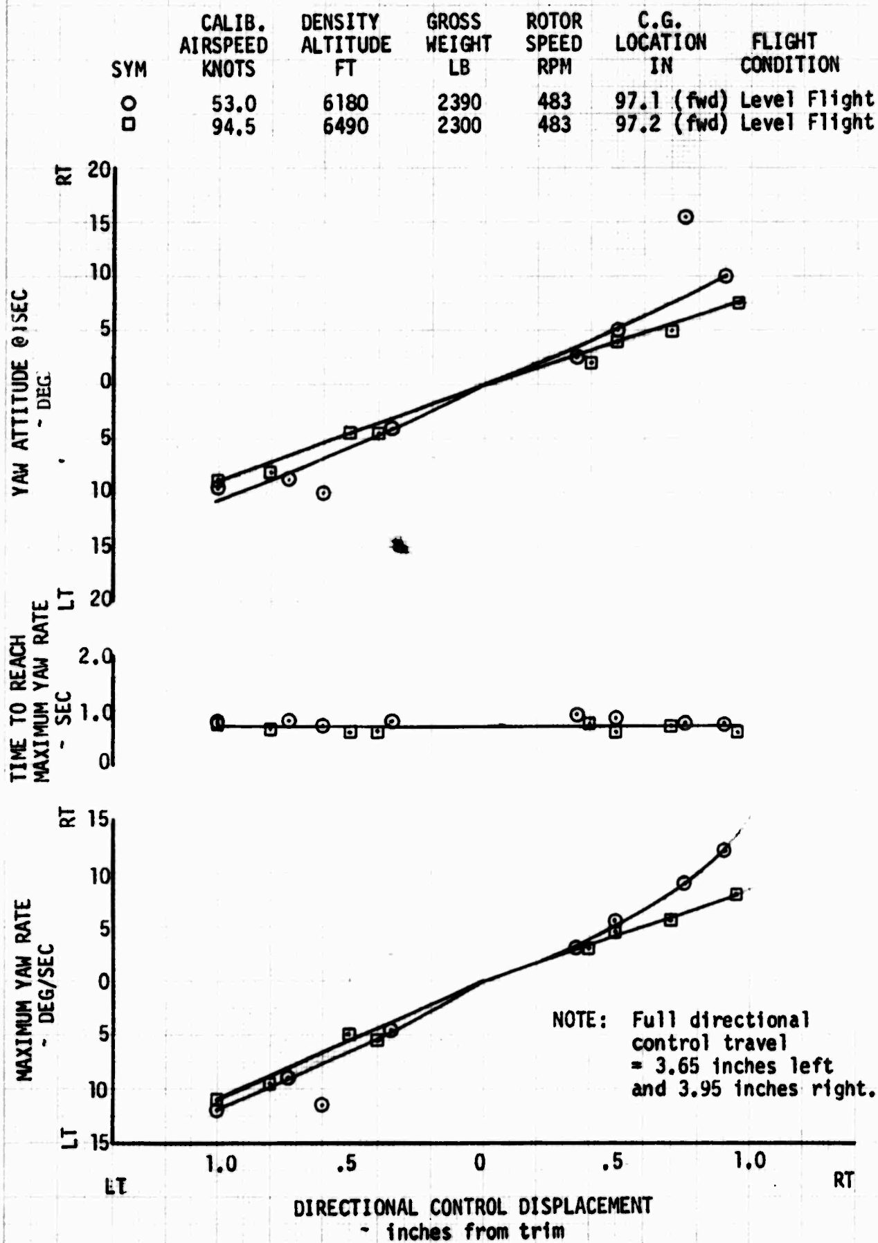
FIGURE NO. 123 DIRECTIONAL CONTROL RESPONSE OH-6A S/N 65-12919 CLEAN CONFIGURATION
