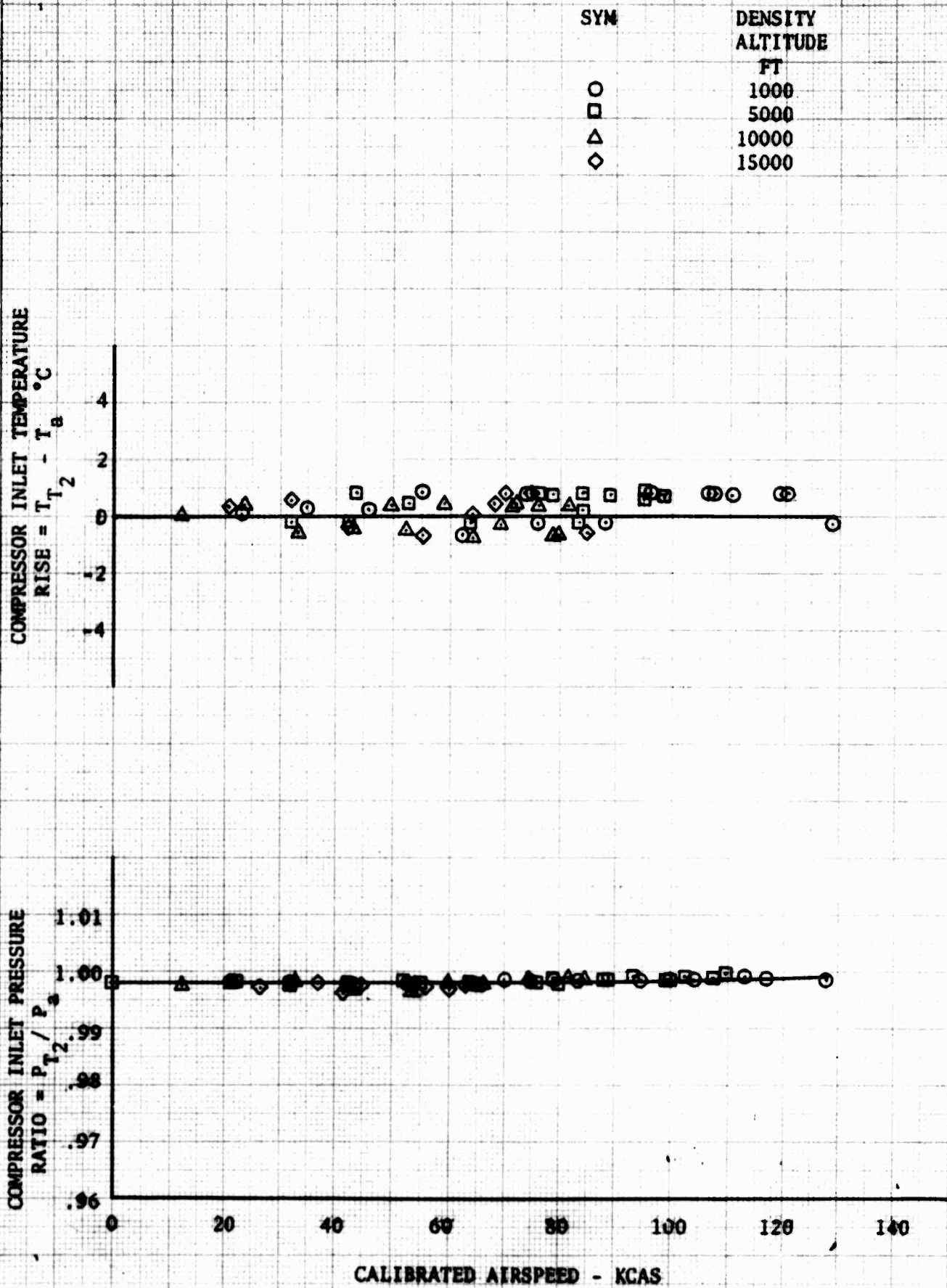
FIGURE NO. 62 INLET PERFORMANCE OH-6A S/N 65-12919
