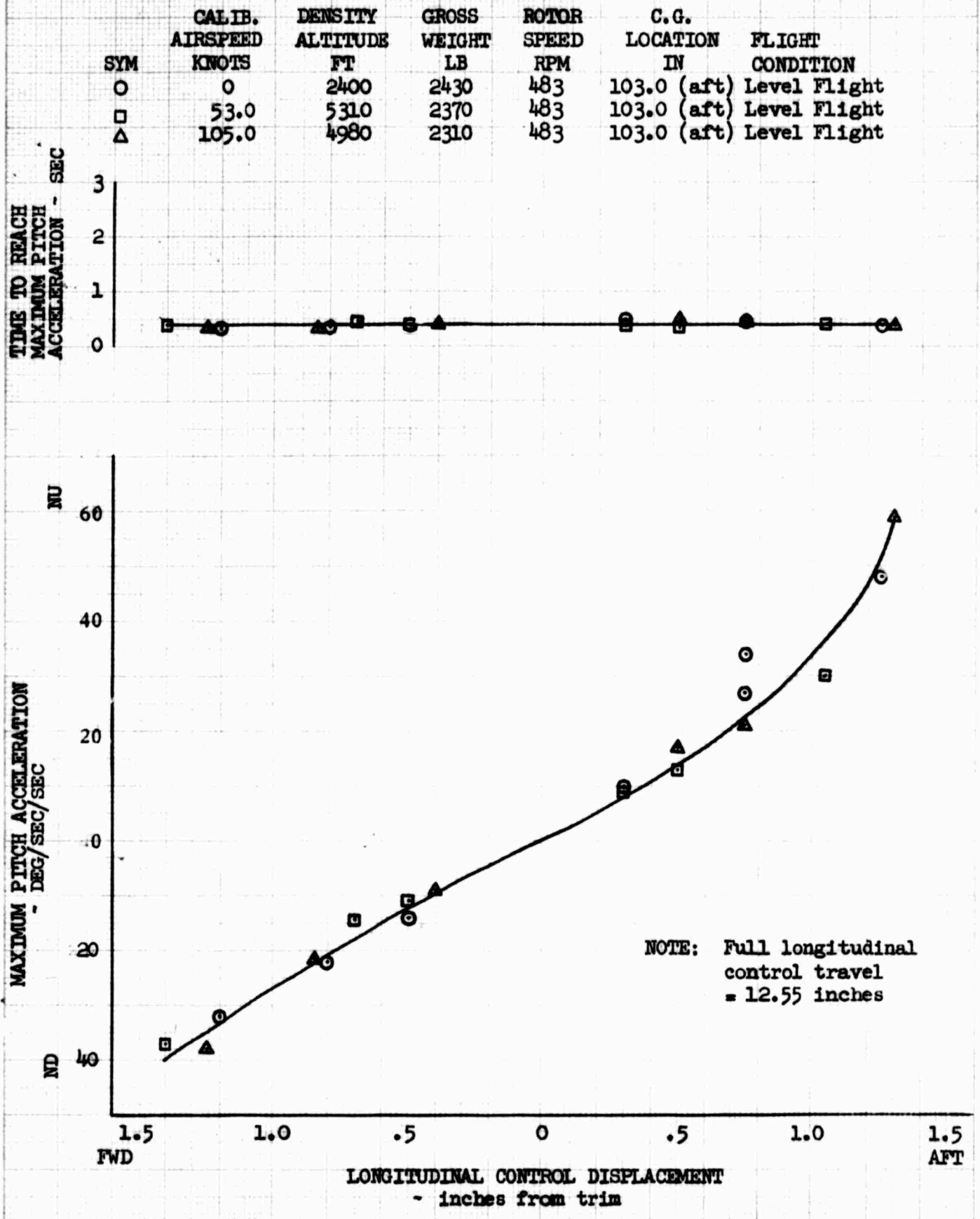
FIGURE NO. 132 LONGITUDINAL CONTROL SENSITIVITY OH-6A S/N 65-12919 CLEAN CONFIGURATION
