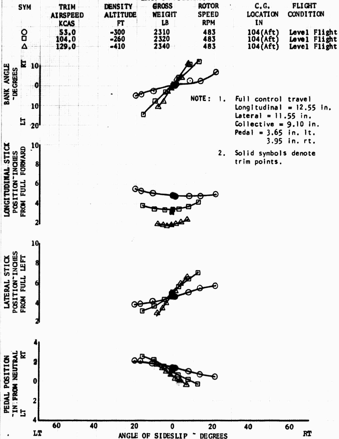
FIGURE NO. 90 STATIC LATERAL-DIRECTIONAL STABILITY OH-6A S/N 65-12919 CLEAN CONFIGURATION
