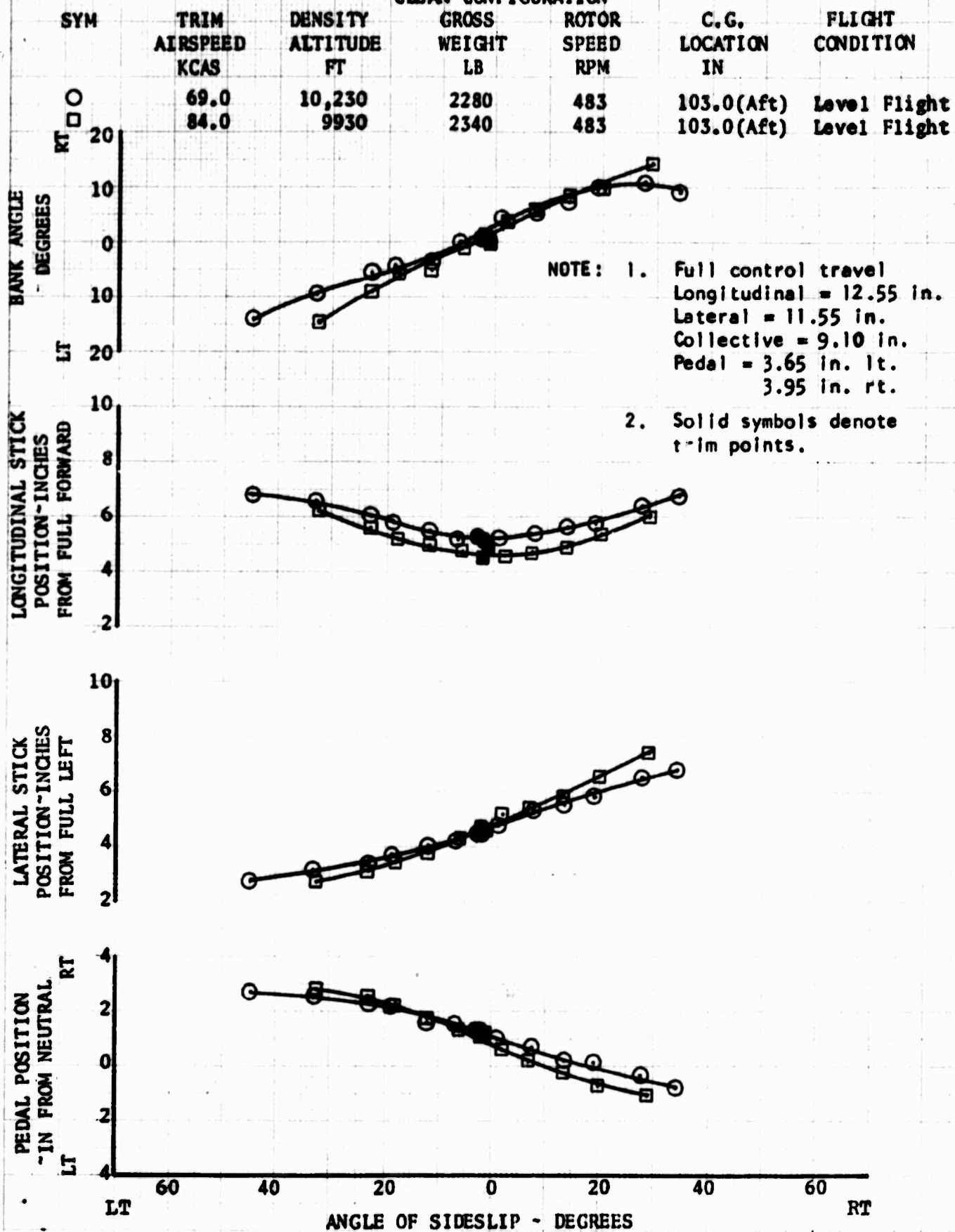
FIGURE NO. 92 STATIC LATERAL-DIRECTIONAL STABILITY OH-6A S/N 65-12919 CLEAN CONFIGURATION
