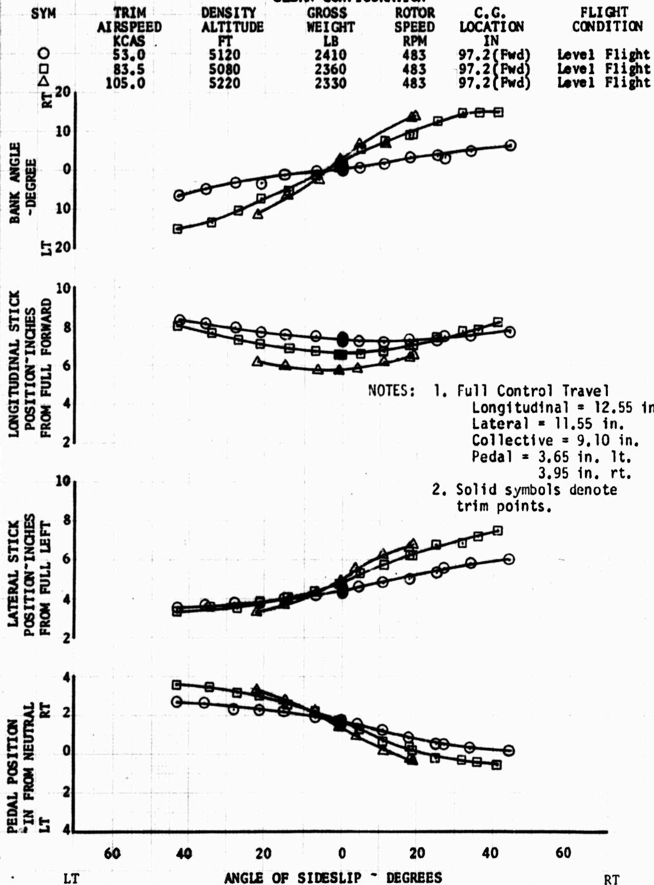
FIGURE NO. 89 STATIC-LATERAL-DIRECTIONAL STABILITY OH-6A S/N 65-12919 CLEAN CONFIGURATION
