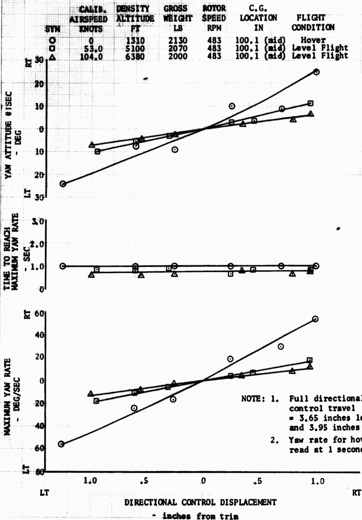
FIGURE NO. 126 DIRECTIONAL CONTROL RESPONSE OH-6A S/N 65-12919 CLEAN CONFIGURATION
