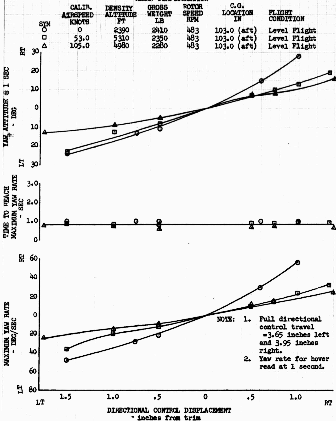
FIGURE NO. 127 DIRECTIONAL CONTROL RESPONSE OH-6A S/N 69-12919 CLEAN CONFIGURATION
