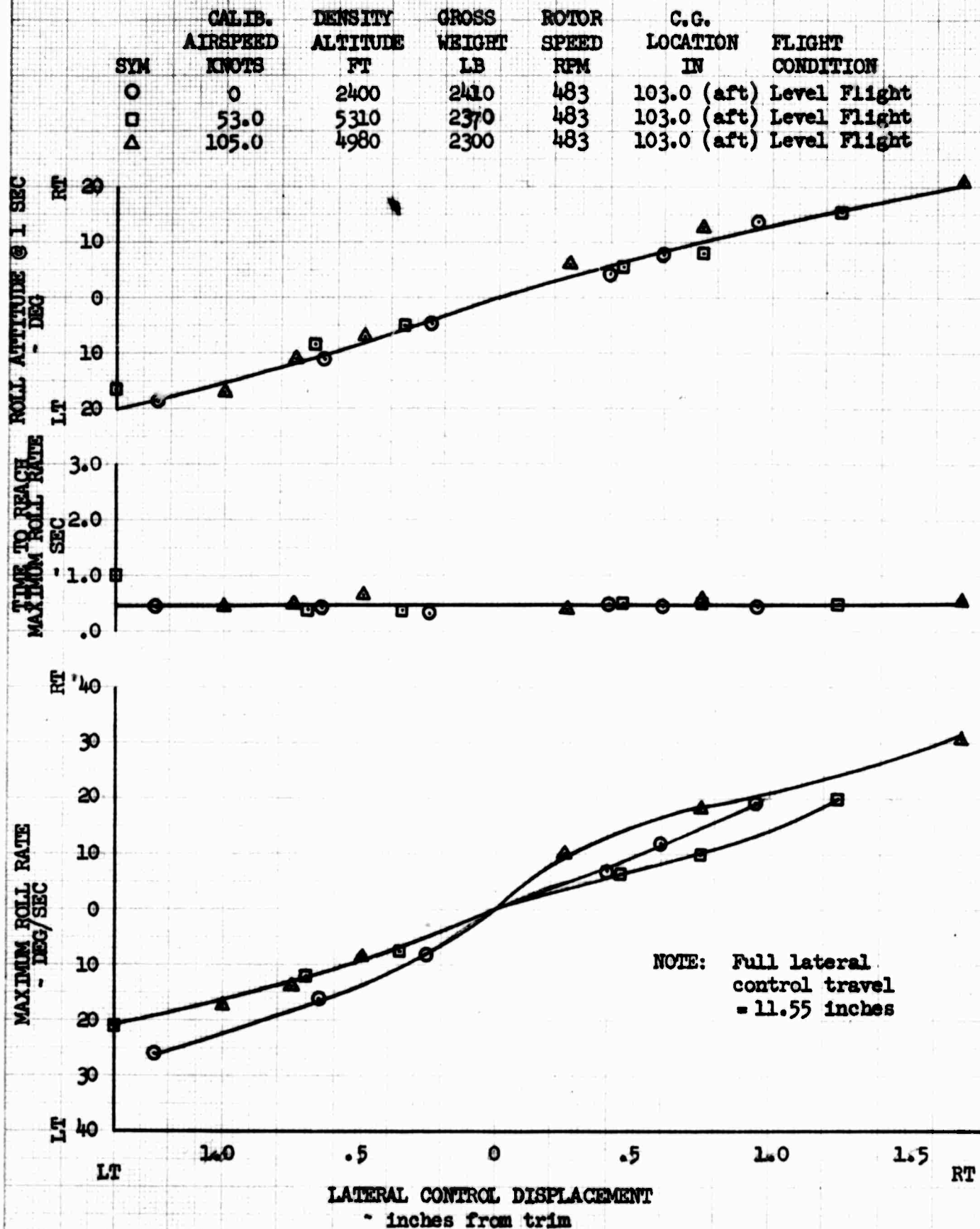
FIGURE NO. 122 LATERAL CONTROL RESPONSE OH-6A S/N 65-12919 CLEAN CONFIGURATION
