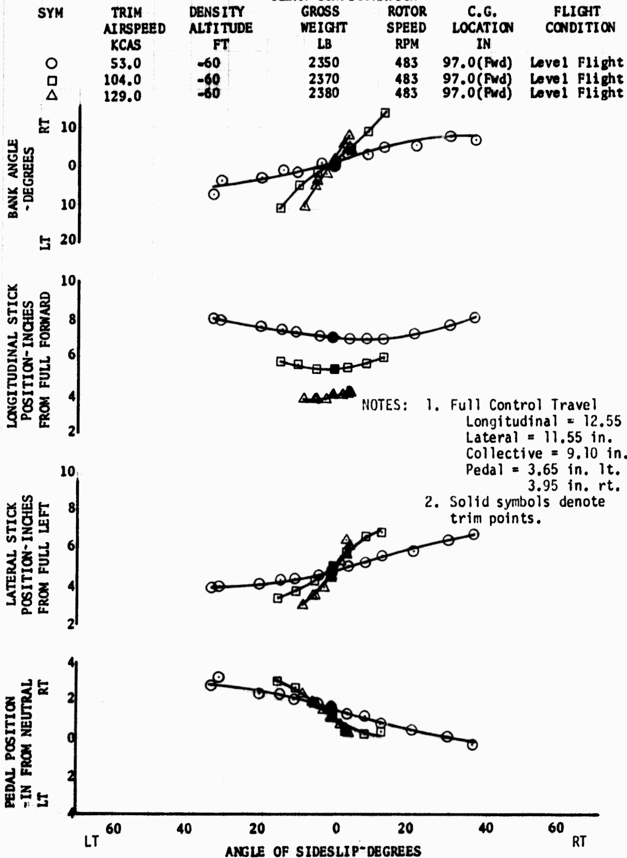
FIGURE NO. 98 STATIC LATERAL-DIRECTIONAL STABILITY OH-6A S/N 65-12919 CLEAN CONFIGURATION
