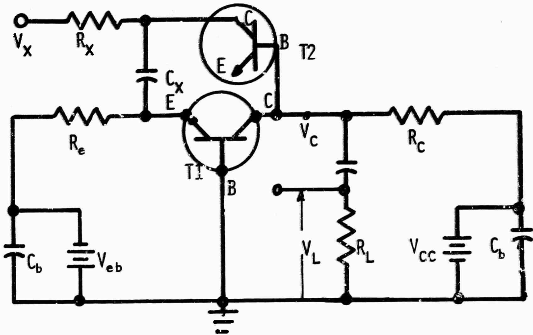
Figure 24. Circuit for Common-Base Amplifier with Collector-to-Emitter Compensation
