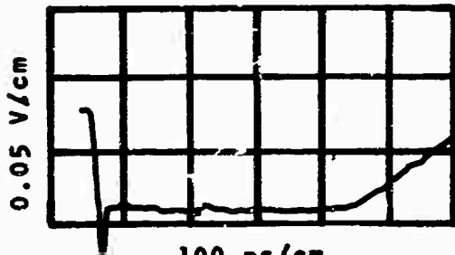
100 ns/cm c) V_b=2.5, V_x=18
