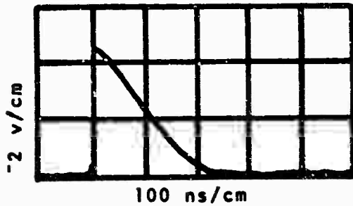
b) V_b=0.23 , Diodes Out
