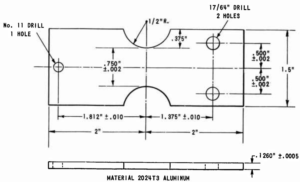
Figure 2. FATIGUE SPECIMEN (FULL SIZE).
