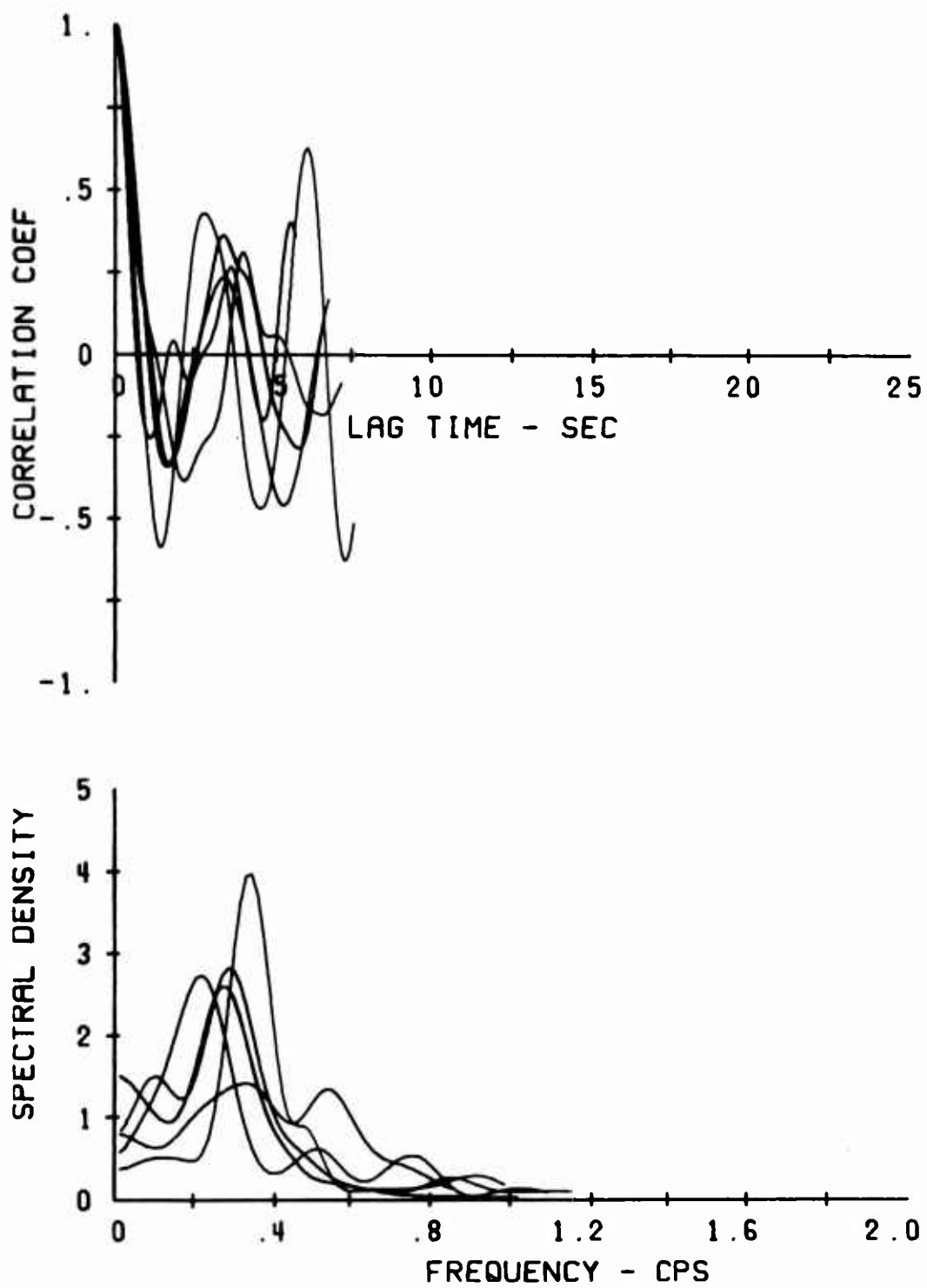
FIGURE 99. LONGITUDINAL STICK PSD, RIGHT HOVER TURN, PILOT 1, WING AND TAIL OFF
