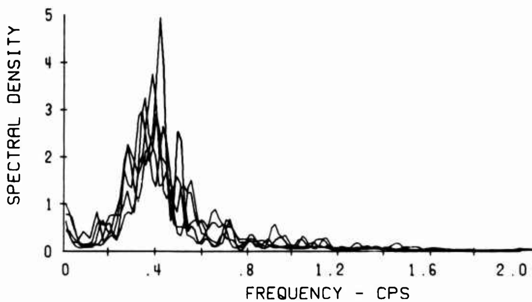
FIGURE 79. LONGITUDINAL STICK PSD, IGE HOVER, PILOT 3, WING AND TAIL OFF
