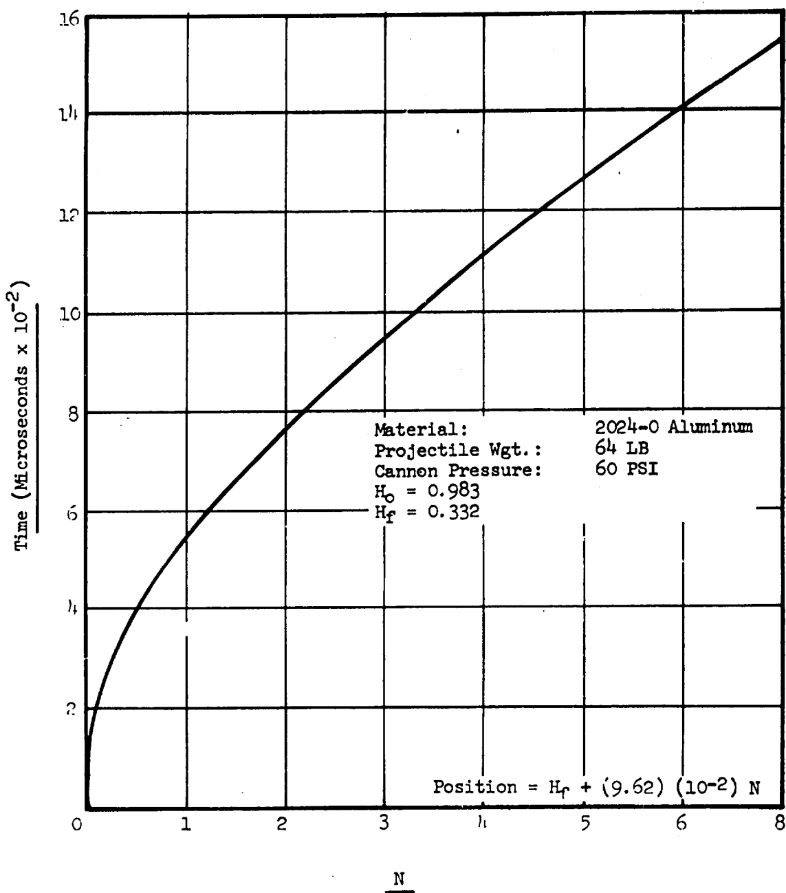
GRAPH 39. POSITION - TIME CURVE FOR SPECIMEN NUMBER A7-925
