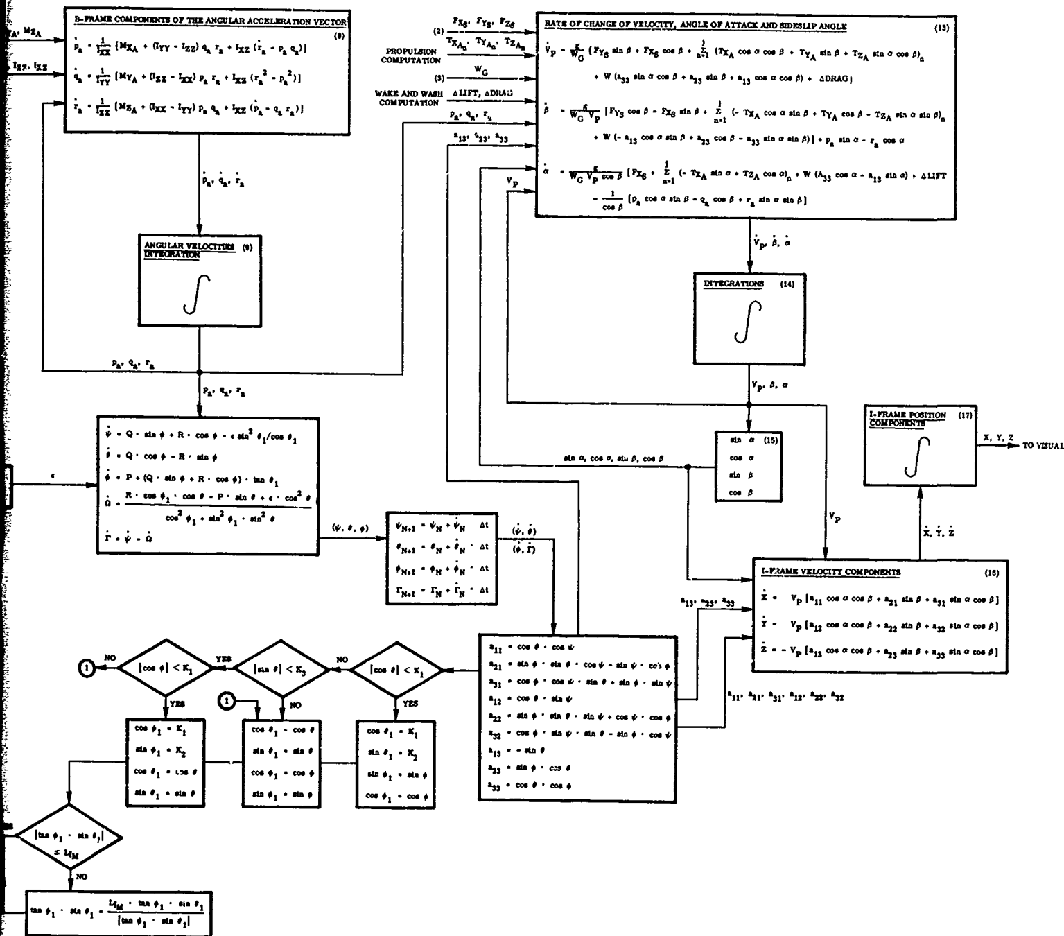
Figure 6 HIGH-FIDELITY SIMULATOR FLIGHT COMPUTATION SYSTEM
