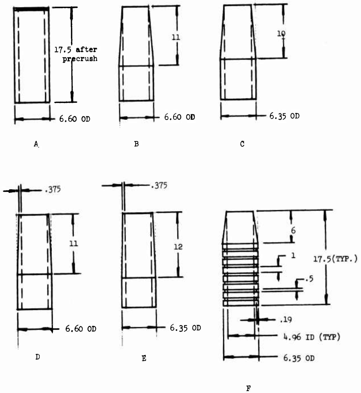
Figure 7 Configurations of the Buffer Test Items
