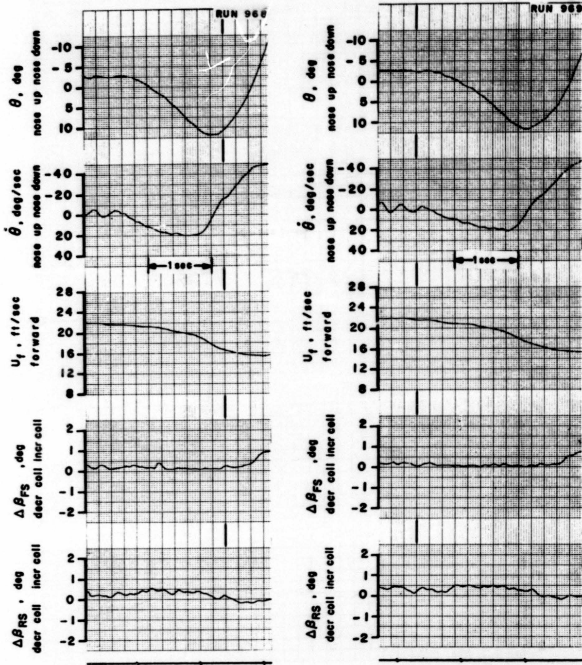
Figure 19. Self-Excited Transient Responses. Two Degrees of Freedom, \theta-U_f . K_{\theta} = 0.021 sec. i_d = 70^\circ , \theta_{.75R} = 26.2^\circ , rpm = 6780.
